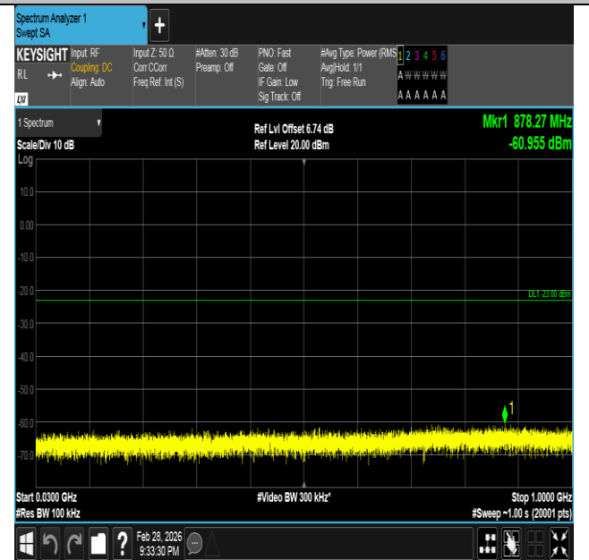
Band66-3MHz-16QAM-132657-1RB#0-30~1000-PASS
