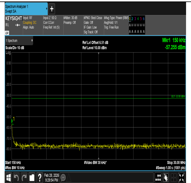
Band66-3MHz-16QAM-132322-1RB#14-0.15~30-PASS
