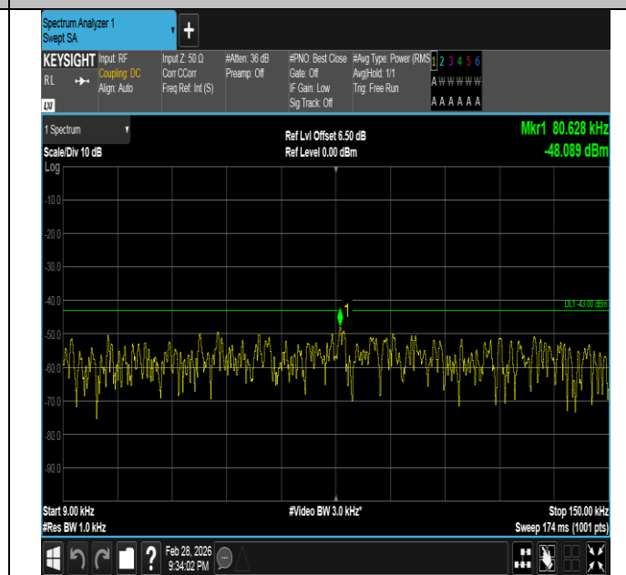
Band66-3MHz-QPSK-132657-1RB#14-0.009~0.15-PASS
