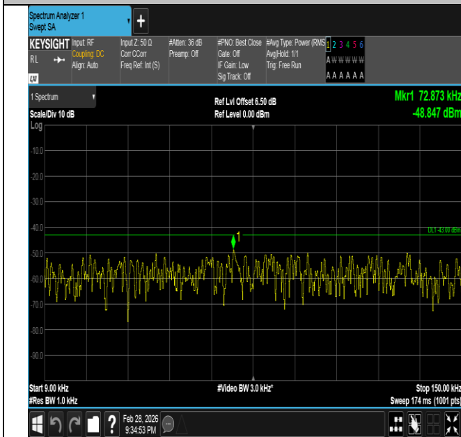
Band66-3MHz-16QAM-132657-1RB#14-0.009~0.15-PASS
