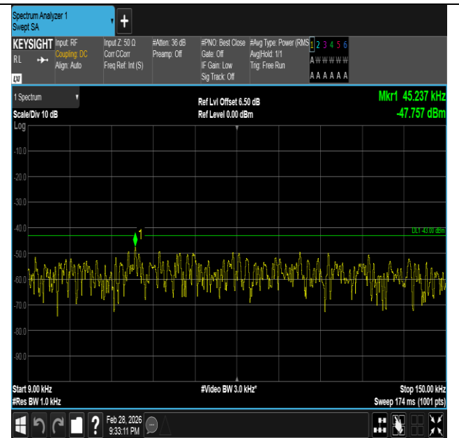
Band66-3MHz-16QAM-132657-1RB#0-0.009~0.15-PASS
