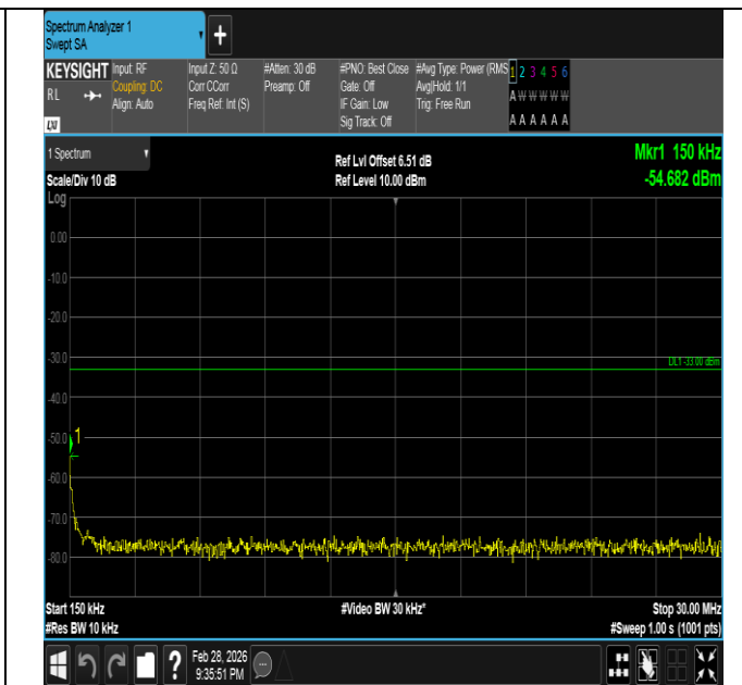
Band66-3MHz-QPSK-132657-15RB#0-0.15~30-PASS
