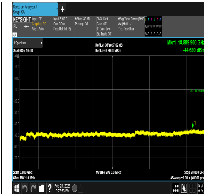
Band66-3MHz-QPSK-132322-1RB#0-3000~20000-PASS
