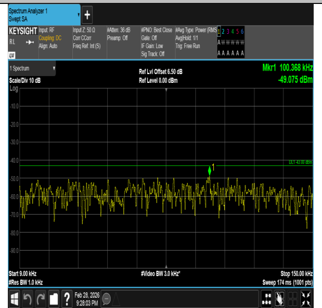
Band66-3MHz-16QAM-132322-1RB#0-0.009~0.15-PASS
