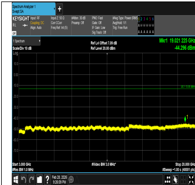
Band66-3MHz-QPSK-131987-15RB#0-3000~20000-PASS
