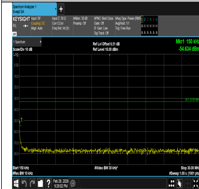
Band66-3MHz-QPSK-132322-1RB#14-0.15~30-PASS
