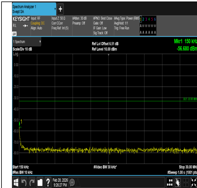
Band66-3MHz-16QAM-131987-15RB#0-0.15~30-PASS
