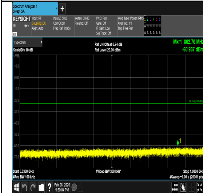
Band66-3MHz-16QAM-132322-1RB#14-30~1000-PASS
