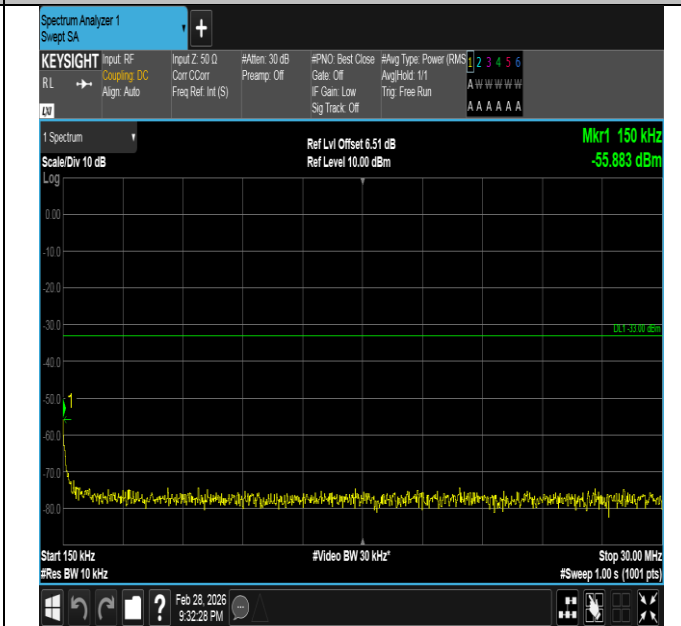
Band66-3MHz-QPSK-132657-1RB#0-0.15~30-PASS
