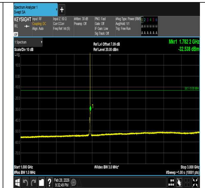
Band66-3MHz-QPSK-132657-1RB#0-1000~3000-PASS
