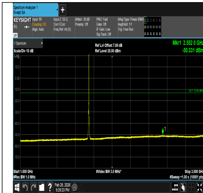
Band66-3MHz-QPSK-132322-1RB#14-1000~3000-PASS
