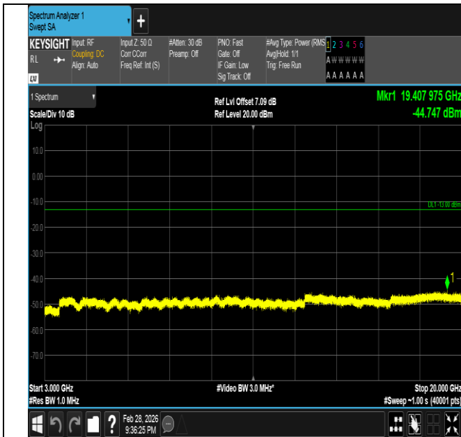
Band66-3MHz-QPSK-132657-15RB#0-3000~20000-PASS
