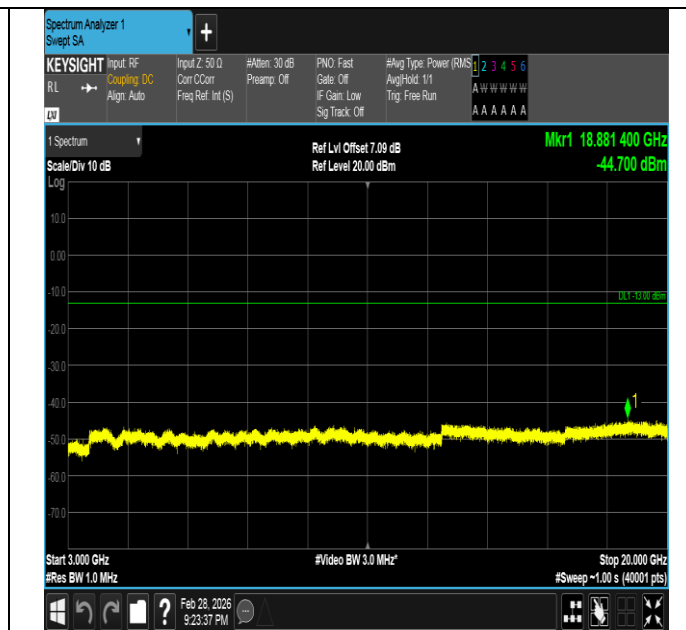
Band66-3MHz-16QAM-131987-1RB#0-3000~20000-PASS
