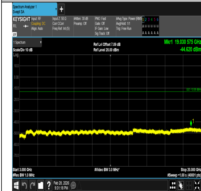
Band66-3MHz-QPSK-132322-15RB#0-3000~20000-PASS
