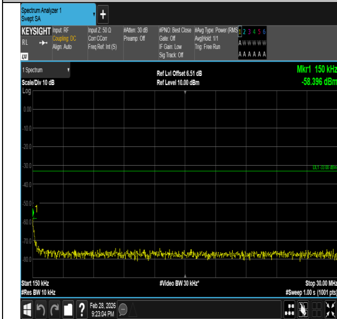
Band66-3MHz-16QAM-131987-1RB#0-0.15~30-PASS
