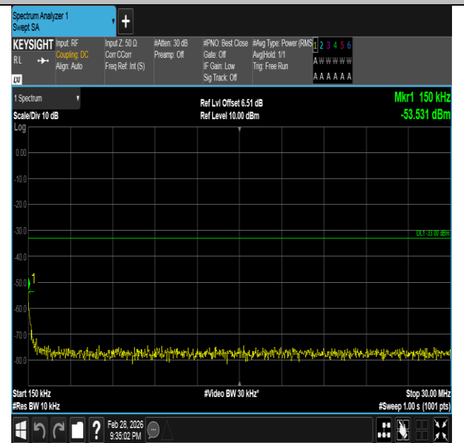
Band66-3MHz-16QAM-132657-1RB#14-0.15~30-PASS
