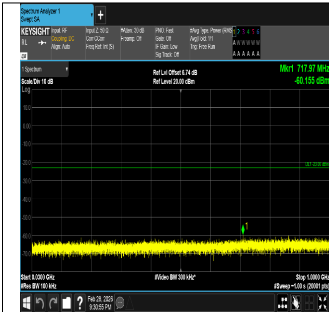
Band66-3MHz-QPSK-132322-15RB#0-30~1000-PASS
