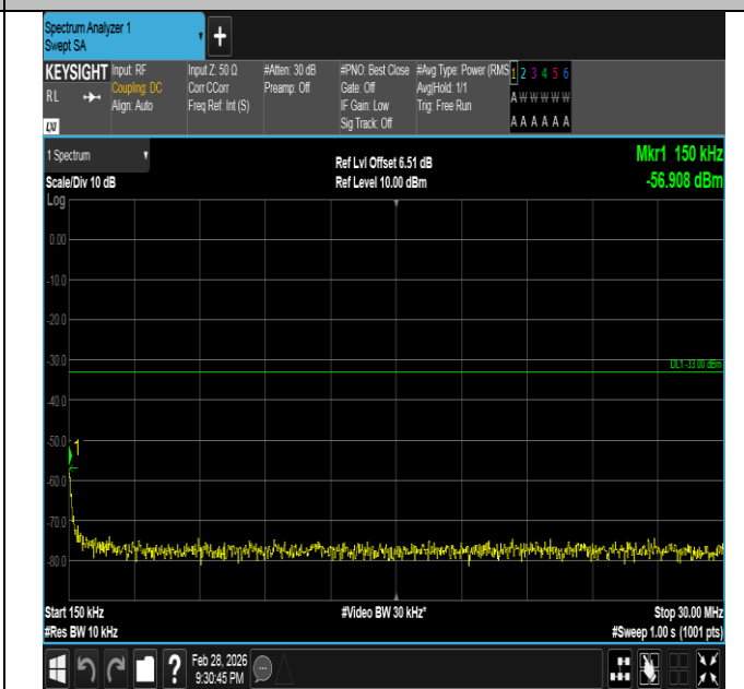
Band66-3MHz-QPSK-132322-15RB#0-0.15~30-PASS
