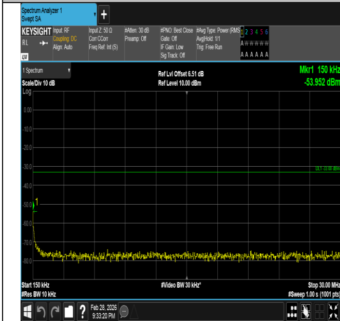
Band66-3MHz-16QAM-132657-1RB#0-0.15~30-PASS
