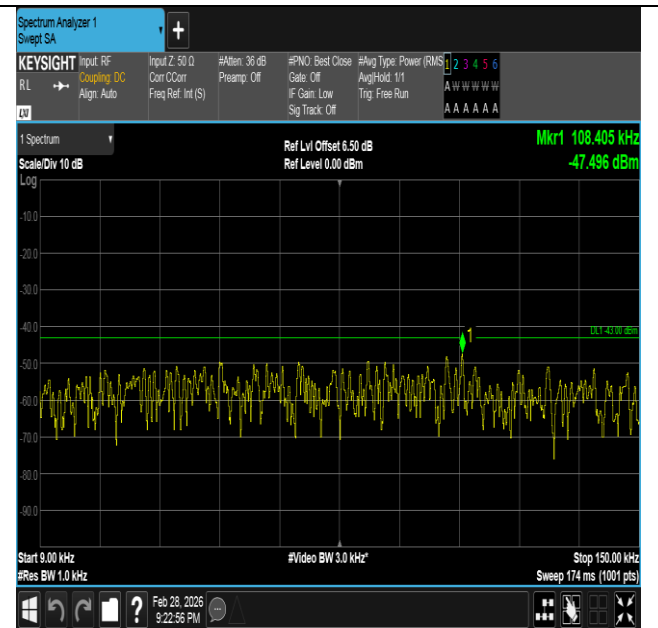
Band66-3MHz-16QAM-131987-1RB#0-0.009~0.15-PASS
