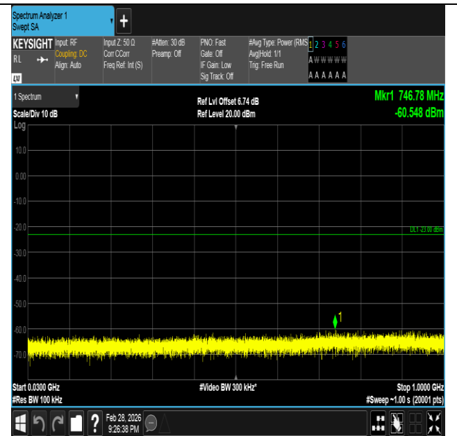
Band66-3MHz-16QAM-131987-15RB#0-30~1000-PASS
