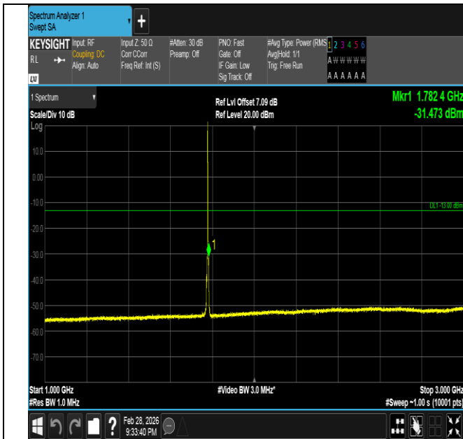
Band66-3MHz-16QAM-132657-1RB#0-1000~3000-PASS
