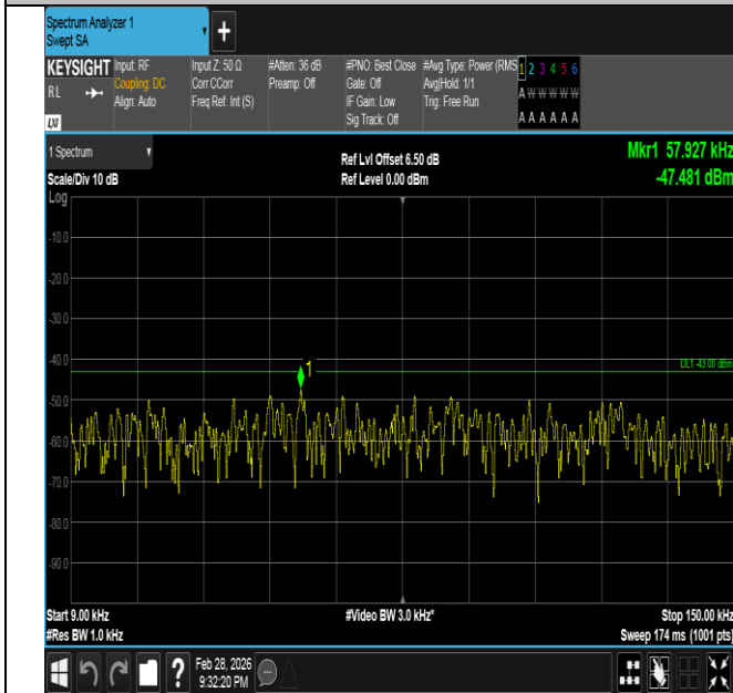
Band66-3MHz-QPSK-132657-1RB#0-0.009~0.15-PASS
