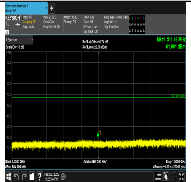
Band66-3MHz-16QAM-131987-1RB#0-30~1000-PASS
