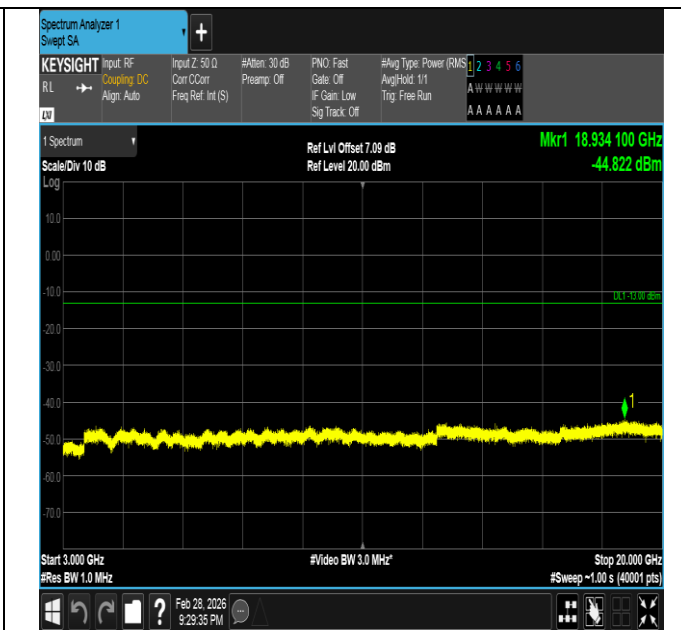
Band66-3MHz-QPSK-132322-1RB#14-3000~20000-PASS
