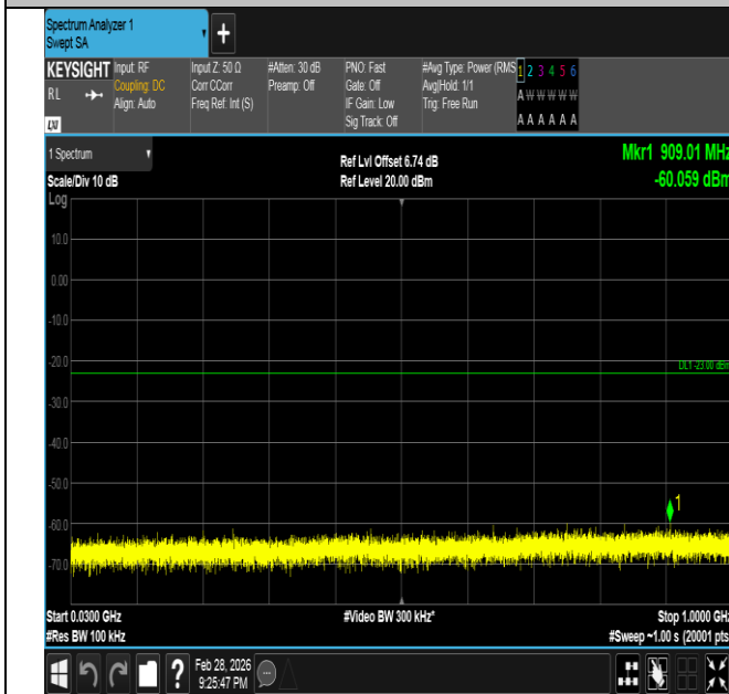
Band66-3MHz-QPSK-131987-15RB#0-30~1000-PASS
