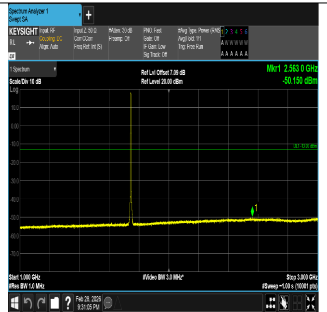
Band66-3MHz-QPSK-132322-15RB#0-1000~3000-PASS
