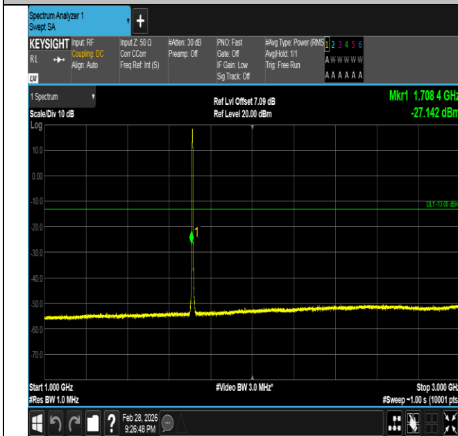
Band66-3MHz-16QAM-131987-15RB#0-1000~3000-PASS
