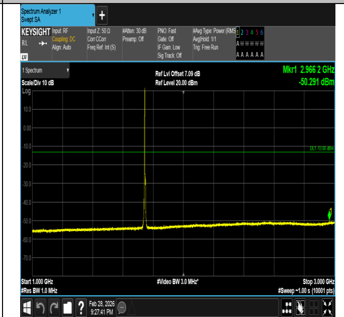
Band66-3MHz-QPSK-132322-1RB#0-1000~3000-PASS
