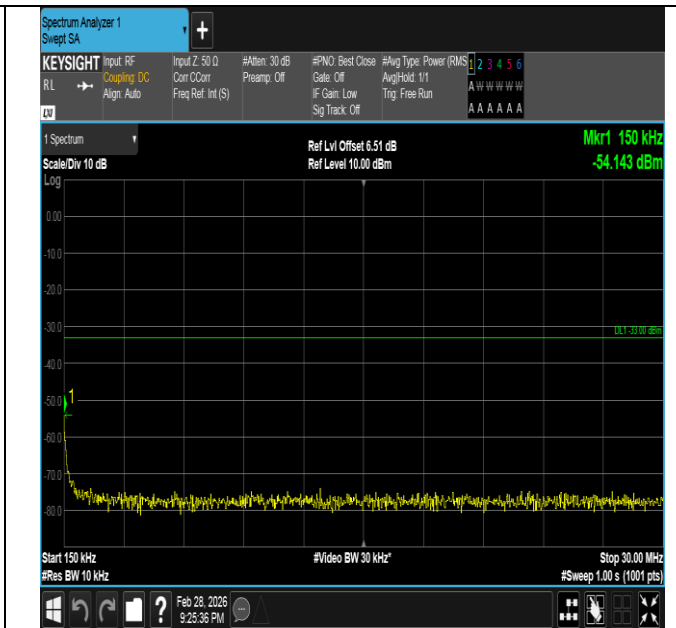
Band66-3MHz-QPSK-131987-15RB#0-0.15~30-PASS
