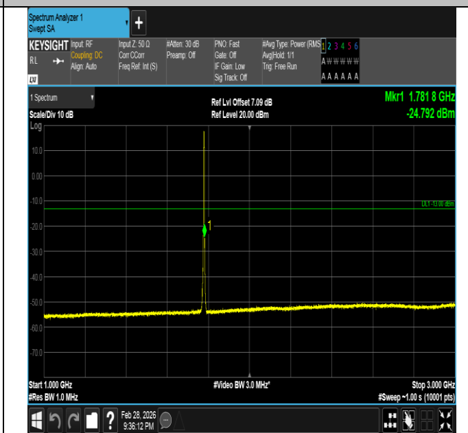
Band66-3MHz-QPSK-132657-15RB#0-1000~3000-PASS
