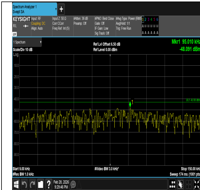
Band66-3MHz-16QAM-132322-1RB#14-0.009~0.15-PASS
