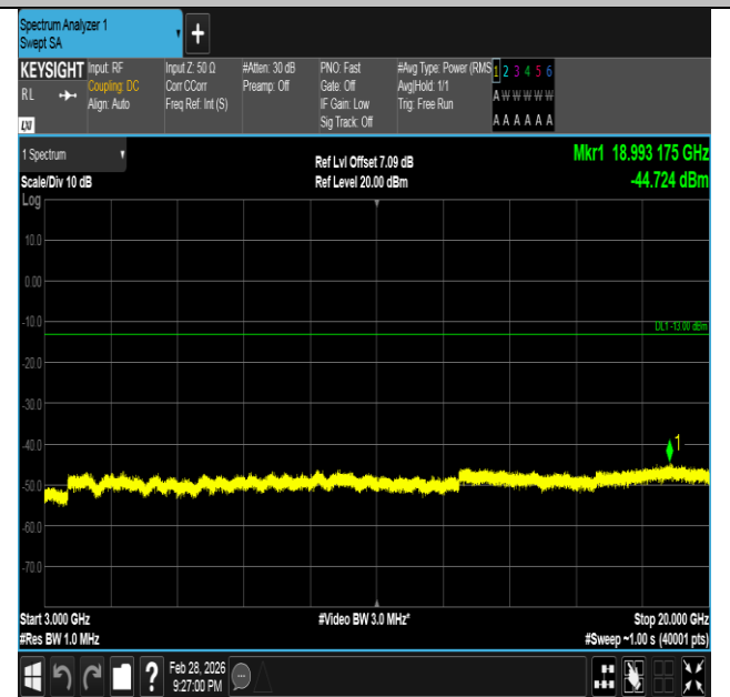
Band66-3MHz-16QAM-131987-15RB#0-3000~20000-PASS
