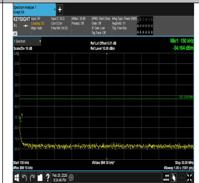
Band66-3MHz-16QAM-131987-1RB#14-0.15~30-PASS
