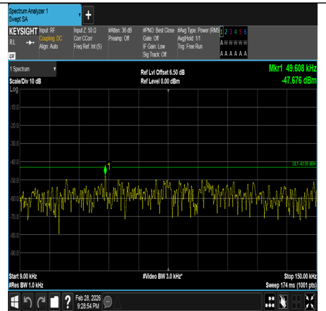
Band66-3MHz-QPSK-132322-1RB#14-0.009~0.15-PASS
