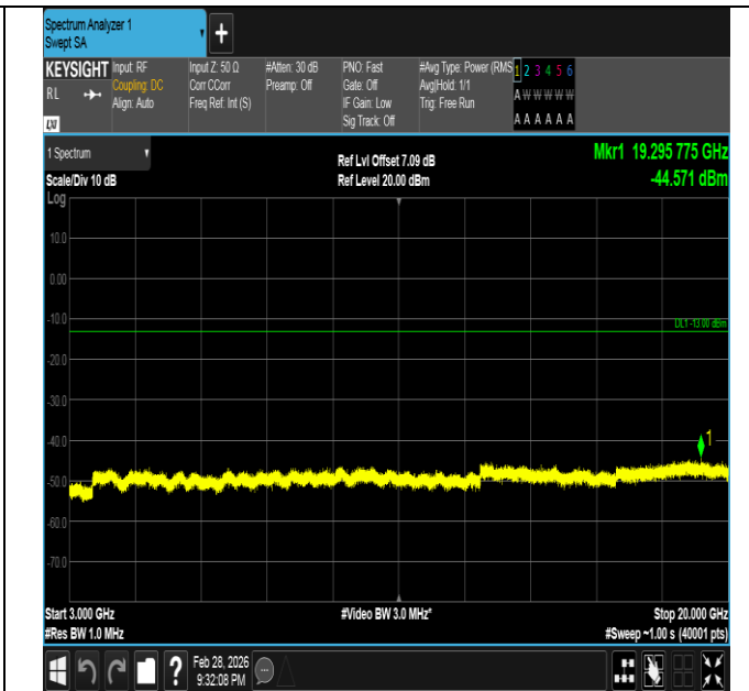
Band66-3MHz-16QAM-132322-15RB#0-3000~20000-PASS
