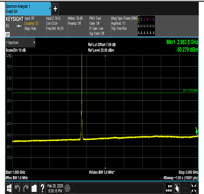
Band66-3MHz-16QAM-132322-1RB#14-1000~3000-PASS
