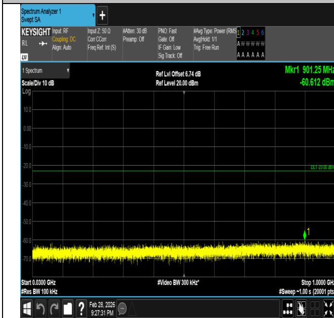
Band66-3MHz-QPSK-132322-1RB#0-30~1000-PASS
