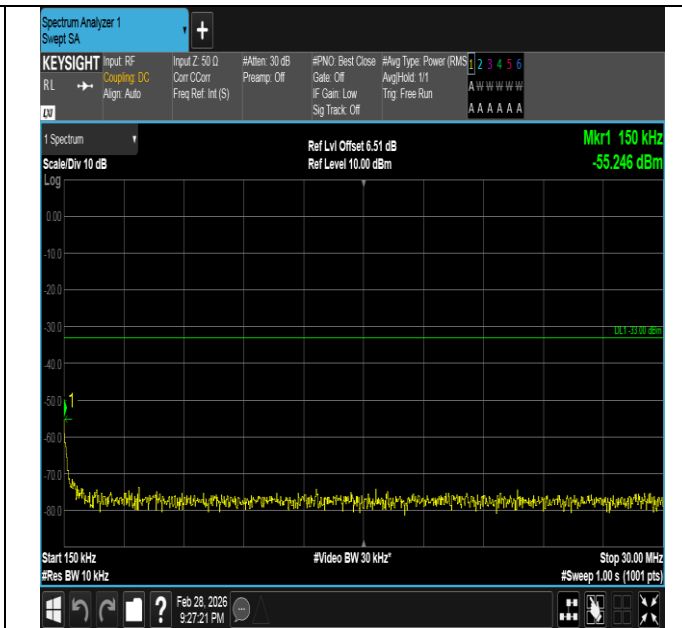
Band66-3MHz-QPSK-132322-1RB#0-0.15~30-PASS
