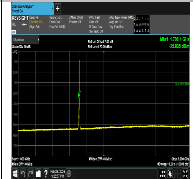
Band66-3MHz-QPSK-131987-15RB#0-1000~3000-PASS
