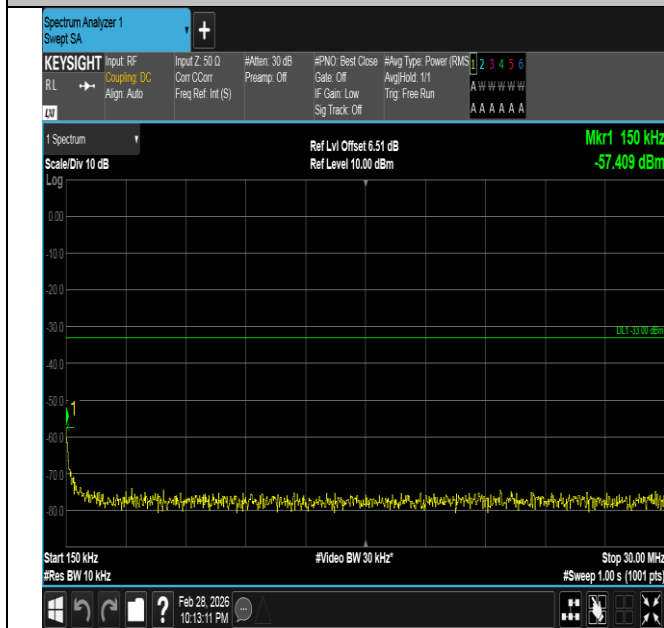
Band66-5MHz-16QAM-132322-1RB#0-0.15~30-PASS
