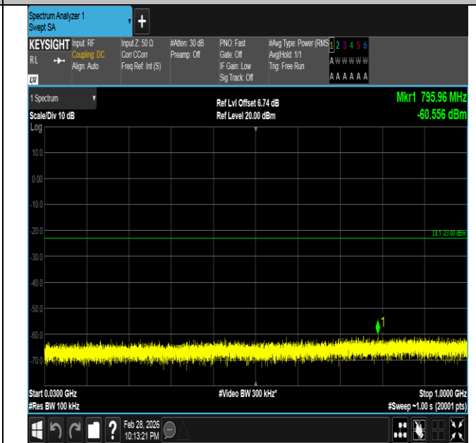
Band66-5MHz-16QAM-132322-1RB#0-30~1000-PASS
