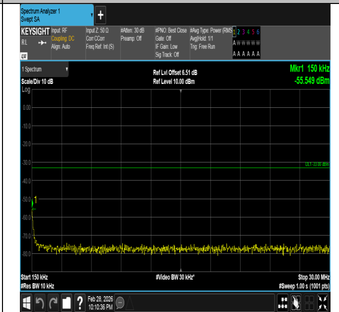
Band66-5MHz-QPSK-131997-25RB#0-0.15~30-PASS
