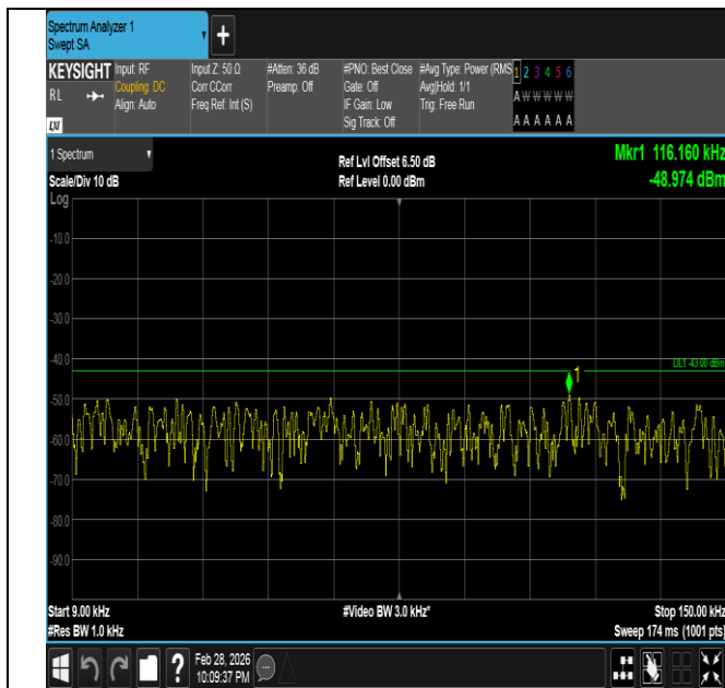
Band66-5MHz-16QAM-131997-1RB#24-0.009~0.15-PASS
