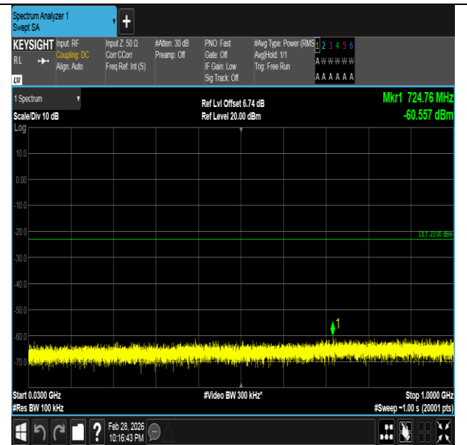
Band66-5MHz-16QAM-132322-25RB#0-30~1000-PASS
