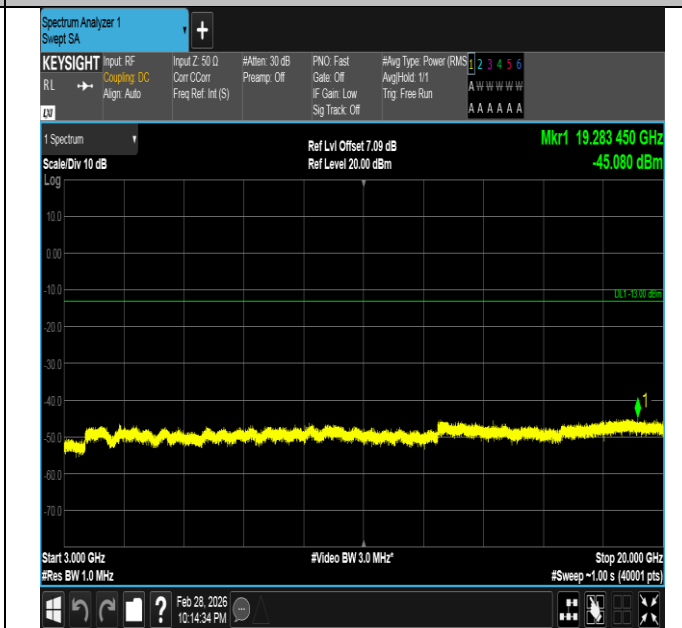
Band66-5MHz-QPSK-132322-1RB#24-3000~20000-PASS
