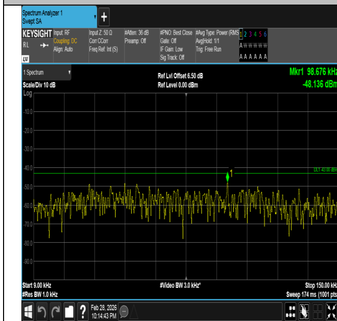
Band66-5MHz-16QAM-132322-1RB#24-0.009~0.15-PASS
