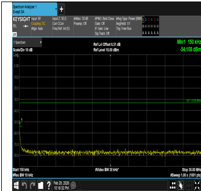
Band66-5MHz-16QAM-132322-25RB#0-0.15~30-PASS
