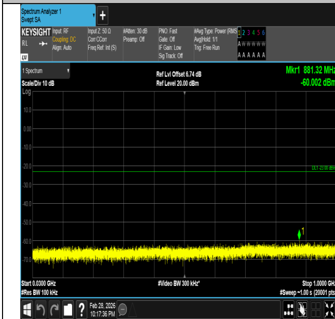
Band66-5MHz-QPSK-132647-1RB#0-30~1000-PASS
