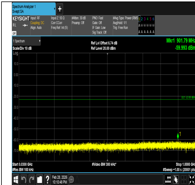
Band66-5MHz-QPSK-131997-25RB#0-30~1000-PASS
