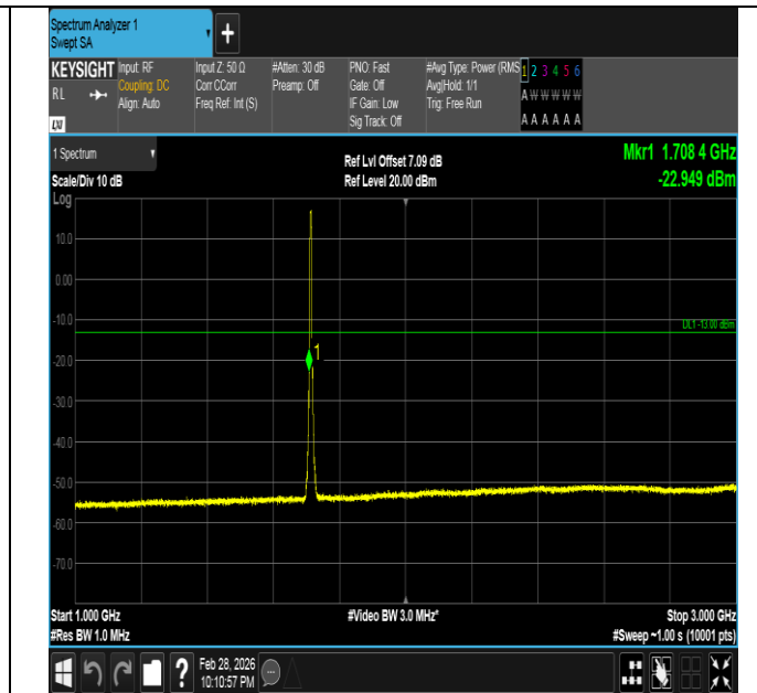
Band66-5MHz-QPSK-131997-25RB#0-1000~3000-PASS
