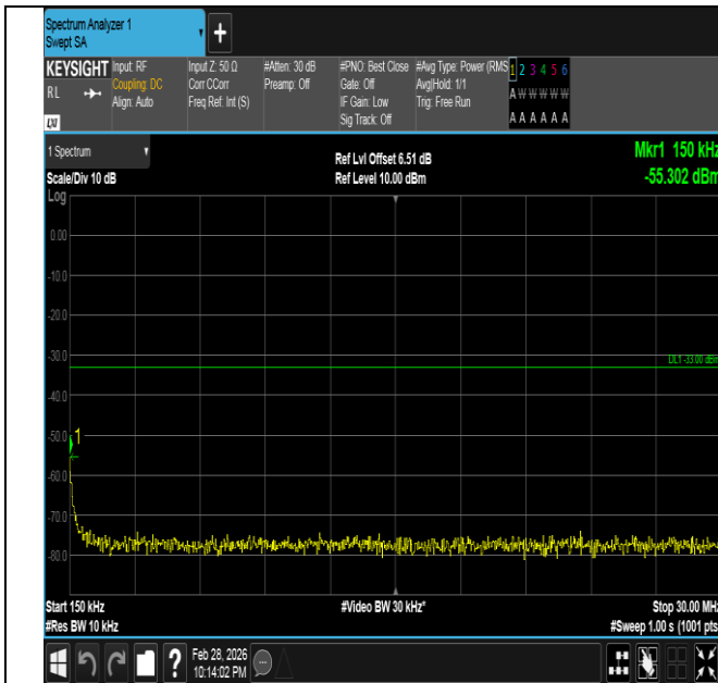
Band66-5MHz-QPSK-132322-1RB#24-0.15~30-PASS
