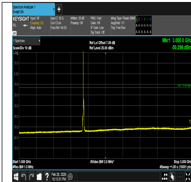
Band66-5MHz-16QAM-132322-1RB#0-1000~3000-PASS
