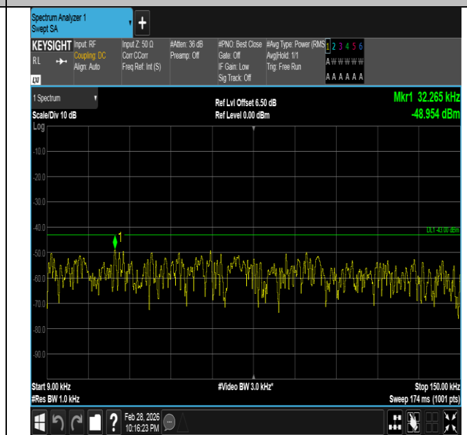
Band66-5MHz-16QAM-132322-25RB#0-0.009~0.15-PASS
