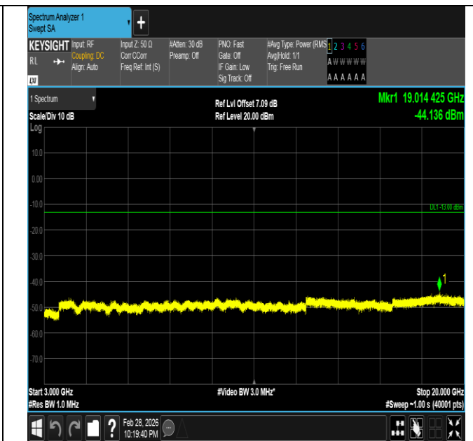
Band66-5MHz-QPSK-132647-1RB#24-3000~20000-PASS
