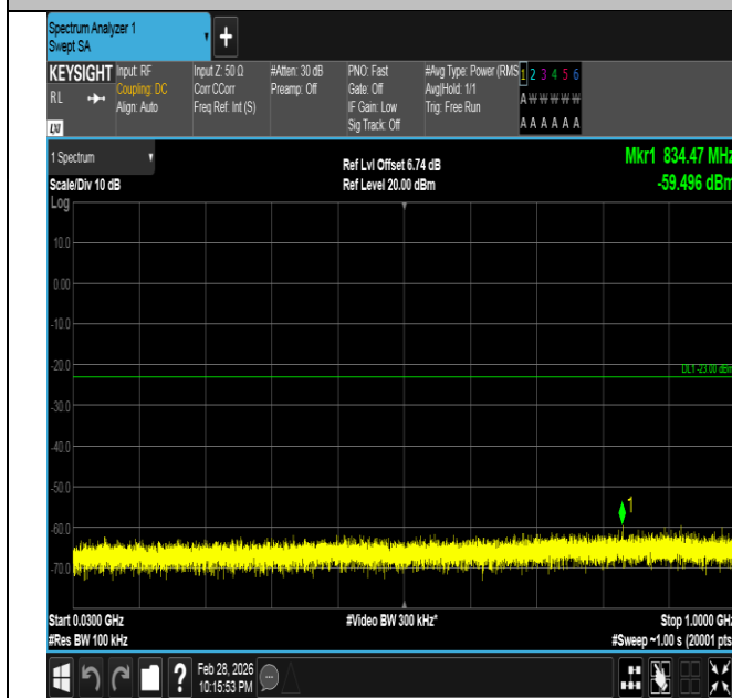
Band66-5MHz-QPSK-132322-25RB#0-30~1000-PASS
