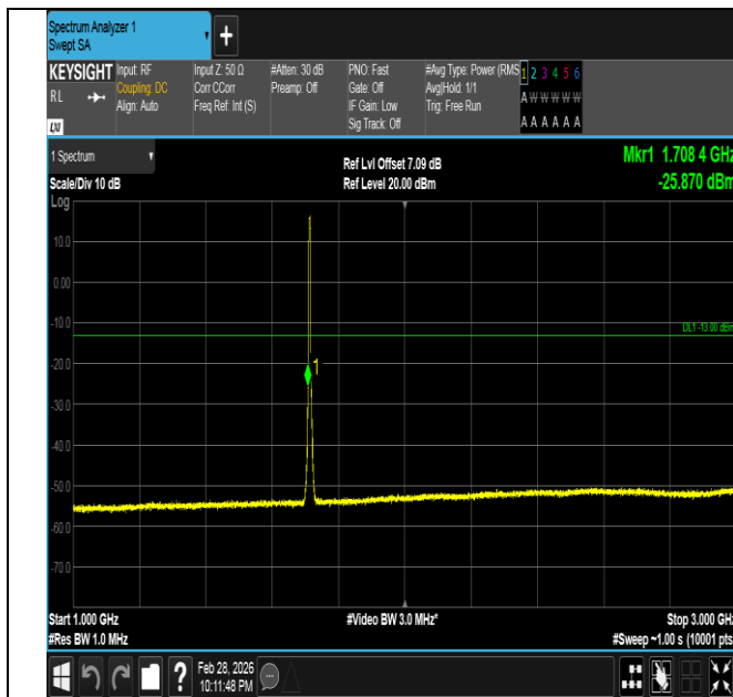
Band66-5MHz-16QAM-131997-25RB#0-1000~3000-PASS
