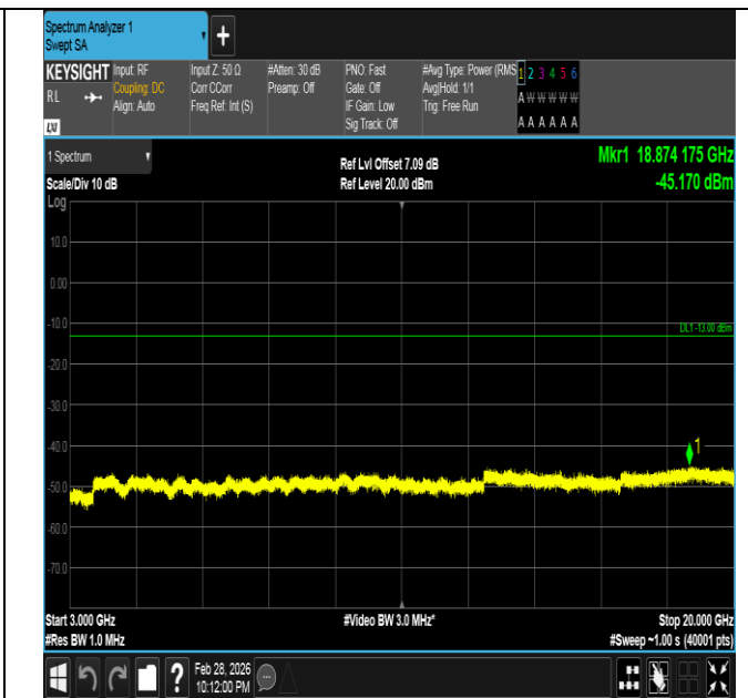
Band66-5MHz-16QAM-131997-25RB#0-3000~20000-PASS
