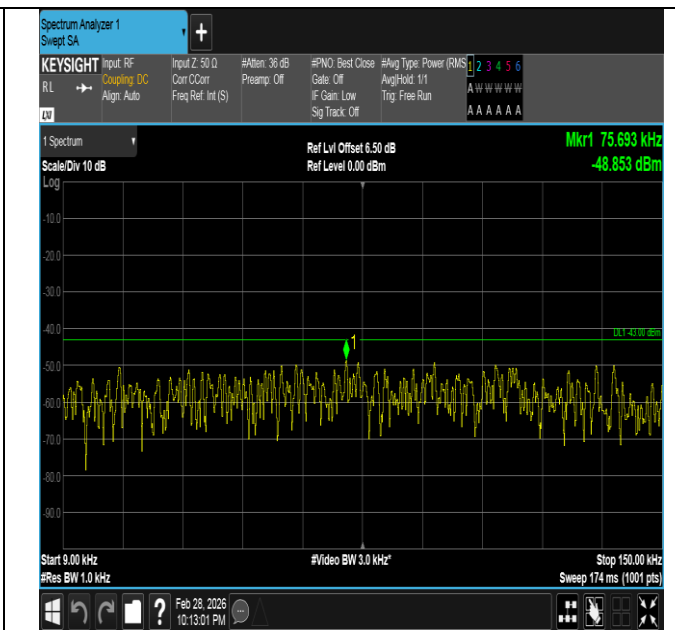
Band66-5MHz-16QAM-132322-1RB#0-0.009~0.15-PASS
