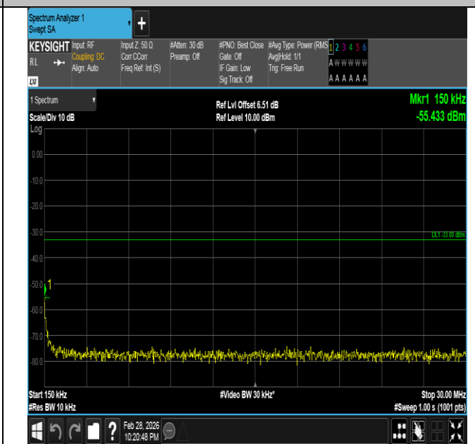
Band66-5MHz-QPSK-132647-25RB#0-0.15~30-PASS
