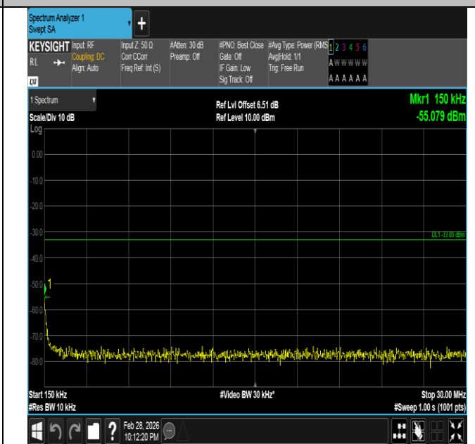
Band66-5MHz-QPSK-132322-1RB#0-0.15~30-PASS
