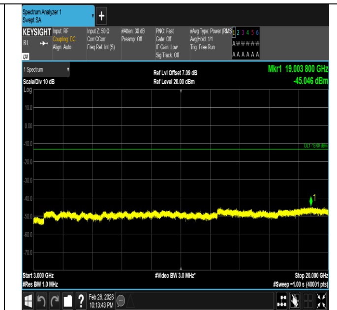
Band66-5MHz-16QAM-132322-1RB#0-3000~20000-PASS
