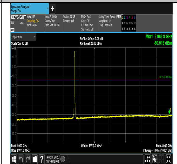
Band66-5MHz-QPSK-132322-25RB#0-1000~3000-PASS
