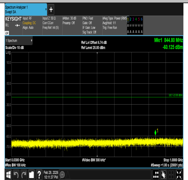
Band66-5MHz-16QAM-131997-25RB#0-30~1000-PASS
