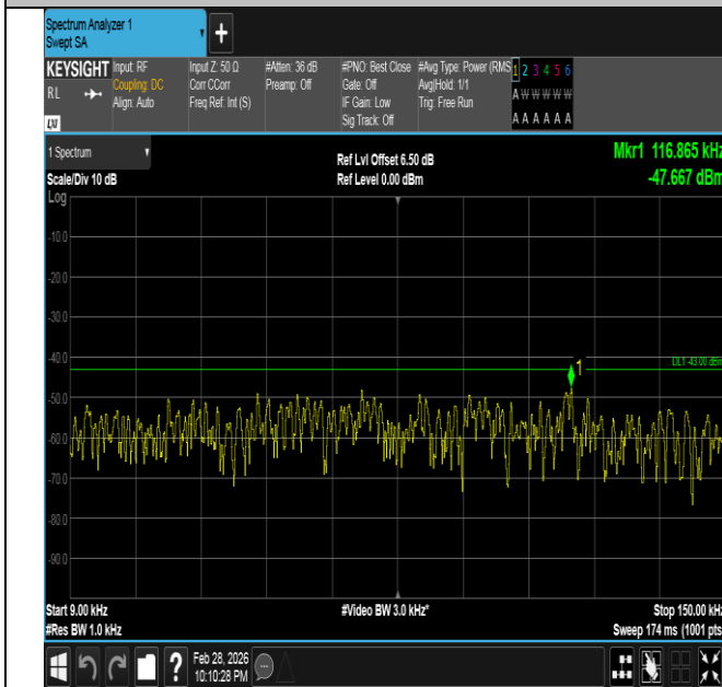
Band66-5MHz-QPSK-131997-25RB#0-0.009~0.15-PASS
