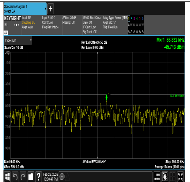
Band66-5MHz-QPSK-131997-1RB#24-0.009~0.15-PASS
