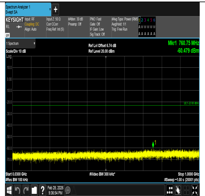
Band66-3MHz-16QAM-132657-15RB#0-30~1000-PASS
