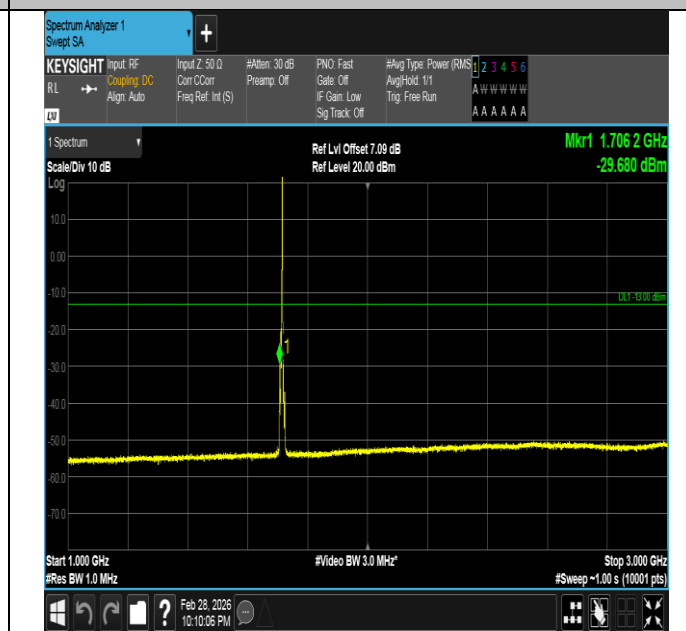
Band66-5MHz-16QAM-131997-1RB#24-1000~3000-PASS
