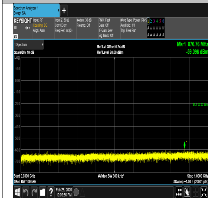
Band66-5MHz-16QAM-131997-1RB#24-30~1000-PASS
