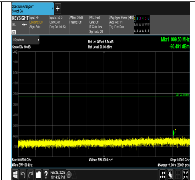
Band66-5MHz-QPSK-132322-1RB#24-30~1000-PASS
