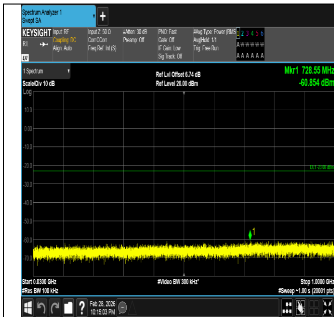
Band66-5MHz-16QAM-132322-1RB#24-30~1000-PASS
