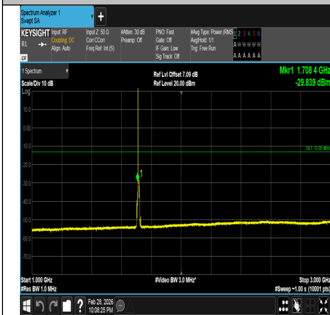
Band66-5MHz-16QAM-131997-1RB#0-1000~3000-PASS
