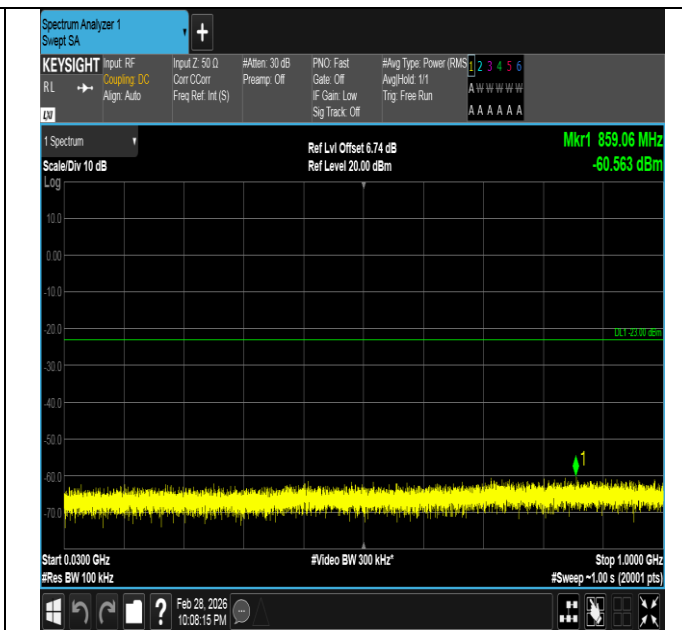
Band66-5MHz-16QAM-131997-1RB#0-30~1000-PASS
