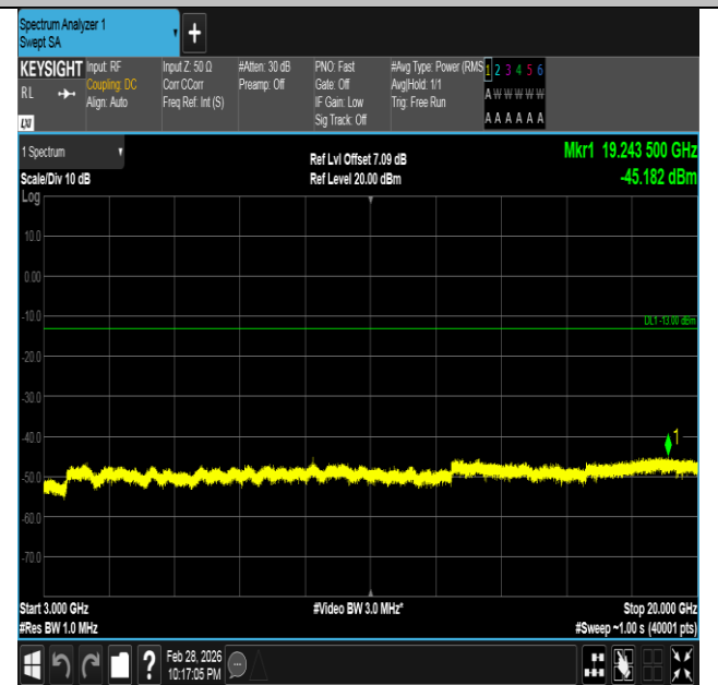
Band66-5MHz-16QAM-132322-25RB#0-3000~20000-PASS
