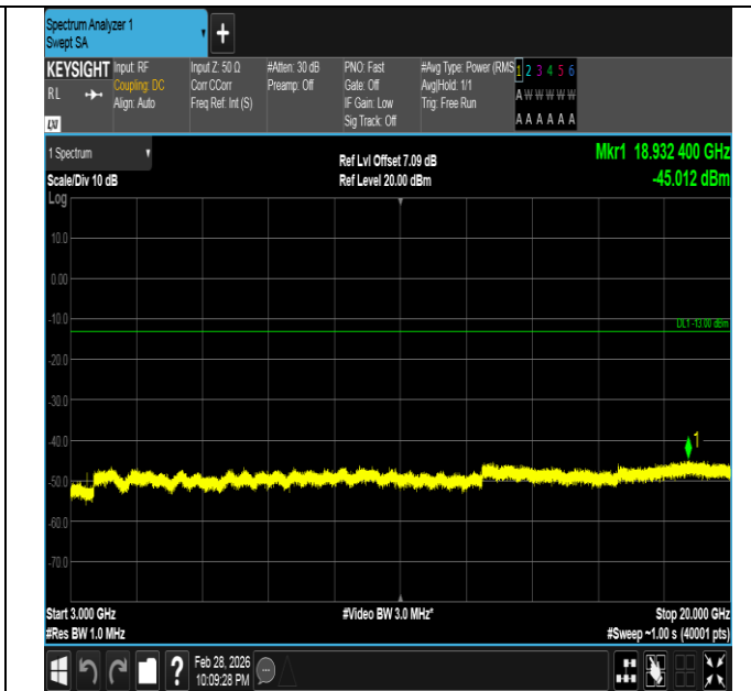
Band66-5MHz-QPSK-131997-1RB#24-3000~20000-PASS
