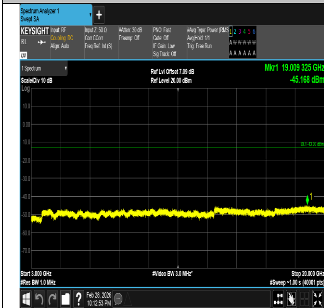
Band66-5MHz-QPSK-132322-1RB#0-3000~20000-PASS
