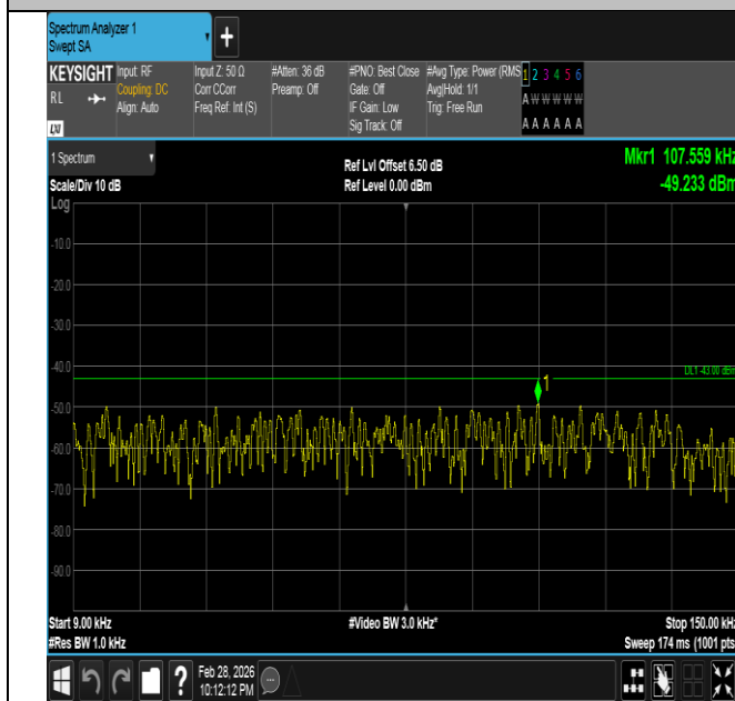
Band66-5MHz-QPSK-132322-1RB#0-0.009~0.15-PASS
