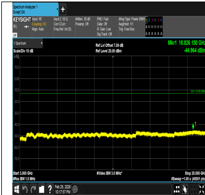
Band66-5MHz-QPSK-132647-1RB#0-3000~20000-PASS
