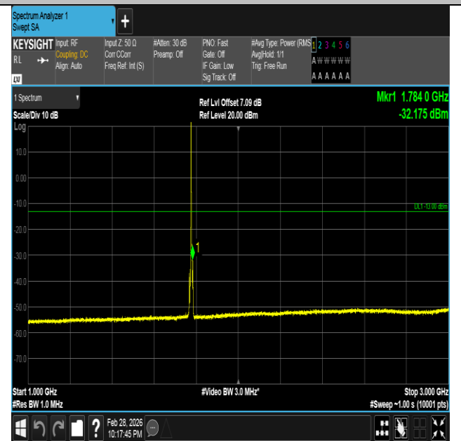
Band66-5MHz-QPSK-132647-1RB#0-1000~3000-PASS
