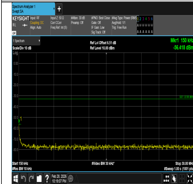
Band66-5MHz-QPSK-132647-1RB#24-0.15~30-PASS
