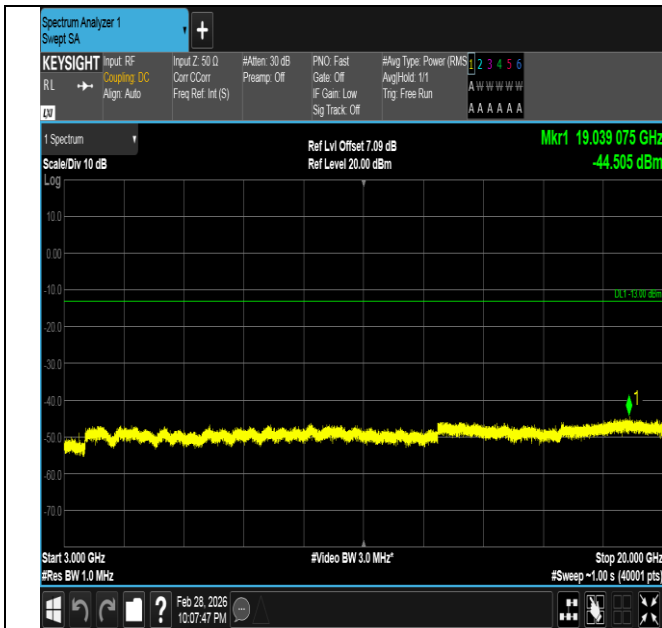
Band66-5MHz-QPSK-131997-1RB#0-3000~20000-PASS
