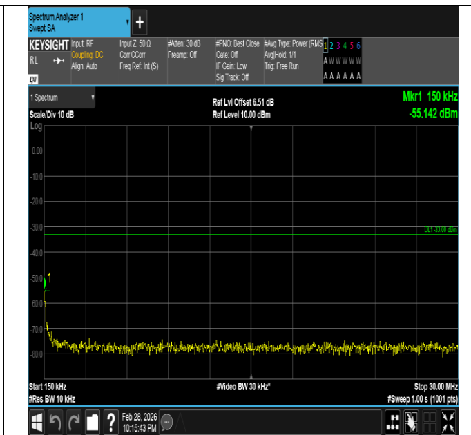
Band66-5MHz-QPSK-132322-25RB#0-0.15~30-PASS
