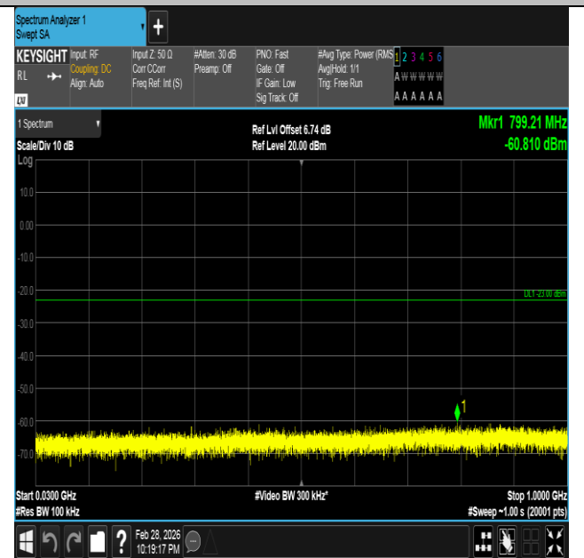
Band66-5MHz-QPSK-132647-1RB#24-30~1000-PASS
