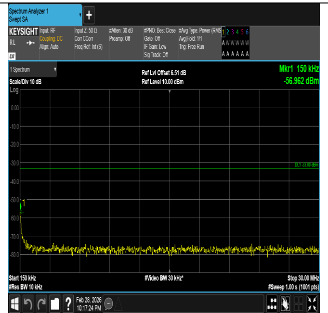
Band66-5MHz-QPSK-132647-1RB#0-0.15~30-PASS
