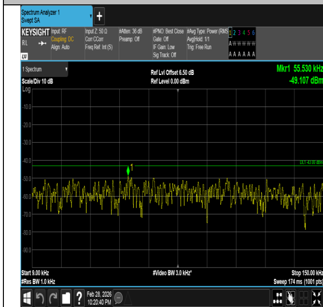
Band66-5MHz-QPSK-132647-25RB#0-0.009~0.15-PASS
