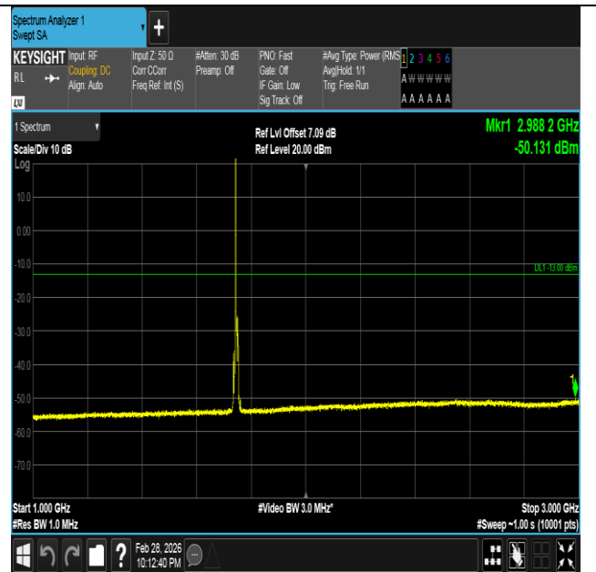
Band66-5MHz-QPSK-132322-1RB#0-1000~3000-PASS
