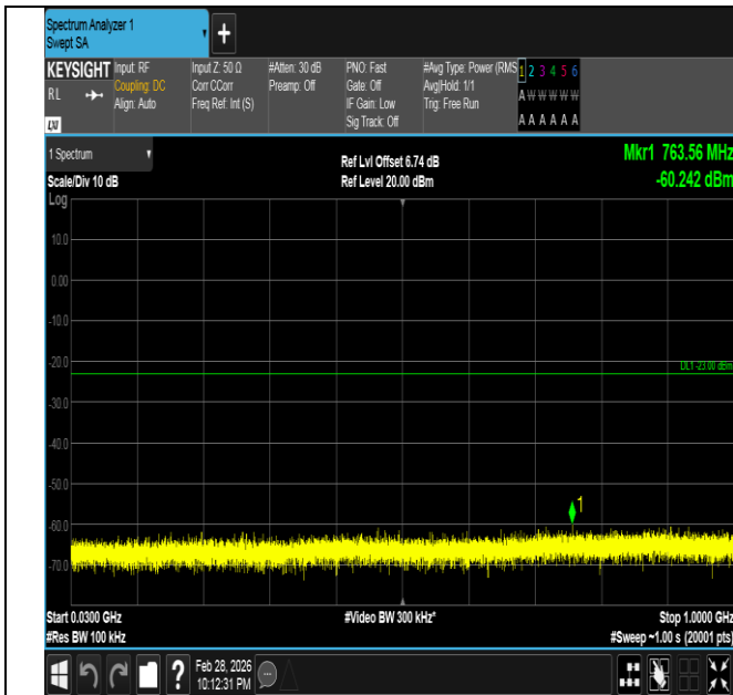
Band66-5MHz-QPSK-132322-1RB#0-30~1000-PASS
