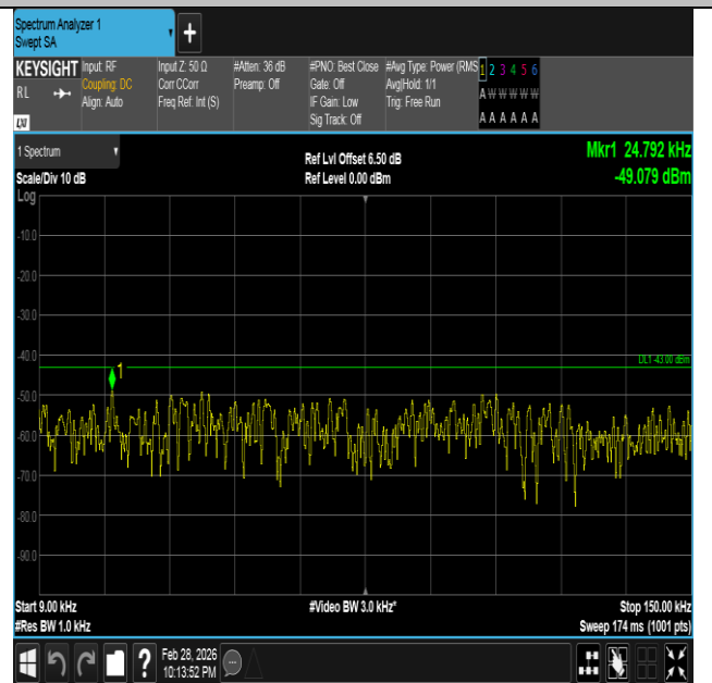
Band66-5MHz-QPSK-132322-1RB#24-0.009~0.15-PASS
