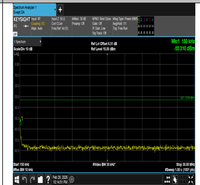
Band66-5MHz-16QAM-132322-1RB#24-0.15~30-PASS
