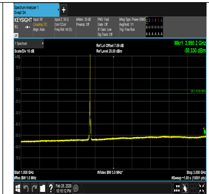
Band66-5MHz-16QAM-132322-1RB#24-1000~3000-PASS
