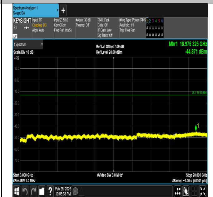
Band66-5MHz-16QAM-131997-1RB#0-3000~20000-PASS
