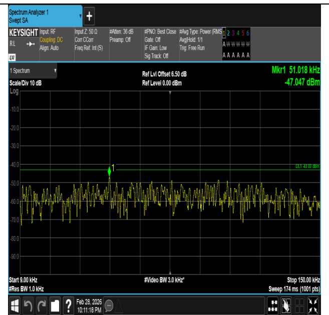
Band66-5MHz-16QAM-131997-25RB#0-0.009~0.15-PASS
