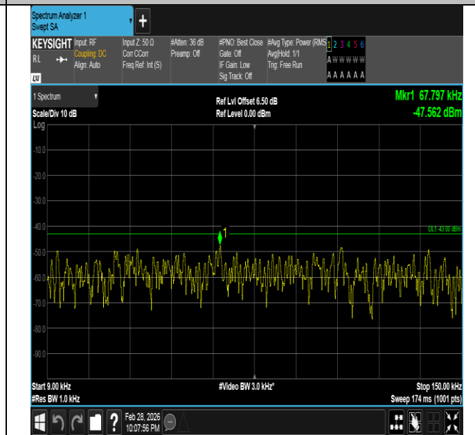
Band66-5MHz-16QAM-131997-1RB#0-0.009~0.15-PASS
