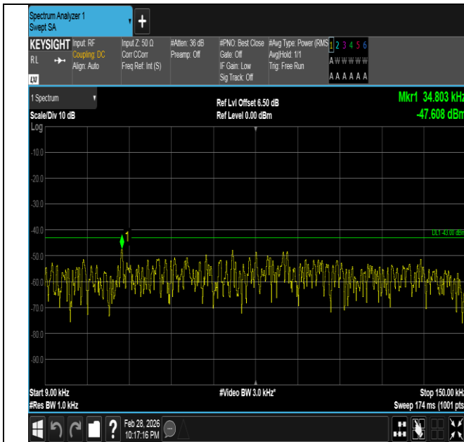
Band66-5MHz-QPSK-132647-1RB#0-0.009~0.15-PASS
