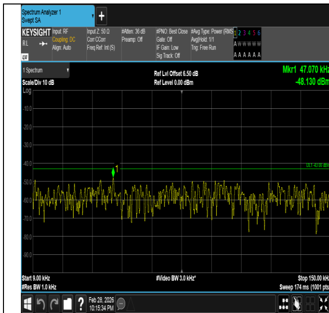
Band66-5MHz-QPSK-132322-25RB#0-0.009~0.15-PASS
