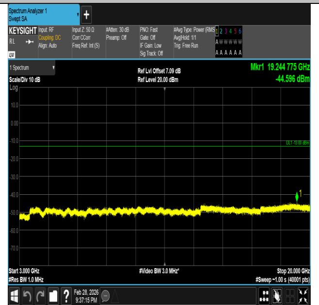
Band66-3MHz-16QAM-132657-15RB#0-3000~20000-PASS
