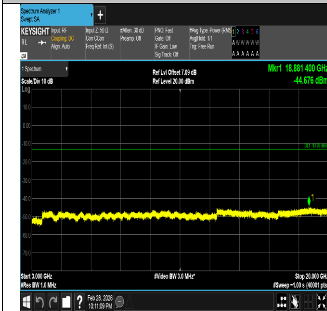
Band66-5MHz-QPSK-131997-25RB#0-3000~20000-PASS
