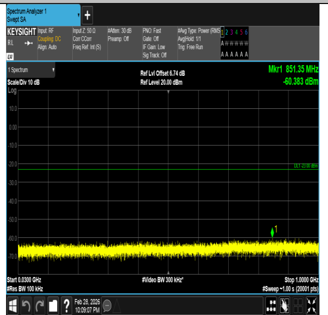
Band66-5MHz-QPSK-131997-1RB#24-30~1000-PASS
