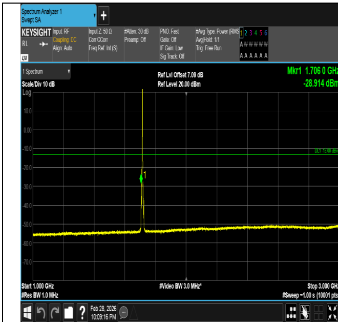
Band66-5MHz-QPSK-131997-1RB#24-1000~3000-PASS
