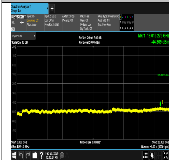
Band66-5MHz-16QAM-132322-1RB#24-3000~20000-PASS
