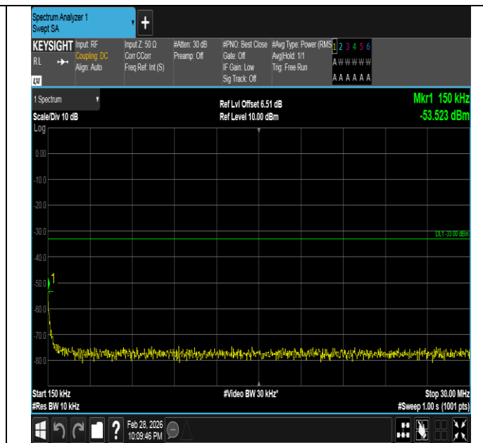
Band66-5MHz-16QAM-131997-1RB#24-0.15~30-PASS
