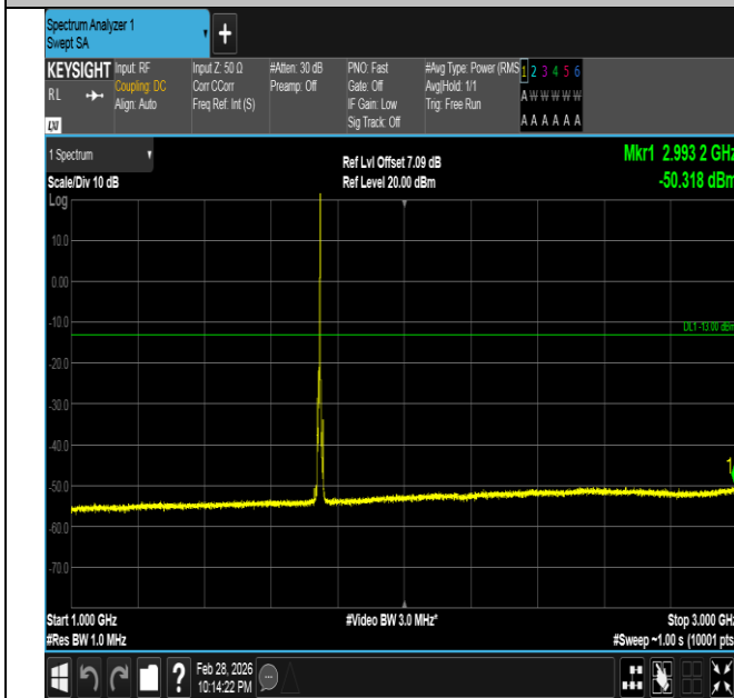
Band66-5MHz-QPSK-132322-1RB#24-1000~3000-PASS
