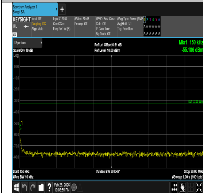
Band66-5MHz-QPSK-131997-1RB#24-0.15~30-PASS
