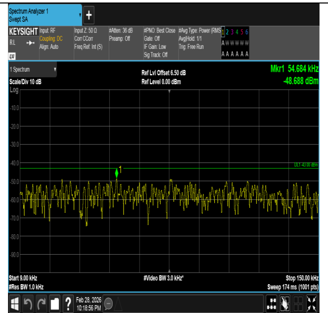
Band66-5MHz-QPSK-132647-1RB#24-0.009~0.15-PASS
