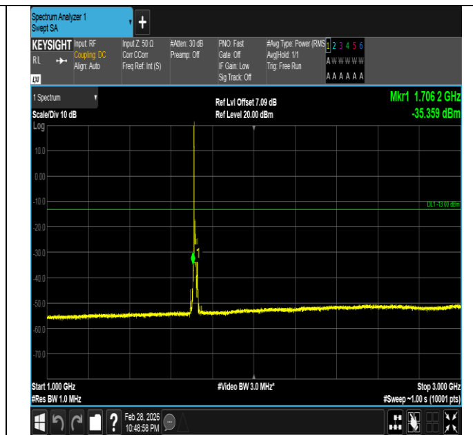
Band66-10MHz-QPSK-132022-1RB#0-1000~3000-PASS
