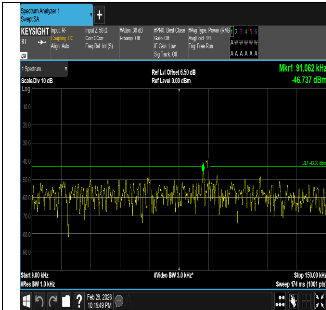
Band66-5MHz-16QAM-132647-1RB#24-0.009~0.15-PASS
