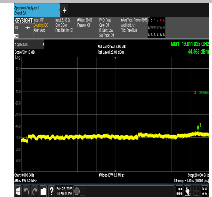
Band66-10MHz-QPSK-132022-1RB#49-3000~20000-PASS
