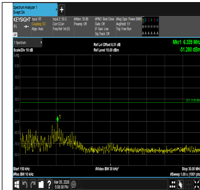
Band66-10MHz-16QAM-132022-50RB#0-0.15~30-PASS
