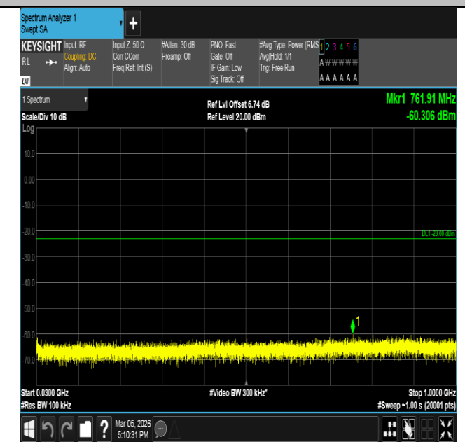
Band66-10MHz-16QAM-132322-50RB#0-30~1000-PASS
