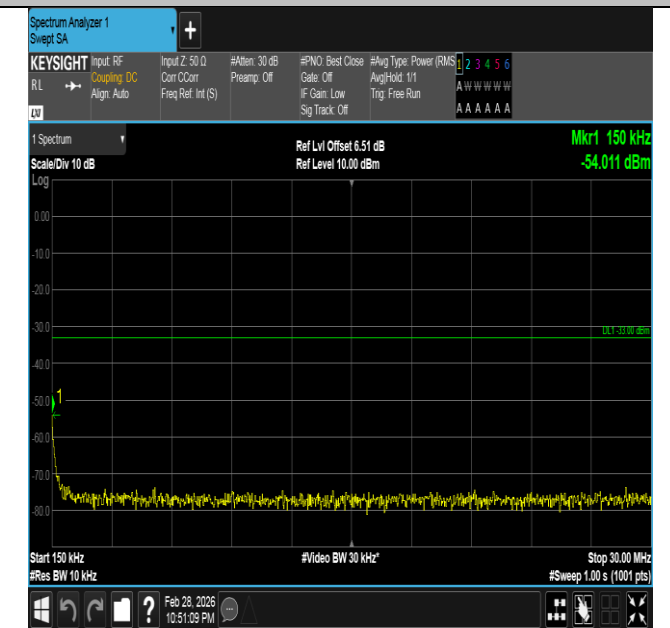
Band66-10MHz-16QAM-132022-1RB#49-0.15~30-PASS
