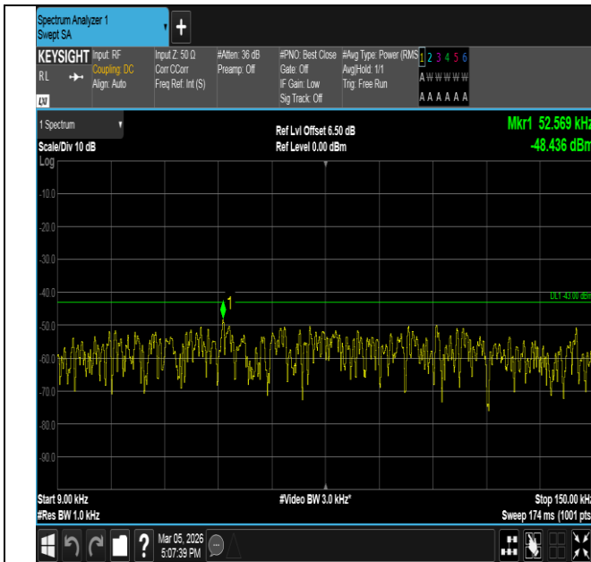
Band66-10MHz-QPSK-132022-50RB#0-0.009~0.15-PASS
