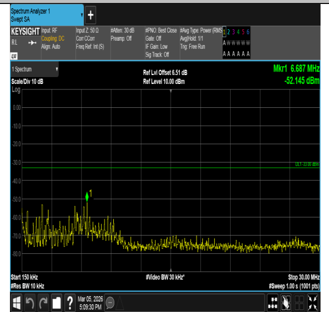
Band66-10MHz-QPSK-132322-50RB#0-0.15~30-PASS
