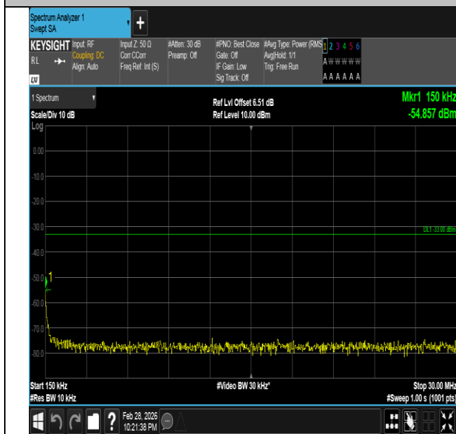
Band66-5MHz-16QAM-132647-25RB#0-0.15~30-PASS
