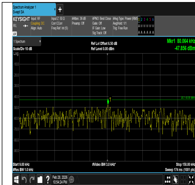
Band66-10MHz-16QAM-132322-1RB#49-0.009~0.15-PASS
