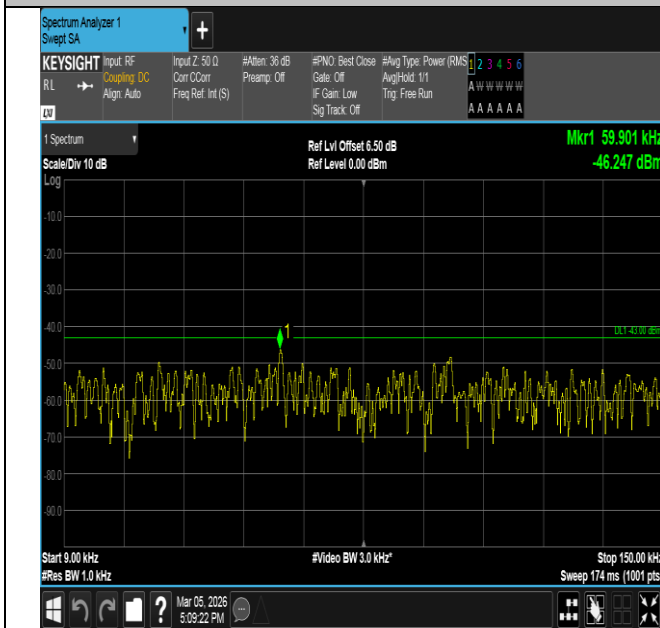
Band66-10MHz-QPSK-132322-50RB#0-0.009~0.15-PASS
