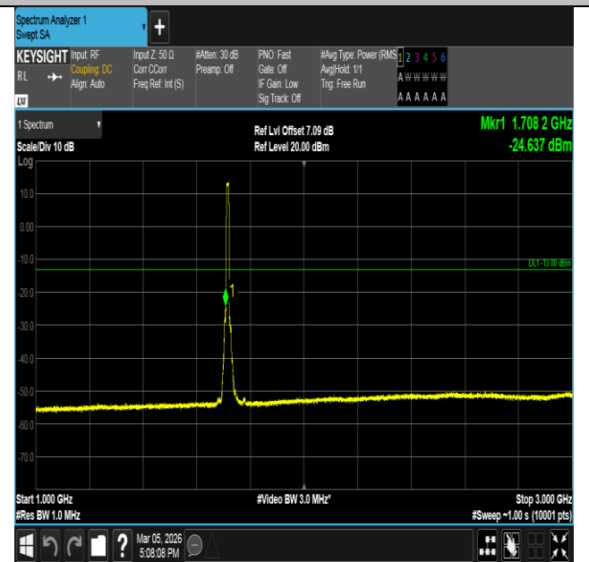
Band66-10MHz-QPSK-132022-50RB#0-1000~3000-PASS
