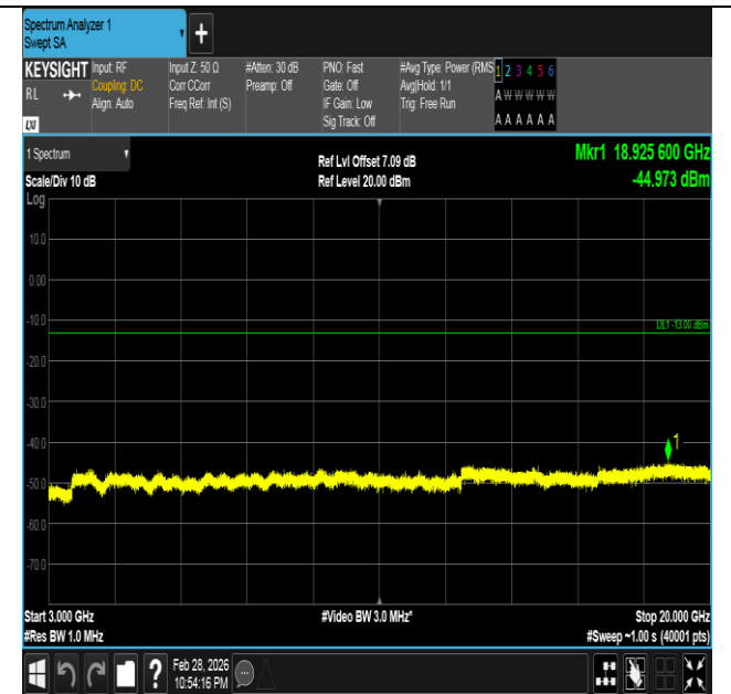
Band66-10MHz-QPSK-132322-1RB#49-3000~20000-PASS
