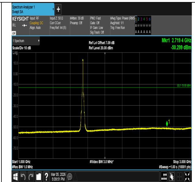
Band66-10MHz-QPSK-132322-50RB#0-1000~3000-PASS
