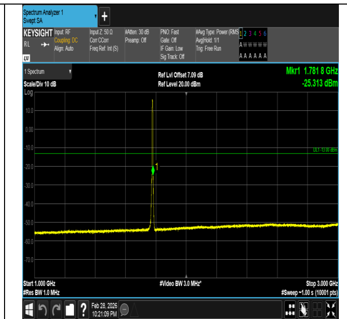
Band66-5MHz-QPSK-132647-25RB#0-1000~3000-PASS
