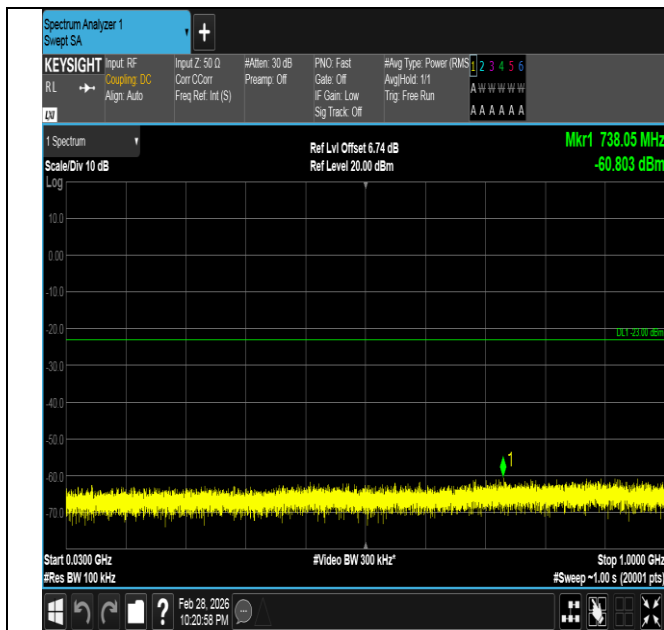
Band66-5MHz-QPSK-132647-25RB#0-30~1000-PASS
