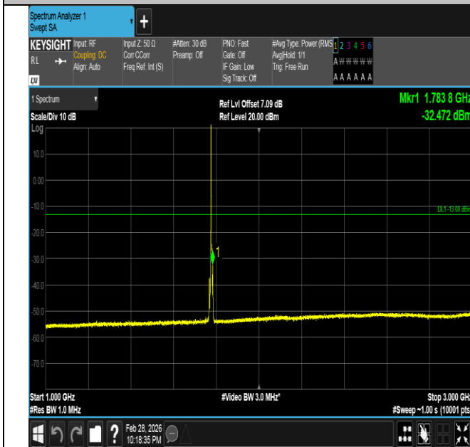
Band66-5MHz-16QAM-132647-1RB#0-1000~3000-PASS
