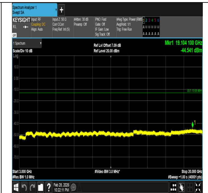
Band66-5MHz-16QAM-132647-25RB#0-3000~20000-PASS
