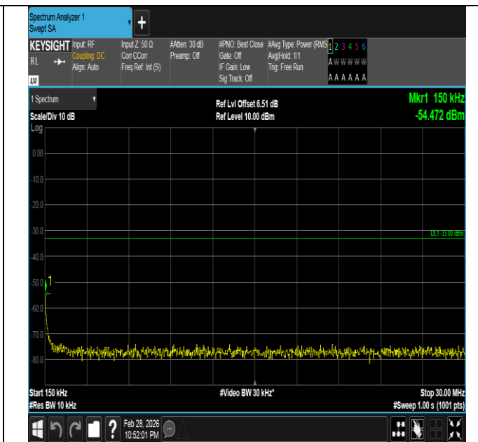
Band66-10MHz-QPSK-132322-1RB#0-0.15~30-PASS
