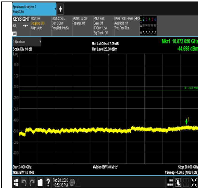
Band66-10MHz-QPSK-132322-1RB#0-3000~20000-PASS
