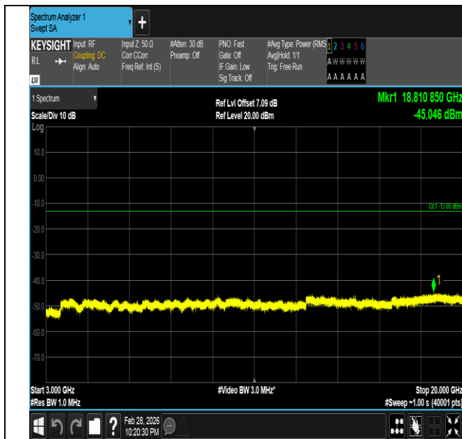
Band66-5MHz-16QAM-132647-1RB#24-3000~20000-PASS
