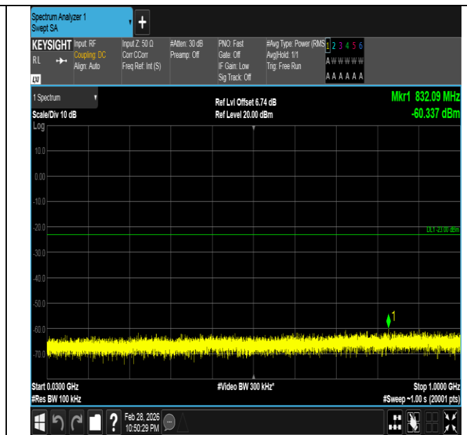
Band66-10MHz-QPSK-132022-1RB#49-30~1000-PASS
