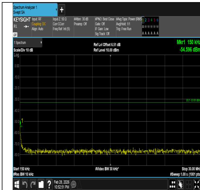
Band66-10MHz-16QAM-132322-1RB#0-0.15~30-PASS
