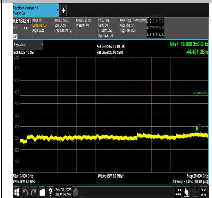
Band66-10MHz-16QAM-132322-1RB#0-3000~20000-PASS
