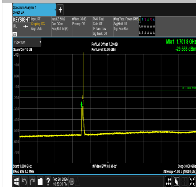
Band66-10MHz-QPSK-132022-1RB#49-1000~3000-PASS
