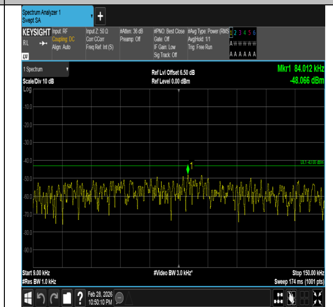
Band66-10MHz-QPSK-132022-1RB#49-0.009~0.15-PASS
