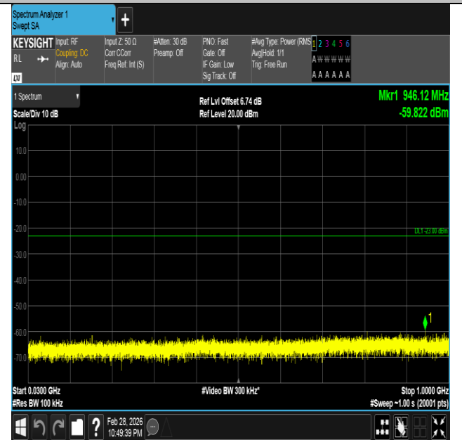
Band66-10MHz-16QAM-132022-1RB#0-30~1000-PASS
