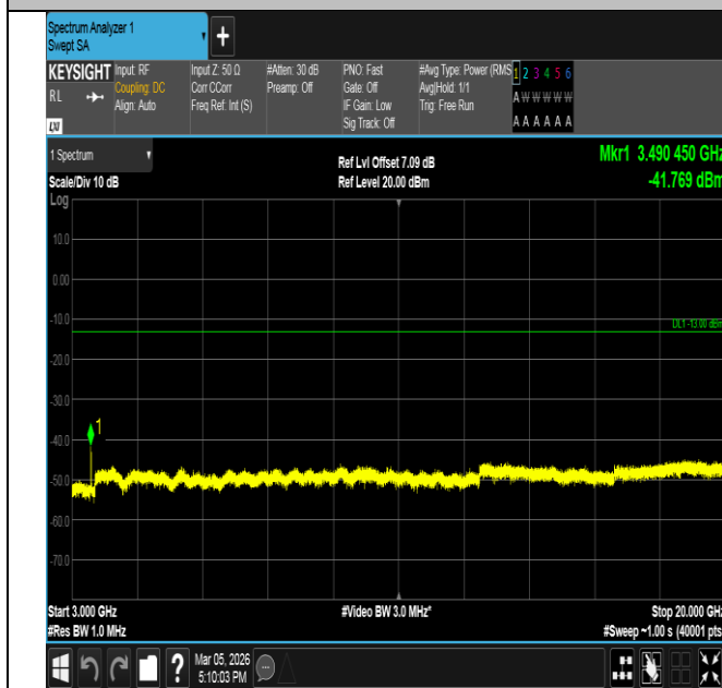
Band66-10MHz-QPSK-132322-50RB#0-3000~20000-PASS
