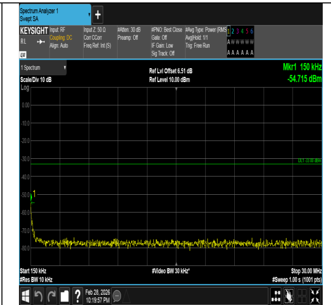
Band66-5MHz-16QAM-132647-1RB#24-0.15~30-PASS
