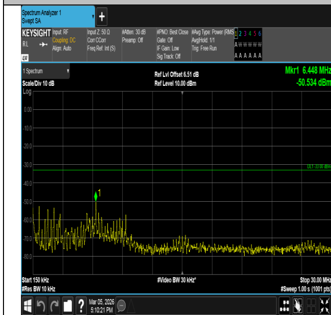
Band66-10MHz-16QAM-132322-50RB#0-0.15~30-PASS
