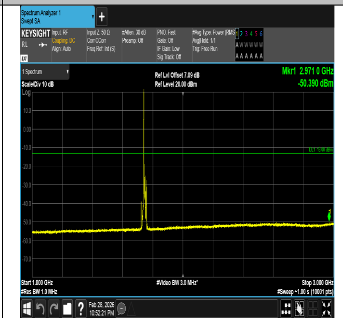
Band66-10MHz-QPSK-132322-1RB#0-1000~3000-PASS
