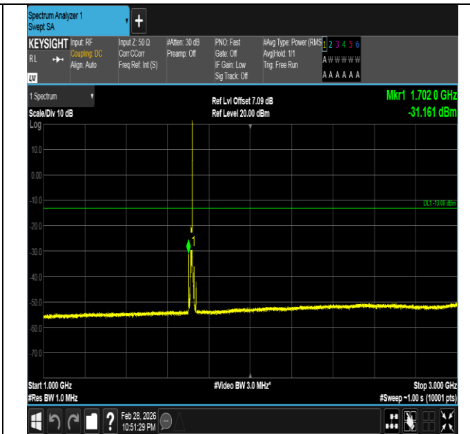
Band66-10MHz-16QAM-132022-1RB#49-1000~3000-PASS
