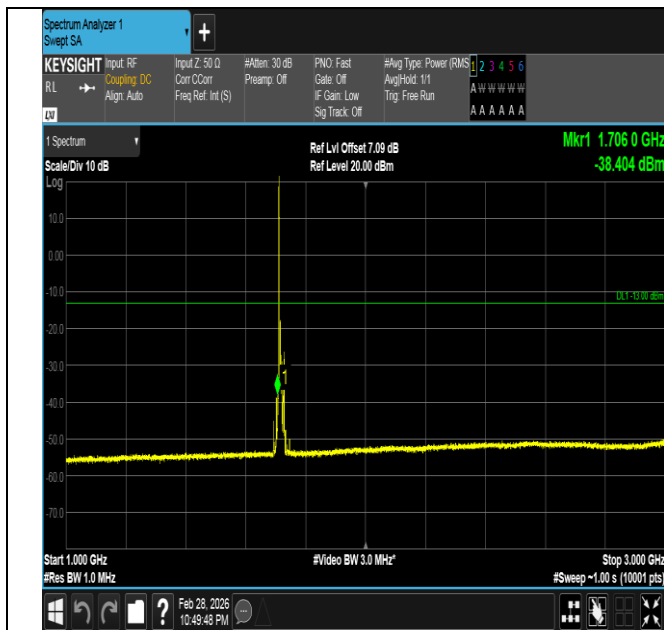
Band66-10MHz-16QAM-132022-1RB#0-1000~3000-PASS
