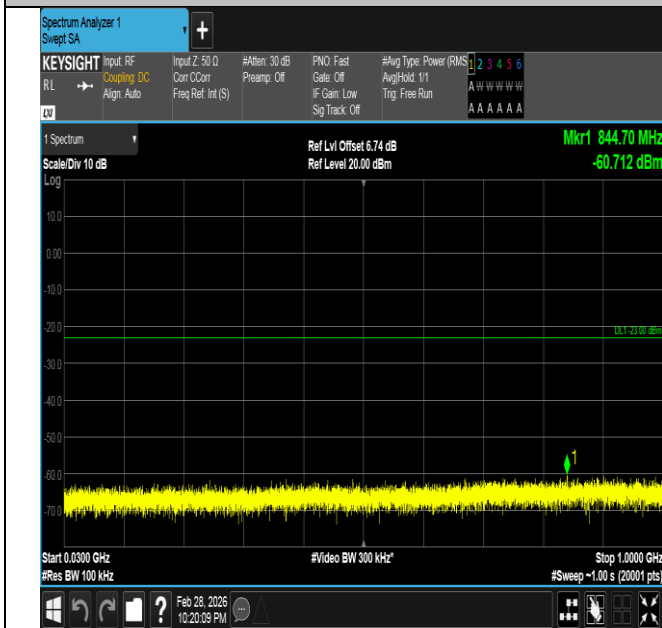
Band66-5MHz-16QAM-132647-1RB#24-30~1000-PASS
