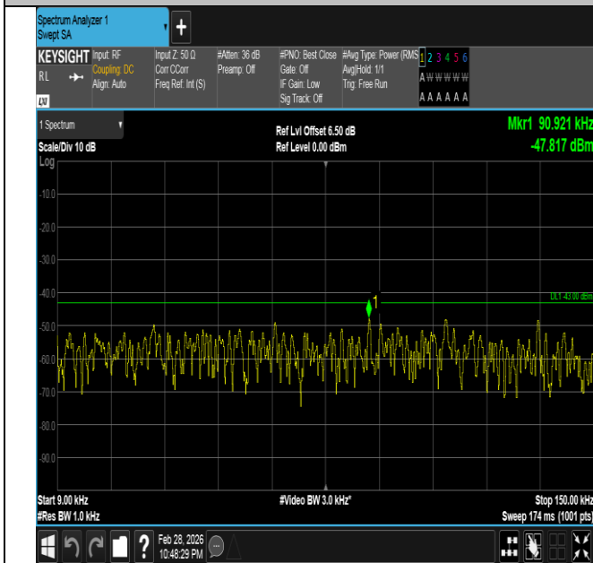
Band66-10MHz-QPSK-132022-1RB#0-0.009~0.15-PASS
