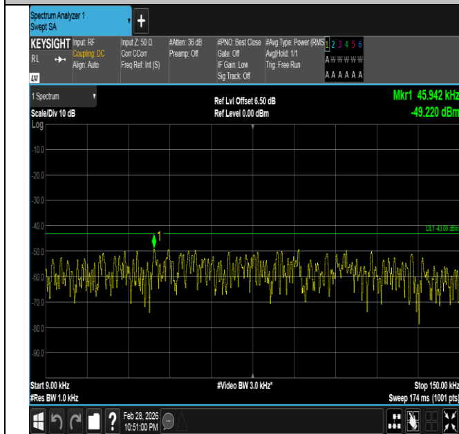
Band66-10MHz-16QAM-132022-1RB#49-0.009~0.15-PASS
