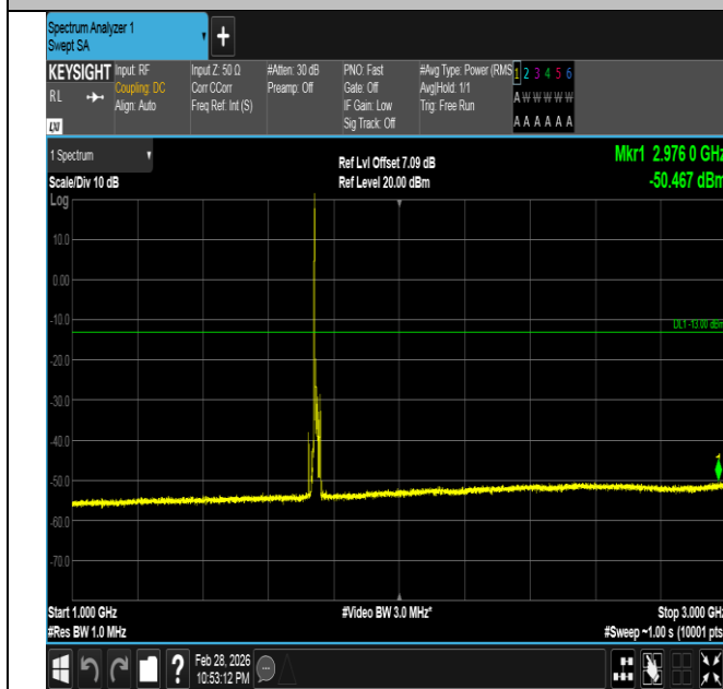
Band66-10MHz-16QAM-132322-1RB#0-1000~3000-PASS
