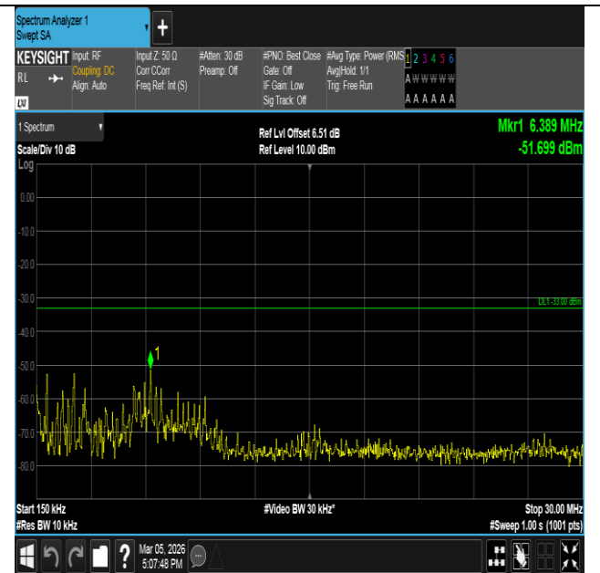
Band66-10MHz-QPSK-132022-50RB#0-0.15~30-PASS
