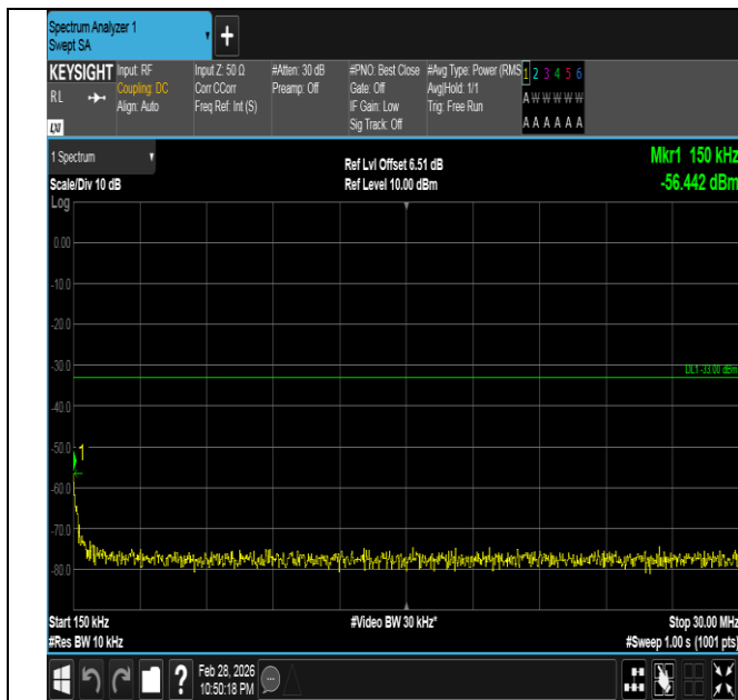
Band66-10MHz-QPSK-132022-1RB#49-0.15~30-PASS
