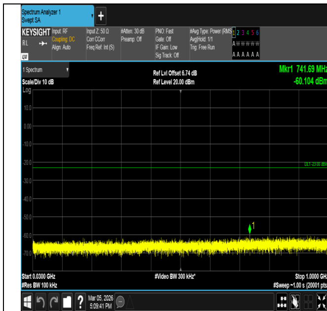
Band66-10MHz-QPSK-132322-50RB#0-30~1000-PASS
