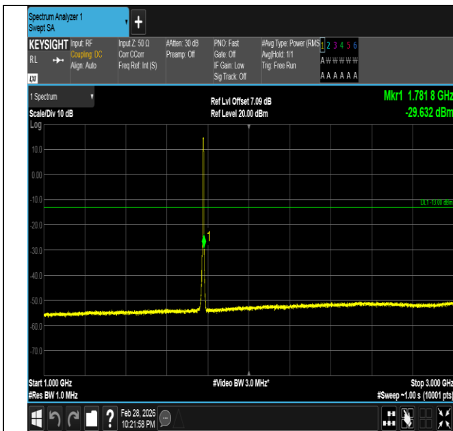
Band66-5MHz-16QAM-132647-25RB#0-1000~3000-PASS
