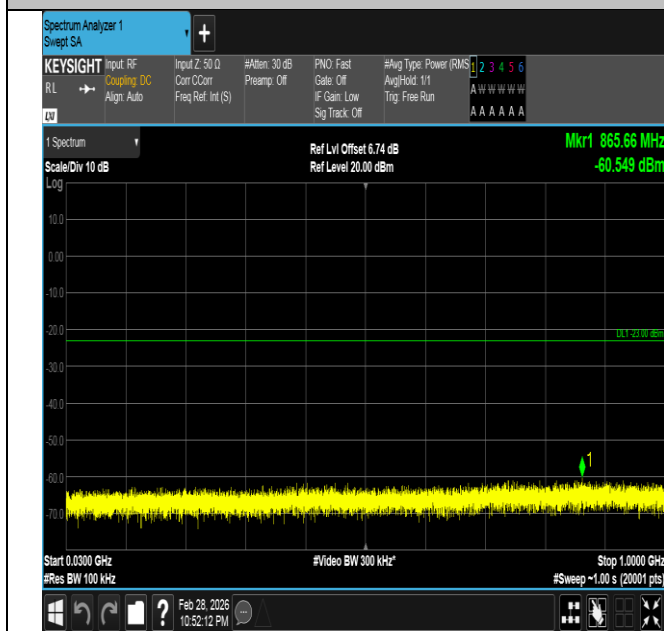
Band66-10MHz-QPSK-132322-1RB#0-30~1000-PASS
