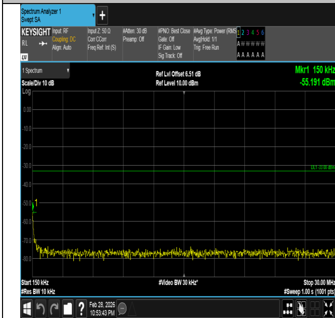
Band66-10MHz-QPSK-132322-1RB#49-0.15~30-PASS
