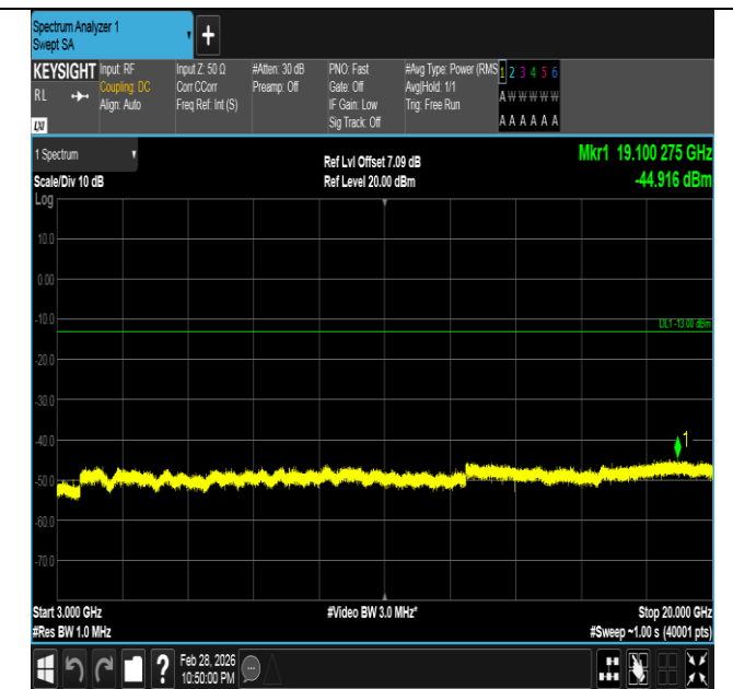
Band66-10MHz-16QAM-132022-1RB#0-3000~20000-PASS
