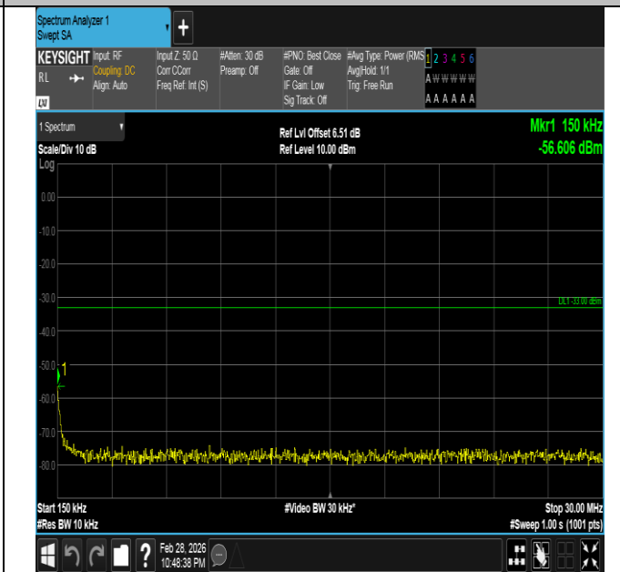
Band66-10MHz-QPSK-132022-1RB#0-0.15~30-PASS
