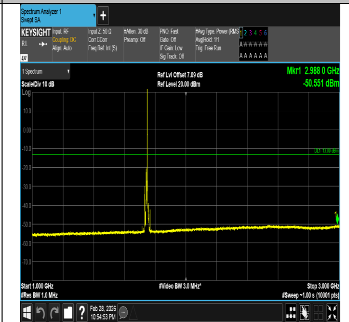
Band66-10MHz-16QAM-132322-1RB#49-1000~3000-PASS
