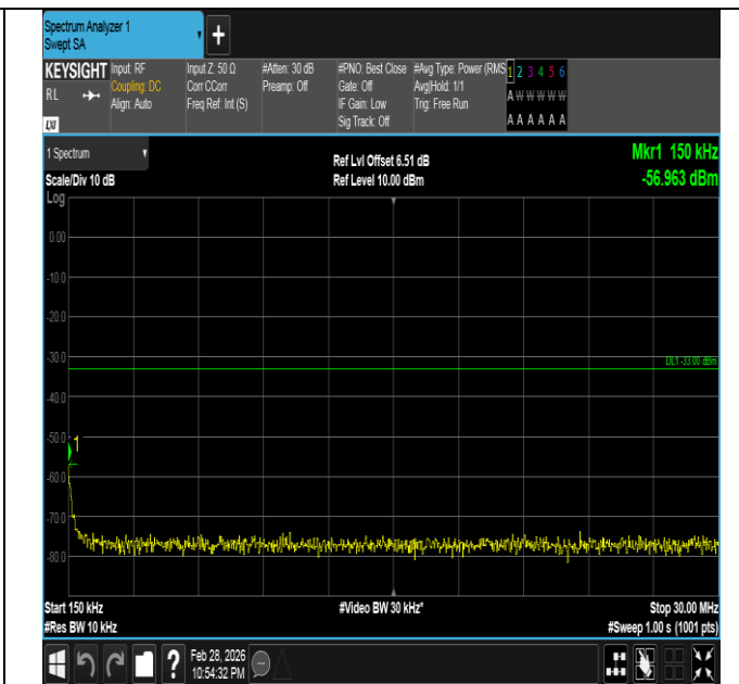
Band66-10MHz-16QAM-132322-1RB#49-0.15~30-PASS
