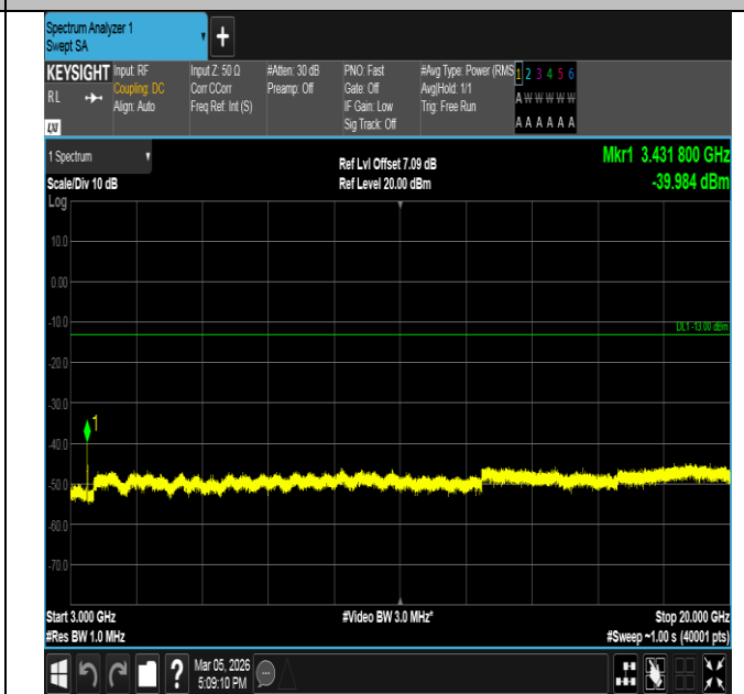
Band66-10MHz-16QAM-132022-50RB#0-3000~20000-PASS
