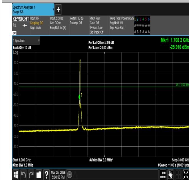
Band66-10MHz-16QAM-132022-50RB#0-1000~3000-PASS
