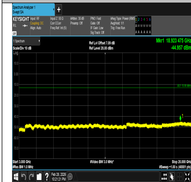
Band66-5MHz-QPSK-132647-25RB#0-3000~20000-PASS
