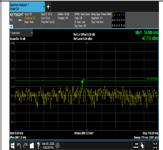
Band66-10MHz-16QAM-132022-50RB#0-0.009~0.15-PASS
