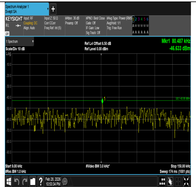
Band66-10MHz-QPSK-132322-1RB#49-0.009~0.15-PASS
