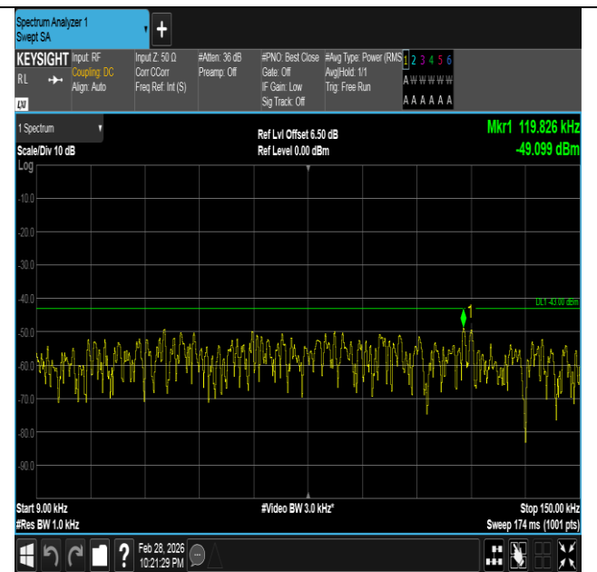
Band66-5MHz-16QAM-132647-25RB#0-0.009~0.15-PASS
