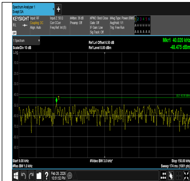
Band66-10MHz-QPSK-132322-1RB#0-0.009~0.15-PASS
