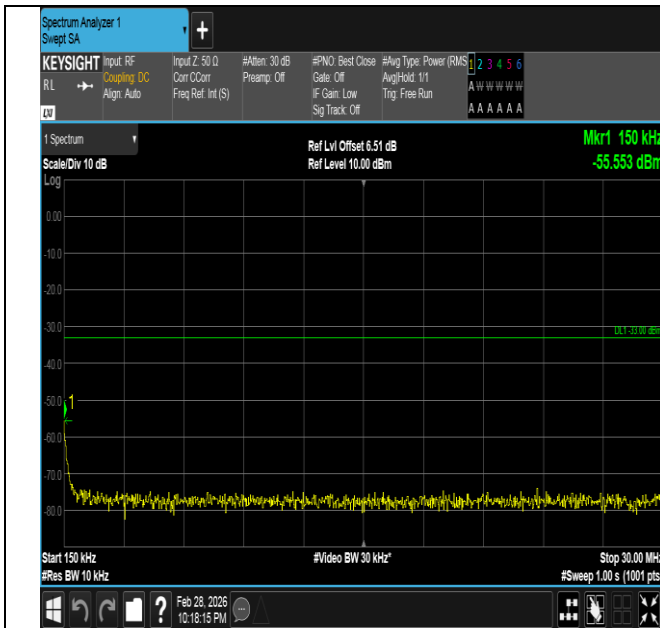
Band66-5MHz-16QAM-132647-1RB#0-0.15~30-PASS
