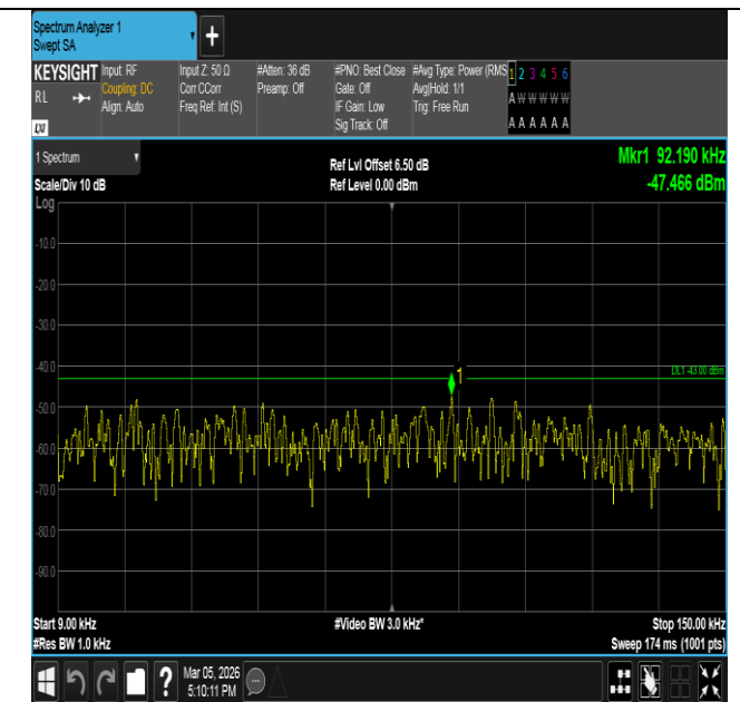
Band66-10MHz-16QAM-132322-50RB#0-0.009~0.15-PASS
