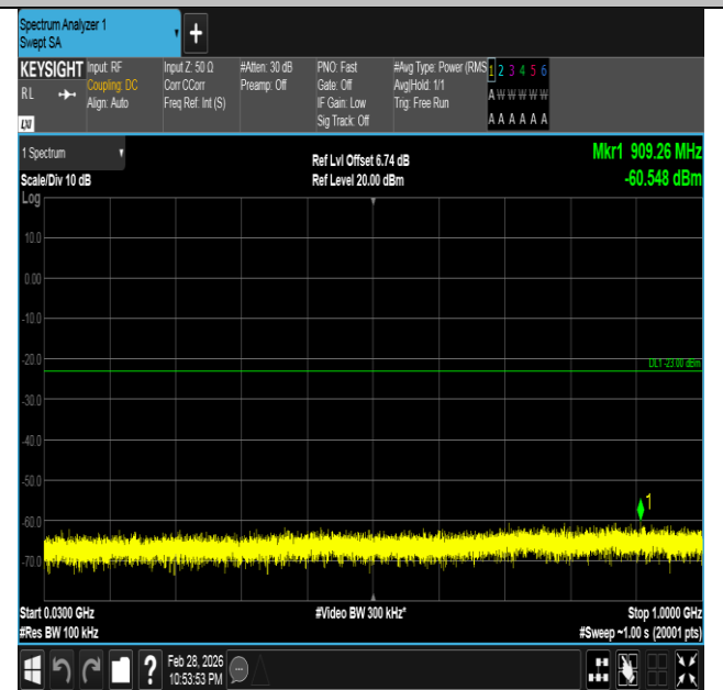
Band66-10MHz-QPSK-132322-1RB#49-30~1000-PASS
