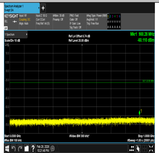
Band66-5MHz-16QAM-132647-25RB#0-30~1000-PASS
