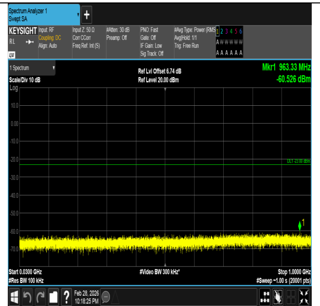
Band66-5MHz-16QAM-132647-1RB#0-30~1000-PASS
