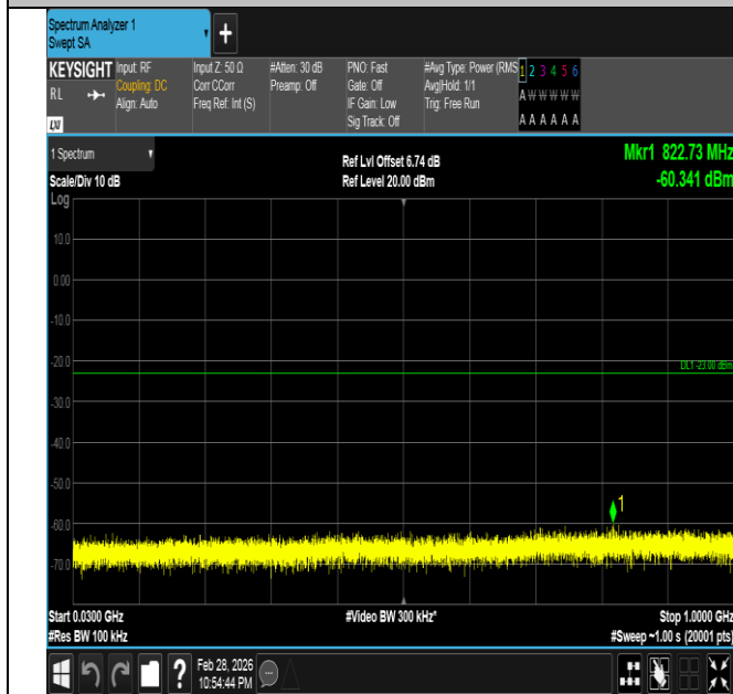
Band66-10MHz-16QAM-132322-1RB#49-30~1000-PASS
