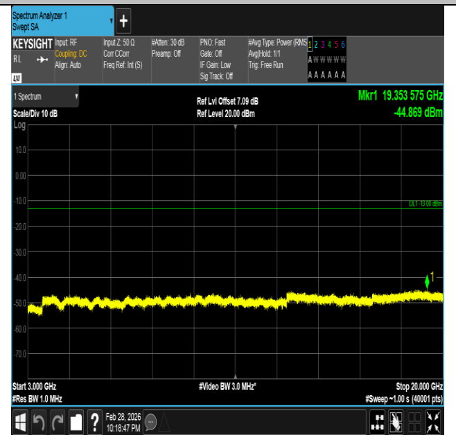
Band66-5MHz-16QAM-132647-1RB#0-3000~20000-PASS
