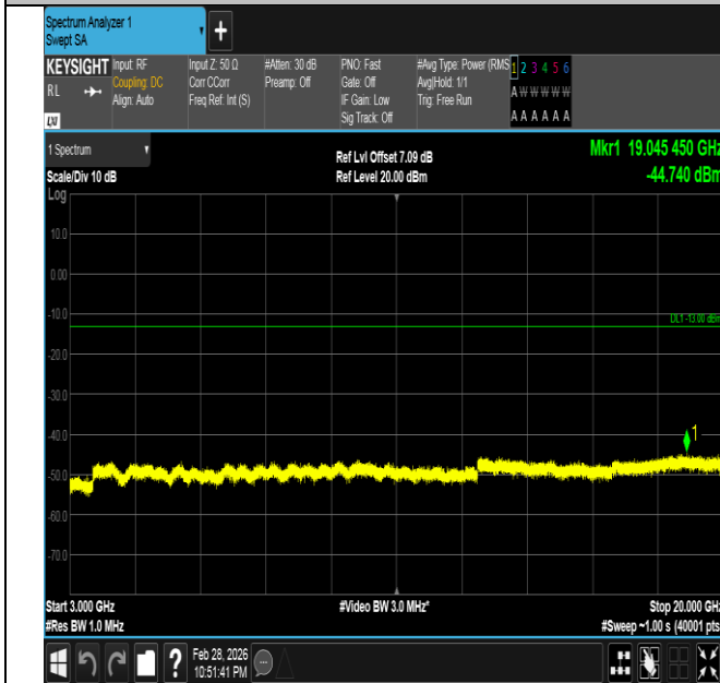
Band66-10MHz-16QAM-132022-1RB#49-3000~20000-PASS
