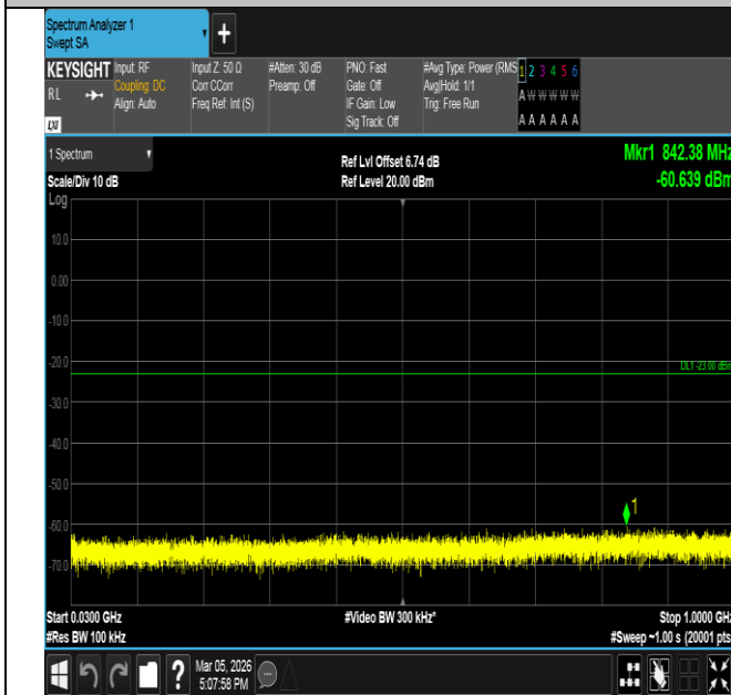
Band66-10MHz-QPSK-132022-50RB#0-30~1000-PASS
