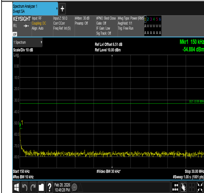
Band66-10MHz-16QAM-132022-1RB#0-0.15~30-PASS
