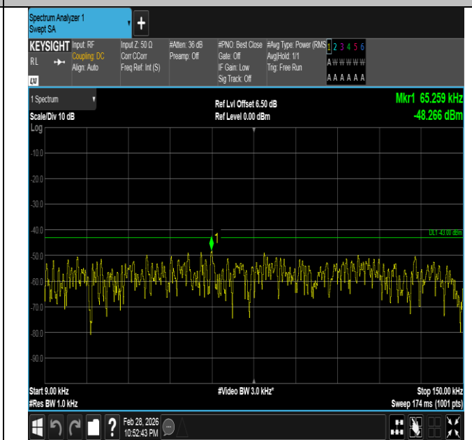
Band66-10MHz-16QAM-132322-1RB#0-0.009~0.15-PASS
