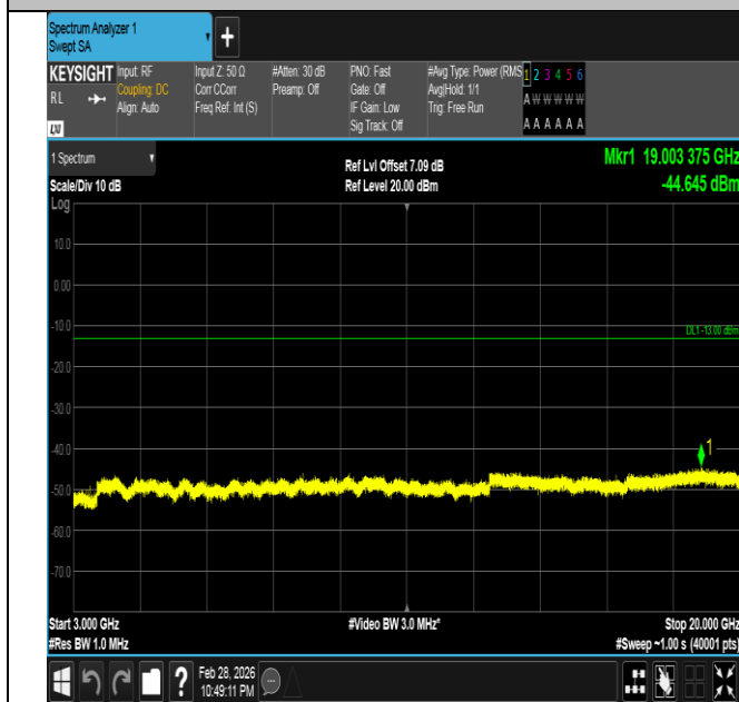
Band66-10MHz-QPSK-132022-1RB#0-3000~20000-PASS
