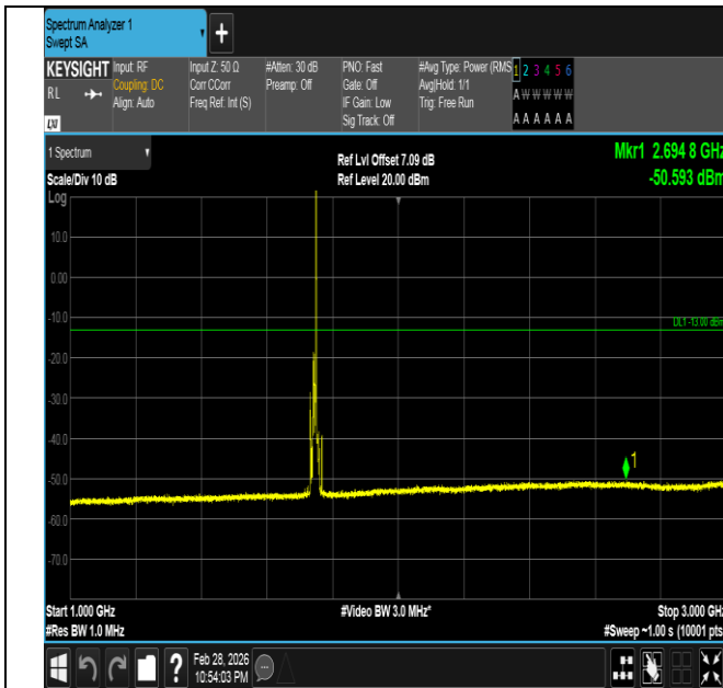
Band66-10MHz-QPSK-132322-1RB#49-1000~3000-PASS
