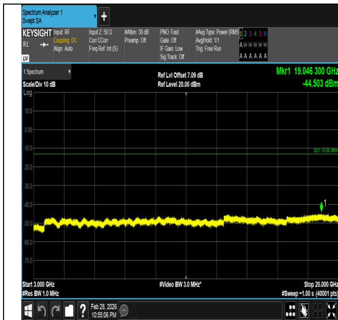
Band66-10MHz-16QAM-132322-1RB#49-3000~20000-PASS
