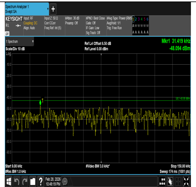
Band66-10MHz-16QAM-132022-1RB#0-0.009~0.15-PASS
