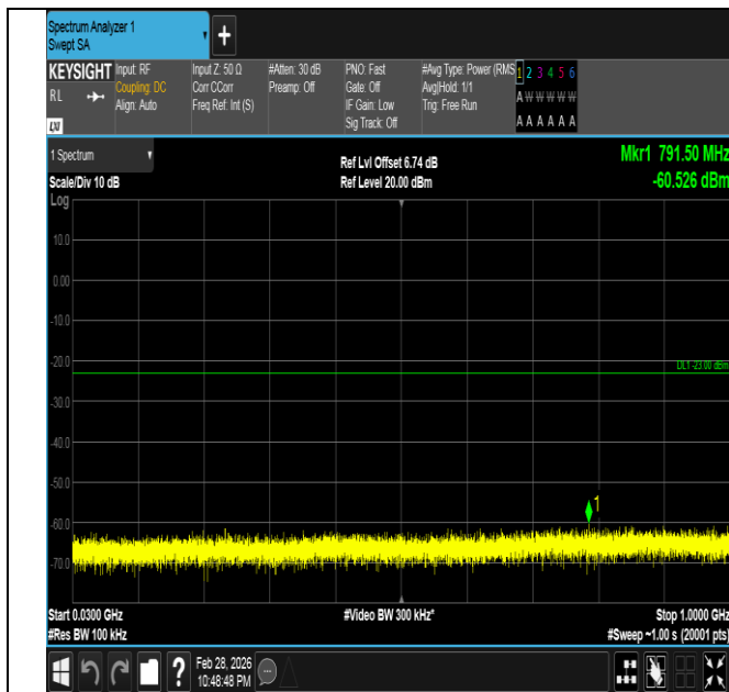
Band66-10MHz-QPSK-132022-1RB#0-30~1000-PASS
