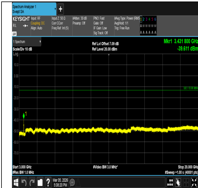
Band66-10MHz-QPSK-132022-50RB#0-3000~20000-PASS
