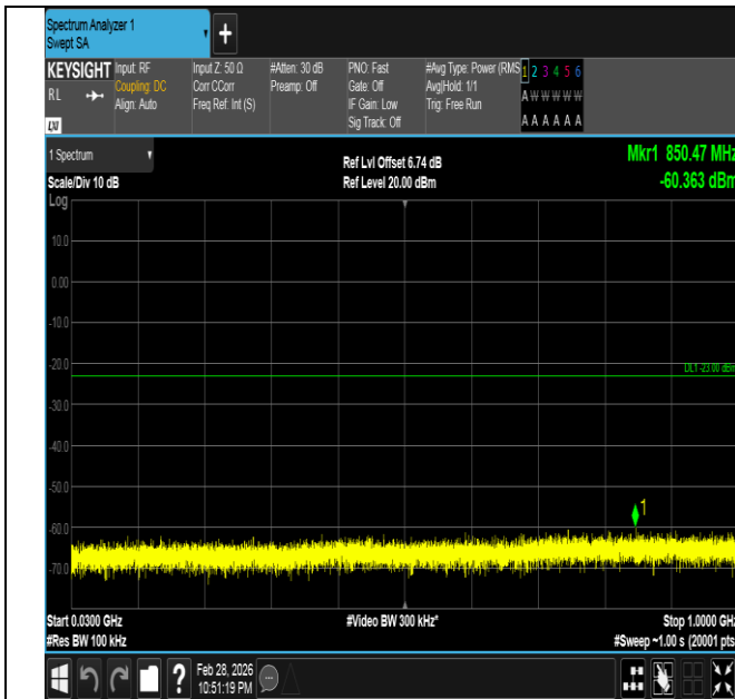
Band66-10MHz-16QAM-132022-1RB#49-30~1000-PASS
