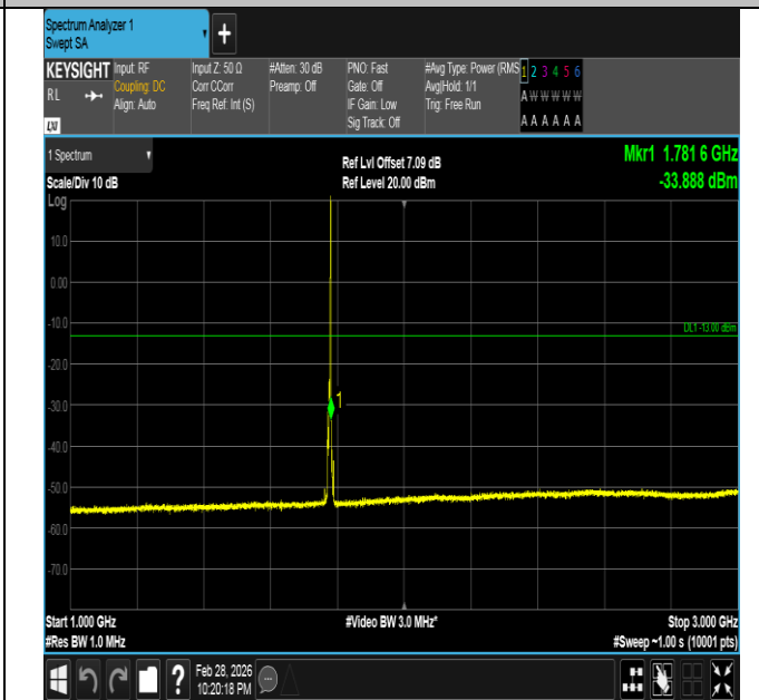
Band66-5MHz-16QAM-132647-1RB#24-1000~3000-PASS
