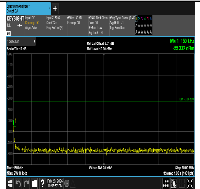
Band66-10MHz-16QAM-132622-1RB#49-0.15~30-PASS
