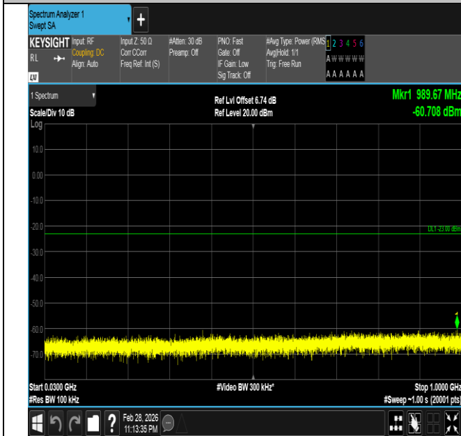
Band66-15MHz-16QAM-132047-1RB#74-30~1000-PASS
