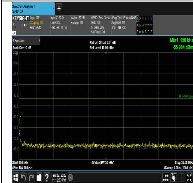
Band66-15MHz-QPSK-132047-1RB#74-0.15~30-PASS
