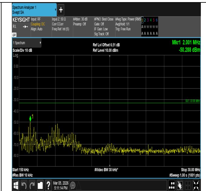
Band66-10MHz-QPSK-132622-50RB#0-0.15~30-PASS
