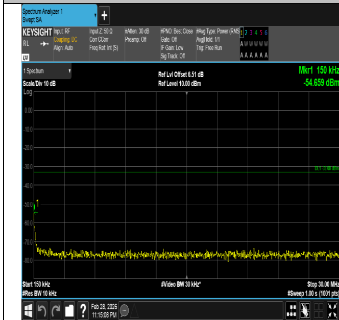
Band66-15MHz-16QAM-132322-1RB#0-0.15~30-PASS
