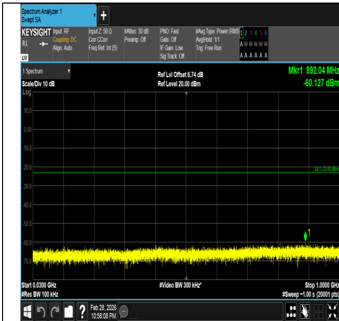
Band66-10MHz-16QAM-132622-1RB#49-30~1000-PASS
