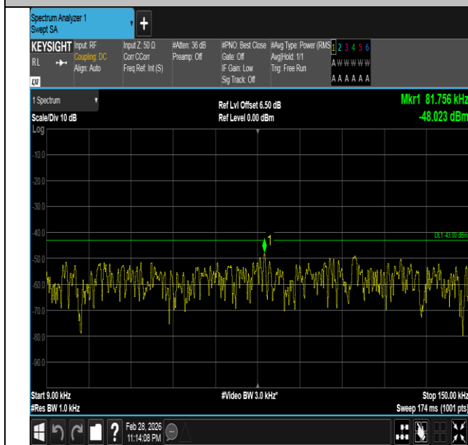
Band66-15MHz-QPSK-132322-1RB#0-0.009~0.15-PASS
