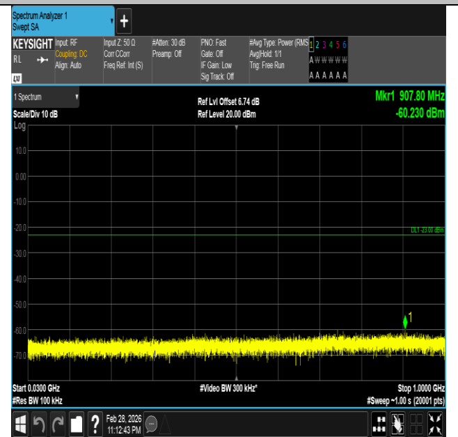
Band66-15MHz-QPSK-132047-1RB#74-30~1000-PASS
