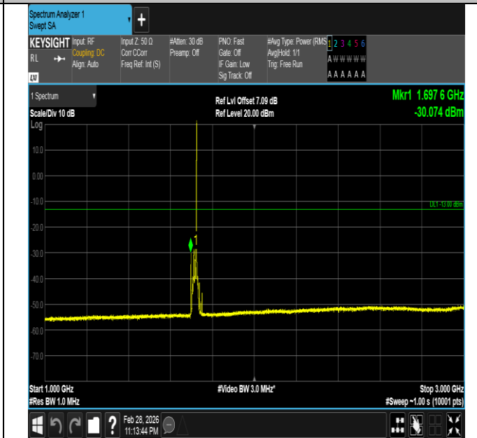
Band66-15MHz-16QAM-132047-1RB#74-1000~3000-PASS
