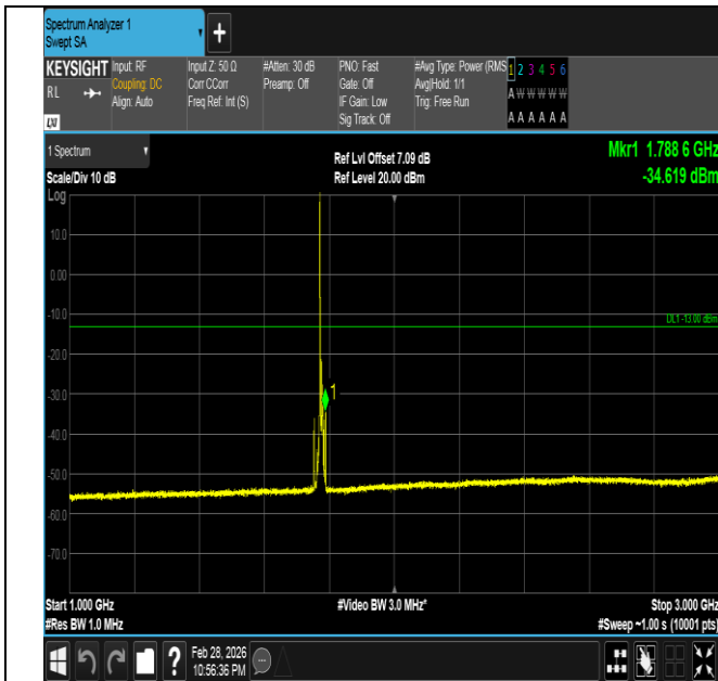
Band66-10MHz-16QAM-132622-1RB#0-1000~3000-PASS
