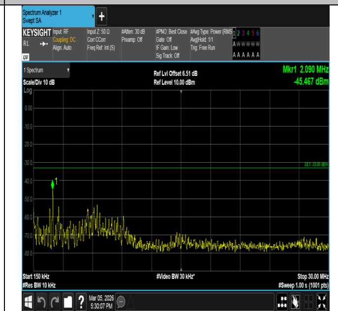
Band66-15MHz-QPSK-132047-75RB#0-0.15~30-PASS
