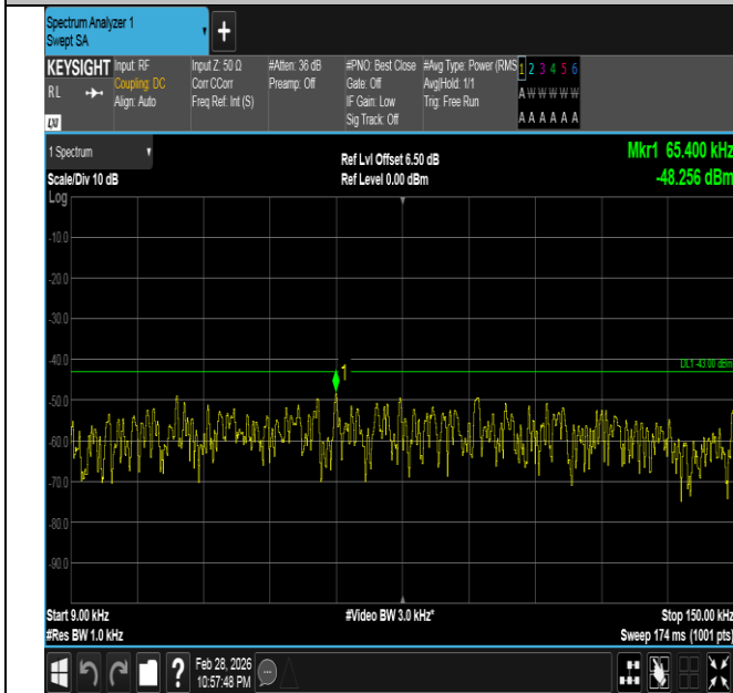
Band66-10MHz-16QAM-132622-1RB#49-0.009~0.15-PASS
