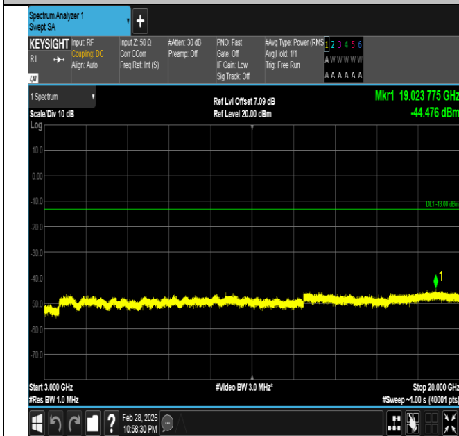
Band66-10MHz-16QAM-132622-1RB#49-3000~20000-PASS
