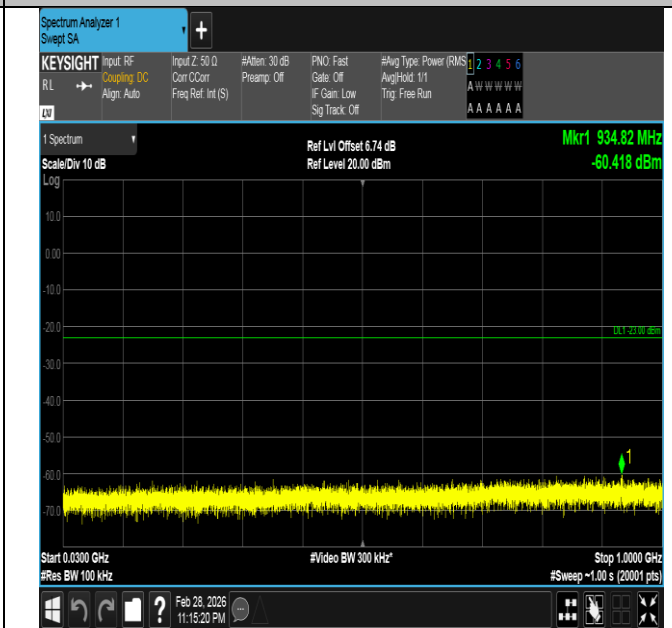
Band66-15MHz-16QAM-132322-1RB#0-30~1000-PASS
