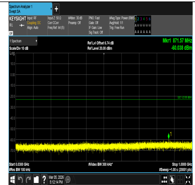
Band66-10MHz-16QAM-132622-50RB#0-30~1000-PASS
