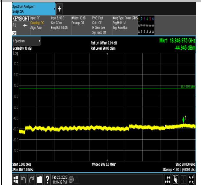
Band66-15MHz-QPSK-132322-1RB#74-3000~20000-PASS
