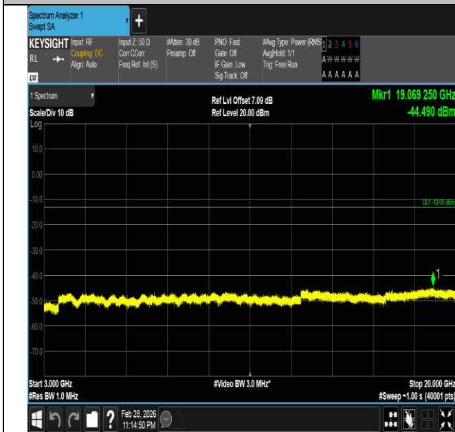
Band66-15MHz-QPSK-132322-1RB#0-3000~20000-PASS
