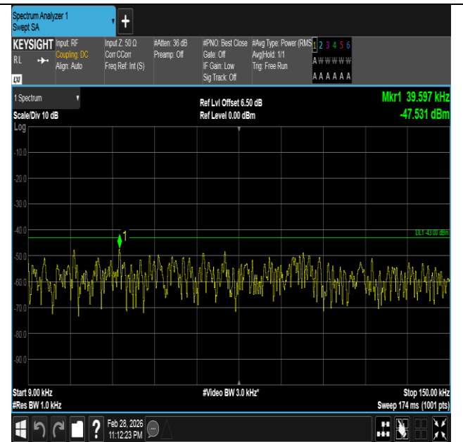
Band66-15MHz-QPSK-132047-1RB#74-0.009~0.15-PASS
