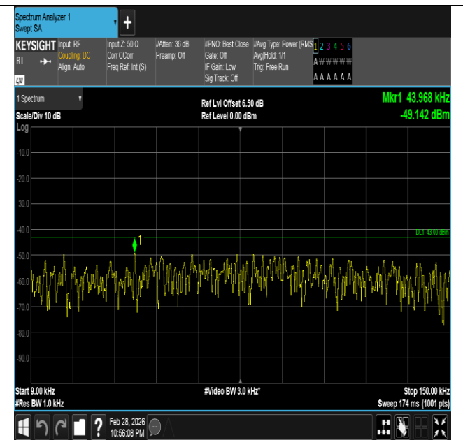
Band66-10MHz-16QAM-132622-1RB#0-0.009~0.15-PASS
