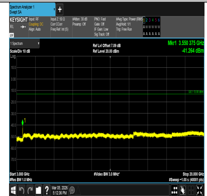
Band66-10MHz-16QAM-132622-50RB#0-3000~20000-PASS
