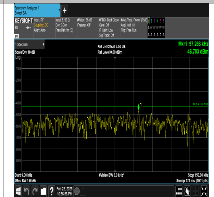
Band66-10MHz-QPSK-132622-1RB#49-0.009~0.15-PASS
