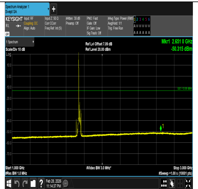
Band66-15MHz-QPSK-132322-1RB#0-1000~3000-PASS
