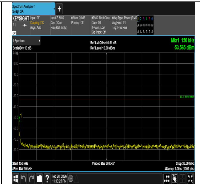
Band66-15MHz-16QAM-132047-1RB#74-0.15~30-PASS
