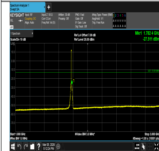
Band66-10MHz-16QAM-132622-50RB#0-1000~3000-PASS
