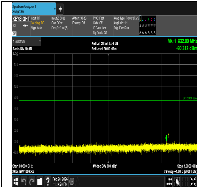
Band66-15MHz-QPSK-132322-1RB#0-30~1000-PASS
