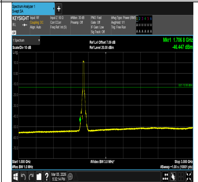
Band66-15MHz-QPSK-132322-75RB#0-1000~3000-PASS
