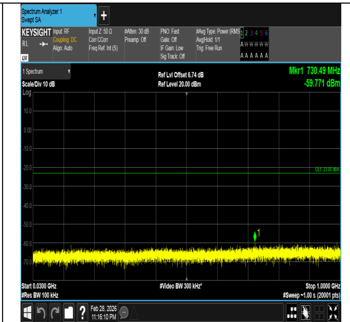
Band66-15MHz-QPSK-132322-1RB#74-30~1000-PASS
