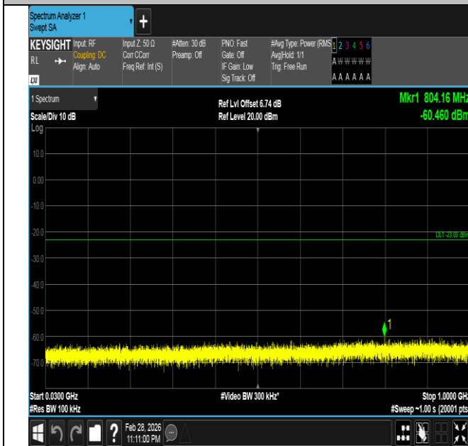
Band66-15MHz-QPSK-132047-1RB#0-30~1000-PASS
