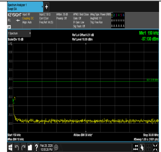
Band66-10MHz-QPSK-132622-1RB#0-0.15~30-PASS
