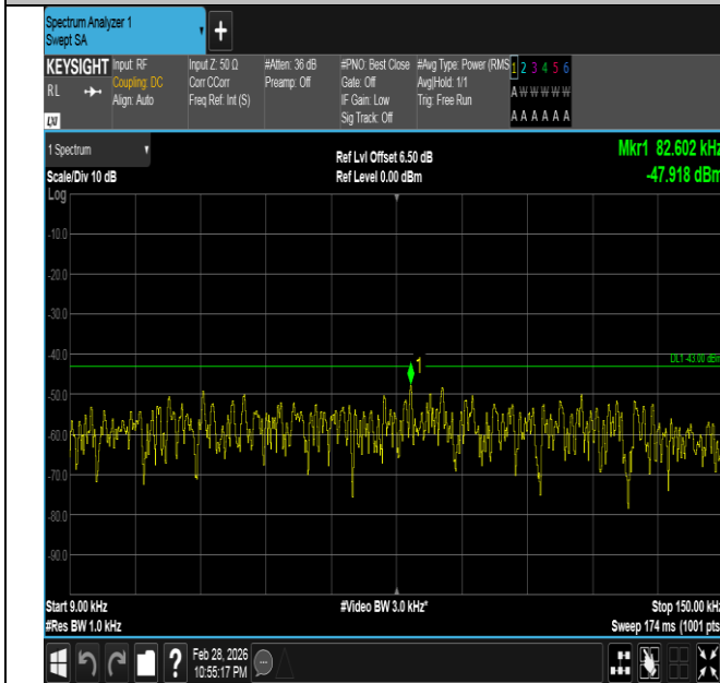
Band66-10MHz-QPSK-132622-1RB#0-0.009~0.15-PASS
