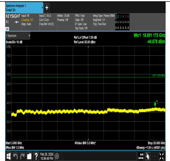
Band66-10MHz-16QAM-132622-1RB#0-3000~20000-PASS
