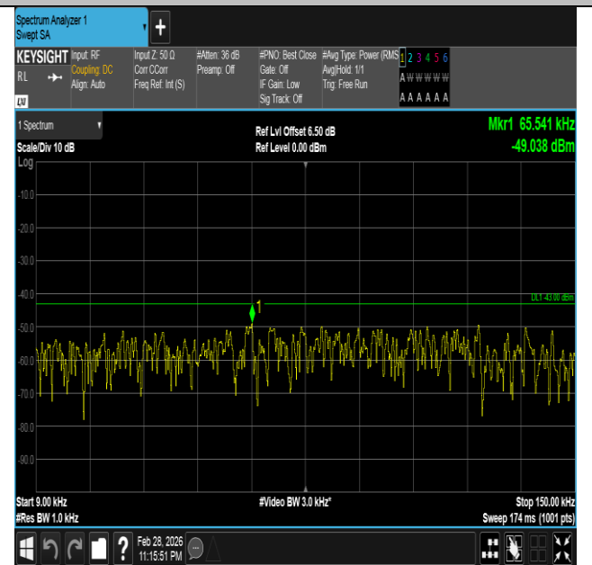
Band66-15MHz-QPSK-132322-1RB#74-0.009~0.15-PASS
