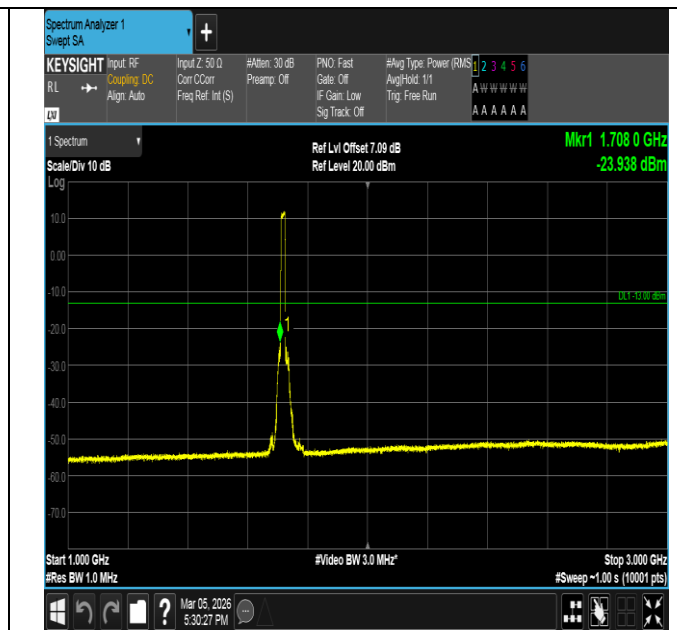
Band66-15MHz-QPSK-132047-75RB#0-1000~3000-PASS
