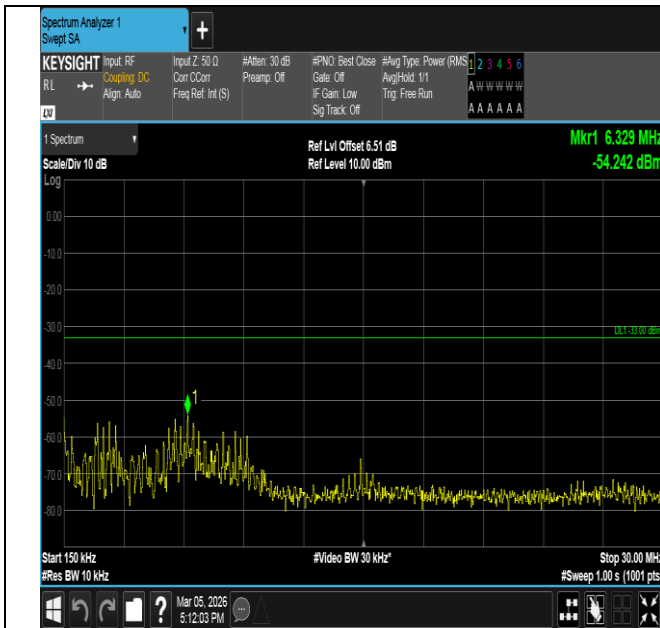
Band66-10MHz-16QAM-132622-50RB#0-0.15~30-PASS
