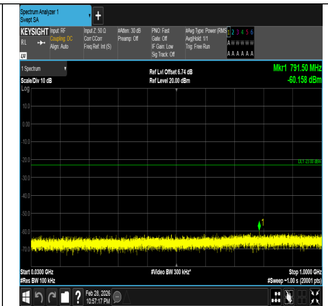
Band66-10MHz-QPSK-132622-1RB#49-30~1000-PASS
