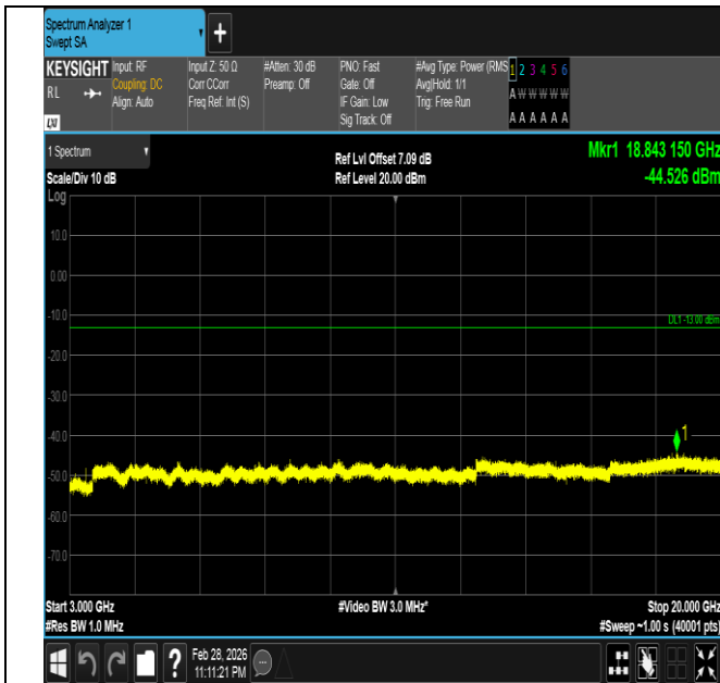
Band66-15MHz-QPSK-132047-1RB#0-3000~20000-PASS
