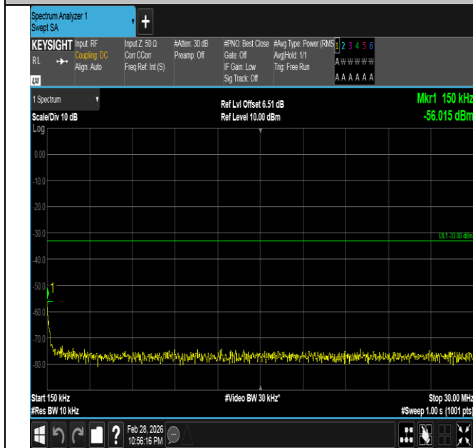
Band66-10MHz-16QAM-132622-1RB#0-0.15~30-PASS
