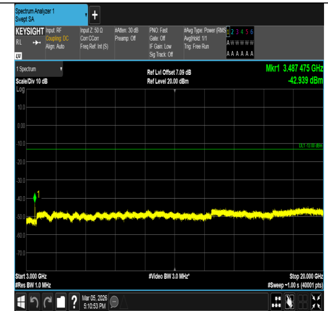
Band66-10MHz-16QAM-132322-50RB#0-3000~20000-PASS
