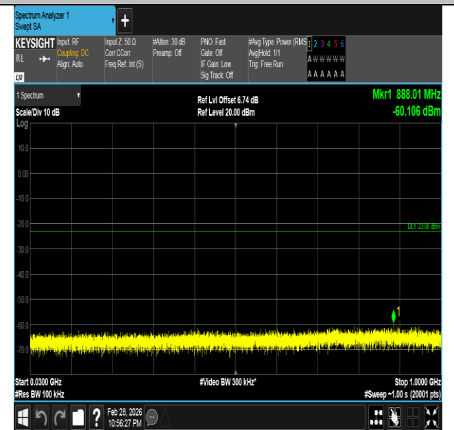
Band66-10MHz-16QAM-132622-1RB#0-30~1000-PASS
