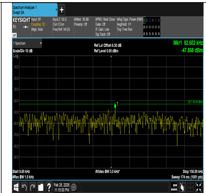
Band66-15MHz-16QAM-132322-1RB#0-0.009~0.15-PASS
