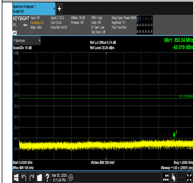
Band66-10MHz-QPSK-132622-50RB#0-30~1000-PASS
