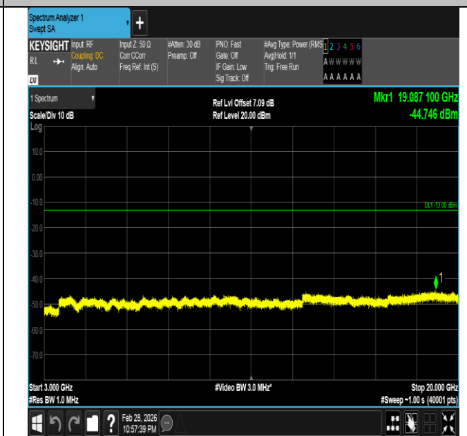
Band66-10MHz-QPSK-132622-1RB#49-3000~20000-PASS
