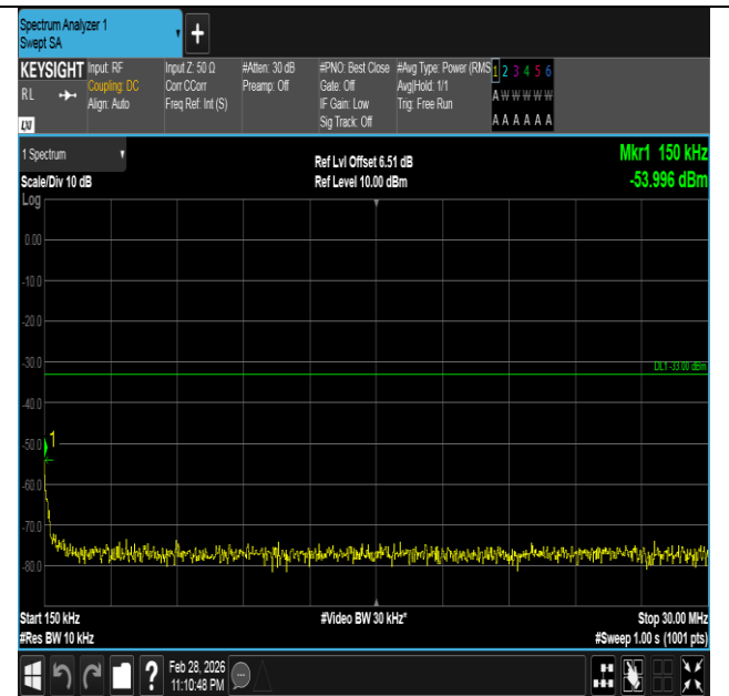
Band66-15MHz-QPSK-132047-1RB#0-0.15~30-PASS
