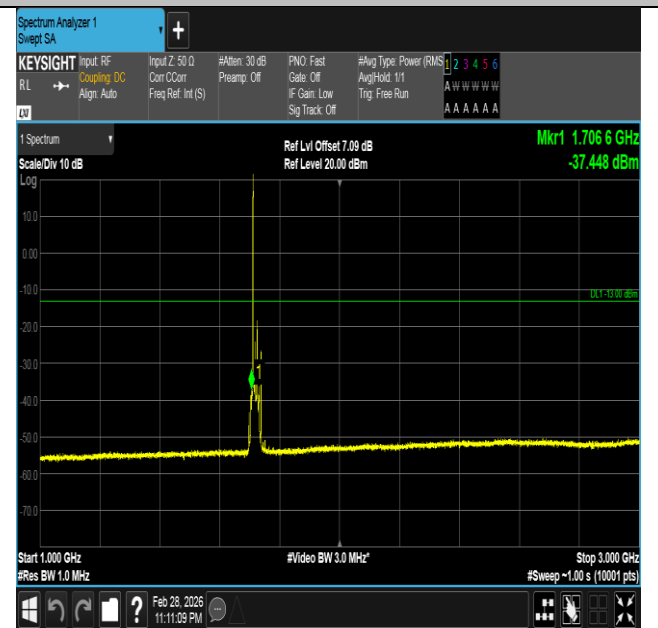
Band66-15MHz-QPSK-132047-1RB#0-1000~3000-PASS
