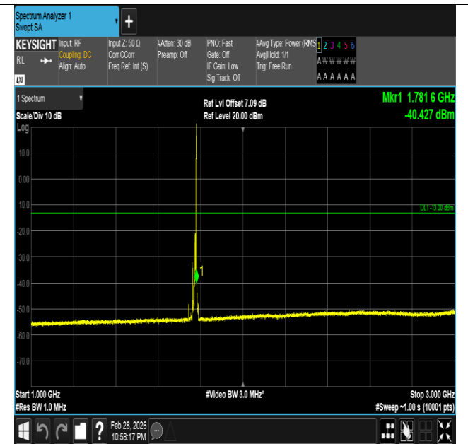
Band66-10MHz-16QAM-132622-1RB#49-1000~3000-PASS
