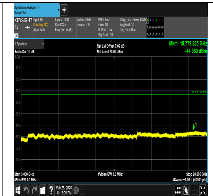
Band66-15MHz-QPSK-132047-1RB#74-3000~20000-PASS
