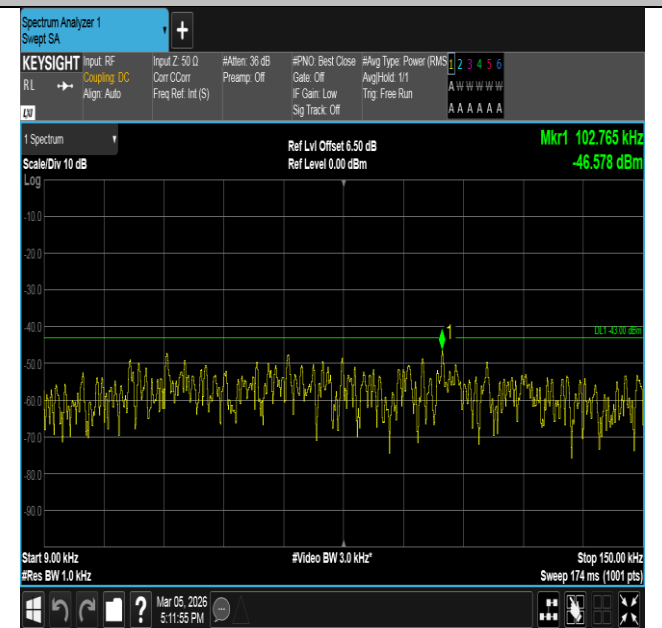
Band66-10MHz-16QAM-132622-50RB#0-0.009~0.15-PASS
