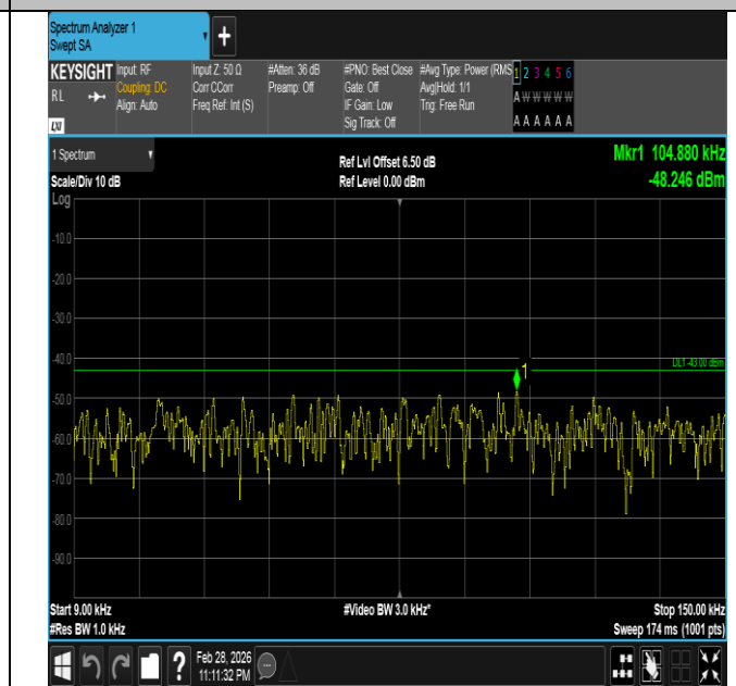
Band66-15MHz-16QAM-132047-1RB#0-0.009~0.15-PASS
