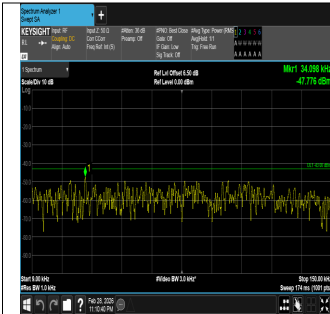
Band66-15MHz-QPSK-132047-1RB#0-0.009~0.15-PASS
