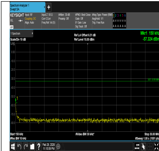
Band66-15MHz-QPSK-132322-1RB#74-0.15~30-PASS
