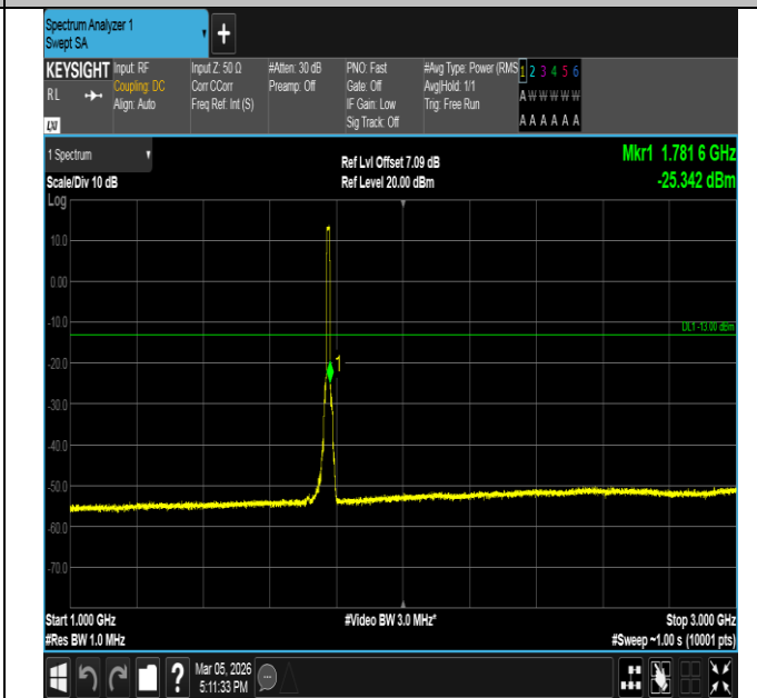
Band66-10MHz-QPSK-132622-50RB#0-1000~3000-PASS
