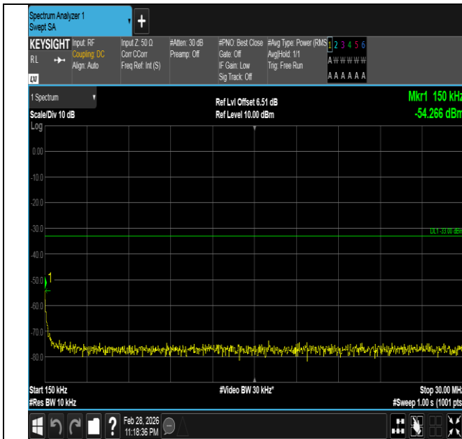
Band66-15MHz-16QAM-132597-1RB#0-0.15~30-PASS
