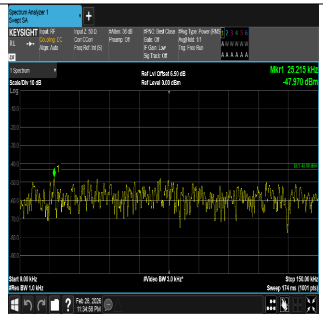
Band66-20MHz-16QAM-132072-1RB#0-0.009~0.15-PASS
