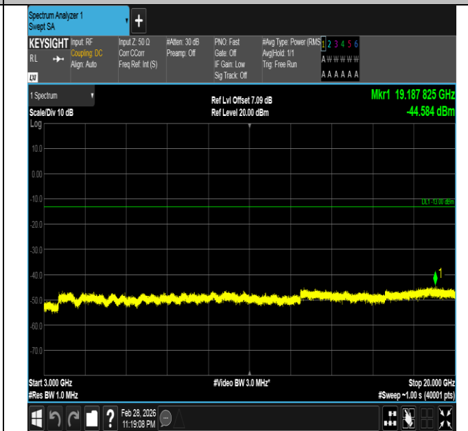
Band66-15MHz-16QAM-132597-1RB#0-3000~20000-PASS
