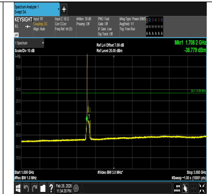
Band66-20MHz-QPSK-132072-1RB#0-1000~3000-PASS
