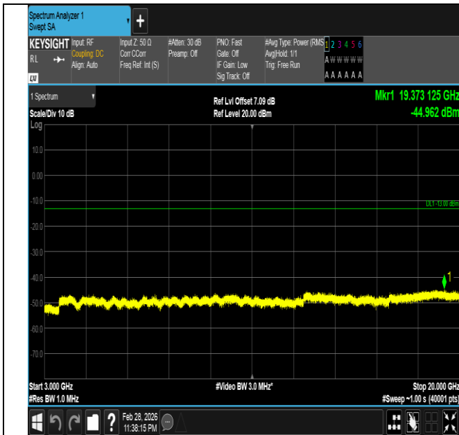
Band66-20MHz-QPSK-132322-1RB#0-3000~20000-PASS
