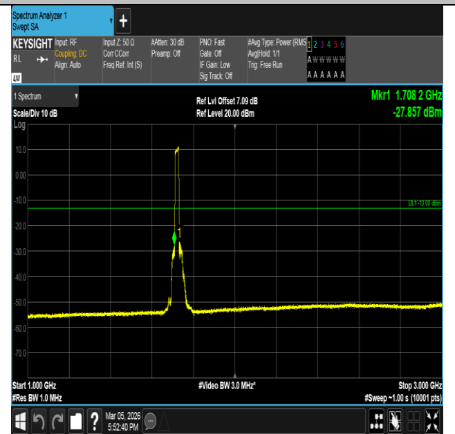
Band66-20MHz-QPSK-132072-100RB#0-1000~3000-PASS
