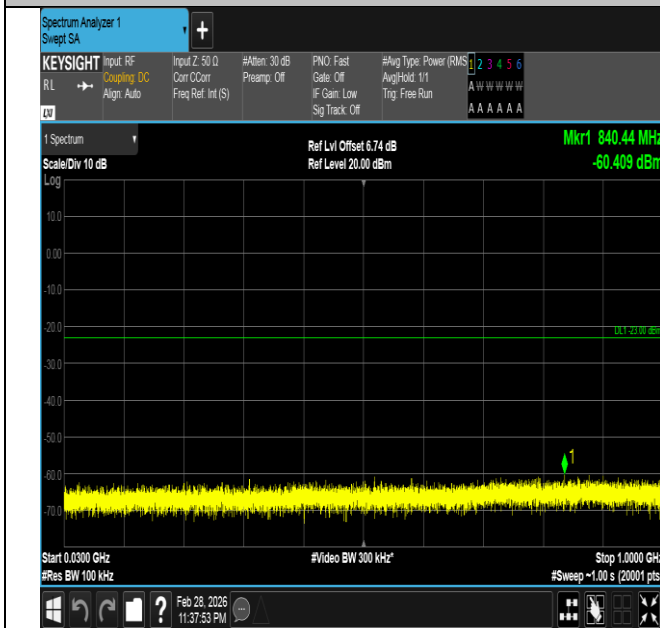
Band66-20MHz-QPSK-132322-1RB#0-30~1000-PASS
