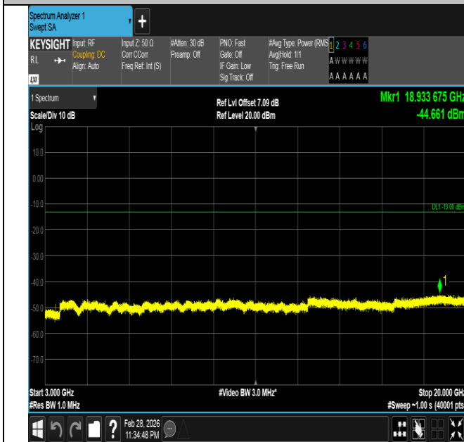
Band66-20MHz-QPSK-132072-1RB#0-3000~20000-PASS
