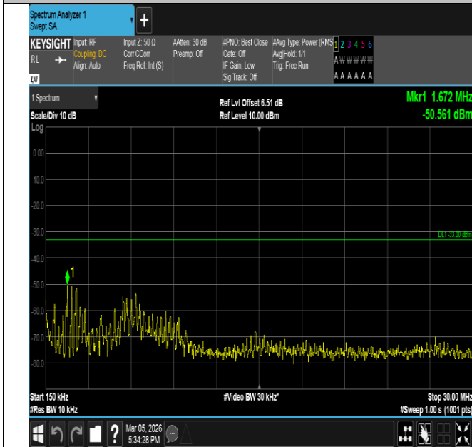
Band66-15MHz-16QAM-132597-75RB#0-0.15~30-PASS
