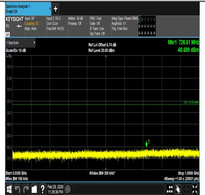
Band66-20MHz-QPSK-132322-1RB#99-30~1000-PASS
