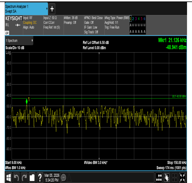
Band66-15MHz-16QAM-132597-75RB#0-0.009~0.15-PASS
