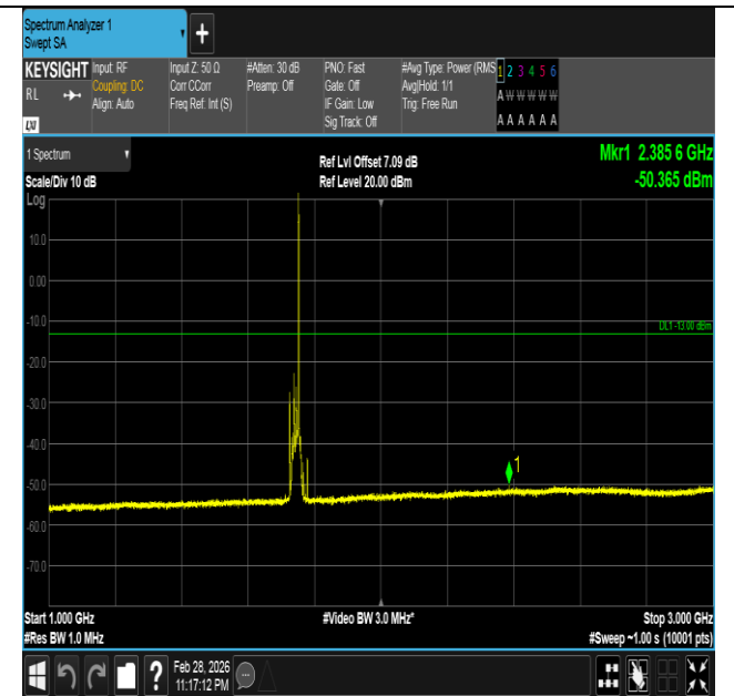
Band66-15MHz-16QAM-132322-1RB#74-1000~3000-PASS
