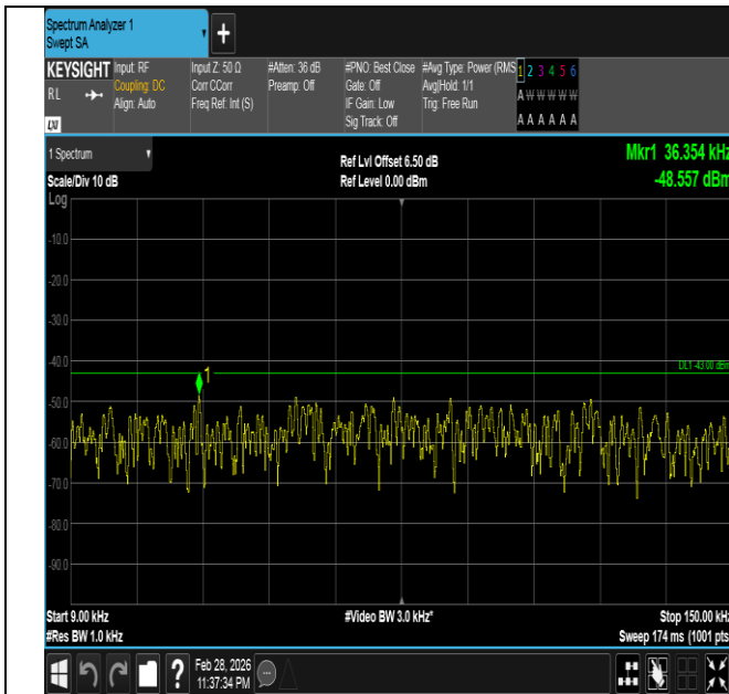
Band66-20MHz-QPSK-132322-1RB#0-0.009~0.15-PASS
