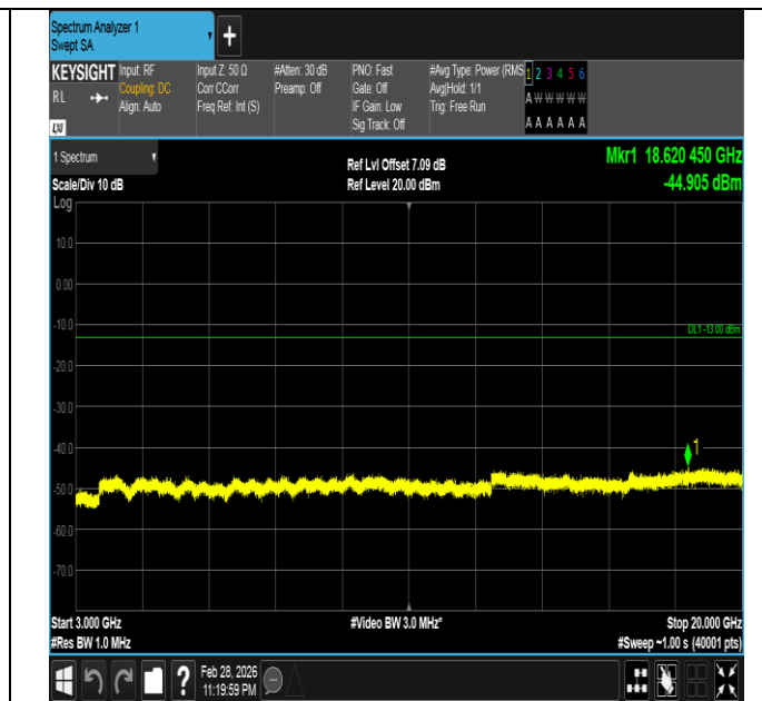
Band66-15MHz-QPSK-132597-1RB#74-3000~20000-PASS
