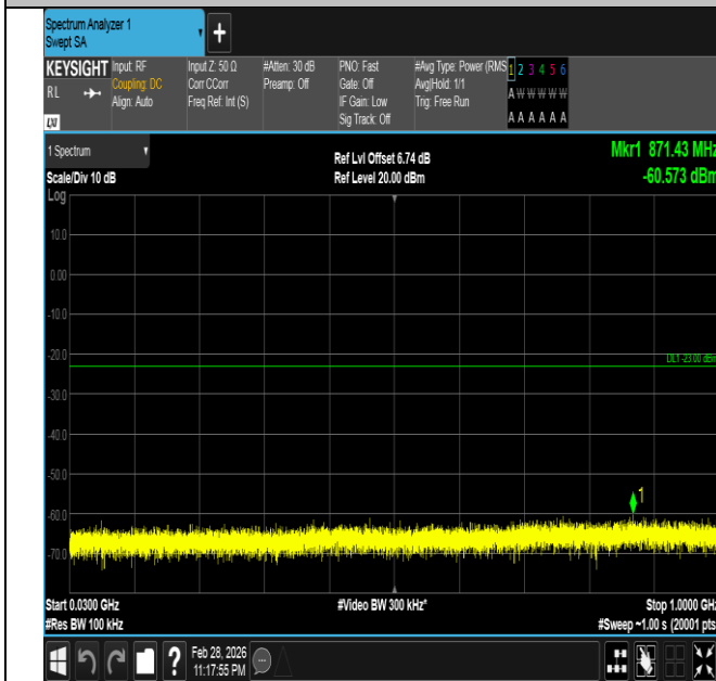
Band66-15MHz-QPSK-132597-1RB#0-30~1000-PASS
