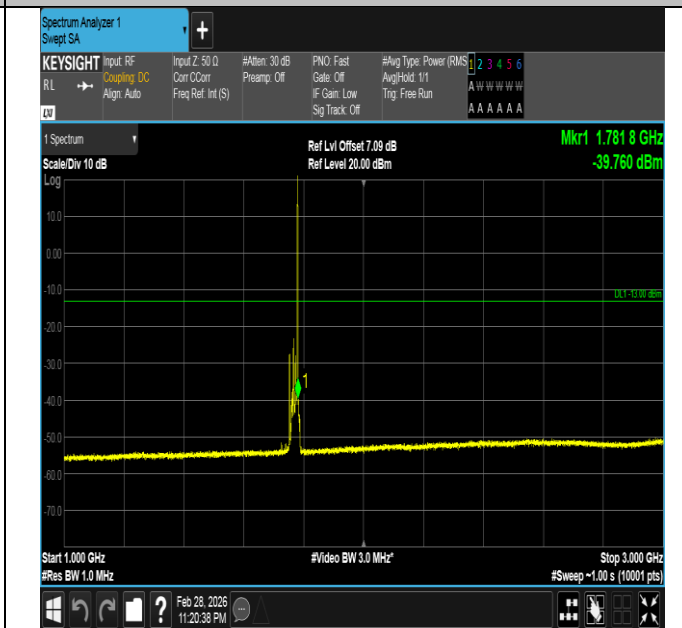
Band66-15MHz-16QAM-132597-1RB#74-1000~3000-PASS
