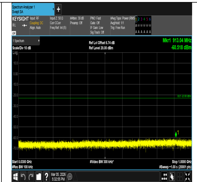
Band66-15MHz-16QAM-132322-75RB#0-30~1000-PASS
