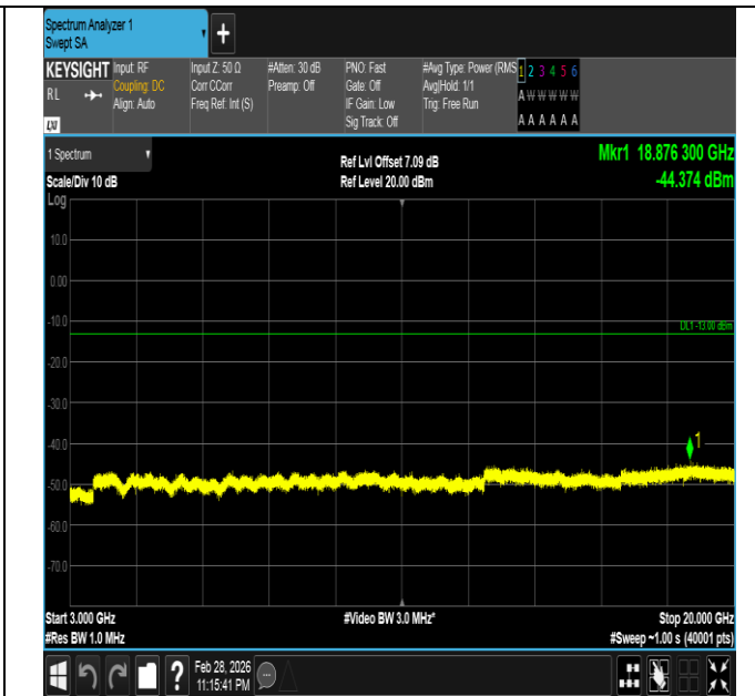
Band66-15MHz-16QAM-132322-1RB#0-3000~20000-PASS
