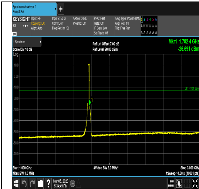
Band66-15MHz-16QAM-132597-75RB#0-1000~3000-PASS
