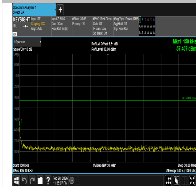
Band66-20MHz-16QAM-132072-1RB#0-0.15~30-PASS
