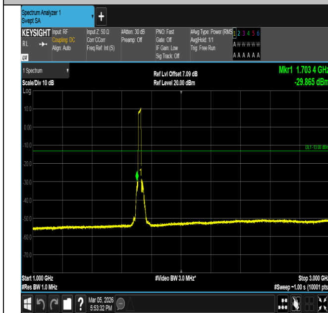
Band66-20MHz-16QAM-132072-100RB#0-1000~3000-PASS
