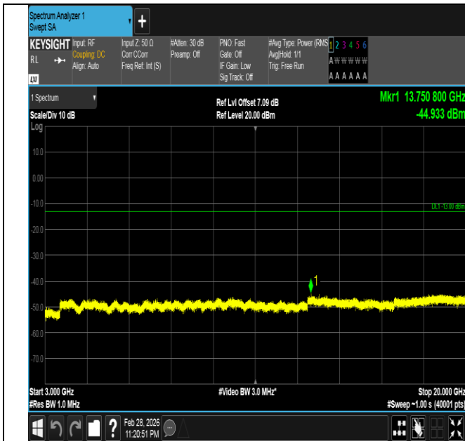
Band66-15MHz-16QAM-132597-1RB#74-3000~20000-PASS
