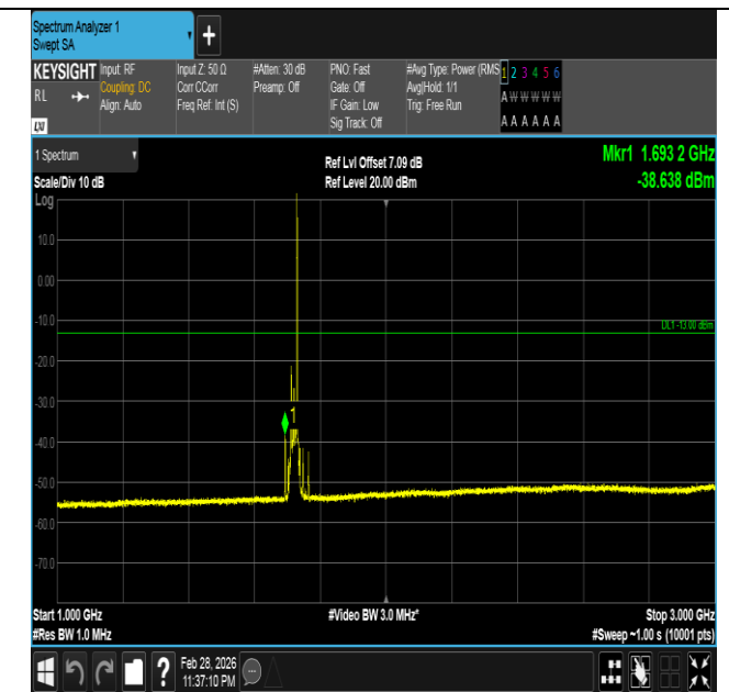
Band66-20MHz-16QAM-132072-1RB#99-1000~3000-PASS
