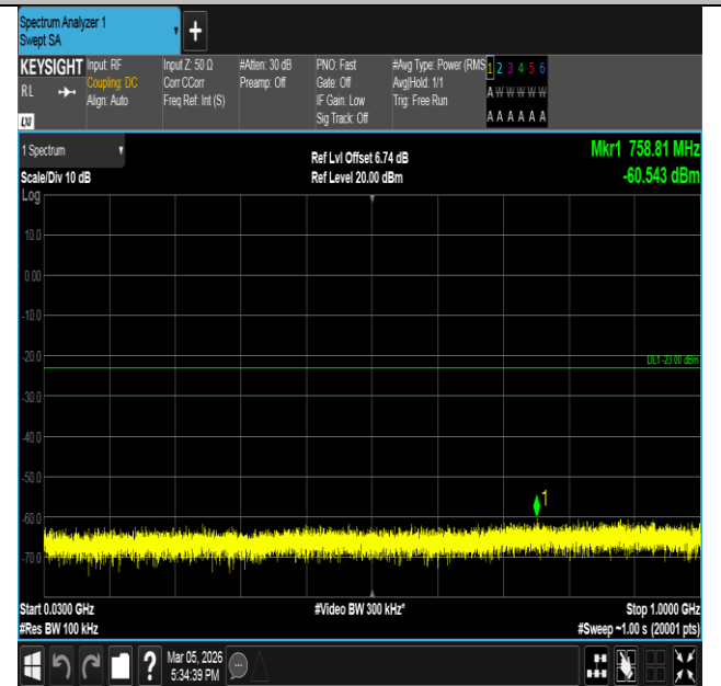
Band66-15MHz-16QAM-132597-75RB#0-30~1000-PASS
