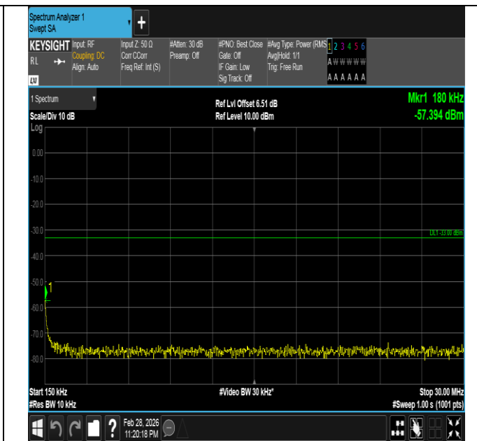
Band66-15MHz-16QAM-132597-1RB#74-0.15~30-PASS
