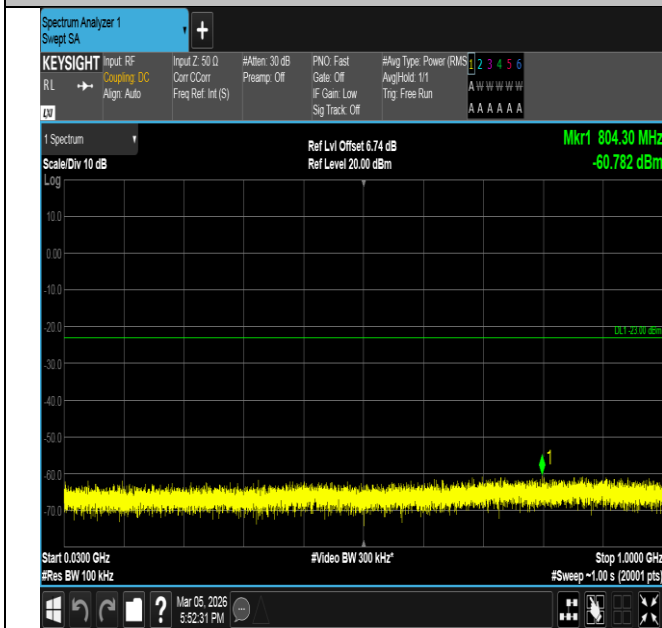
Band66-20MHz-QPSK-132072-100RB#0-30~1000-PASS
