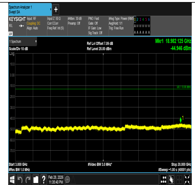
Band66-20MHz-16QAM-132072-1RB#0-3000~20000-PASS
