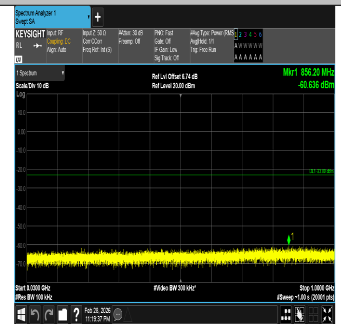
Band66-15MHz-QPSK-132597-1RB#74-30~1000-PASS
