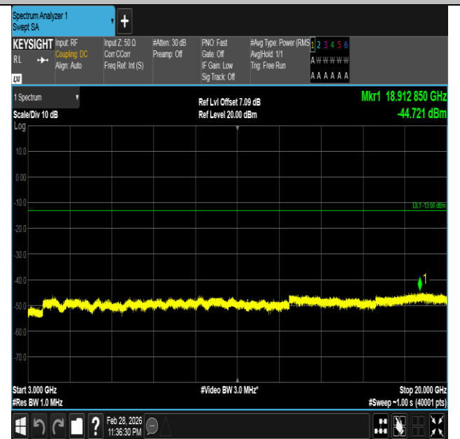
Band66-20MHz-QPSK-132072-1RB#99-3000~20000-PASS
