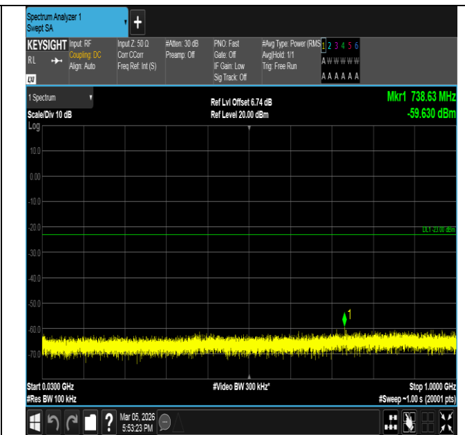
Band66-20MHz-16QAM-132072-100RB#0-30~1000-PASS
