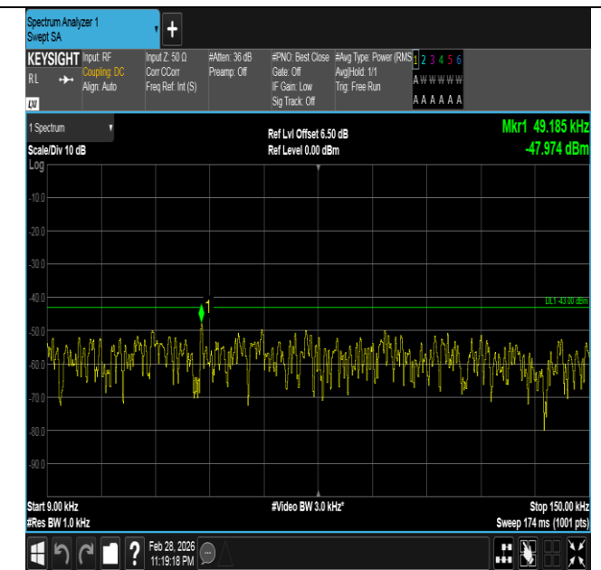
Band66-15MHz-QPSK-132597-1RB#74-0.009~0.15-PASS
