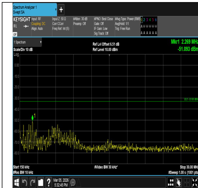
Band66-15MHz-16QAM-132322-75RB#0-0.15~30-PASS
