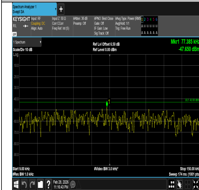
Band66-15MHz-16QAM-132322-1RB#74-0.009~0.15-PASS
