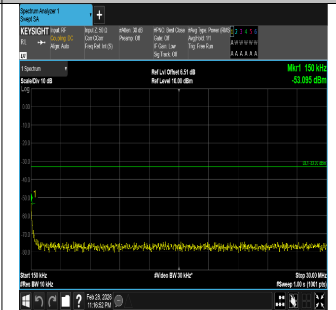
Band66-15MHz-16QAM-132322-1RB#74-0.15~30-PASS
