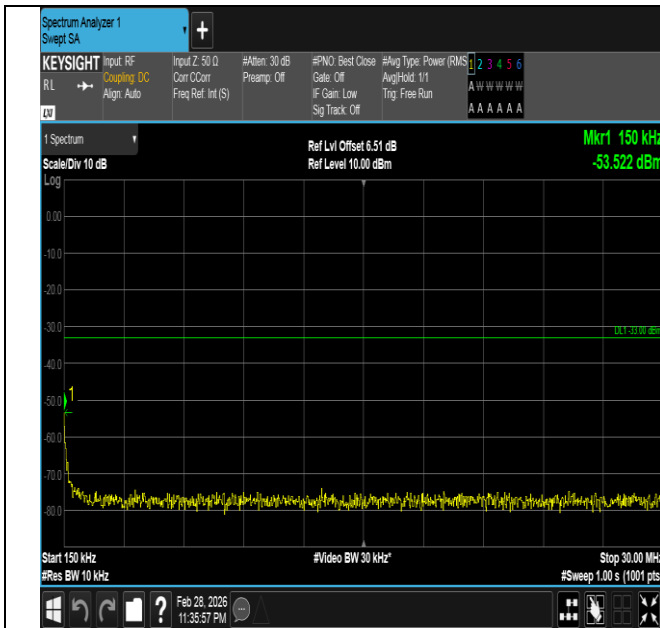
Band66-20MHz-QPSK-132072-1RB#99-0.15~30-PASS
