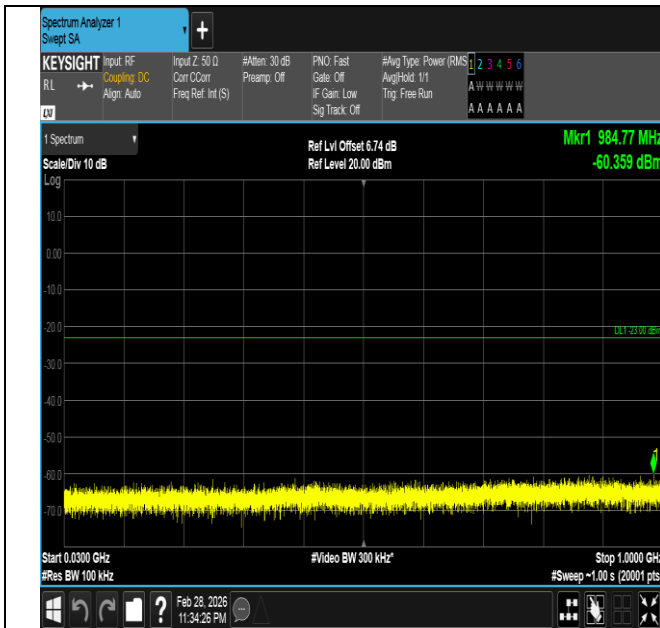
Band66-20MHz-QPSK-132072-1RB#0-30~1000-PASS
