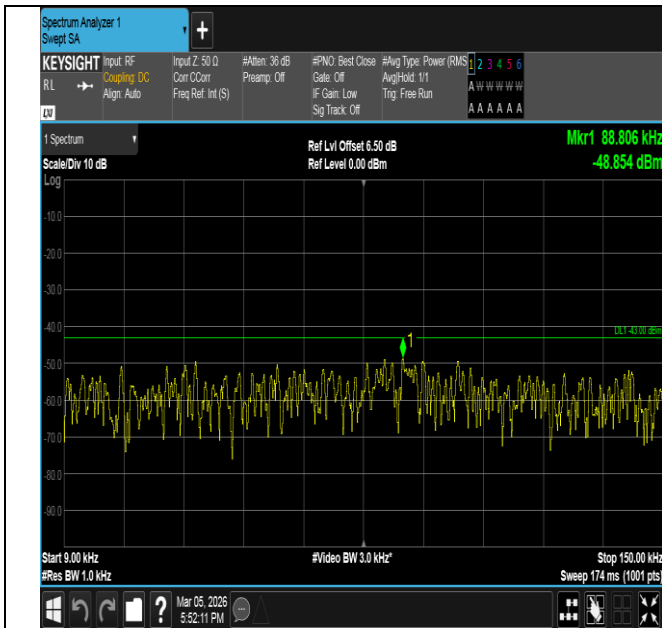
Band66-20MHz-QPSK-132072-100RB#0-0.009~0.15-PASS
