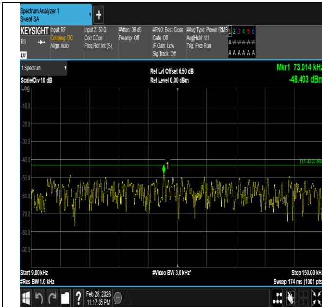
Band66-15MHz-QPSK-132597-1RB#0-0.009~0.15-PASS
