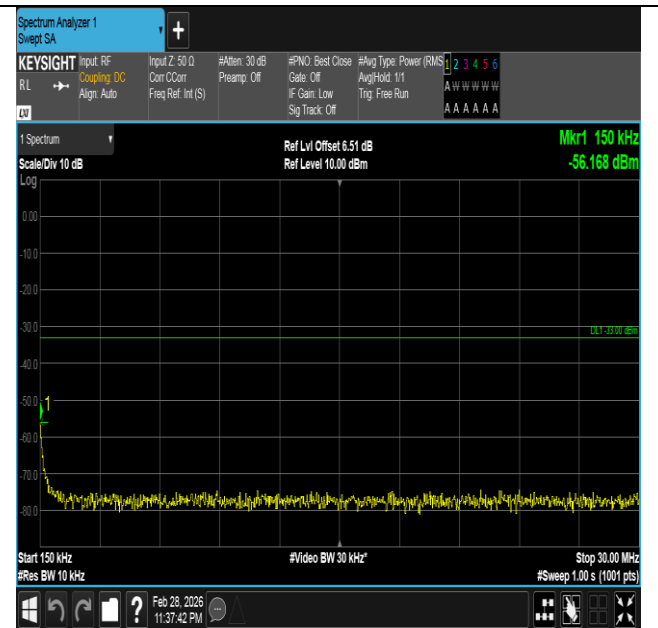
Band66-20MHz-QPSK-132322-1RB#0-0.15~30-PASS
