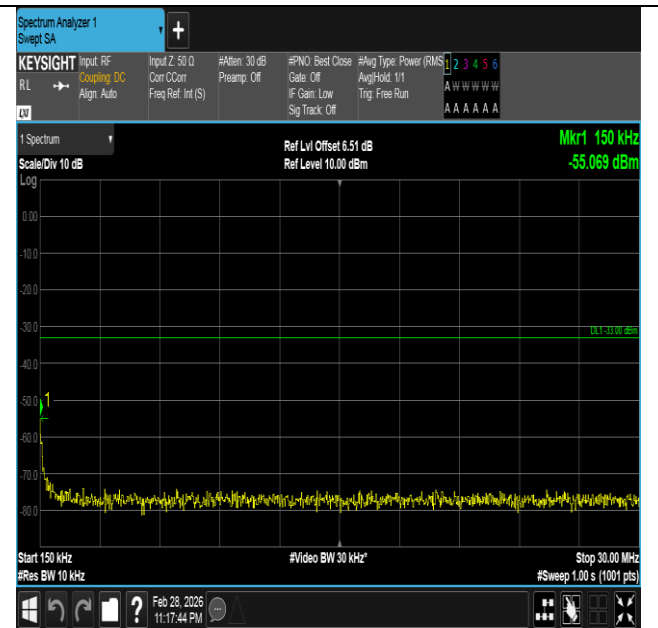
Band66-15MHz-QPSK-132597-1RB#0-0.15~30-PASS
