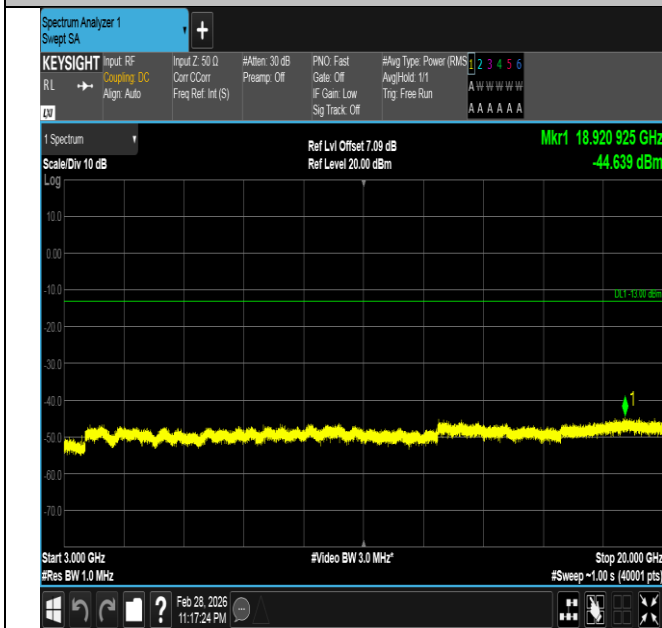
Band66-15MHz-16QAM-132322-1RB#74-3000~20000-PASS
