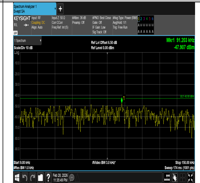
Band66-20MHz-QPSK-132072-1RB#99-0.009~0.15-PASS
