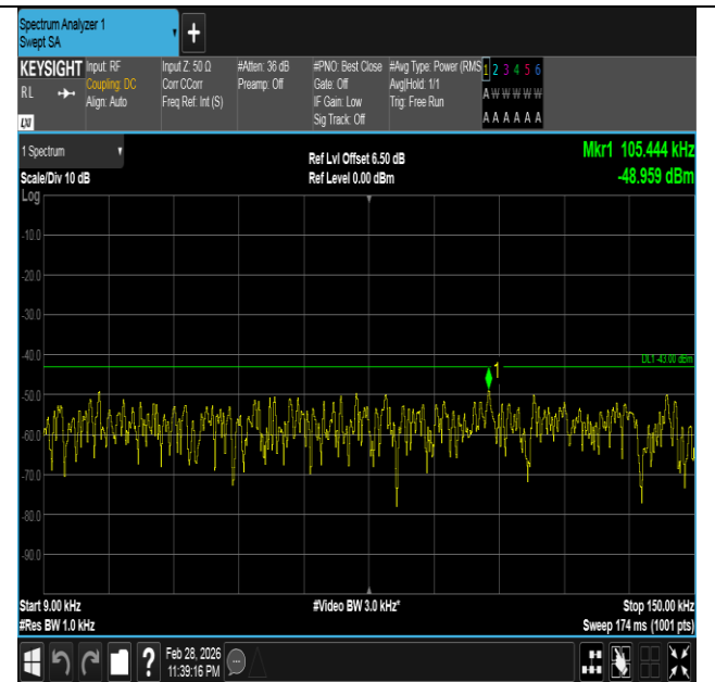
Band66-20MHz-QPSK-132322-1RB#99-0.009~0.15-PASS
