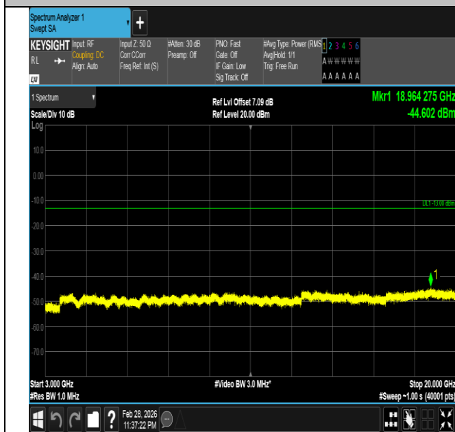
Band66-20MHz-16QAM-132072-1RB#99-3000~20000-PASS
