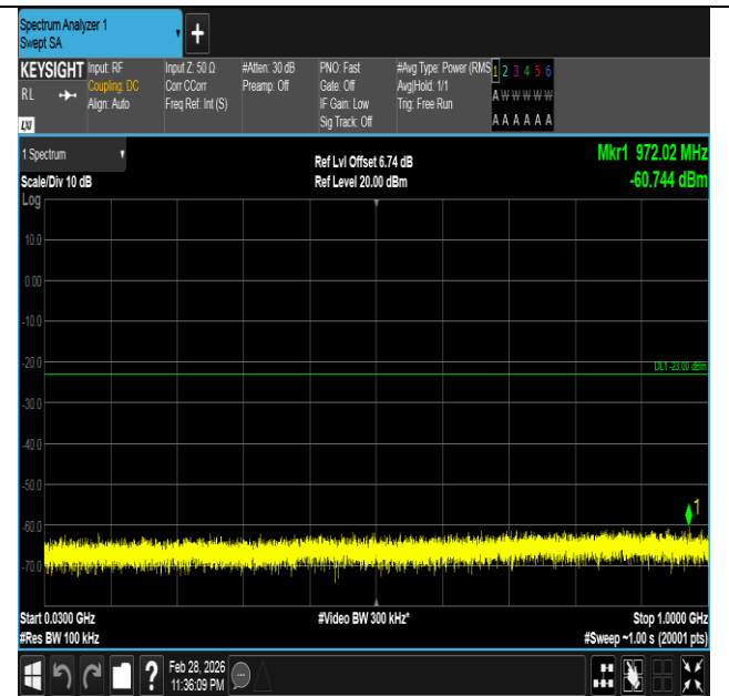
Band66-20MHz-QPSK-132072-1RB#99-30~1000-PASS
