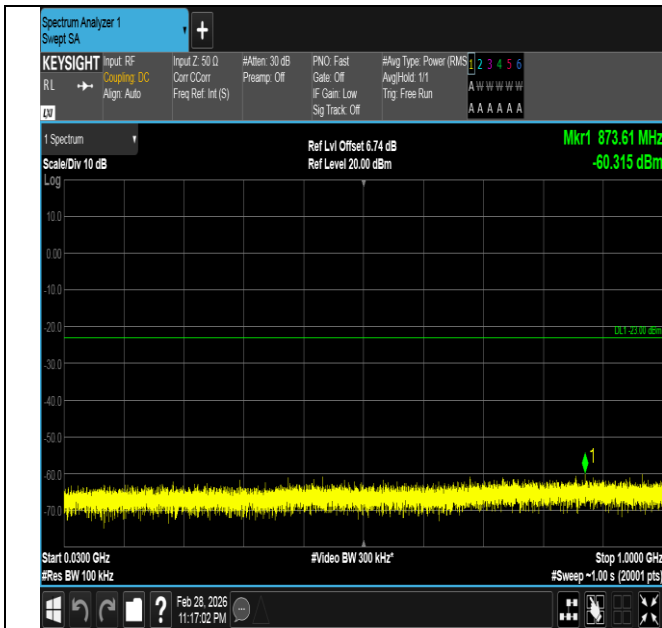
Band66-15MHz-16QAM-132322-1RB#74-30~1000-PASS
