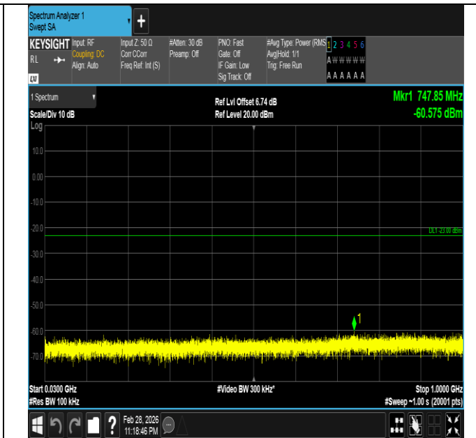
Band66-15MHz-16QAM-132597-1RB#0-30~1000-PASS
