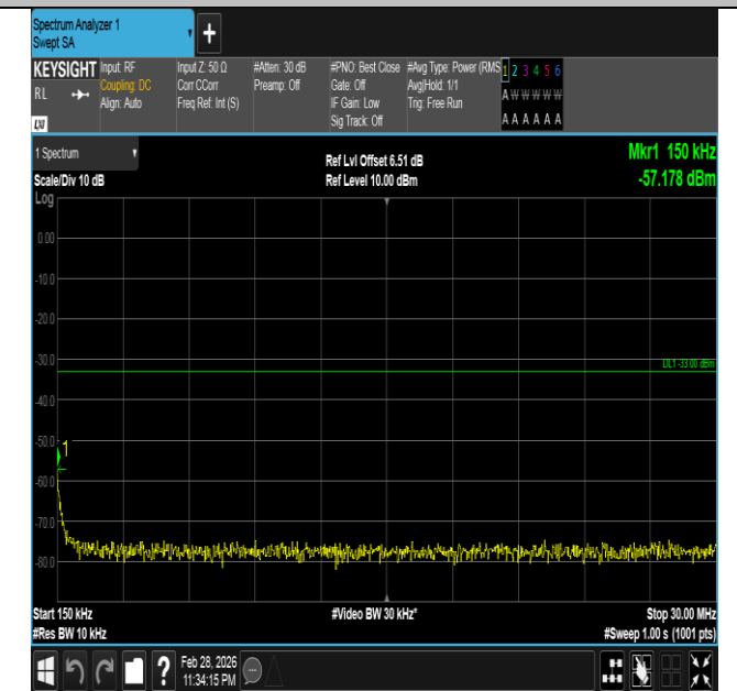
Band66-20MHz-QPSK-132072-1RB#0-0.15~30-PASS
