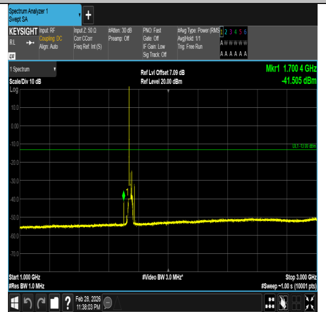
Band66-20MHz-QPSK-132322-1RB#0-1000~3000-PASS
