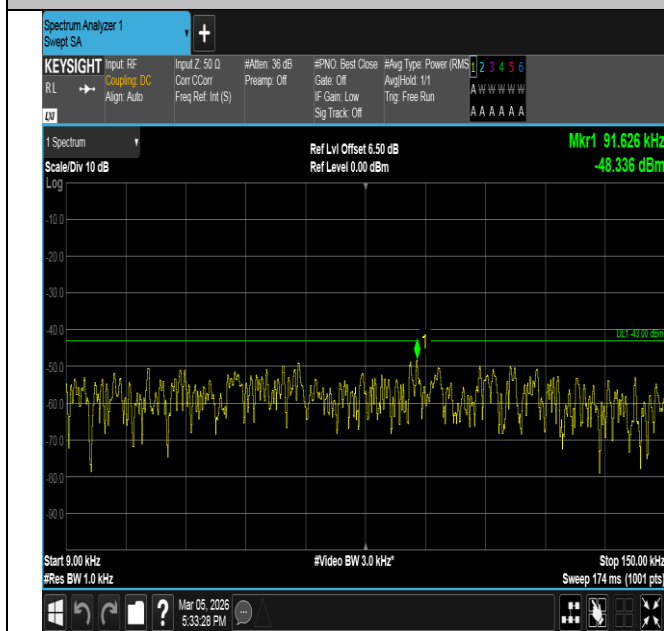
Band66-15MHz-QPSK-132597-75RB#0-0.009~0.15-PASS
