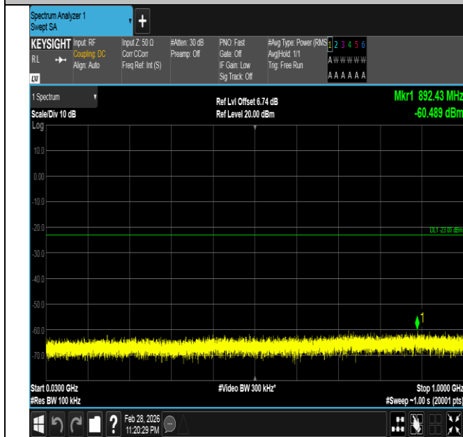
Band66-15MHz-16QAM-132597-1RB#74-30~1000-PASS
