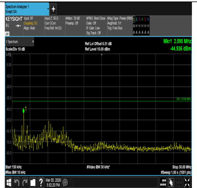
Band66-20MHz-QPSK-132072-100RB#0-0.15~30-PASS
