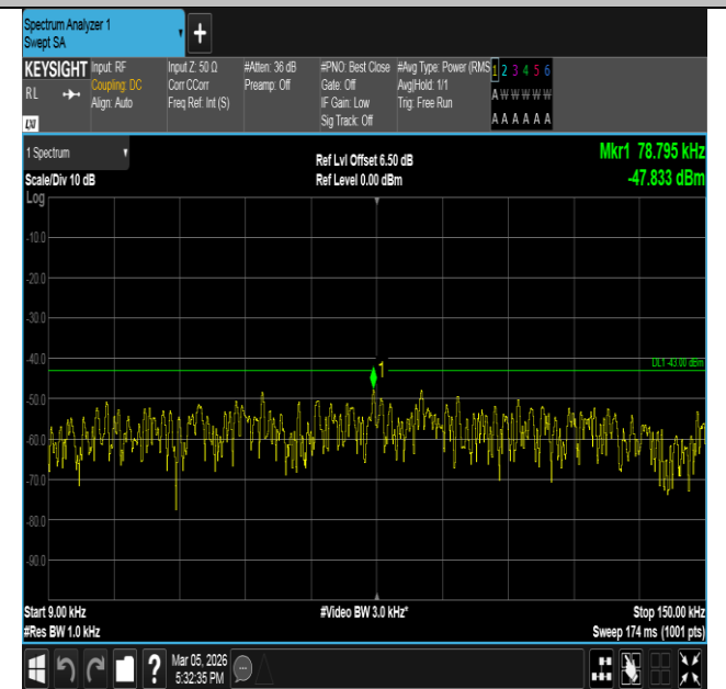
Band66-15MHz-16QAM-132322-75RB#0-0.009~0.15-PASS
