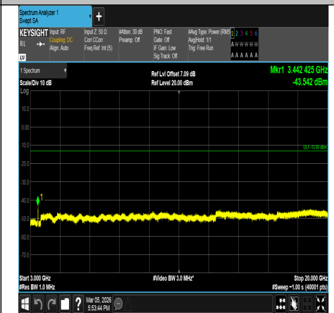
Band66-20MHz-16QAM-132072-100RB#0-3000~20000-PASS
