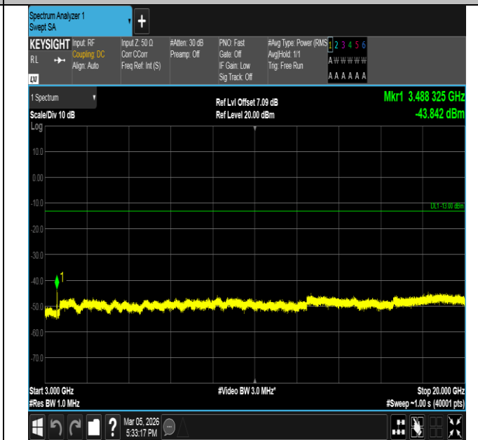
Band66-15MHz-16QAM-132322-75RB#0-3000~20000-PASS
