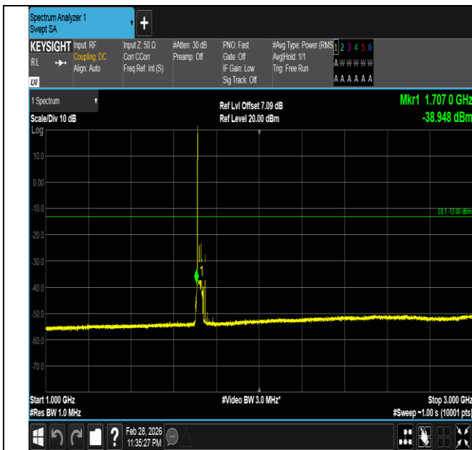
Band66-20MHz-16QAM-132072-1RB#0-1000~3000-PASS
