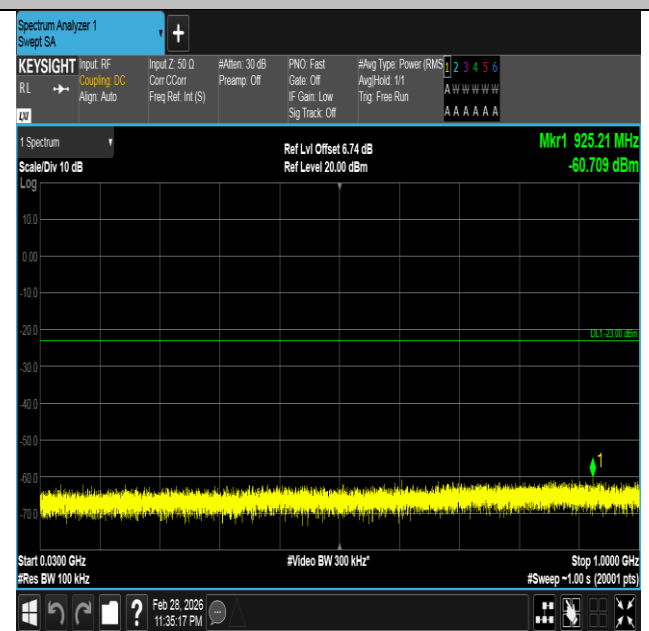
Band66-20MHz-16QAM-132072-1RB#0-30~1000-PASS
