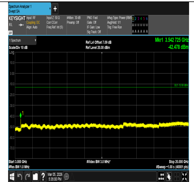
Band66-15MHz-16QAM-132597-75RB#0-3000~20000-PASS
