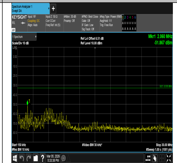
Band66-15MHz-QPSK-132597-75RB#0-0.15~30-PASS
