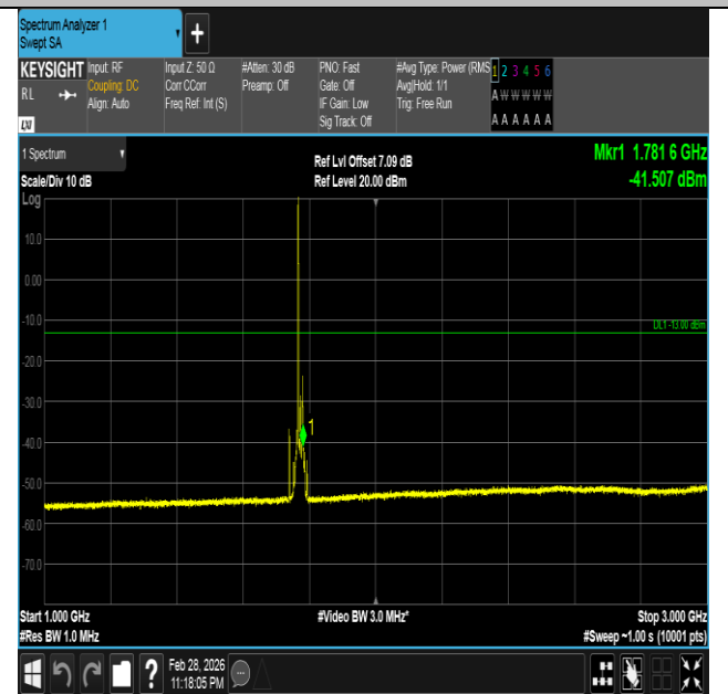
Band66-15MHz-QPSK-132597-1RB#0-1000~3000-PASS
