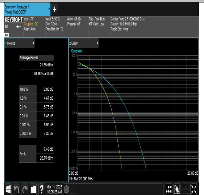
Band7-20MHz-16QAM-20850-100RB#0-PASS
