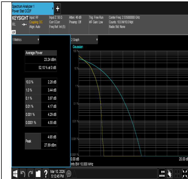
Band7-10MHz-QPSK-21100-1RB#0-PASS
