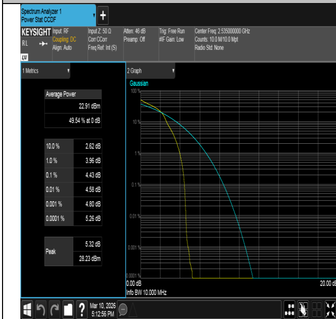
Band7-10MHz-16QAM-21100-1RB#0-PASS
