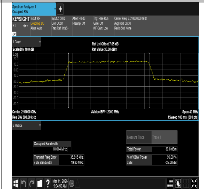
Band7-20MHz-16QAM-20850-100RB#0-PASS
