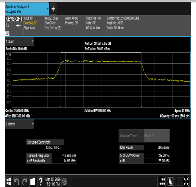
Band7-15MHz-16QAM-21100-75RB#0-PASS
