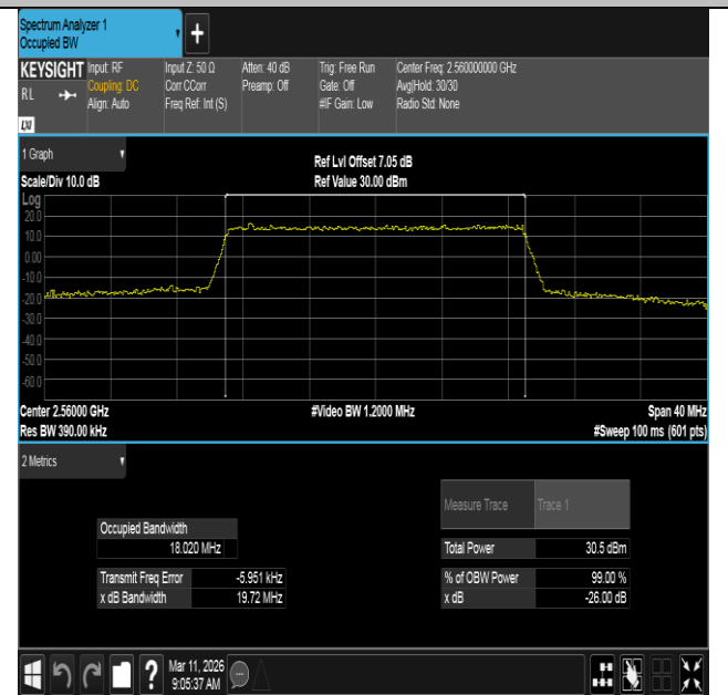
Band7-20MHz-16QAM-21350-100RB#0-PASS
