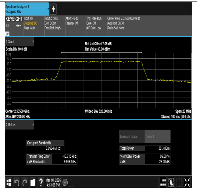
Band7-10MHz-16QAM-21100-50RB#0-PASS
