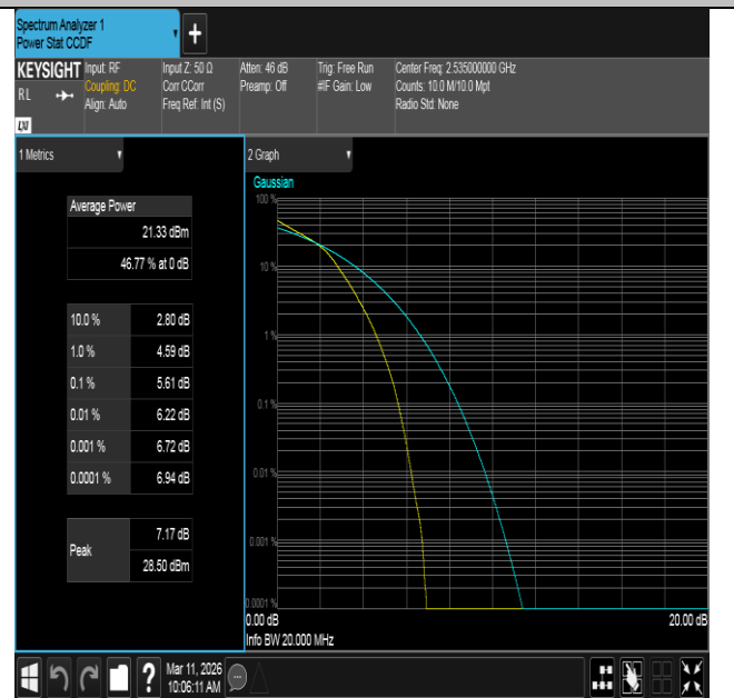
Band7-20MHz-16QAM-21100-100RB#0-PASS
