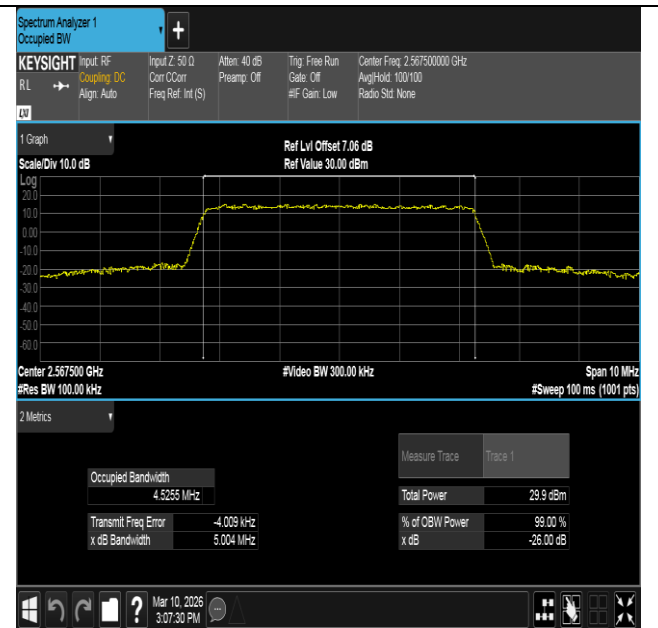
Band7-5MHz-16QAM-21425-25RB#0-PASS
