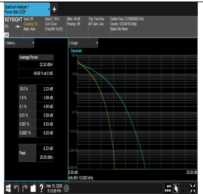
Band7-10MHz-QPSK-21100-50RB#0-PASS
