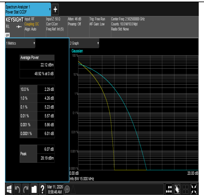
Band7-15MHz-QPSK-21375-75RB#0-PASS
