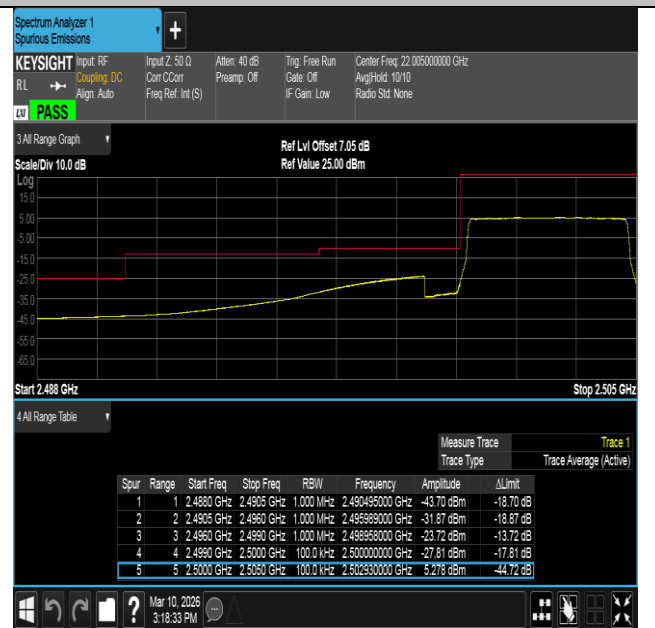
Band7-5MHz-16QAM-20775-25RB#0-PASS
