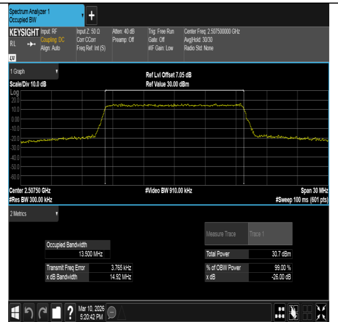
Band7-15MHz-16QAM-20825-75RB#0-PASS
