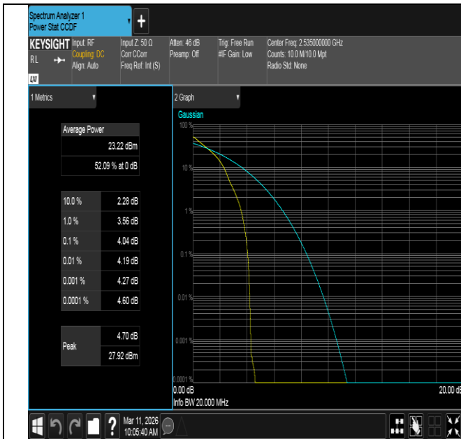
Band7-20MHz-QPSK-21100-1RB#0-PASS
