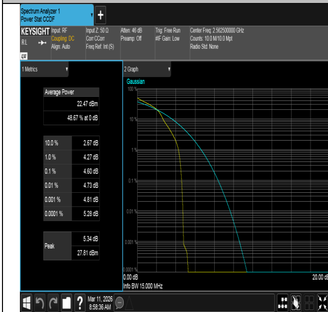
Band7-15MHz-16QAM-21375-1RB#0-PASS
