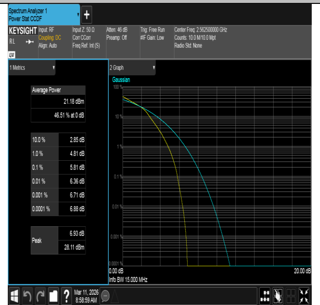
Band7-15MHz-16QAM-21375-75RB#0-PASS
