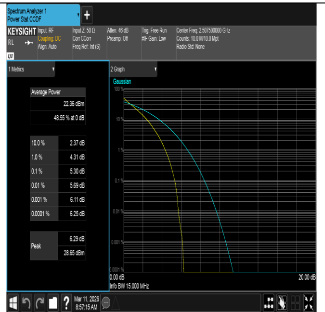
Band7-15MHz-QPSK-20825-75RB#0-PASS
