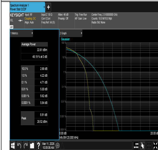
Band7-20MHz-16QAM-20850-1RB#0-PASS
