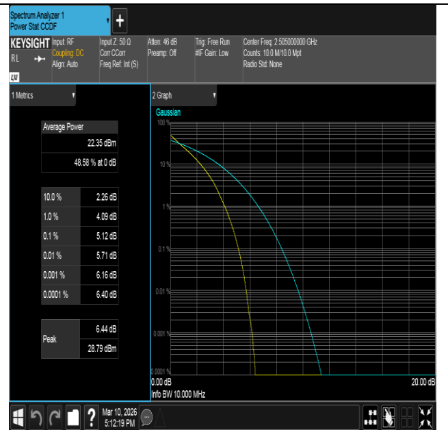
Band7-10MHz-QPSK-20800-50RB#0-PASS
