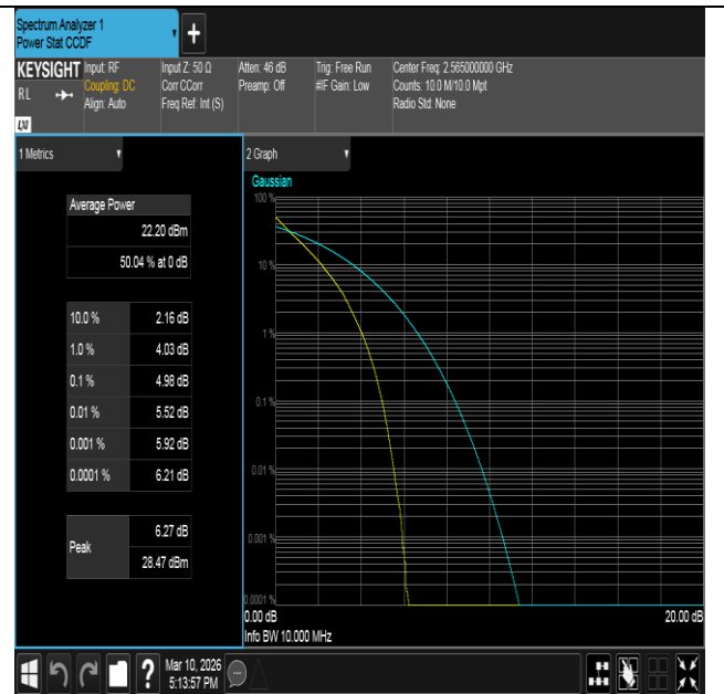
Band7-10MHz-QPSK-21400-50RB#0-PASS
