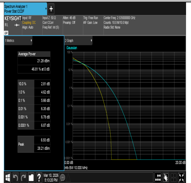
Band7-10MHz-16QAM-21100-50RB#0-PASS
