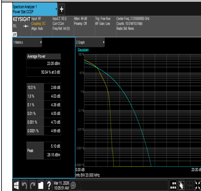
Band7-20MHz-16QAM-21100-1RB#0-PASS
