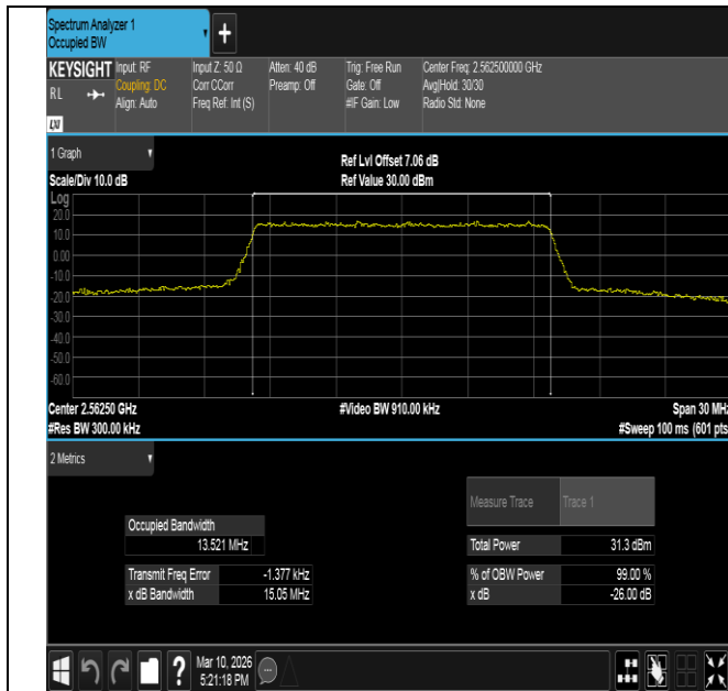
Band7-15MHz-QPSK-21375-75RB#0-PASS
