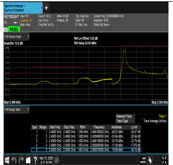
Band7-5MHz-16QAM-20775-1RB#0-PASS
