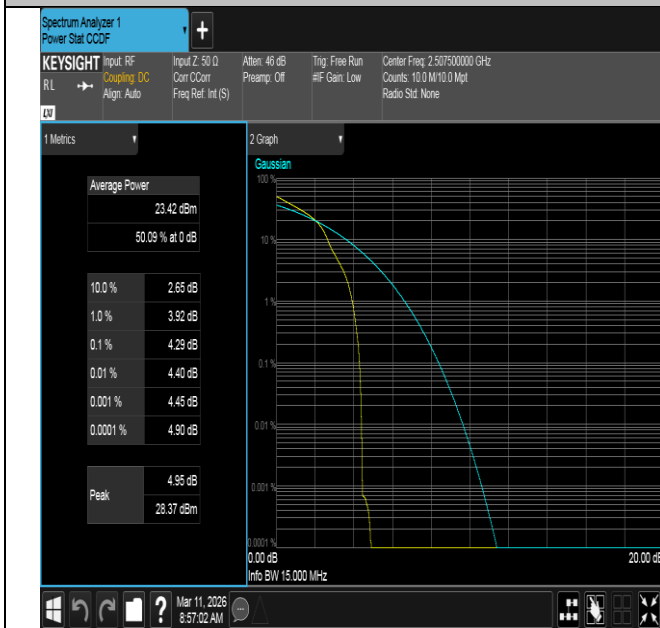
Band7-15MHz-16QAM-20825-1RB#0-PASS
