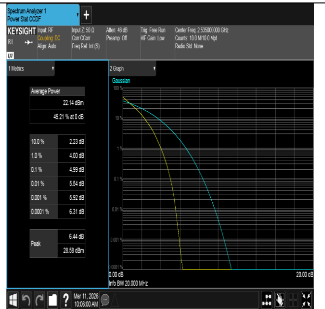
Band7-20MHz-QPSK-21100-100RB#0-PASS
