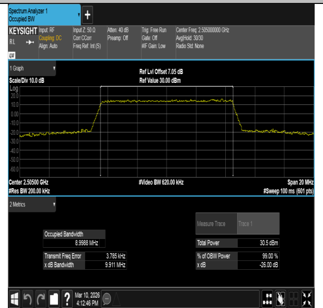
Band7-10MHz-16QAM-20800-50RB#0-PASS
