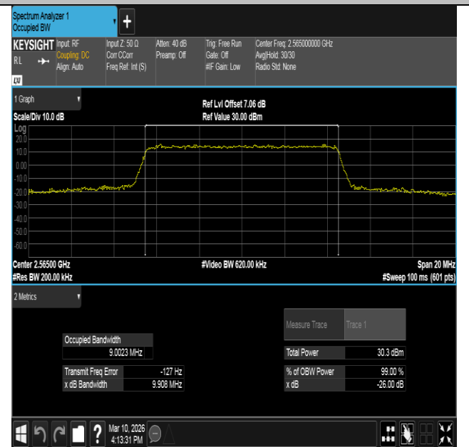
Band7-10MHz-16QAM-21400-50RB#0-PASS
