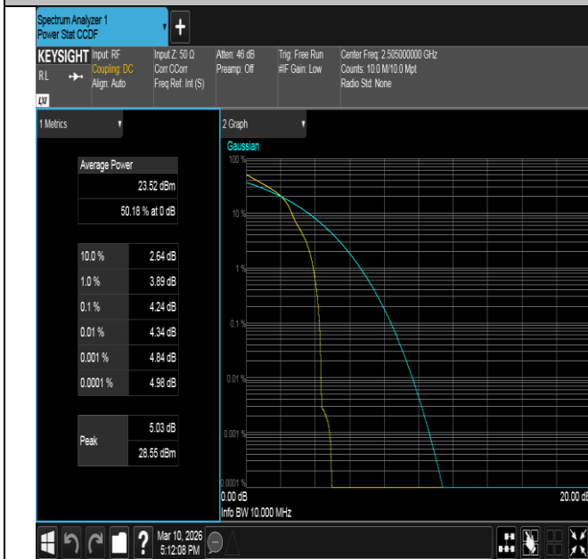
Band7-10MHz-16QAM-20800-1RB#0-PASS
