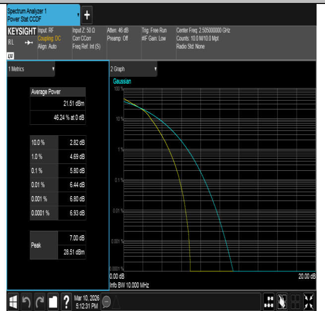
Band7-10MHz-16QAM-20800-50RB#0-PASS
