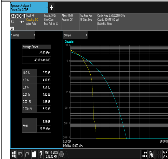
Band7-10MHz-16QAM-21400-1RB#0-PASS
