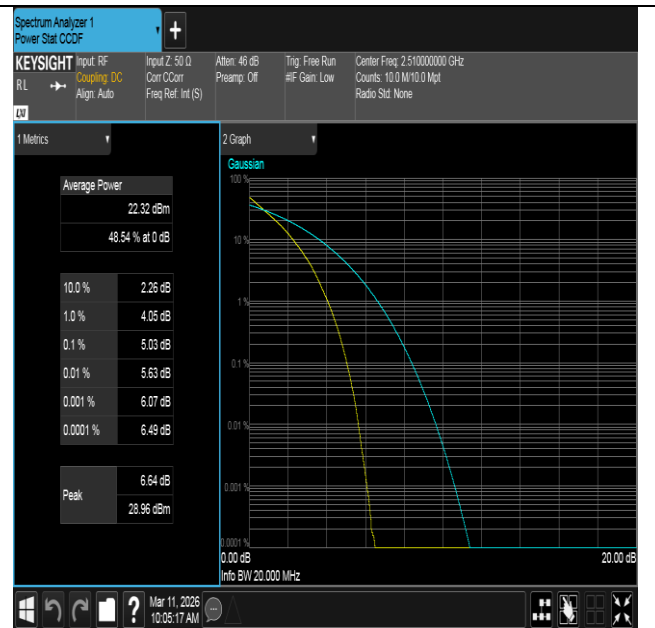
Band7-20MHz-QPSK-20850-100RB#0-PASS
