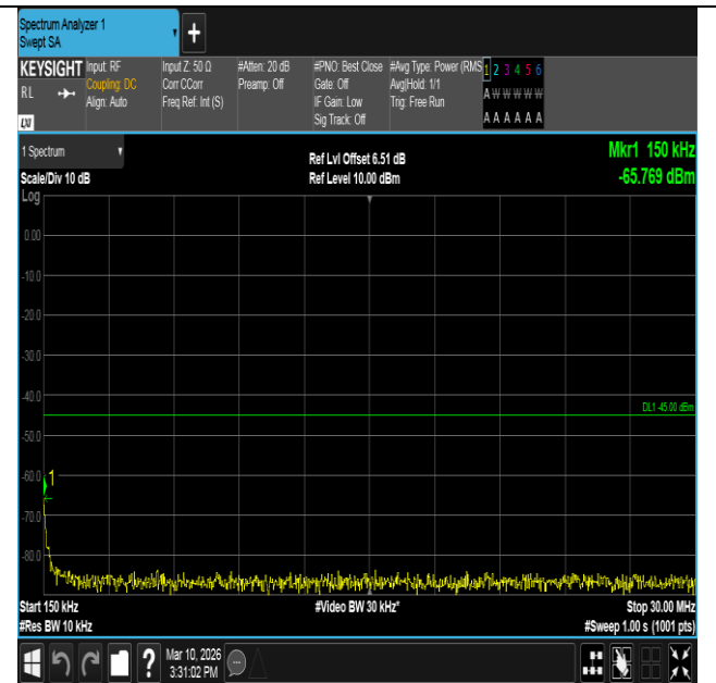
Band7-5MHz-16QAM-20775-1RB#0-0.15~30-PASS
