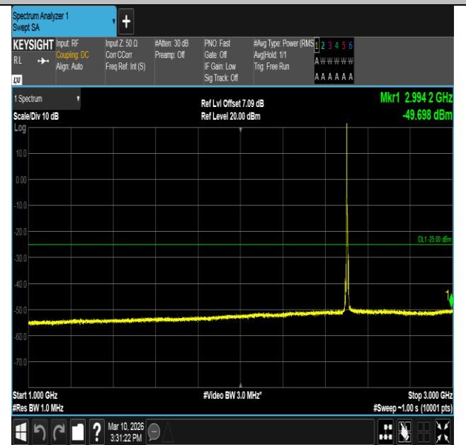
Band7-5MHz-16QAM-20775-1RB#0-1000~3000-PASS
