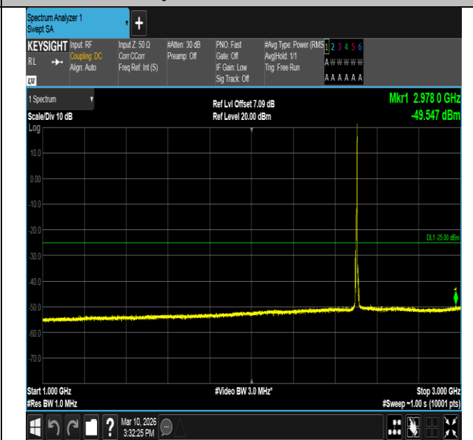
Band7-5MHz-QPSK-20775-1RB#24-1000~3000-PASS
