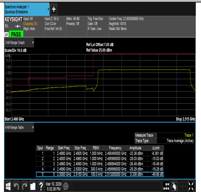
Band7-15MHz-16QAM-20825-75RB#0-PASS
