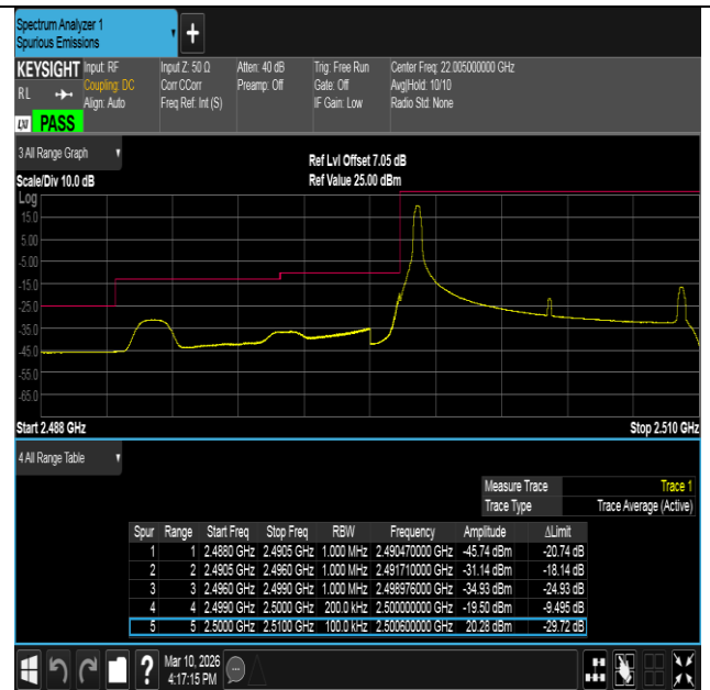
Band7-10MHz-16QAM-20800-1RB#0-PASS
