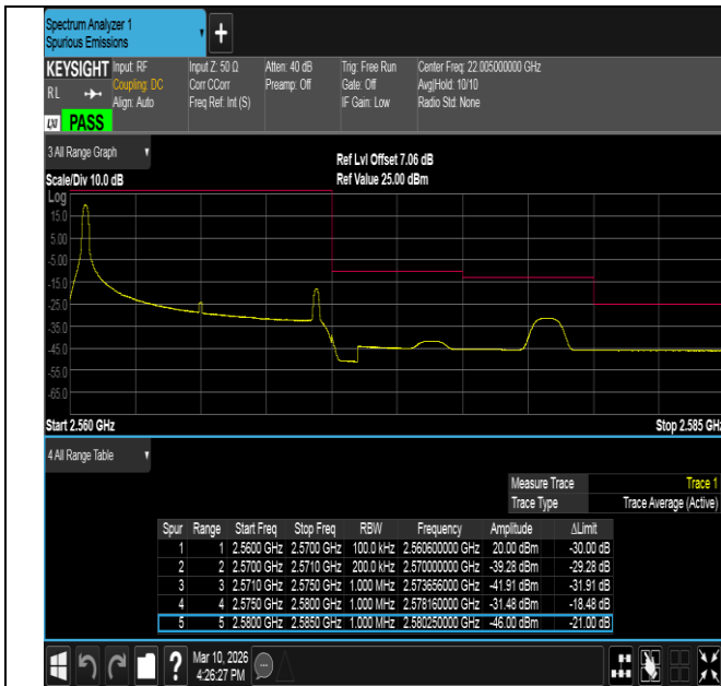
Band7-10MHz-QPSK-21400-1RB#0-PASS
