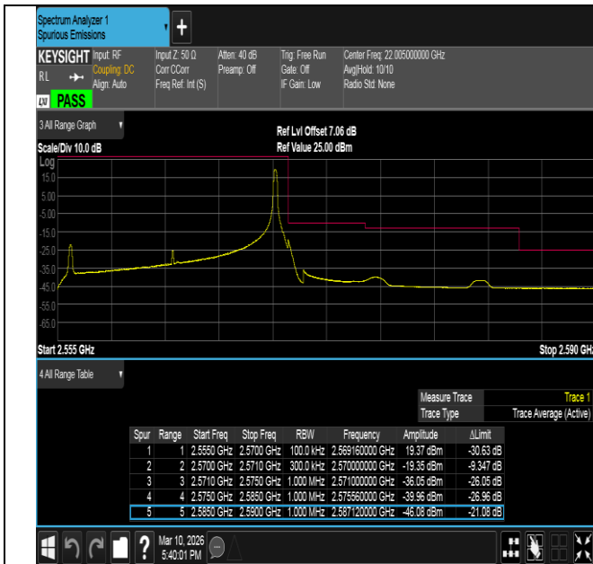
Band7-15MHz-16QAM-21375-1RB#74-PASS
