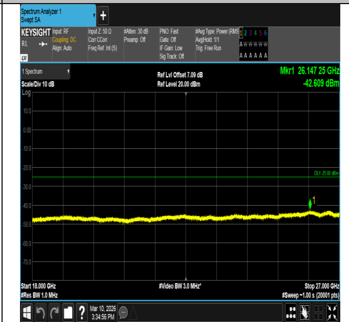
Band7-5MHz-QPSK-20775-25RB#0-18000~27000-PASS
