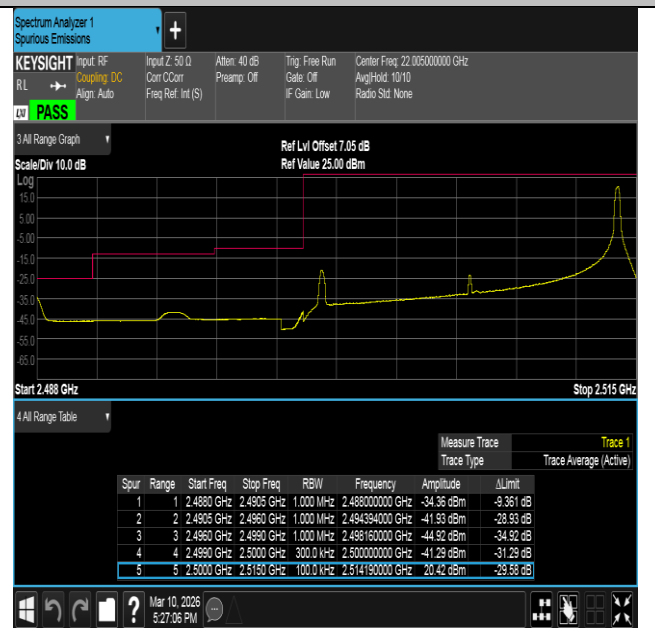
Band7-15MHz-QPSK-20825-1RB#74-PASS
