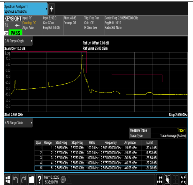
Band7-15MHz-QPSK-21375-1RB#74-PASS
