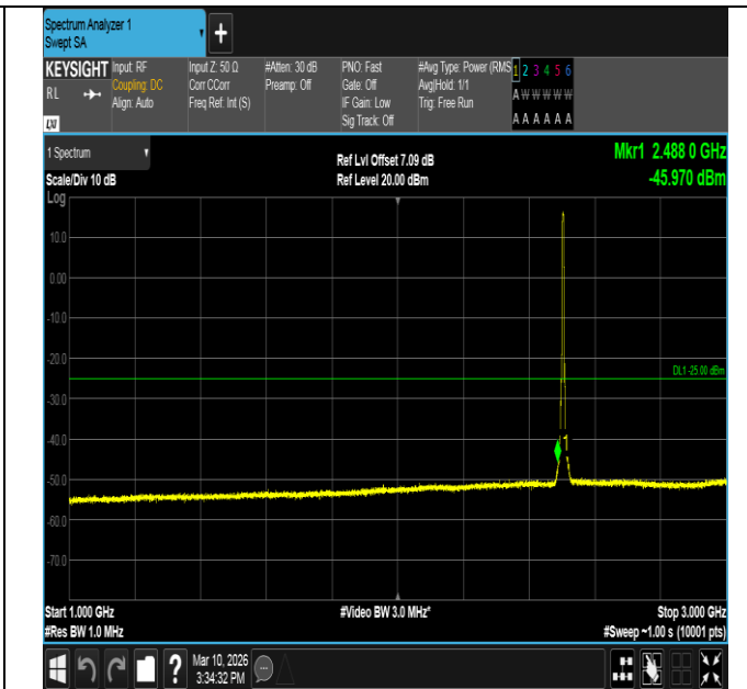
Band7-5MHz-QPSK-20775-25RB#0-1000~3000-PASS
