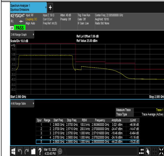
Band7-10MHz-QPSK-21400-50RB#0-PASS
