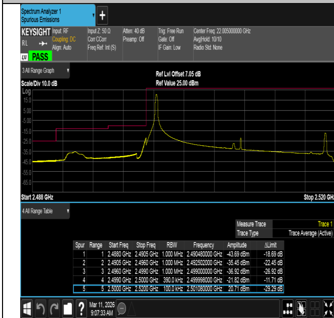
Band7-20MHz-QPSK-20850-1RB#0-PASS
