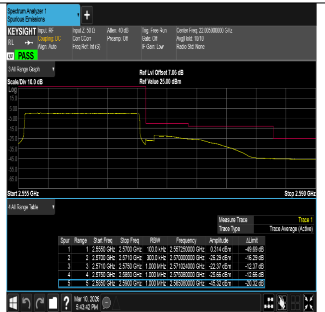
Band7-15MHz-16QAM-21375-75RB#0-PASS
