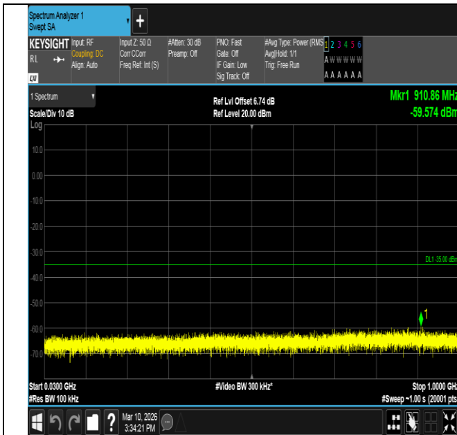
Band7-5MHz-QPSK-20775-25RB#0-30~1000-PASS
