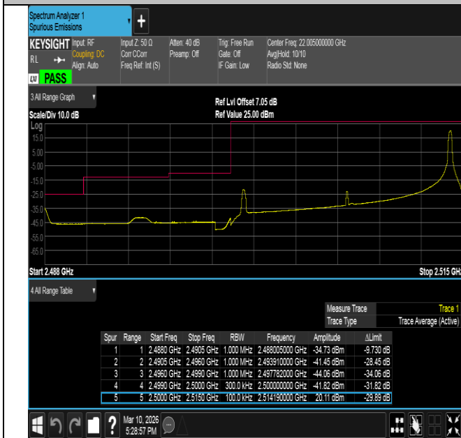
Band7-15MHz-16QAM-20825-1RB#74-PASS
