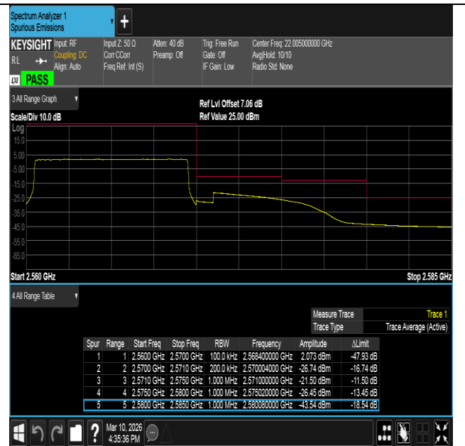
Band7-10MHz-16QAM-21400-50RB#0-PASS
