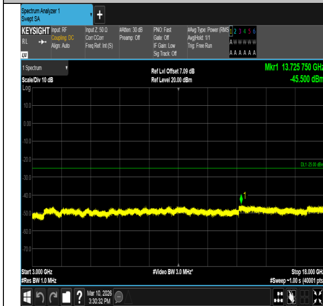
Band7-5MHz-QPSK-20775-1RB#0-3000~18000-PASS
