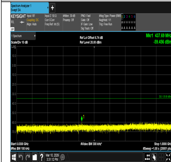
Band7-5MHz-16QAM-20775-1RB#0-30~1000-PASS
