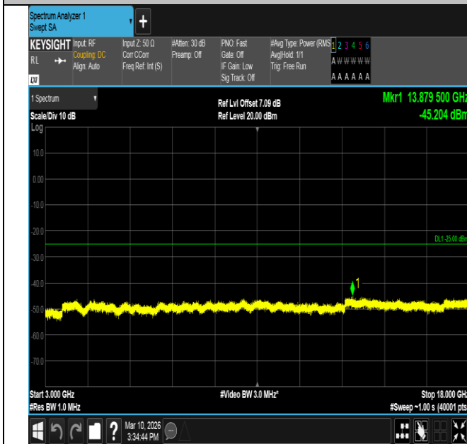
Band7-5MHz-QPSK-20775-25RB#0-3000~18000-PASS
