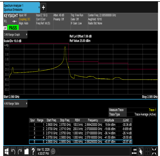
Band7-10MHz-QPSK-21400-1RB#49-PASS
