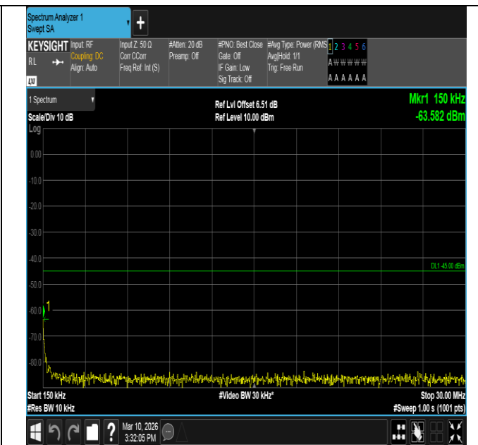
Band7-5MHz-QPSK-20775-1RB#24-0.15~30-PASS
