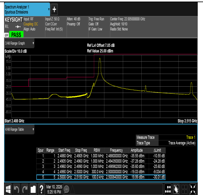
Band7-15MHz-16QAM-20825-1RB#0-PASS
