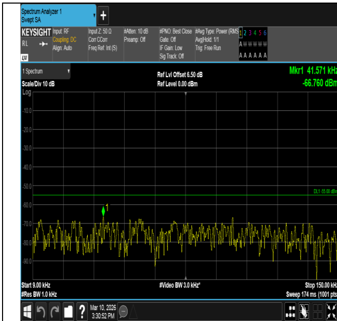
Band7-5MHz-16QAM-20775-1RB#0-0.009~0.15-PASS
