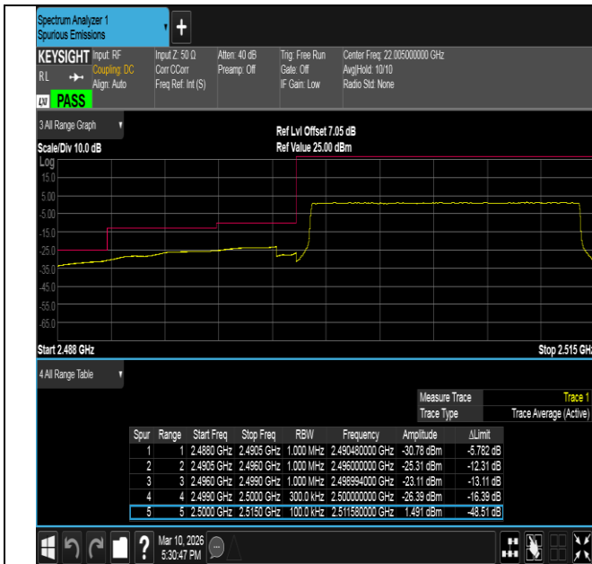
Band7-15MHz-QPSK-20825-75RB#0-PASS
