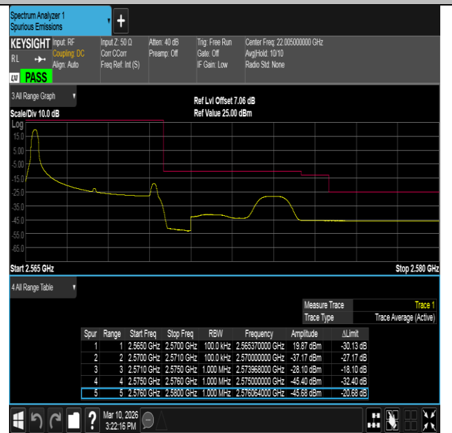
Band7-5MHz-16QAM-21425-1RB#0-PASS
