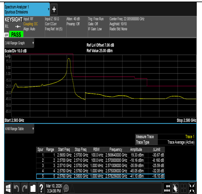
Band7-5MHz-QPSK-21425-1RB#24-PASS
