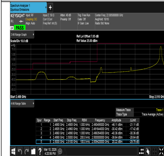
Band7-10MHz-16QAM-20800-1RB#49-PASS
