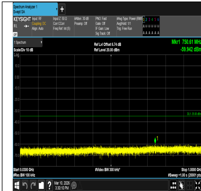
Band7-5MHz-QPSK-20775-1RB#0-30~1000-PASS
