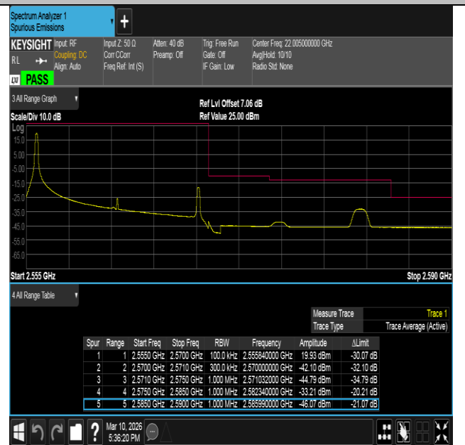
Band7-15MHz-16QAM-21375-1RB#0-PASS
