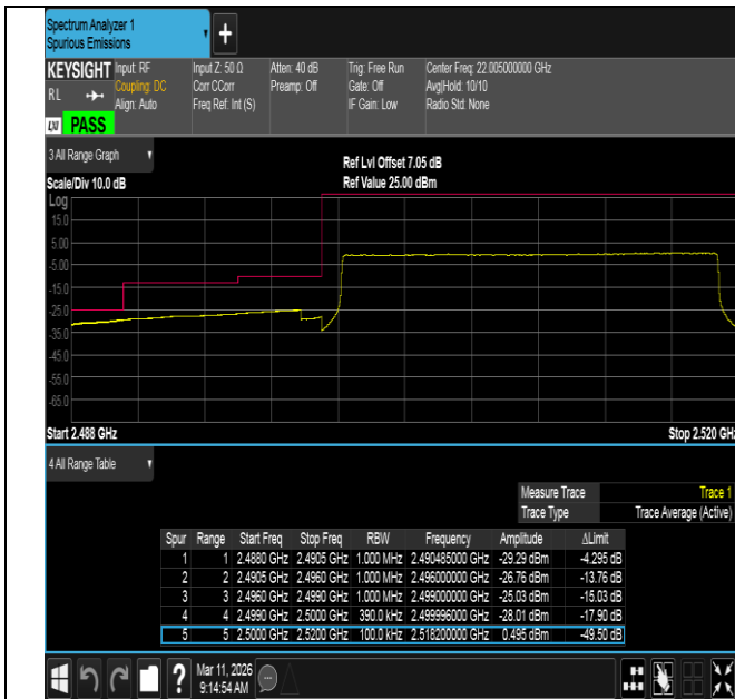
Band7-20MHz-QPSK-20850-100RB#0-PASS
