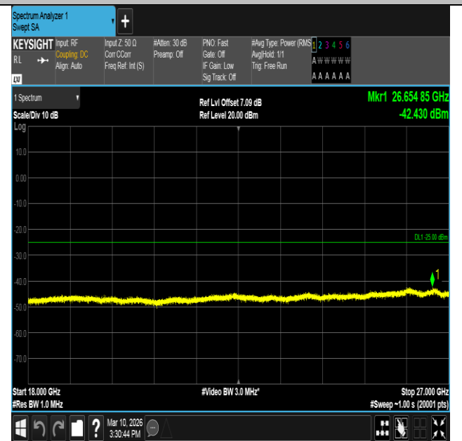
Band7-5MHz-QPSK-20775-1RB#0-18000~27000-PASS
