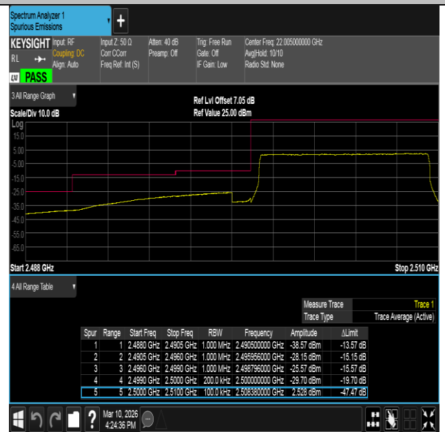
Band7-10MHz-16QAM-20800-50RB#0-PASS
