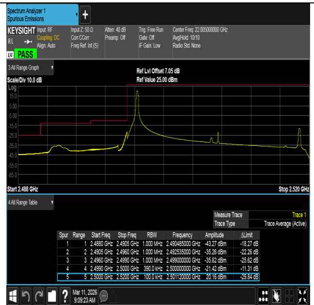
Band7-20MHz-16QAM-20850-1RB#0-PASS
