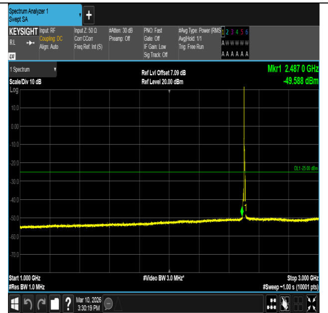
Band7-5MHz-QPSK-20775-1RB#0-1000~3000-PASS
