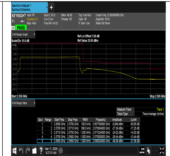
Band7-20MHz-16QAM-21350-100RB#0-PASS
