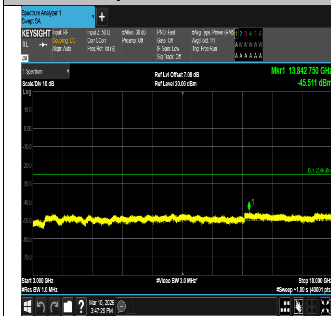
Band7-5MHz-QPSK-21425-25RB#0-3000~18000-PASS
