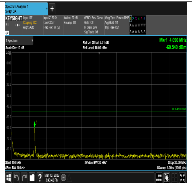
Band7-5MHz-16QAM-21425-1RB#0-0.15~30-PASS
