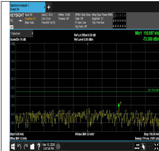
Band7-5MHz-16QAM-21425-25RB#0-0.009~0.15-PASS
