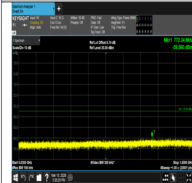
Band7-5MHz-16QAM-20775-25RB#0-30~1000-PASS
