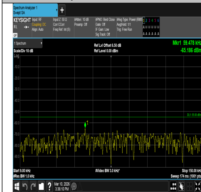
Band7-5MHz-QPSK-21100-1RB#0-0.009~0.15-PASS
