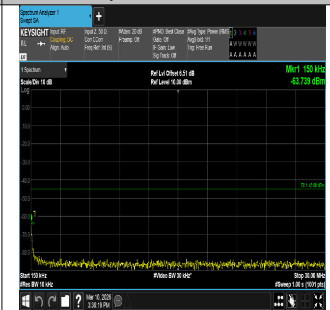
Band7-5MHz-QPSK-21100-1RB#0-0.15~30-PASS
