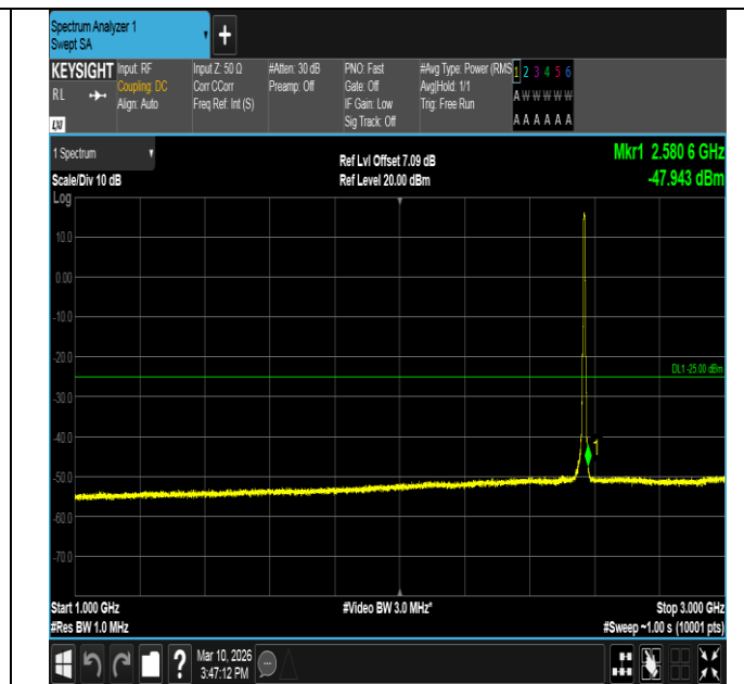
Band7-5MHz-QPSK-21425-25RB#0-1000~3000-PASS
