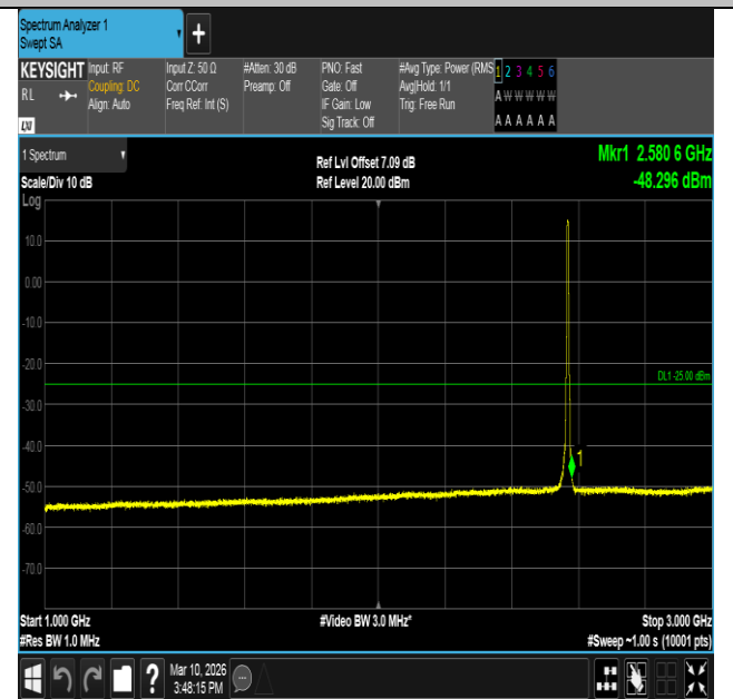
Band7-5MHz-16QAM-21425-25RB#0-1000~3000-PASS
