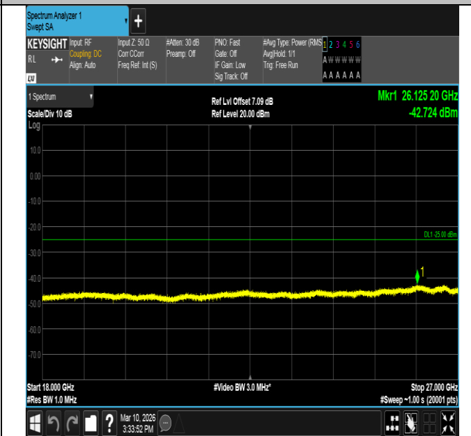
Band7-5MHz-16QAM-20775-1RB#24-18000~27000-PASS
