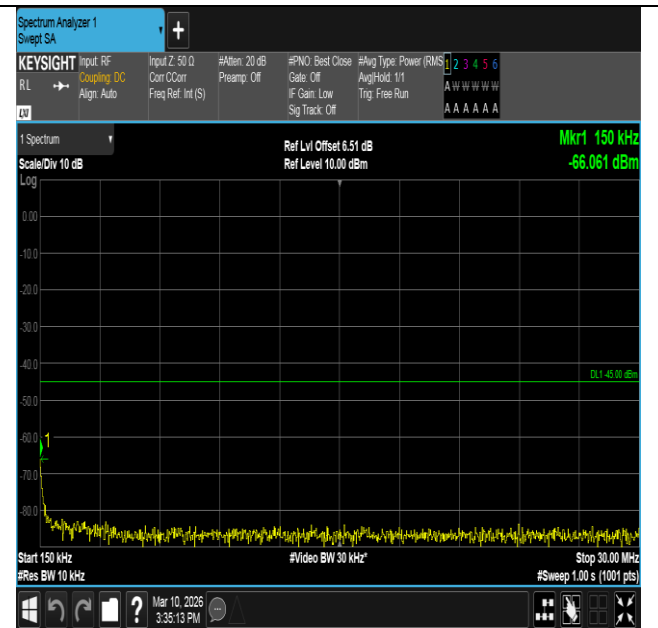
Band7-5MHz-16QAM-20775-25RB#0-0.15~30-PASS
