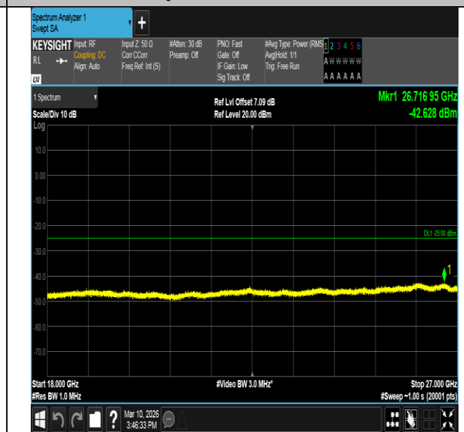
Band7-5MHz-16QAM-21425-1RB#24-18000~27000-PASS
