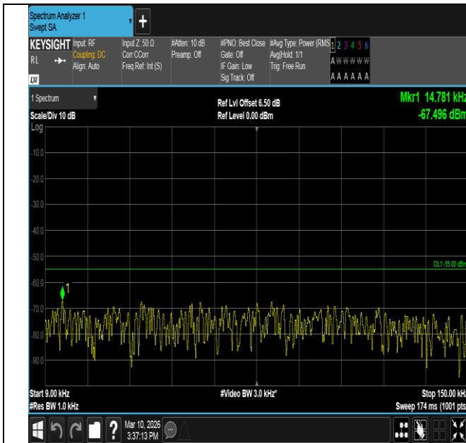
Band7-5MHz-16QAM-21100-1RB#0-0.009~0.15-PASS
