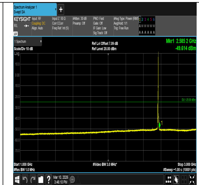
Band7-5MHz-16QAM-21425-1RB#24-1000~3000-PASS
