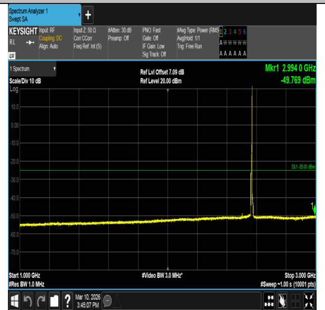
Band7-5MHz-QPSK-21425-1RB#24-1000~3000-PASS
