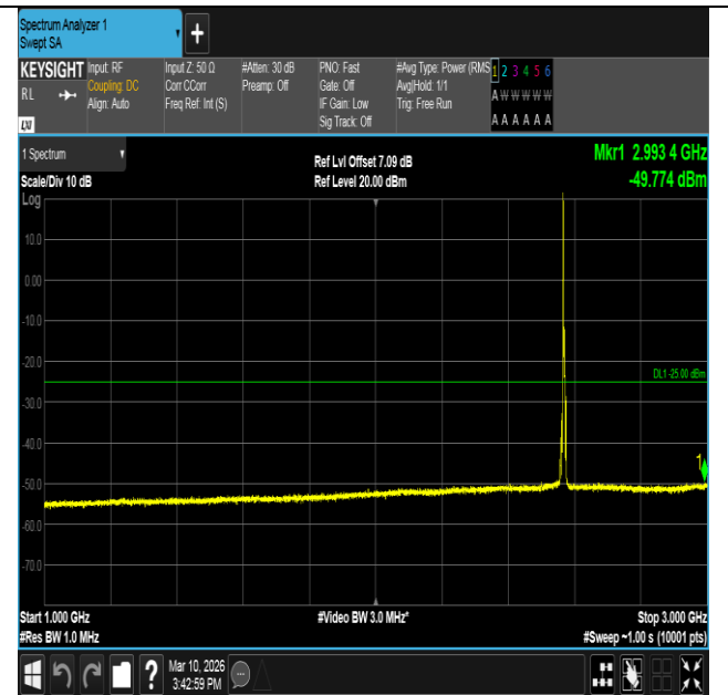
Band7-5MHz-QPSK-21425-1RB#0-1000~3000-PASS
