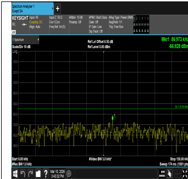
Band7-5MHz-16QAM-21425-1RB#0-0.009~0.15-PASS
