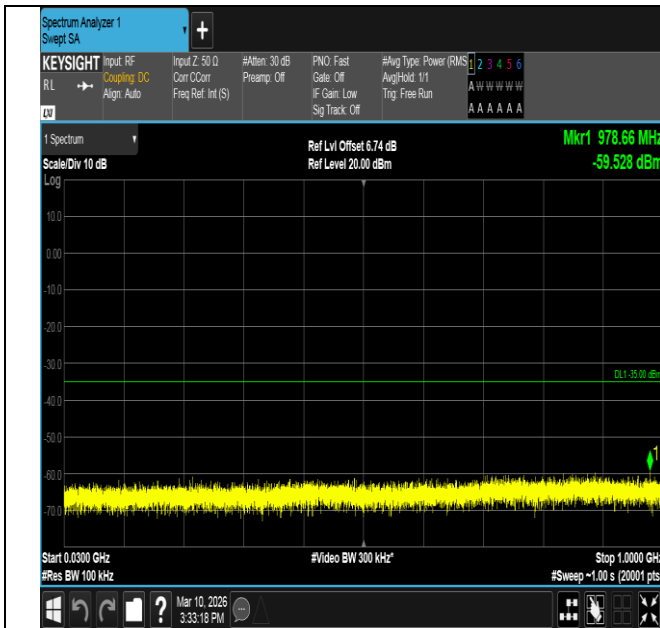
Band7-5MHz-16QAM-20775-1RB#24-30~1000-PASS
