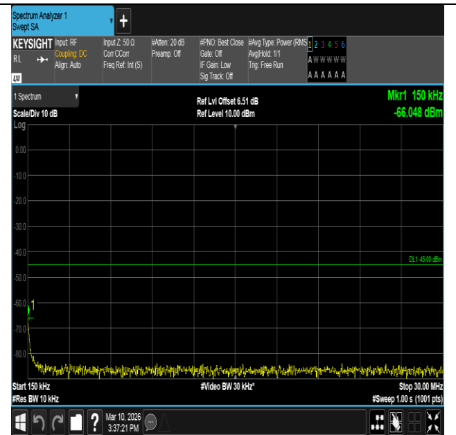
Band7-5MHz-16QAM-21100-1RB#0-0.15~30-PASS
