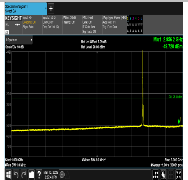
Band7-5MHz-16QAM-21100-1RB#0-1000~3000-PASS
