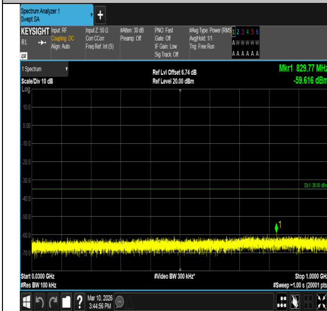
Band7-5MHz-QPSK-21425-1RB#24-30~1000-PASS
