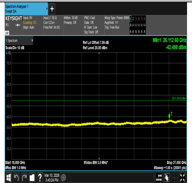
Band7-5MHz-QPSK-21425-1RB#0-18000~27000-PASS
