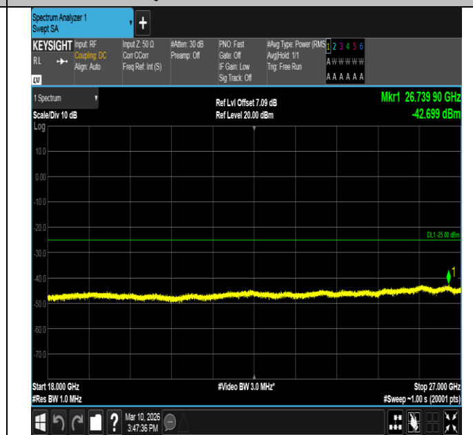
Band7-5MHz-QPSK-21425-25RB#0-18000~27000-PASS
