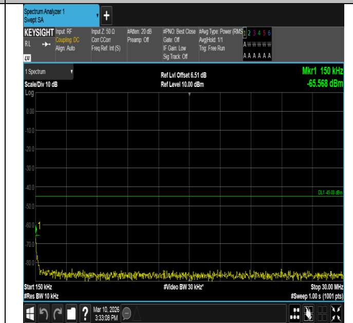
Band7-5MHz-16QAM-20775-1RB#24-0.15~30-PASS
