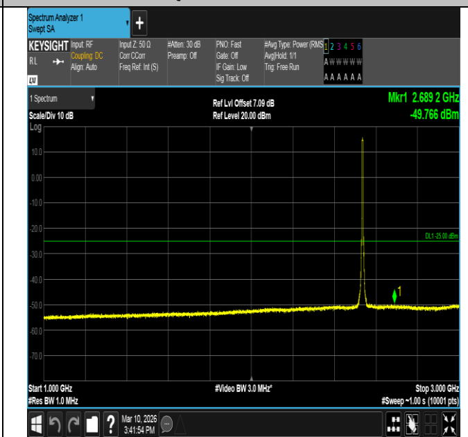
Band7-5MHz-16QAM-21100-25RB#0-1000~3000-PASS
