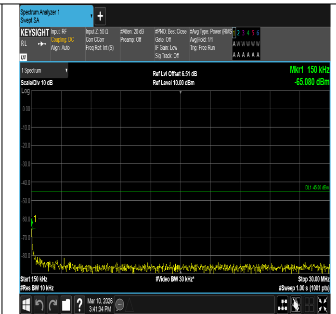
Band7-5MHz-16QAM-21100-25RB#0-0.15~30-PASS
