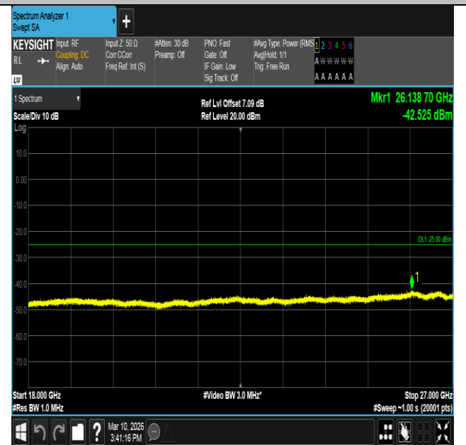
Band7-5MHz-QPSK-21100-25RB#0-18000~27000-PASS
