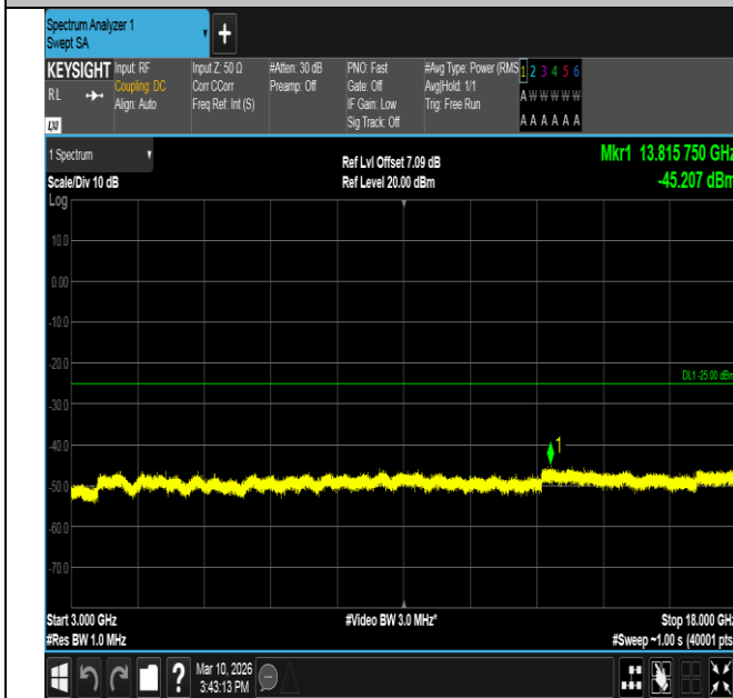
Band7-5MHz-QPSK-21425-1RB#0-3000~18000-PASS
