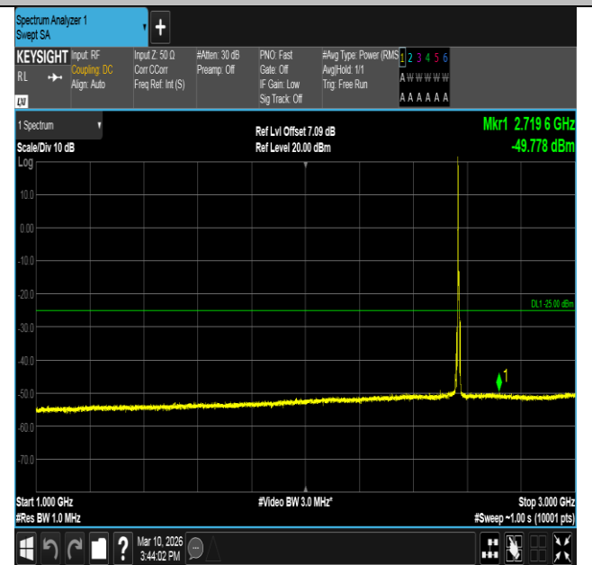
Band7-5MHz-16QAM-21425-1RB#0-1000~3000-PASS
