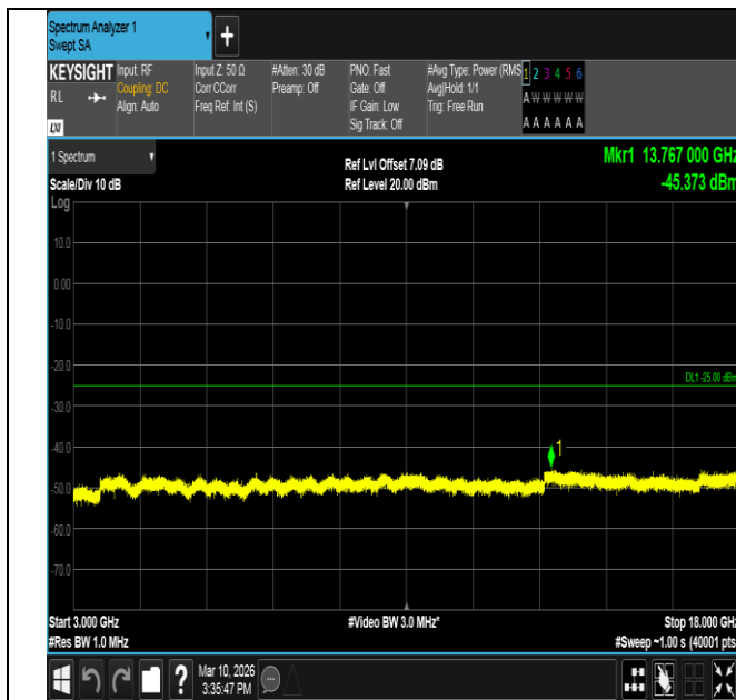
Band7-5MHz-16QAM-20775-25RB#0-3000~18000-PASS
