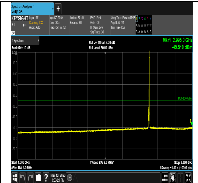
Band7-5MHz-16QAM-20775-1RB#24-1000~3000-PASS
