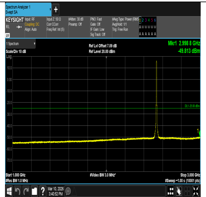
Band7-5MHz-QPSK-21100-25RB#0-1000~3000-PASS
