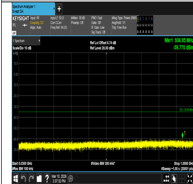
Band7-5MHz-16QAM-21100-1RB#0-30~1000-PASS
