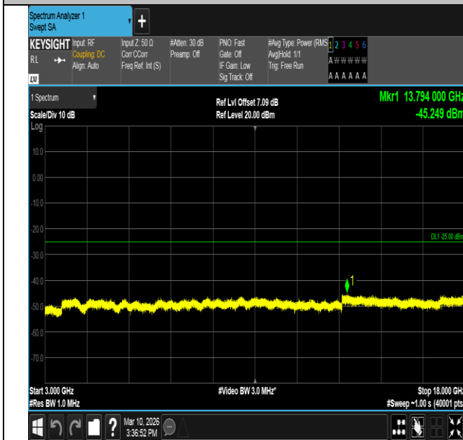
Band7-5MHz-QPSK-21100-1RB#0-3000~18000-PASS
