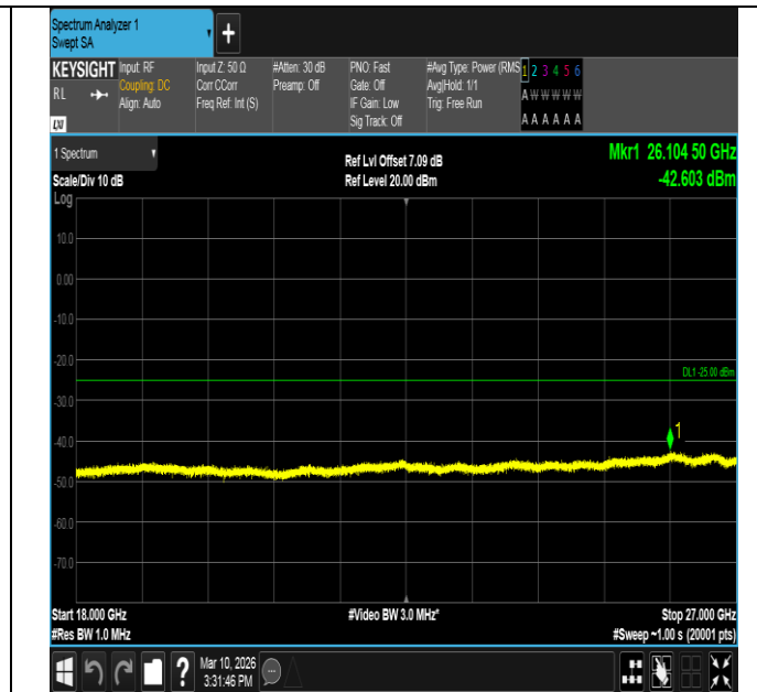
Band7-5MHz-16QAM-20775-1RB#0-18000~27000-PASS
