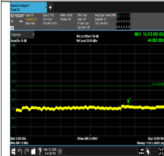
Band7-5MHz-QPSK-21100-25RB#0-3000~18000-PASS
