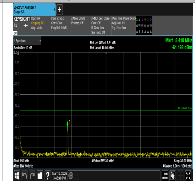
Band7-5MHz-16QAM-21425-1RB#24-0.15~30-PASS
