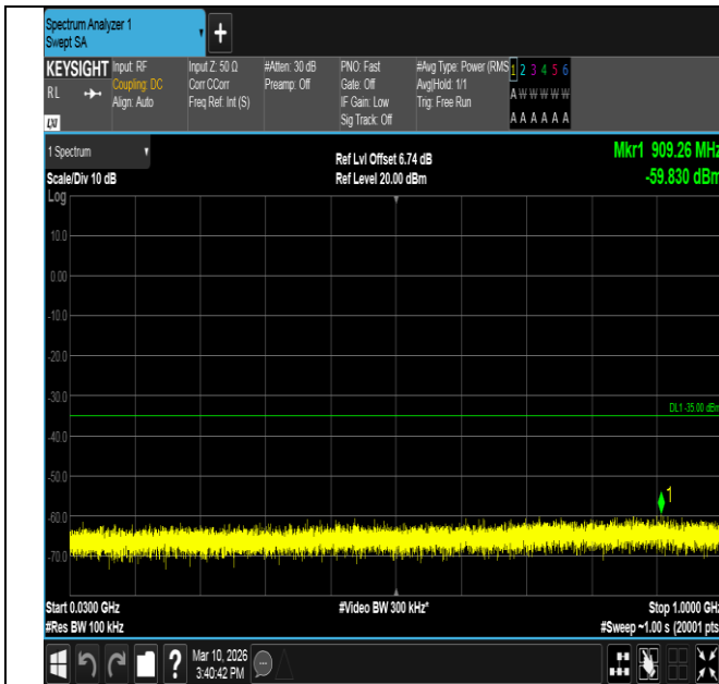
Band7-5MHz-QPSK-21100-25RB#0-30~1000-PASS
