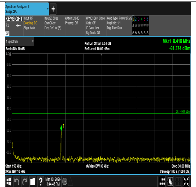
Band7-5MHz-QPSK-21425-1RB#24-0.15~30-PASS
