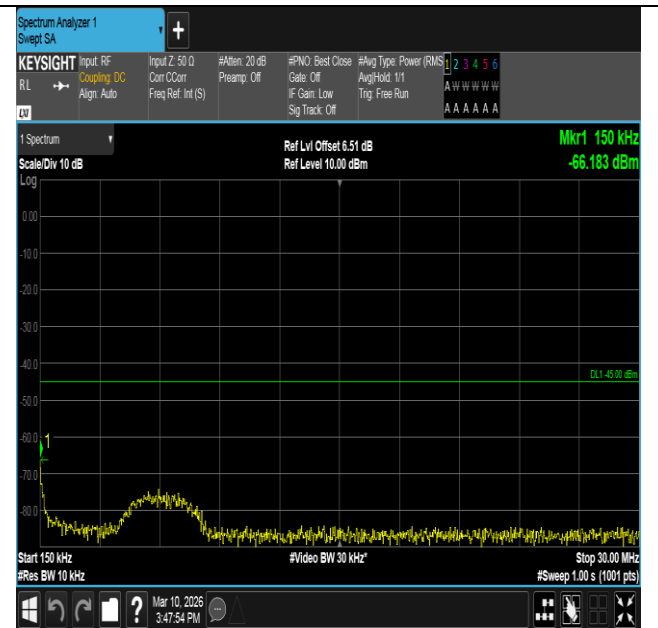
Band7-5MHz-16QAM-21425-25RB#0-0.15~30-PASS
