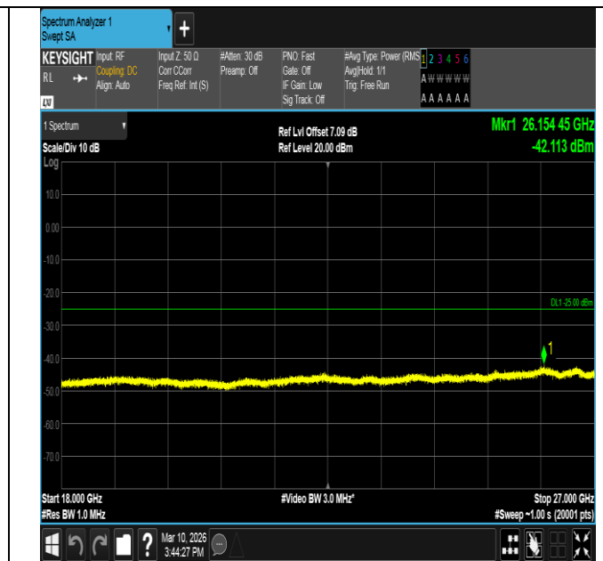
Band7-5MHz-16QAM-21425-1RB#0-18000~27000-PASS
