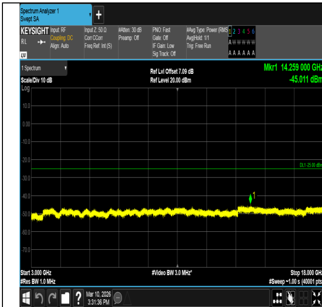
Band7-5MHz-16QAM-20775-1RB#0-3000~18000-PASS
