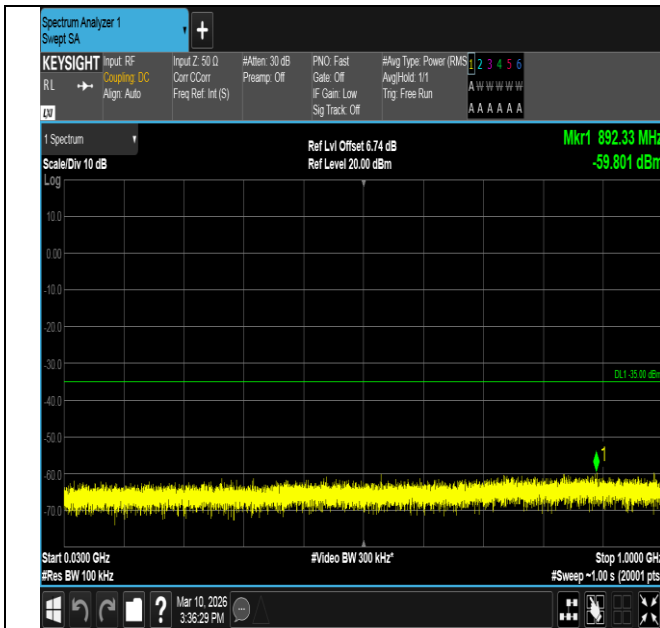
Band7-5MHz-QPSK-21100-1RB#0-30~1000-PASS
