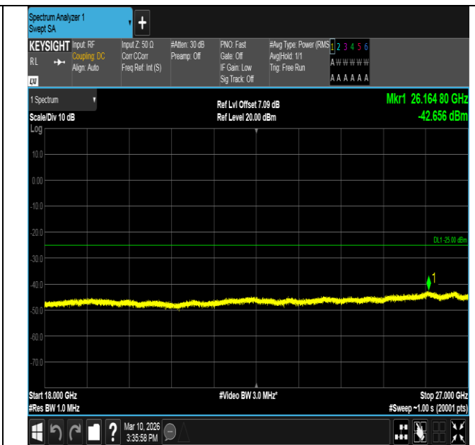
Band7-5MHz-16QAM-20775-25RB#0-18000~27000-PASS
