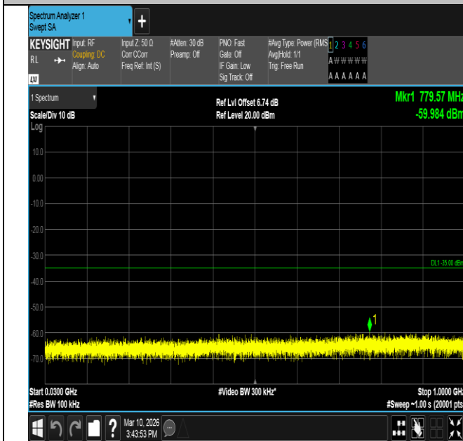
Band7-5MHz-16QAM-21425-1RB#0-30~1000-PASS
