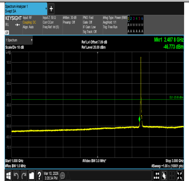
Band7-5MHz-16QAM-20775-25RB#0-1000~3000-PASS
