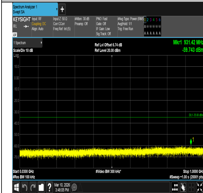
Band7-5MHz-16QAM-21425-25RB#0-30~1000-PASS
