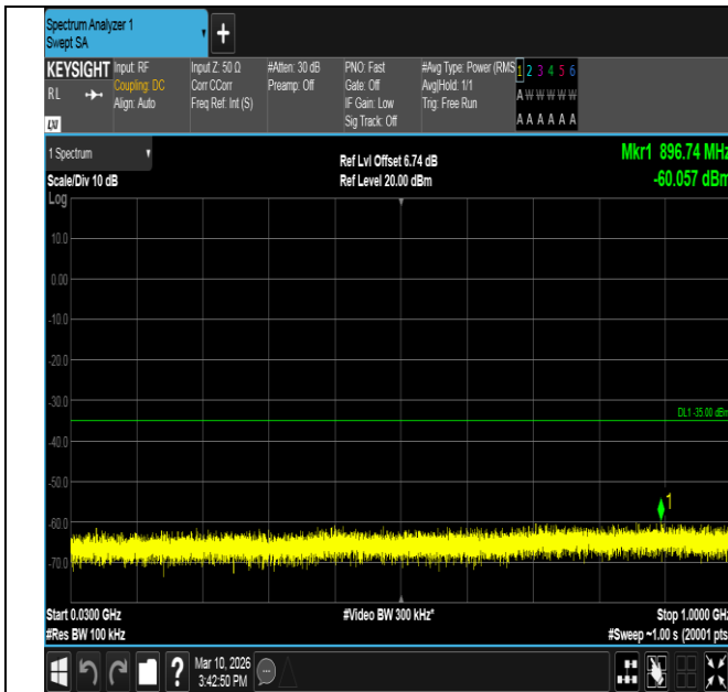
Band7-5MHz-QPSK-21425-1RB#0-30~1000-PASS
