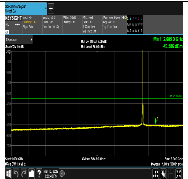
Band7-5MHz-QPSK-21100-1RB#0-1000~3000-PASS
