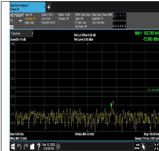
Band7-5MHz-16QAM-20775-25RB#0-0.009~0.15-PASS
