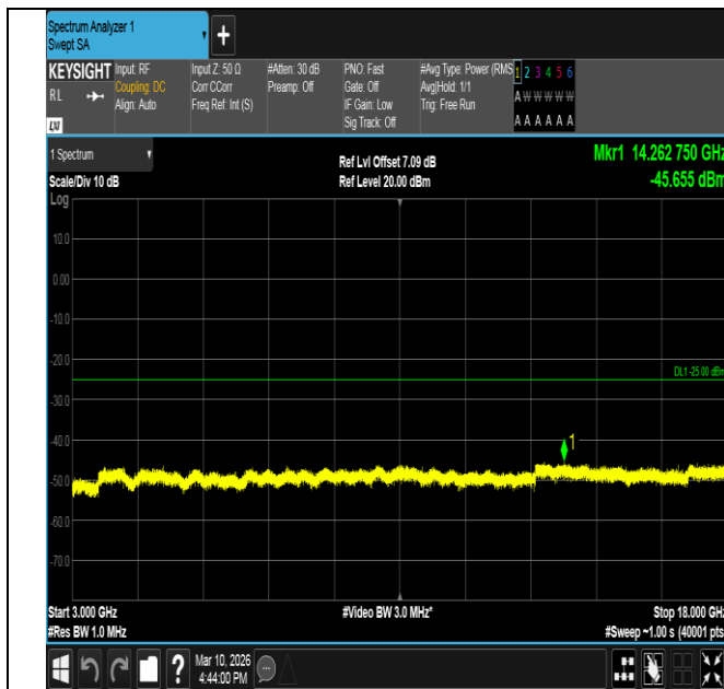
Band7-10MHz-16QAM-21100-1RB#0-3000~18000-PASS
