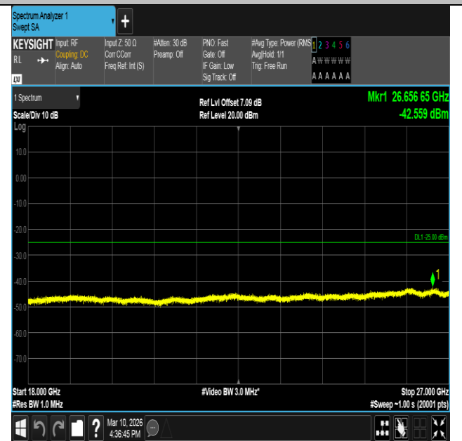
Band7-10MHz-QPSK-20800-1RB#0-18000~27000-PASS
