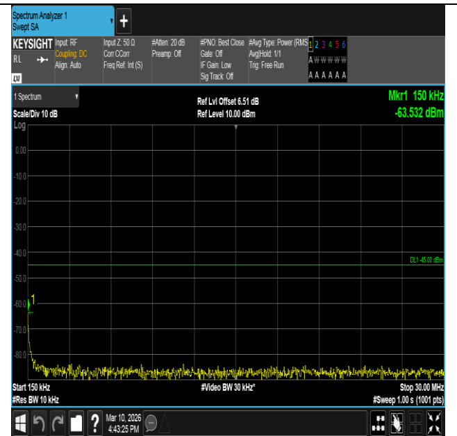
Band7-10MHz-16QAM-21100-1RB#0-0.15~30-PASS
