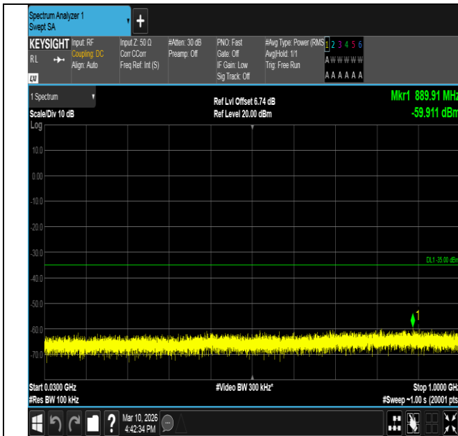
Band7-10MHz-QPSK-21100-1RB#0-30~1000-PASS
