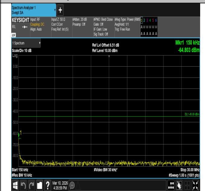
Band7-10MHz-QPSK-20800-1RB#0-0.15~30-PASS
