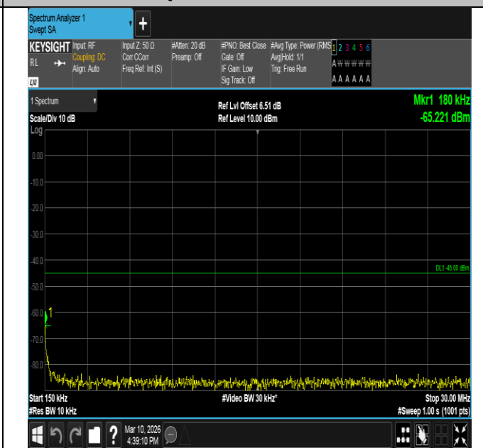
Band7-10MHz-16QAM-20800-1RB#49-0.15~30-PASS
