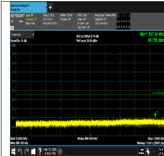
Band7-10MHz-16QAM-20800-1RB#49-30~1000-PASS
