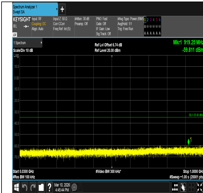
Band7-10MHz-16QAM-21100-1RB#49-30~1000-PASS
