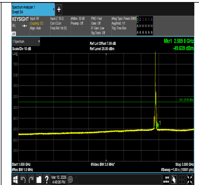
Band7-10MHz-QPSK-21400-1RB#0-1000~3000-PASS
