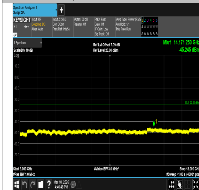
Band7-10MHz-QPSK-20800-50RB#0-3000~18000-PASS
