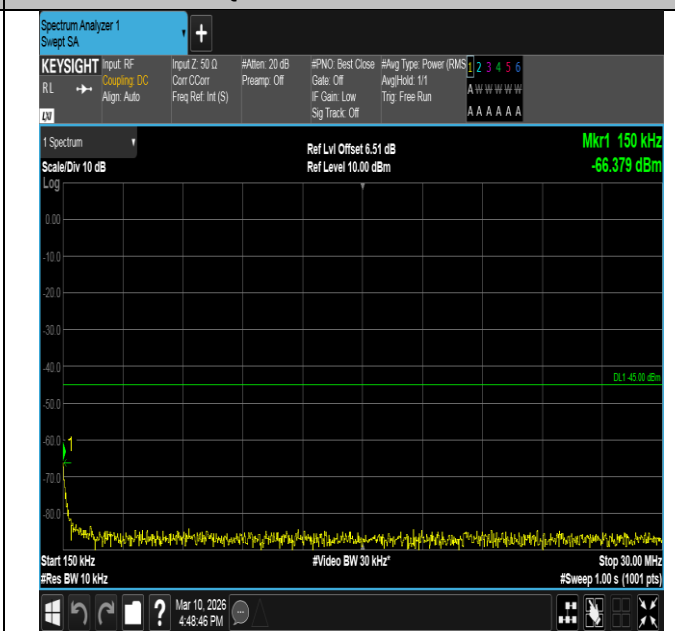
Band7-10MHz-QPSK-21400-1RB#0-0.15~30-PASS
