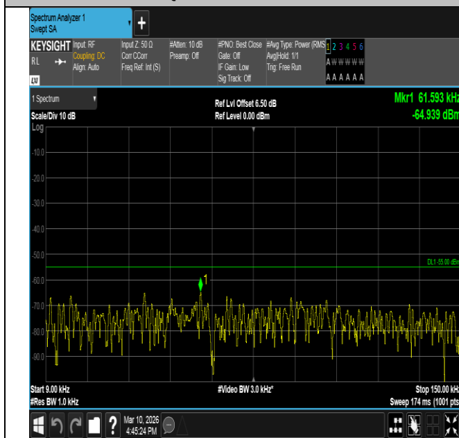
Band7-10MHz-16QAM-21100-1RB#49-0.009~0.15-PASS
