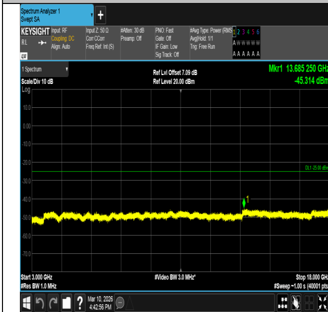
Band7-10MHz-QPSK-21100-1RB#0-3000~18000-PASS
