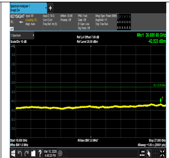
Band7-10MHz-16QAM-21100-50RB#0-18000~27000-PASS
