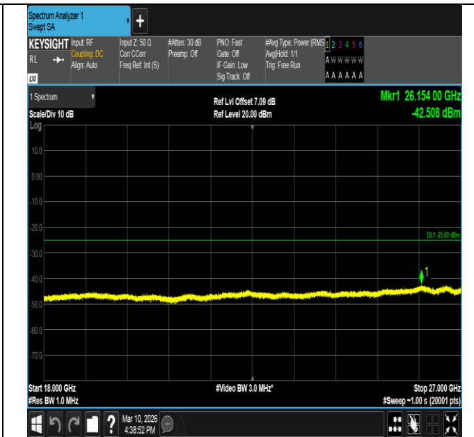
Band7-10MHz-QPSK-20800-1RB#49-18000~27000-PASS
