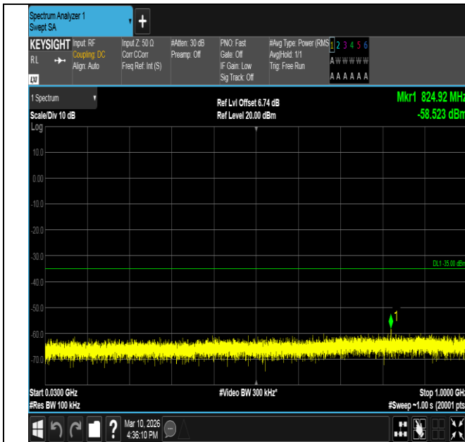
Band7-10MHz-QPSK-20800-1RB#0-30~1000-PASS
