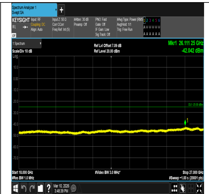
Band7-5MHz-16QAM-21425-25RB#0-18000~27000-PASS
