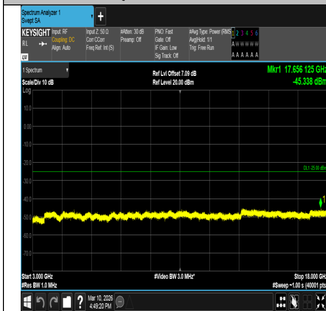
Band7-10MHz-QPSK-21400-1RB#0-3000~18000-PASS
