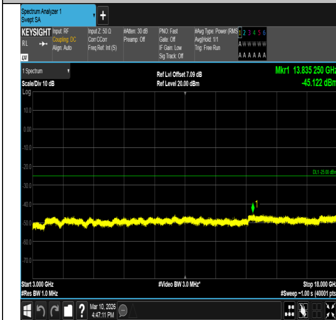
Band7-10MHz-QPSK-21100-50RB#0-3000~18000-PASS
