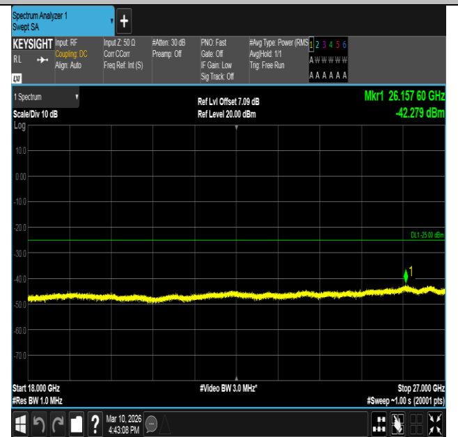
Band7-10MHz-QPSK-21100-1RB#0-18000~27000-PASS
