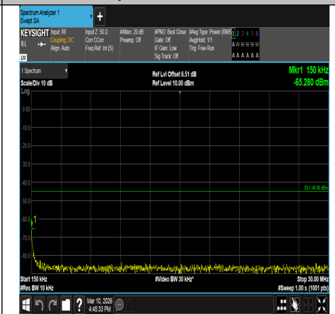
Band7-10MHz-16QAM-21100-1RB#49-0.15~30-PASS
