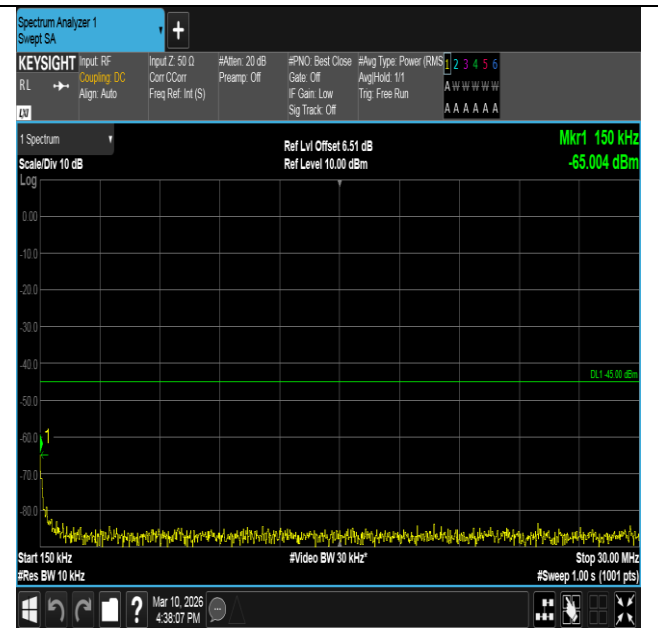
Band7-10MHz-QPSK-20800-1RB#49-0.15~30-PASS
