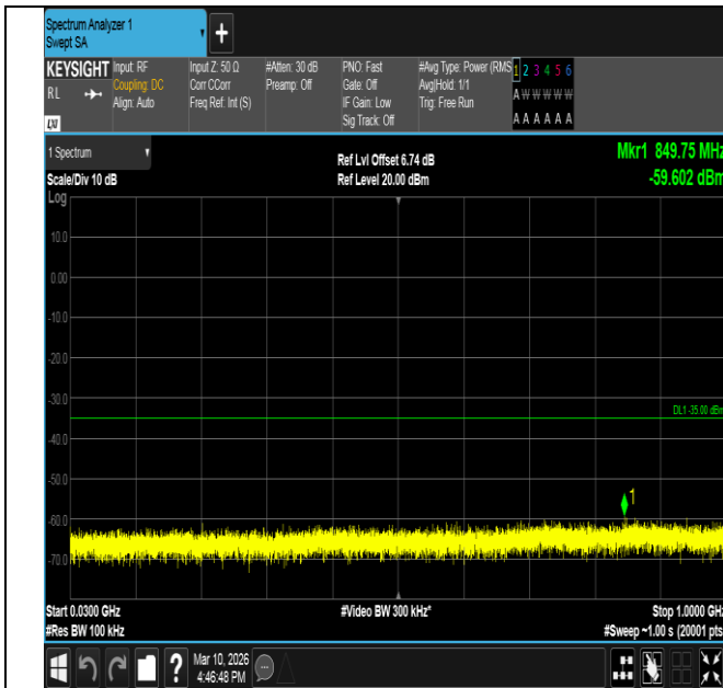
Band7-10MHz-QPSK-21100-50RB#0-30~1000-PASS
