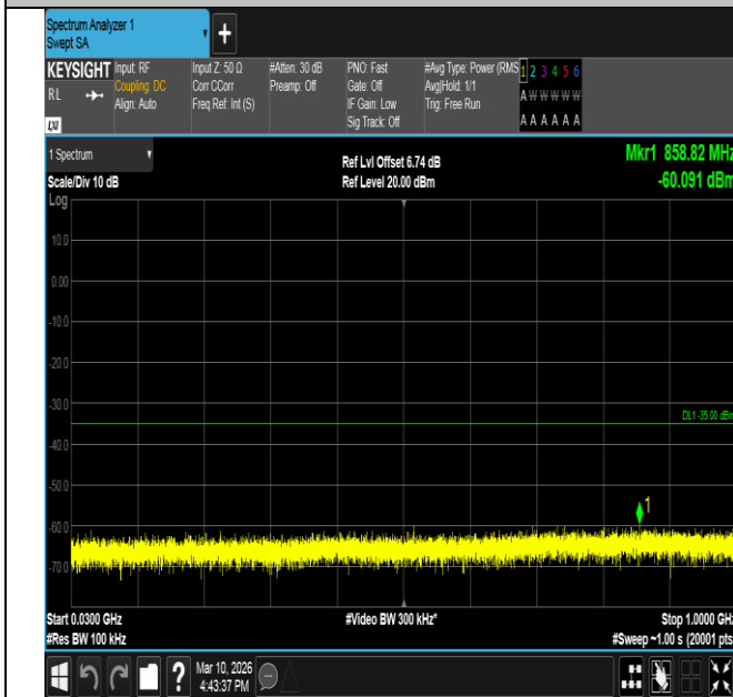
Band7-10MHz-16QAM-21100-1RB#0-30~1000-PASS
