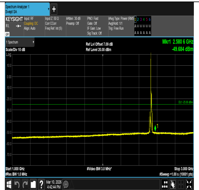
Band7-10MHz-QPSK-21100-1RB#0-1000~3000-PASS
