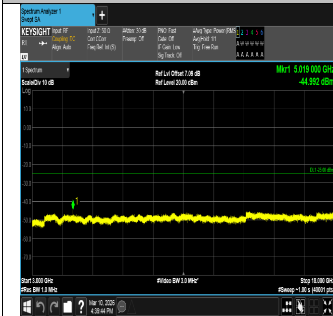
Band7-10MHz-16QAM-20800-1RB#49-3000~18000-PASS
