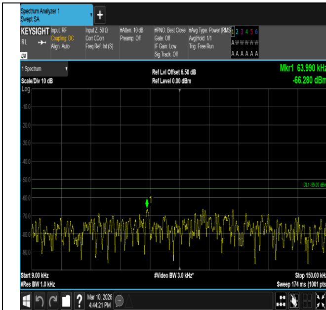
Band7-10MHz-QPSK-21100-1RB#49-0.009~0.15-PASS
