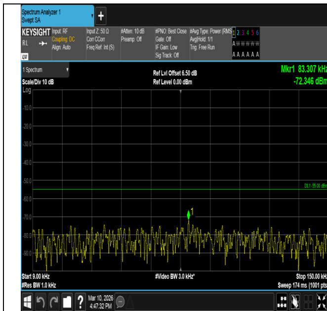
Band7-10MHz-16QAM-21100-50RB#0-0.009~0.15-PASS
