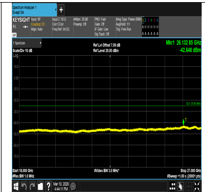
Band7-10MHz-16QAM-21100-1RB#0-18000~27000-PASS
