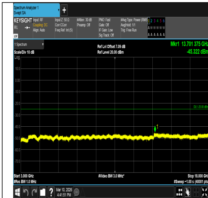
Band7-10MHz-16QAM-20800-50RB#0-3000~18000-PASS
