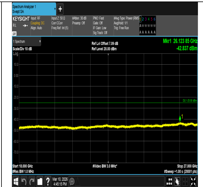
Band7-10MHz-QPSK-21100-1RB#49-18000~27000-PASS
