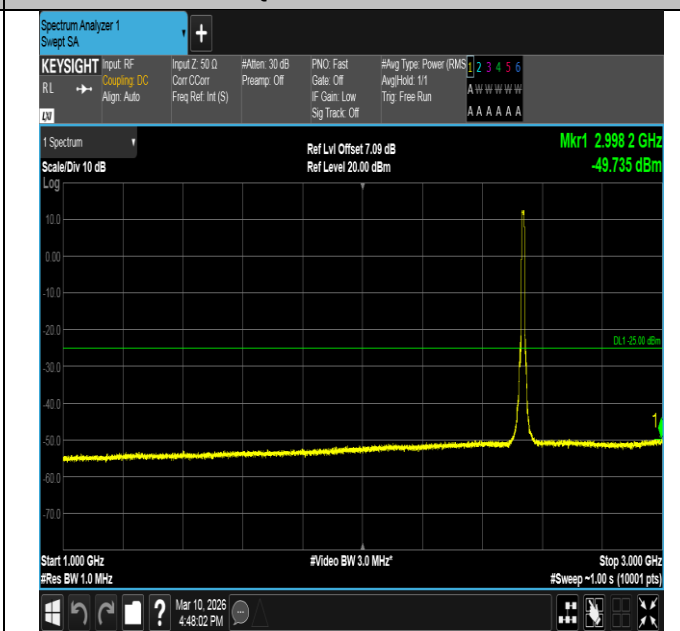
Band7-10MHz-16QAM-21100-50RB#0-1000~3000-PASS
