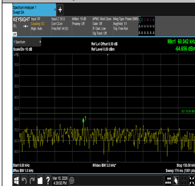
Band7-10MHz-16QAM-20800-1RB#49-0.009~0.15-PASS
