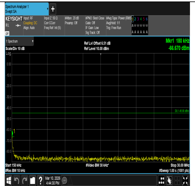
Band7-10MHz-QPSK-21100-1RB#49-0.15~30-PASS
