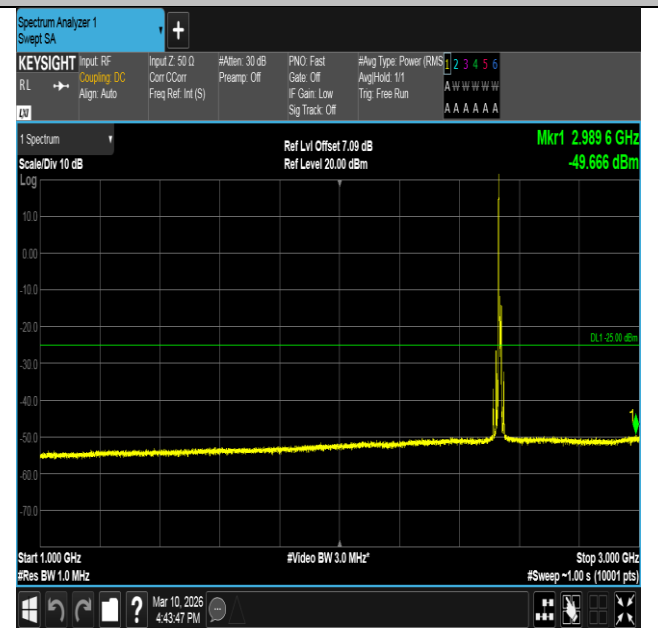
Band7-10MHz-16QAM-21100-1RB#0-1000~3000-PASS
