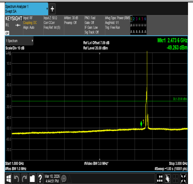
Band7-10MHz-QPSK-21100-1RB#49-1000~3000-PASS
