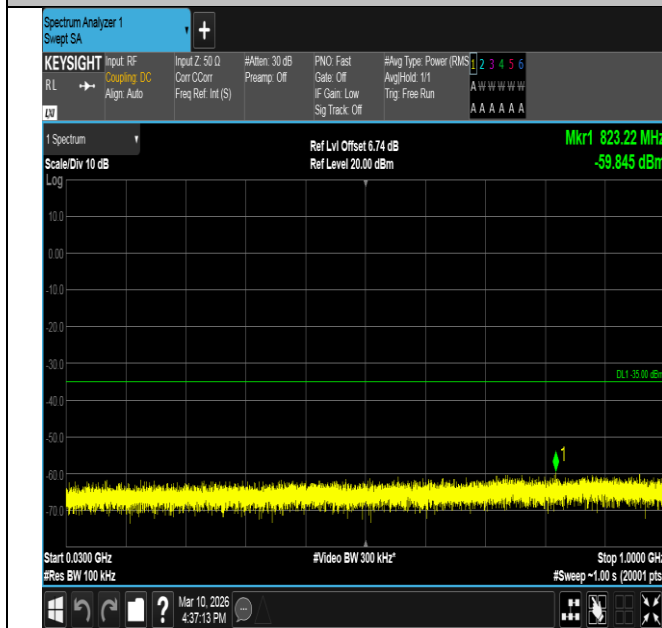
Band7-10MHz-16QAM-20800-1RB#0-30~1000-PASS
