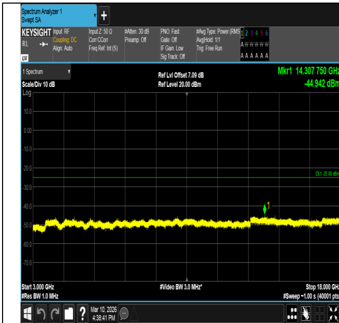
Band7-10MHz-QPSK-20800-1RB#49-3000~18000-PASS
