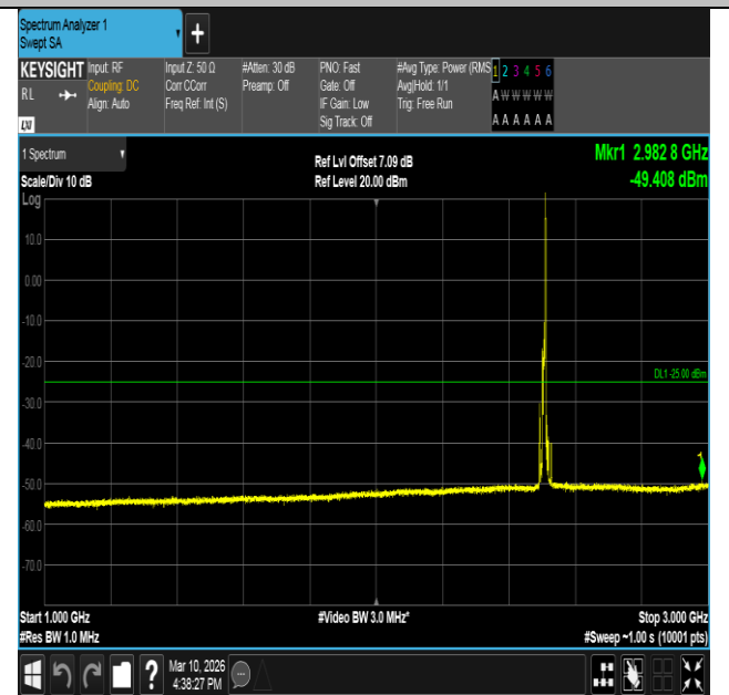
Band7-10MHz-QPSK-20800-1RB#49-1000~3000-PASS
