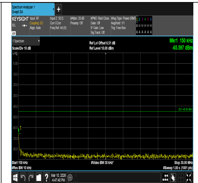
Band7-10MHz-16QAM-21100-50RB#0-0.15~30-PASS
