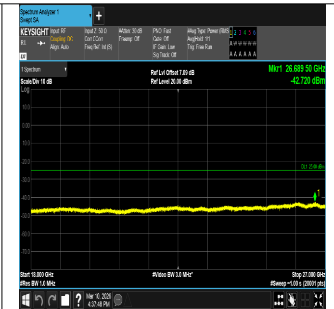
Band7-10MHz-16QAM-20800-1RB#0-18000~27000-PASS
