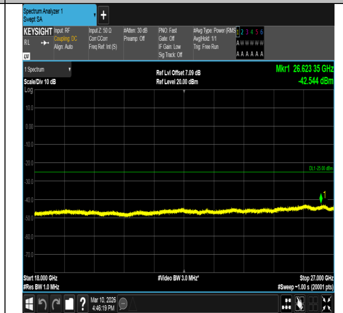
Band7-10MHz-16QAM-21100-1RB#49-18000~27000-PASS
