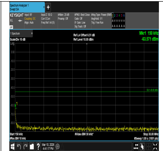
Band7-10MHz-16QAM-20800-50RB#0-0.15~30-PASS
