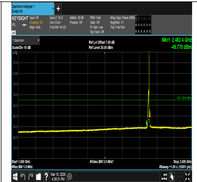
Band7-10MHz-16QAM-20800-1RB#49-1000~3000-PASS
