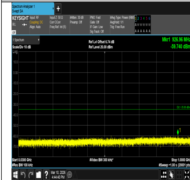
Band7-10MHz-QPSK-21100-1RB#49-30~1000-PASS
