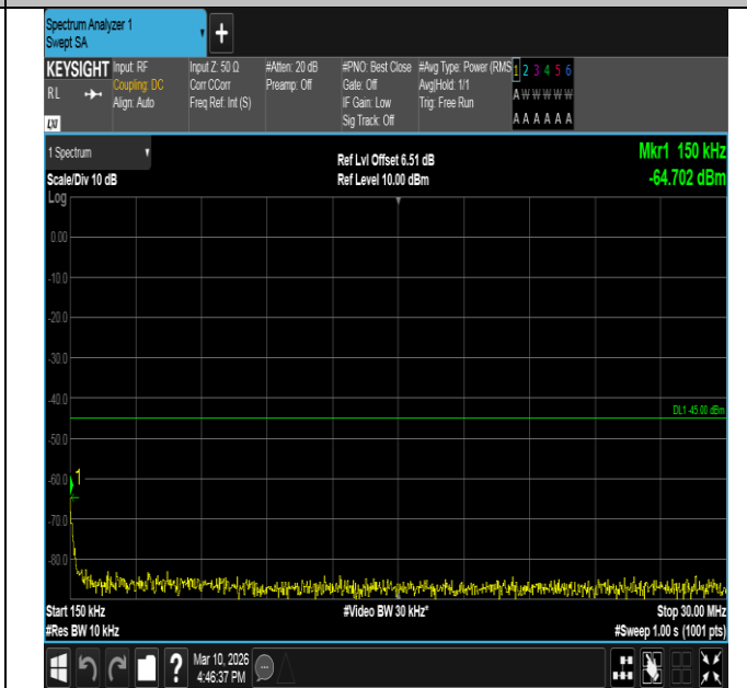
Band7-10MHz-QPSK-21100-50RB#0-0.15~30-PASS
