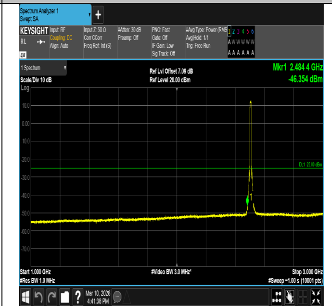
Band7-10MHz-16QAM-20800-50RB#0-1000~3000-PASS
