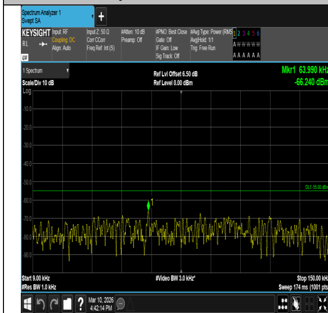
Band7-10MHz-QPSK-21100-1RB#0-0.009~0.15-PASS
