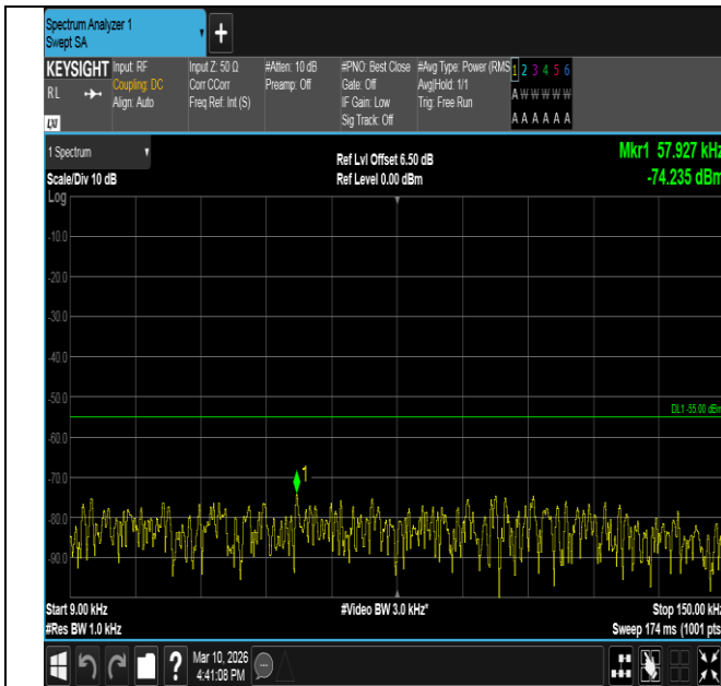
Band7-10MHz-16QAM-20800-50RB#0-0.009~0.15-PASS
