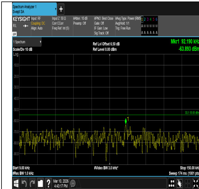
Band7-10MHz-16QAM-21100-1RB#0-0.009~0.15-PASS
