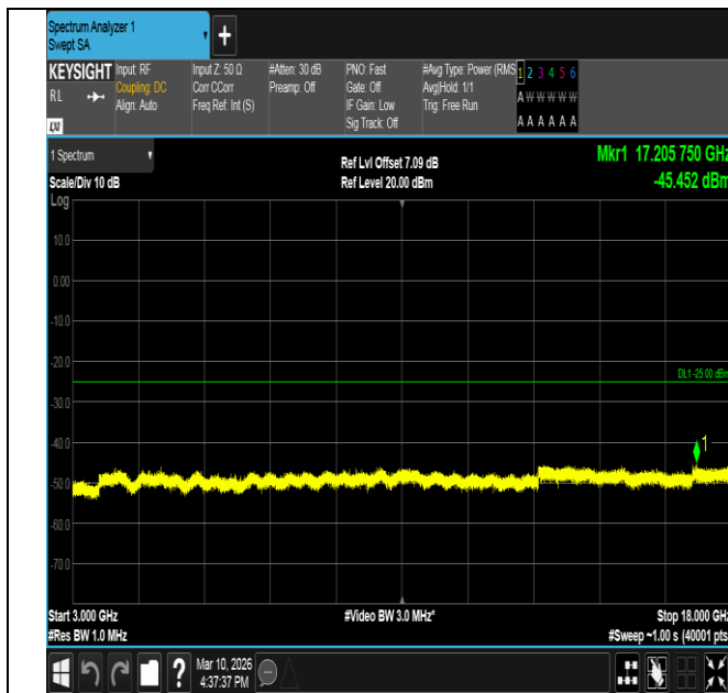
Band7-10MHz-16QAM-20800-1RB#0-3000~18000-PASS
