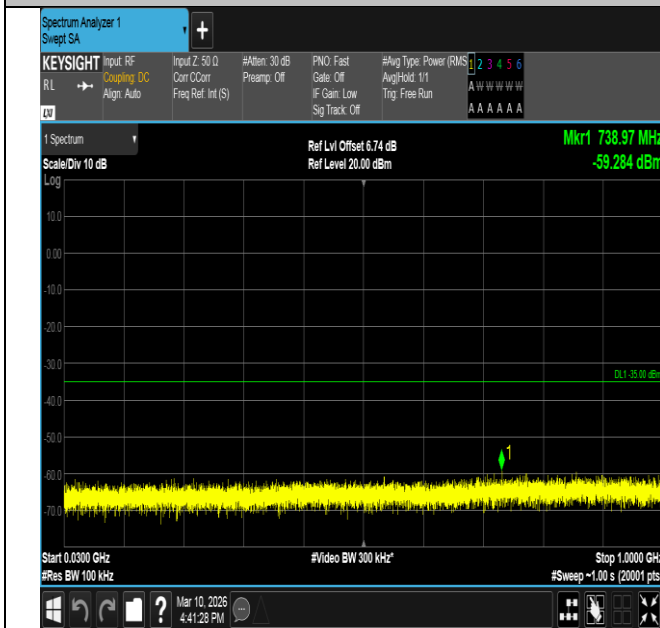
Band7-10MHz-16QAM-20800-50RB#0-30~1000-PASS
