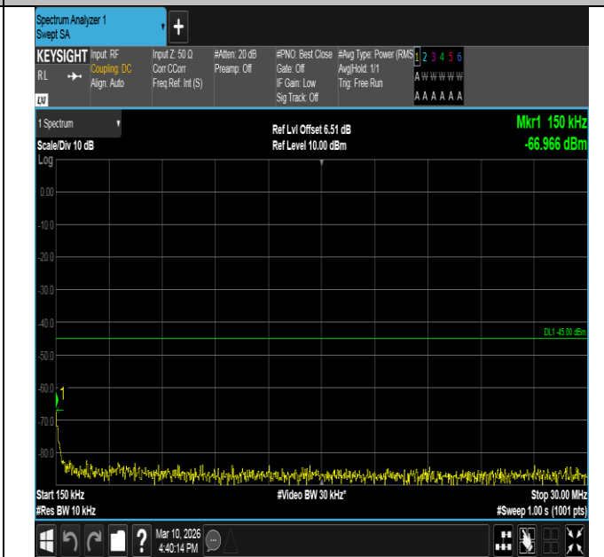
Band7-10MHz-QPSK-20800-50RB#0-0.15~30-PASS
