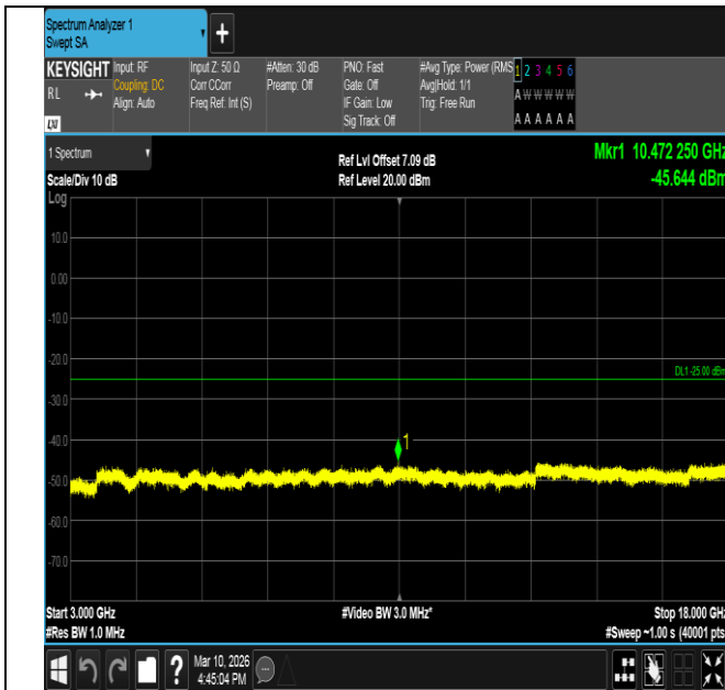
Band7-10MHz-QPSK-21100-1RB#49-3000~18000-PASS
