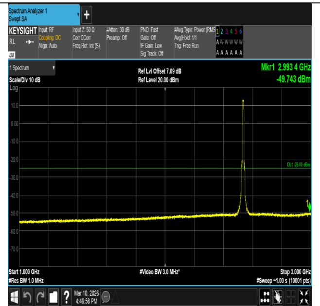
Band7-10MHz-QPSK-21100-50RB#0-1000~3000-PASS
