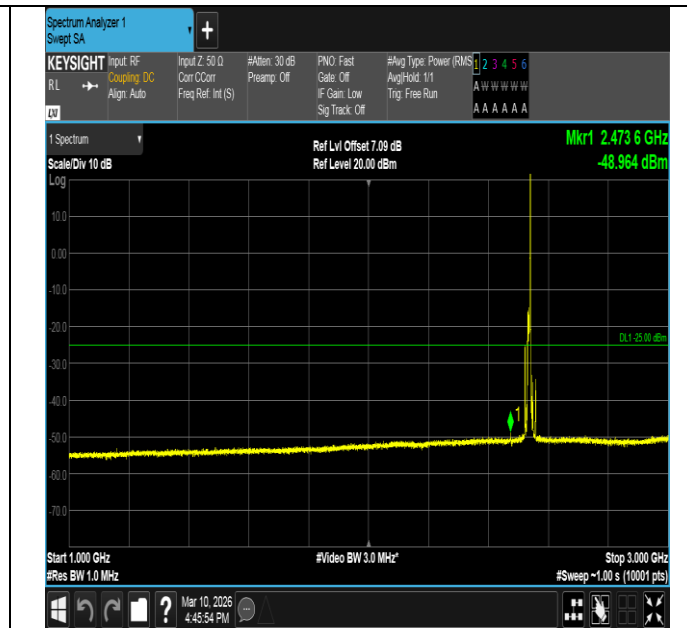
Band7-10MHz-16QAM-21100-1RB#49-1000~3000-PASS
