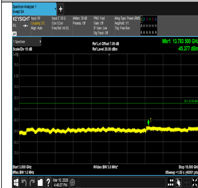
Band7-10MHz-16QAM-21100-1RB#49-3000~18000-PASS
