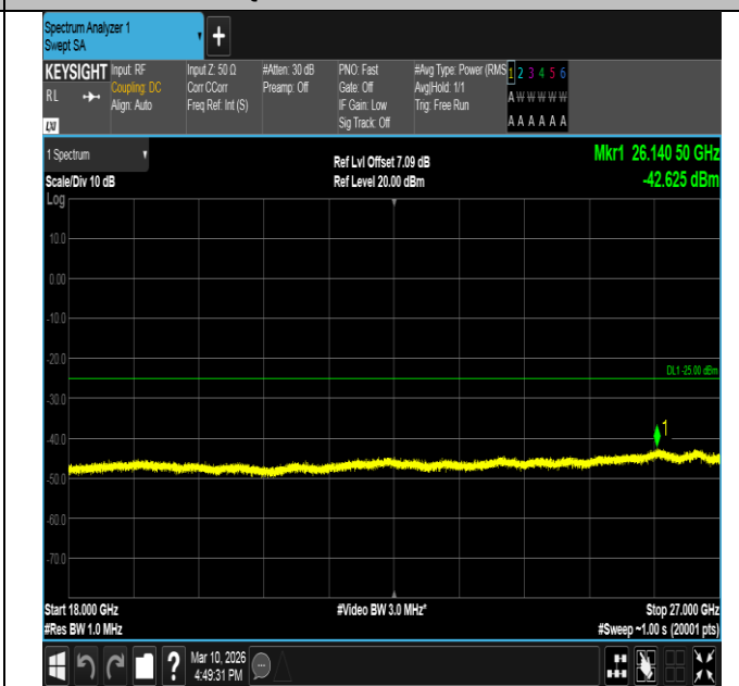
Band7-10MHz-QPSK-21400-1RB#0-18000~27000-PASS
