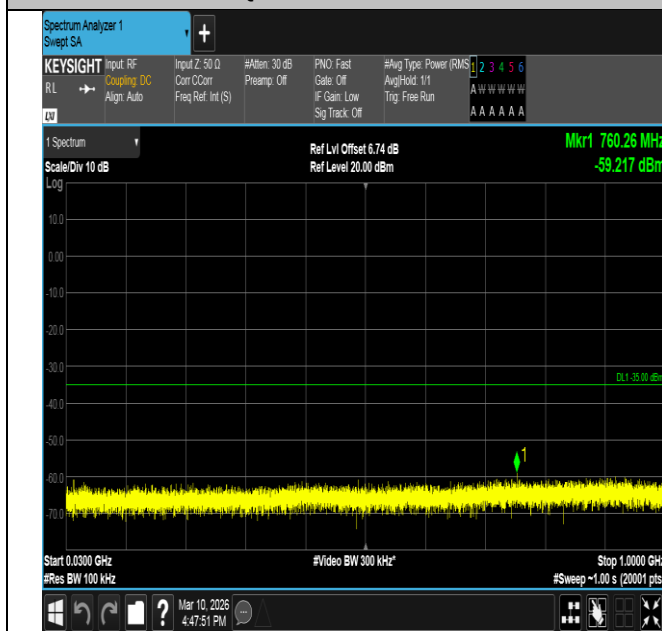
Band7-10MHz-16QAM-21100-50RB#0-30~1000-PASS
