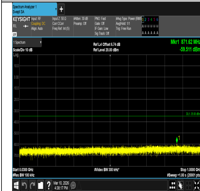
Band7-10MHz-QPSK-20800-1RB#49-30~1000-PASS
