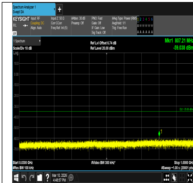
Band7-10MHz-QPSK-21400-1RB#0-30~1000-PASS
