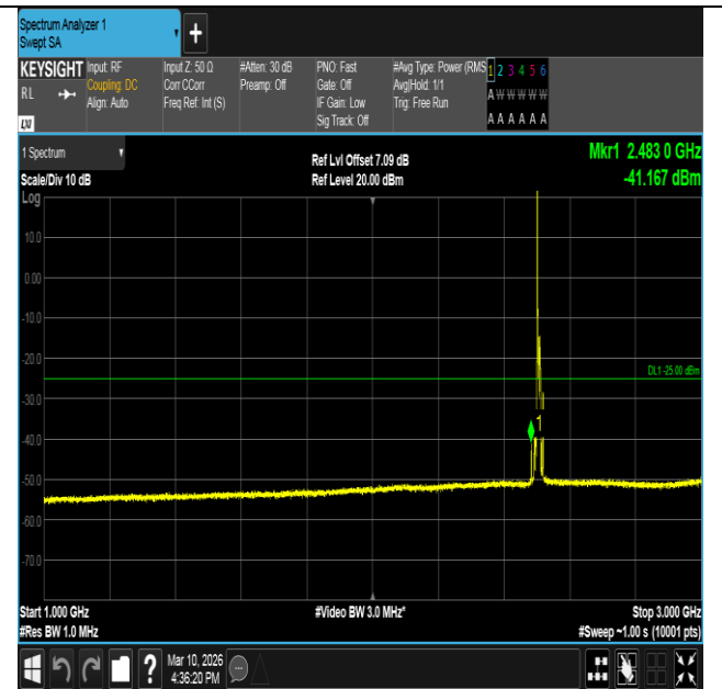
Band7-10MHz-QPSK-20800-1RB#0-1000~3000-PASS
