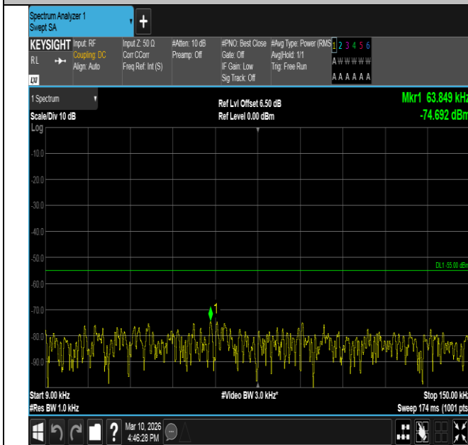
Band7-10MHz-QPSK-21100-50RB#0-0.009~0.15-PASS
