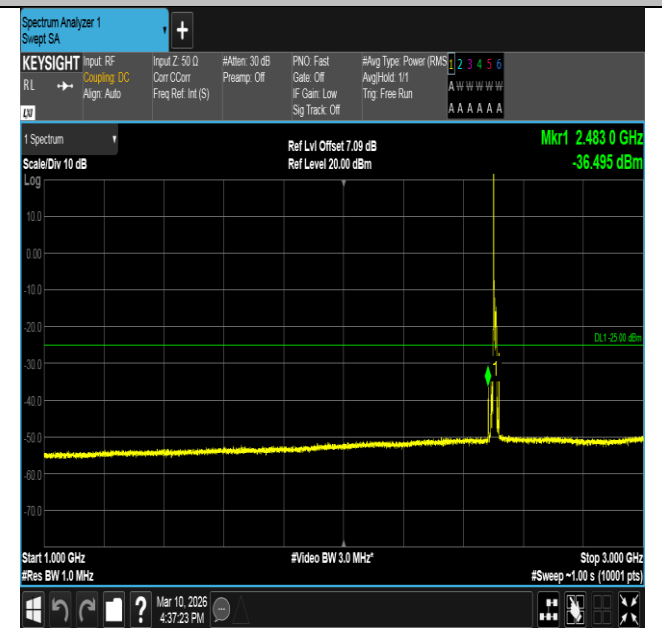
Band7-10MHz-16QAM-20800-1RB#0-1000~3000-PASS
