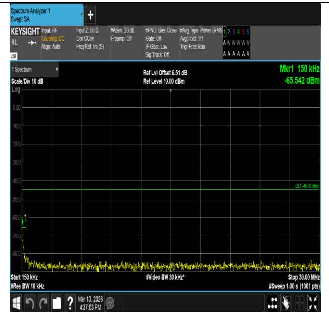
Band7-10MHz-16QAM-20800-1RB#0-0.15~30-PASS
