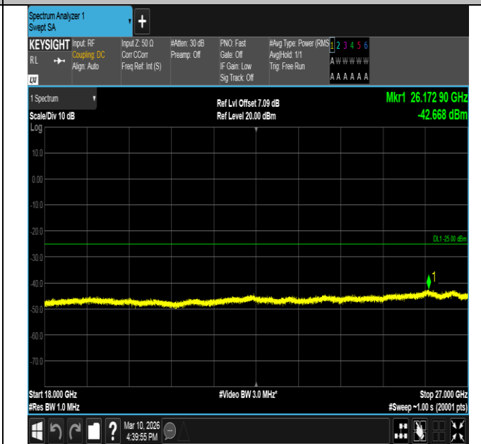
Band7-10MHz-16QAM-20800-1RB#49-18000~27000-PASS
