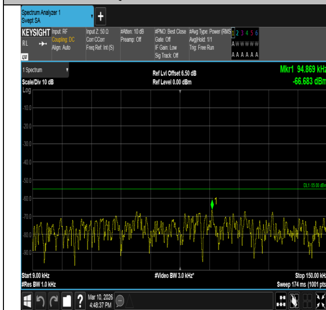
Band7-10MHz-QPSK-21400-1RB#0-0.009~0.15-PASS
