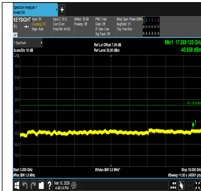
Band7-10MHz-16QAM-21100-50RB#0-3000~18000-PASS
