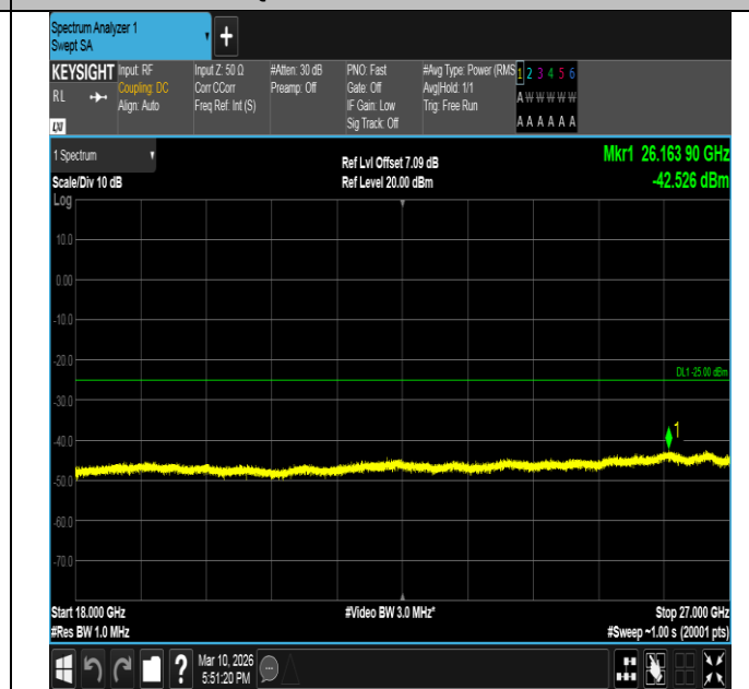
Band7-15MHz-QPSK-21100-1RB#0-18000~27000-PASS
