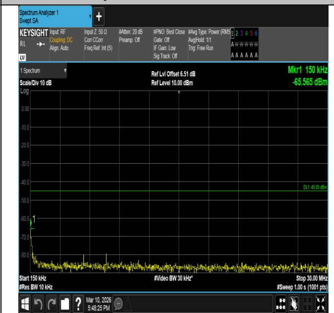
Band7-15MHz-QPSK-20825-75RB#0-0.15~30-PASS
