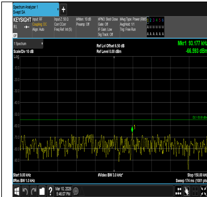
Band7-15MHz-QPSK-20825-1RB#74-0.009~0.15-PASS
