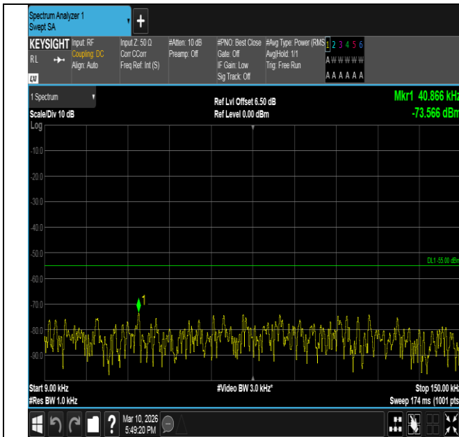
Band7-15MHz-16QAM-20825-75RB#0-0.009~0.15-PASS
