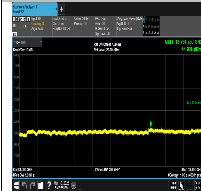
Band7-15MHz-16QAM-20825-1RB#74-3000~18000-PASS
