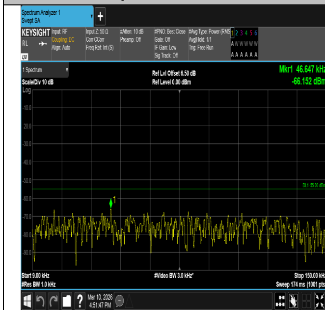
Band7-10MHz-16QAM-21400-1RB#49-0.009~0.15-PASS
