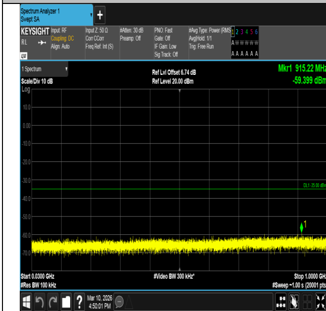
Band7-10MHz-16QAM-21400-1RB#0-30~1000-PASS
