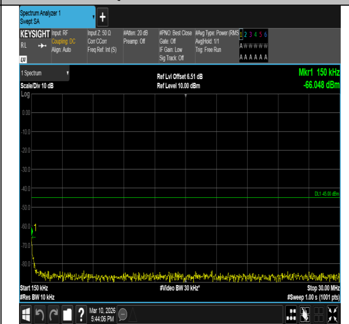
Band7-15MHz-QPSK-20825-1RB#0-0.15~30-PASS
