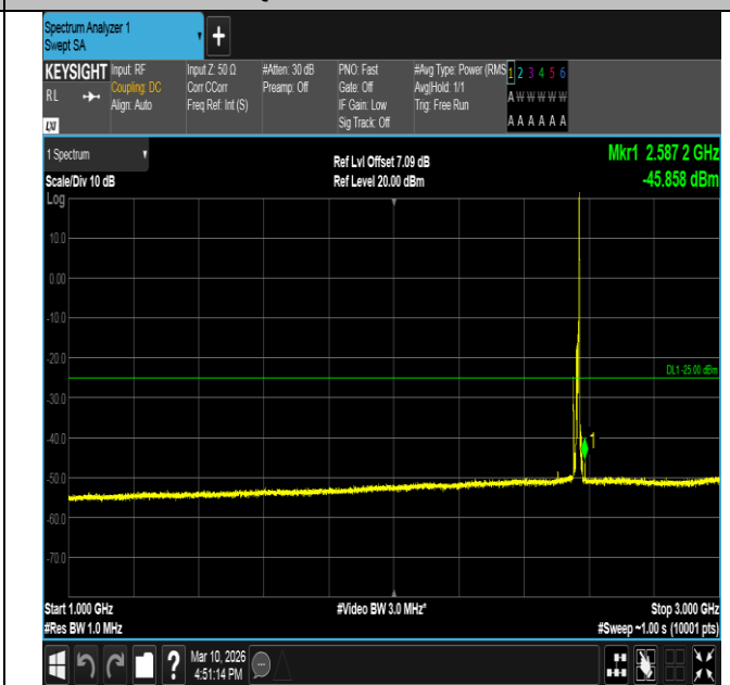
Band7-10MHz-QPSK-21400-1RB#49-1000~3000-PASS
