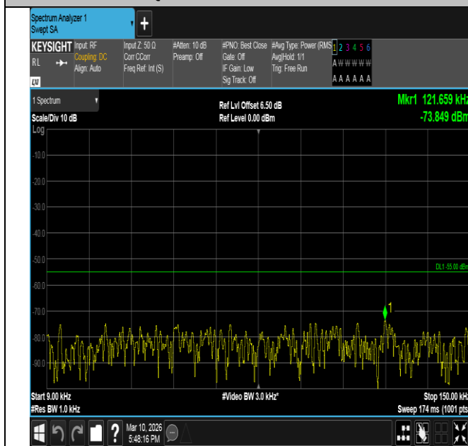
Band7-15MHz-QPSK-20825-75RB#0-0.009~0.15-PASS
