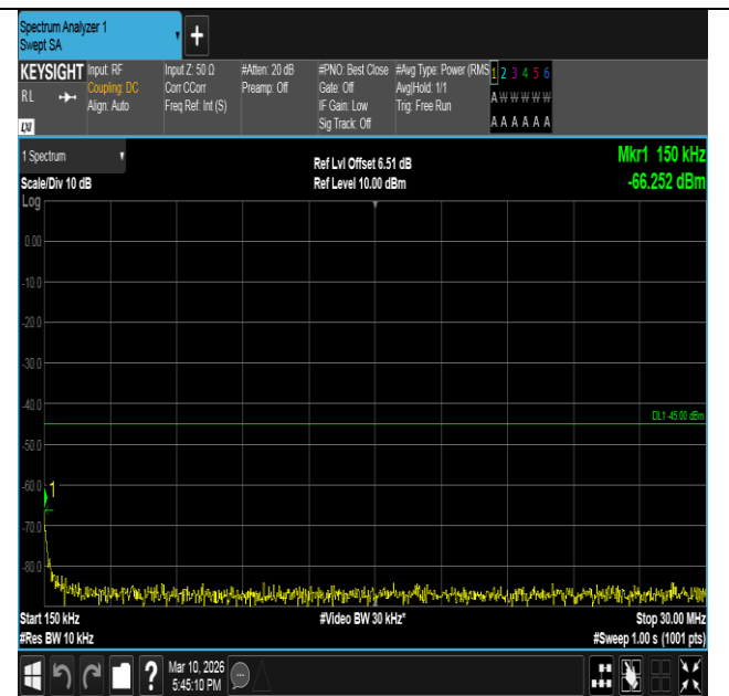
Band7-15MHz-16QAM-20825-1RB#0-0.15~30-PASS
