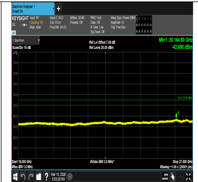
Band7-15MHz-QPSK-21100-1RB#74-18000~27000-PASS
