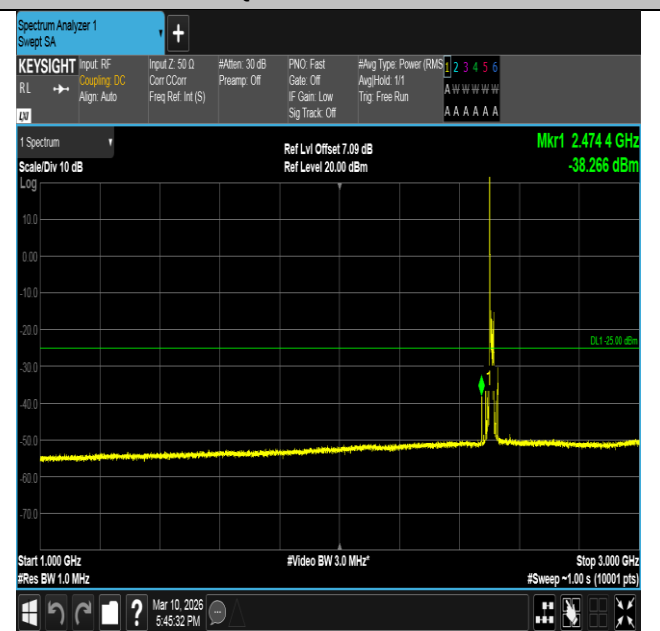
Band7-15MHz-16QAM-20825-1RB#0-1000~3000-PASS
