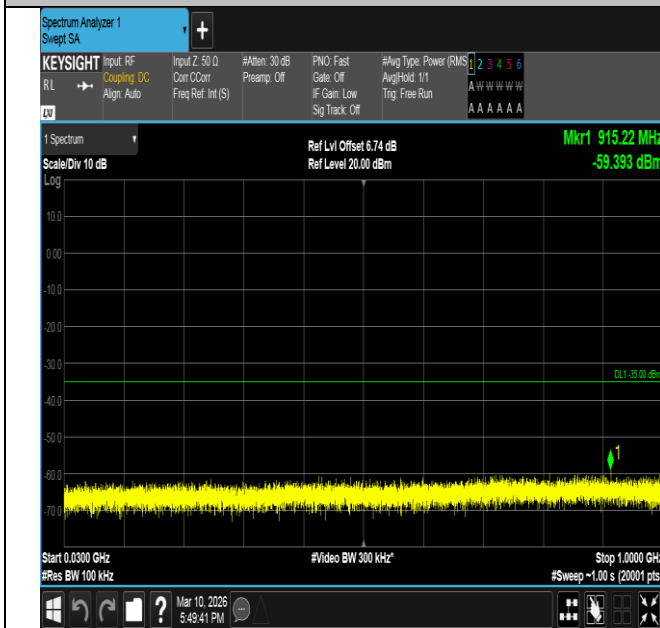
Band7-15MHz-16QAM-20825-75RB#0-30~1000-PASS
