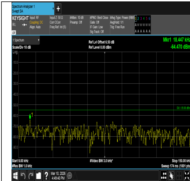
Band7-10MHz-16QAM-21400-1RB#0-0.009~0.15-PASS
