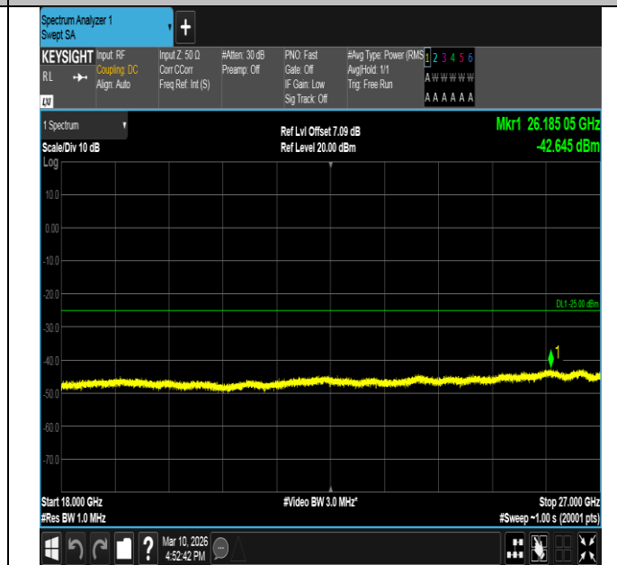
Band7-10MHz-16QAM-21400-1RB#49-18000~27000-PASS
