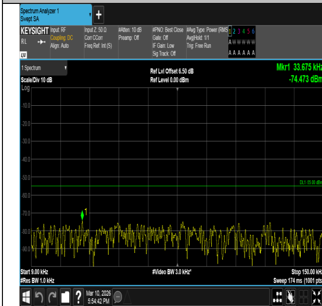
Band7-15MHz-QPSK-21100-75RB#0-0.009~0.15-PASS
