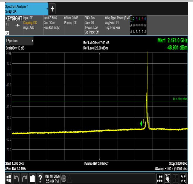
Band7-15MHz-QPSK-21100-1RB#74-1000~3000-PASS
