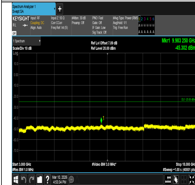
Band7-10MHz-QPSK-21400-50RB#0-3000~18000-PASS
