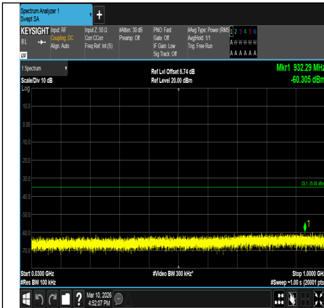
Band7-10MHz-16QAM-21400-1RB#49-30~1000-PASS
