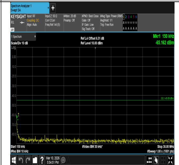
Band7-15MHz-QPSK-21100-75RB#0-0.15~30-PASS
