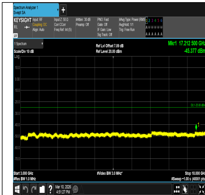
Band7-10MHz-QPSK-21400-1RB#49-3000~18000-PASS
