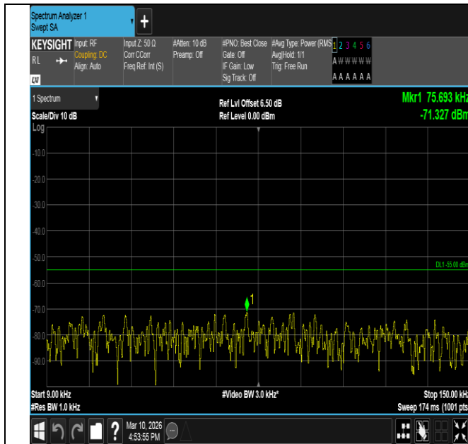
Band7-10MHz-16QAM-21400-50RB#0-0.009~0.15-PASS
