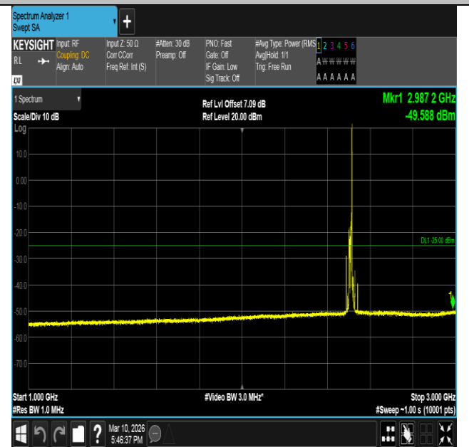
Band7-15MHz-QPSK-20825-1RB#74-1000~3000-PASS
