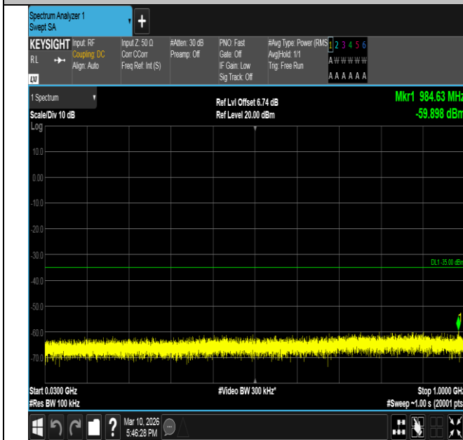
Band7-15MHz-QPSK-20825-1RB#74-30~1000-PASS
