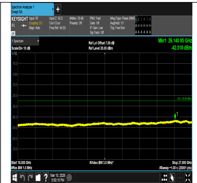
Band7-15MHz-16QAM-20825-75RB#0-18000~27000-PASS
