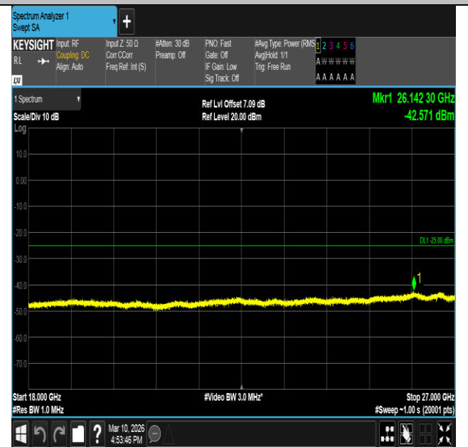
Band7-10MHz-QPSK-21400-50RB#0-18000~27000-PASS
