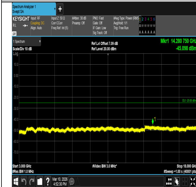
Band7-10MHz-16QAM-21400-1RB#49-3000~18000-PASS
