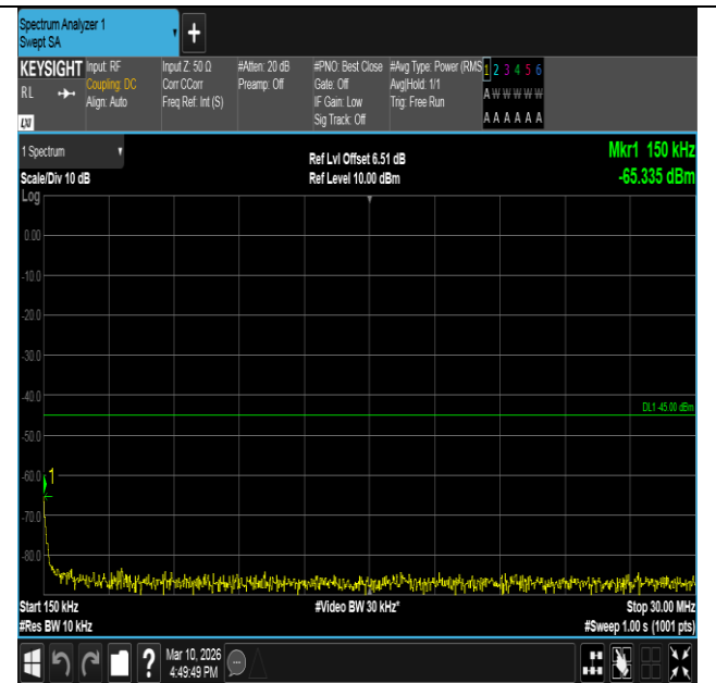
Band7-10MHz-16QAM-21400-1RB#0-0.15~30-PASS
