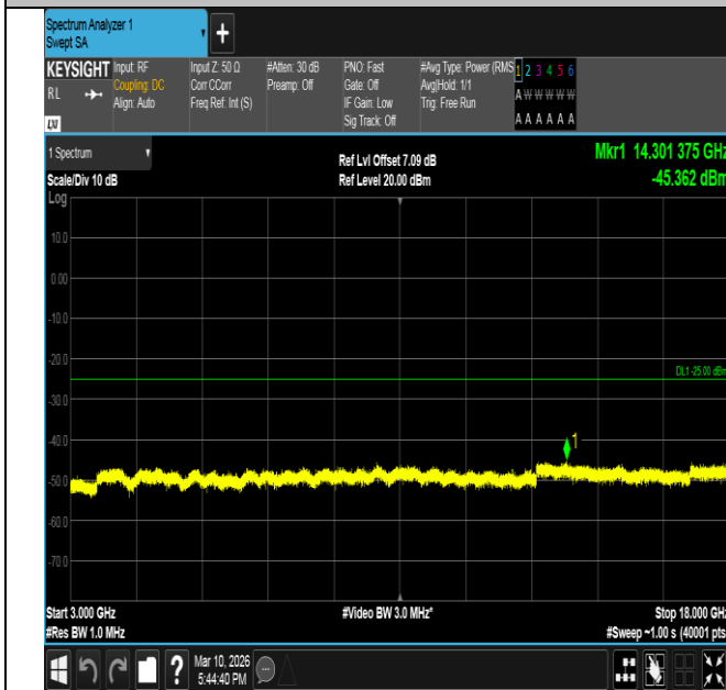
Band7-15MHz-QPSK-20825-1RB#0-3000~18000-PASS
