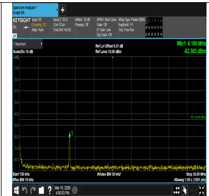
Band7-10MHz-QPSK-21400-1RB#49-0.15~30-PASS
