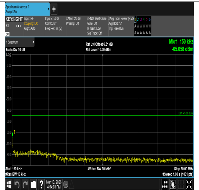
Band7-10MHz-16QAM-21400-50RB#0-0.15~30-PASS
