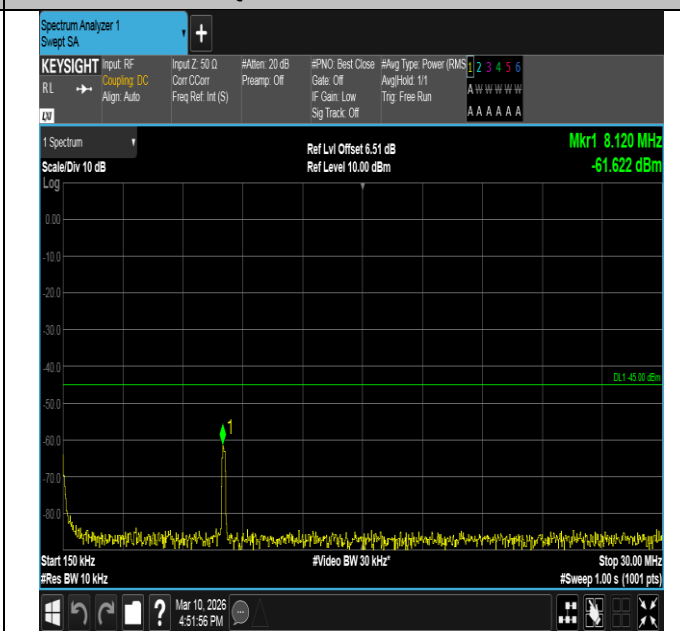
Band7-10MHz-16QAM-21400-1RB#49-0.15~30-PASS
