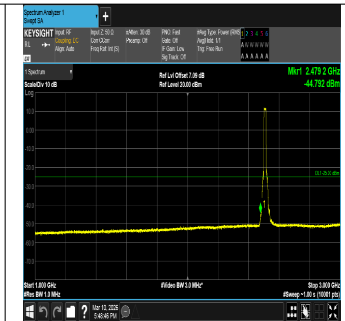
Band7-15MHz-QPSK-20825-75RB#0-1000~3000-PASS
