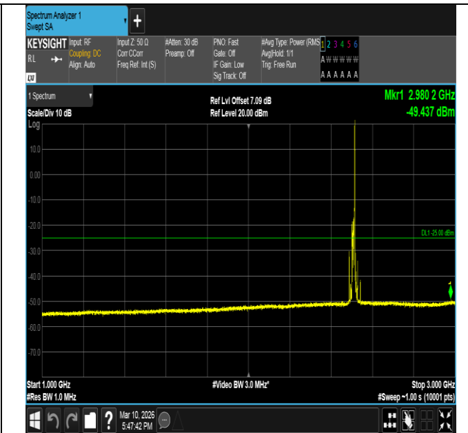
Band7-15MHz-16QAM-20825-1RB#74-1000~3000-PASS
