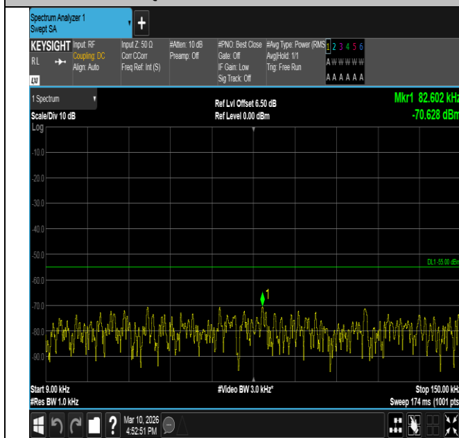
Band7-10MHz-QPSK-21400-50RB#0-0.009~0.15-PASS
