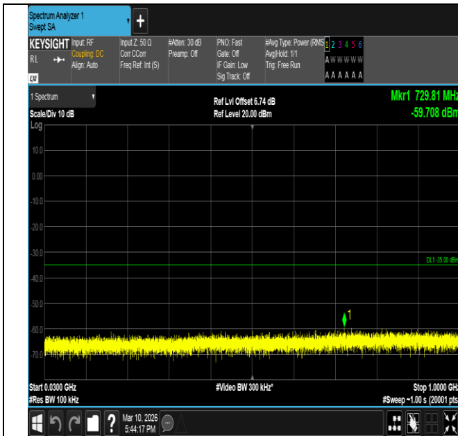
Band7-15MHz-QPSK-20825-1RB#0-30~1000-PASS
