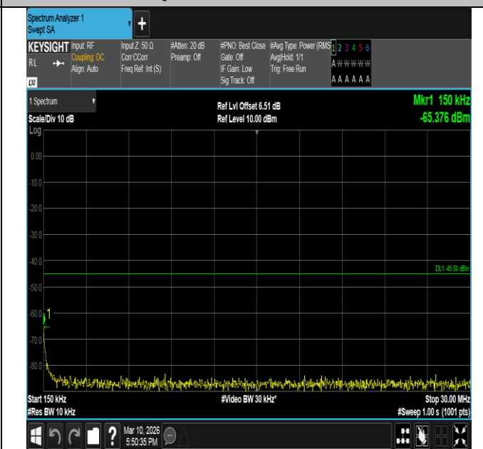
Band7-15MHz-QPSK-21100-1RB#0-0.15~30-PASS
