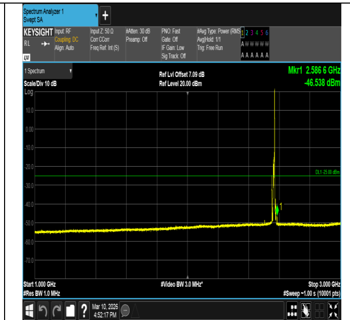
Band7-10MHz-16QAM-21400-1RB#49-1000~3000-PASS
