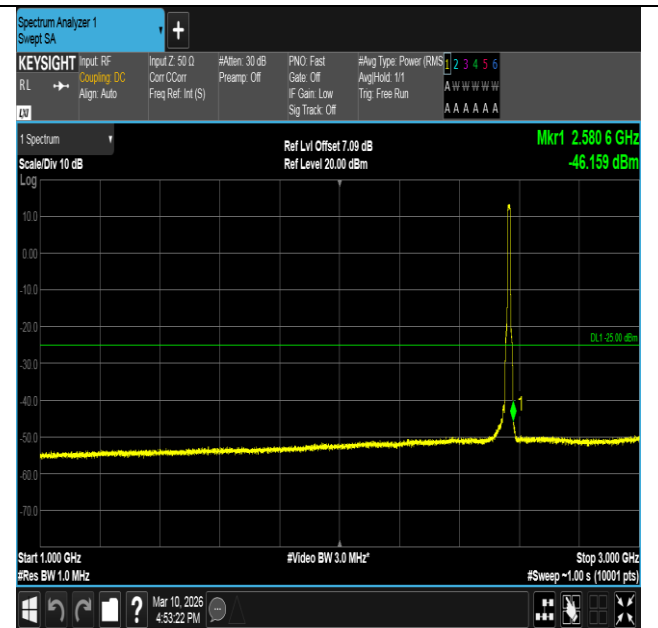
Band7-10MHz-QPSK-21400-50RB#0-1000~3000-PASS
