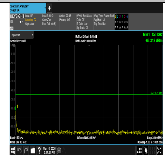
Band7-15MHz-16QAM-20825-1RB#74-0.15~30-PASS
