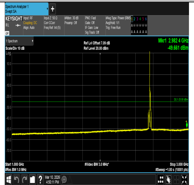
Band7-10MHz-16QAM-21400-1RB#0-1000~3000-PASS
