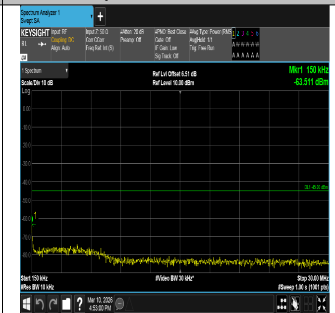
Band7-10MHz-QPSK-21400-50RB#0-0.15~30-PASS
