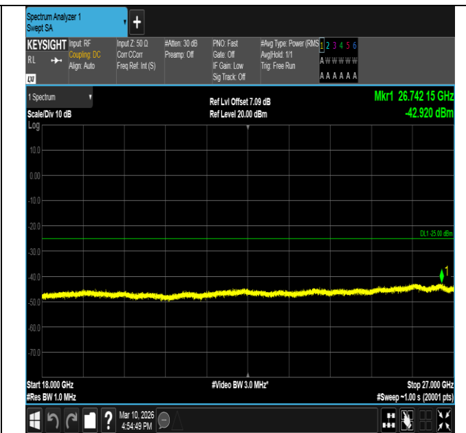
Band7-10MHz-16QAM-21400-50RB#0-18000~27000-PASS
