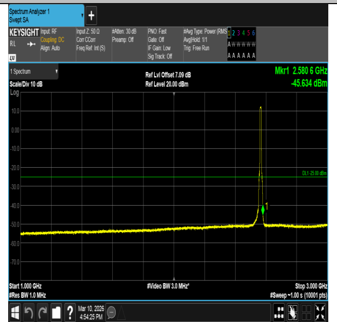
Band7-10MHz-16QAM-21400-50RB#0-1000~3000-PASS
