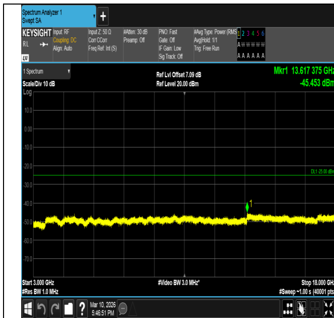
Band7-15MHz-QPSK-20825-1RB#74-3000~18000-PASS
