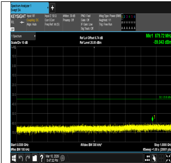
Band7-15MHz-16QAM-20825-1RB#74-30~1000-PASS
