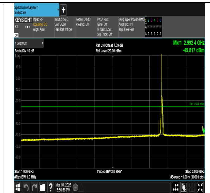
Band7-15MHz-QPSK-21100-1RB#0-1000~3000-PASS
