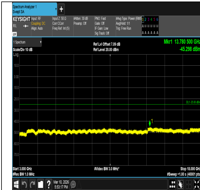
Band7-15MHz-QPSK-21100-1RB#74-3000~18000-PASS
