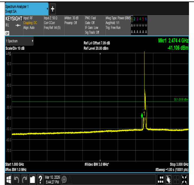
Band7-15MHz-QPSK-20825-1RB#0-1000~3000-PASS
