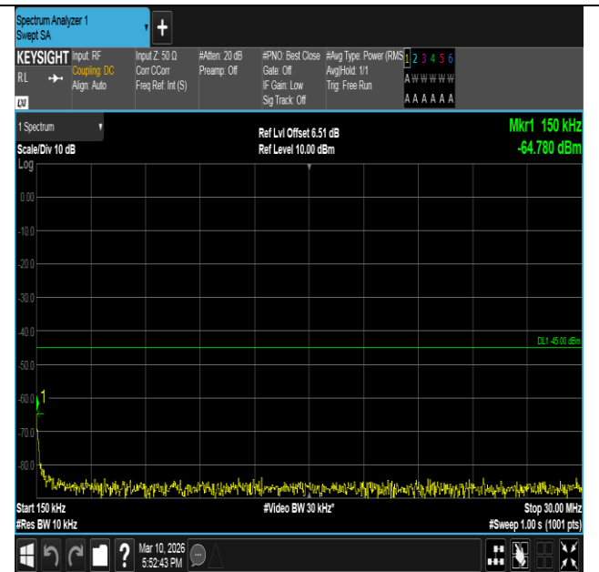
Band7-15MHz-QPSK-21100-1RB#74-0.15~30-PASS
