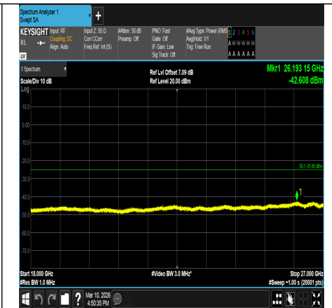
Band7-10MHz-16QAM-21400-1RB#0-18000~27000-PASS
