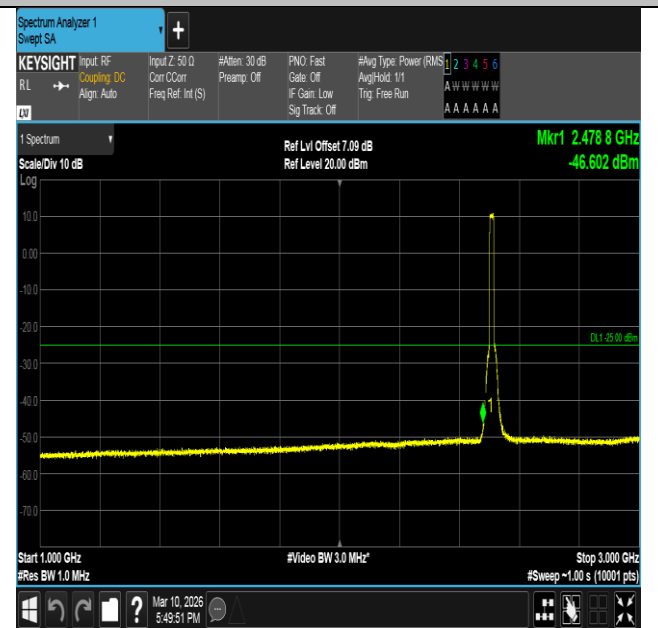
Band7-15MHz-16QAM-20825-75RB#0-1000~3000-PASS
