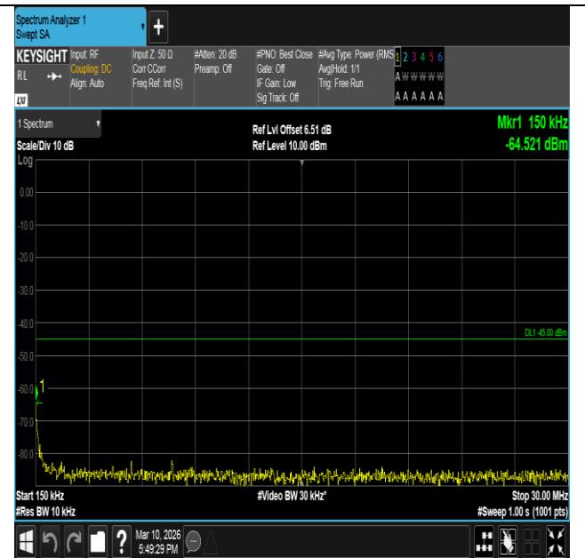
Band7-15MHz-16QAM-20825-75RB#0-0.15~30-PASS
