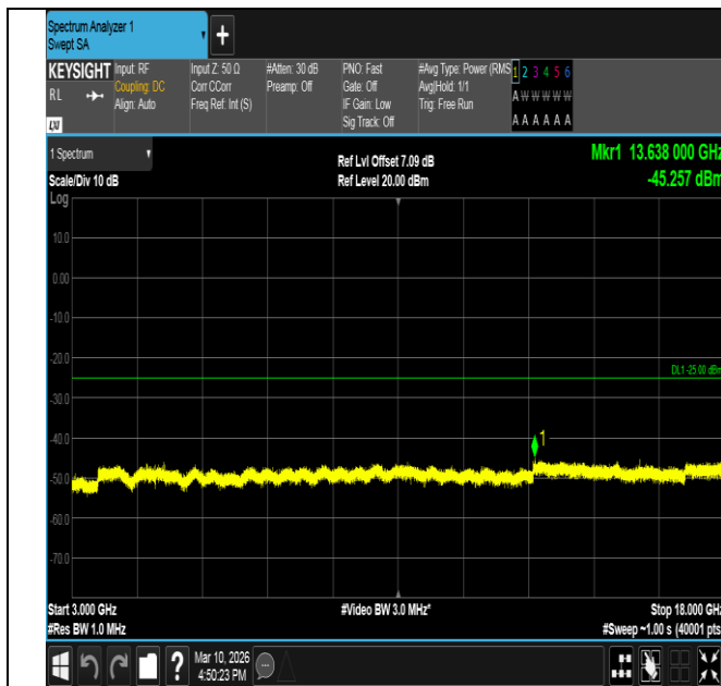
Band7-10MHz-16QAM-21400-1RB#0-3000~18000-PASS
