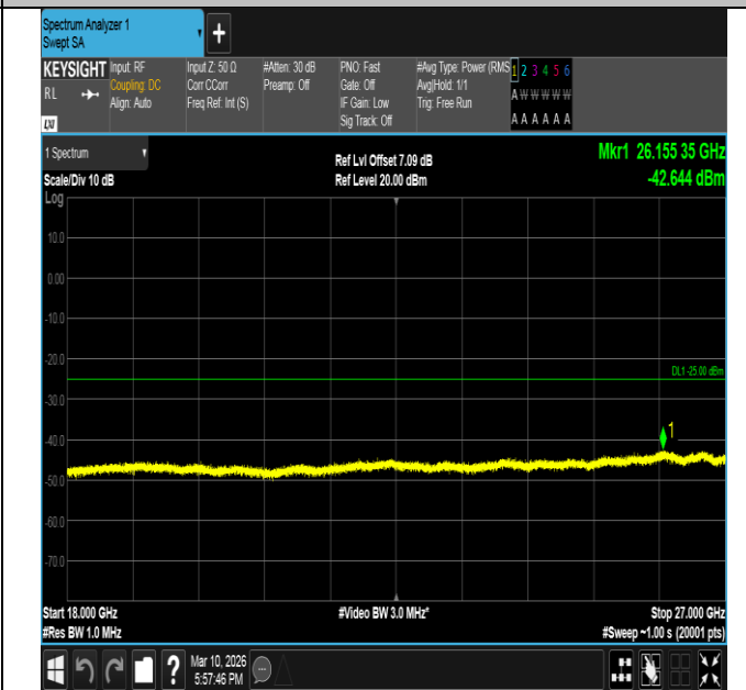
Band7-15MHz-QPSK-21375-1RB#0-18000~27000-PASS
