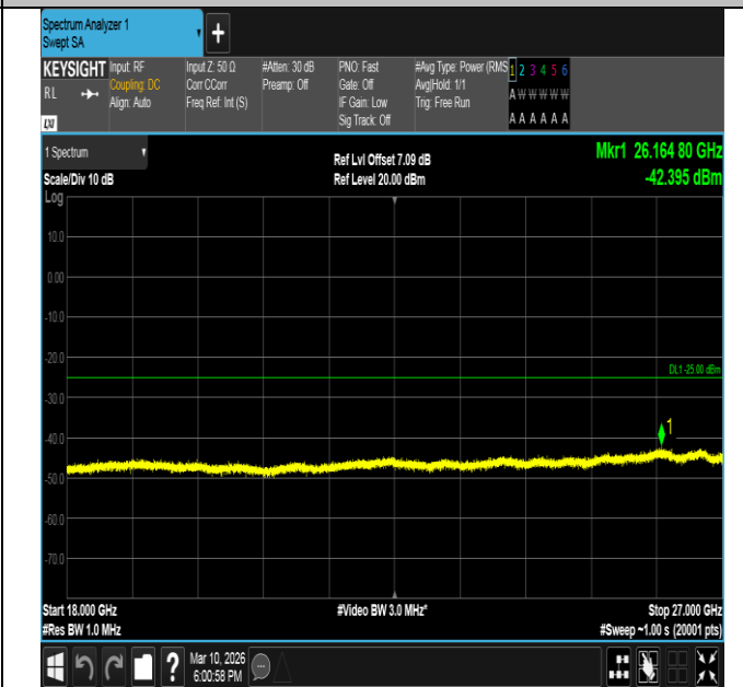
Band7-15MHz-16QAM-21375-1RB#74-18000~27000-PASS
