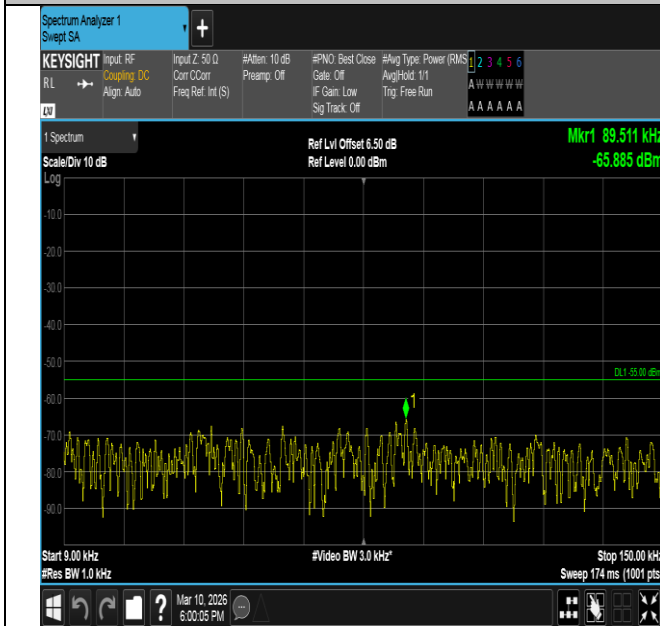
Band7-15MHz-16QAM-21375-1RB#74-0.009~0.15-PASS
