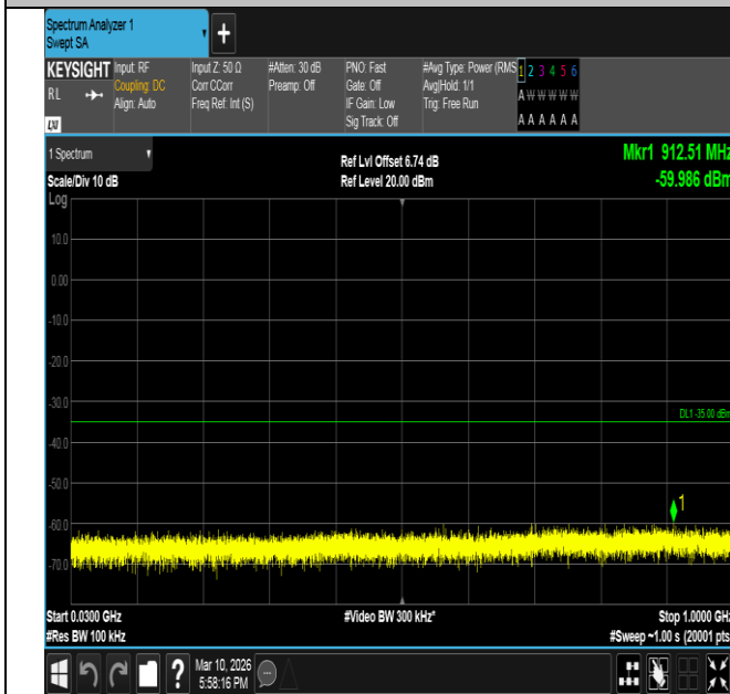
Band7-15MHz-16QAM-21375-1RB#0-30~1000-PASS
