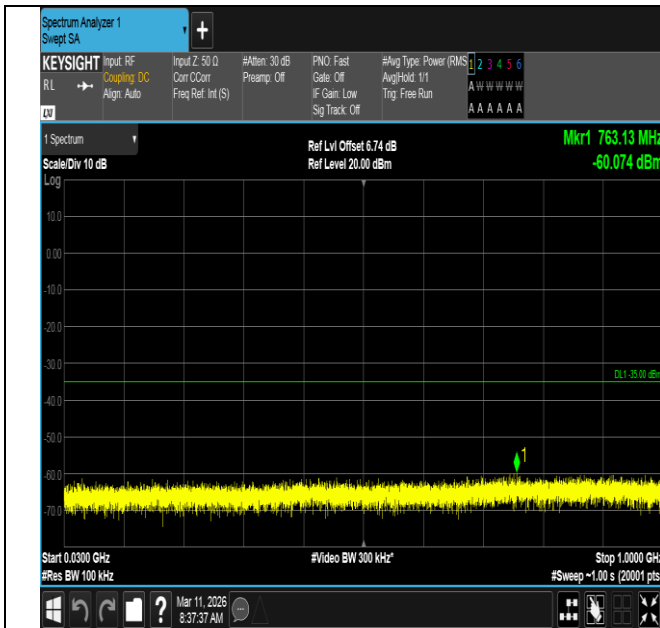
Band7-15MHz-QPSK-21375-75RB#0-30~1000-PASS
