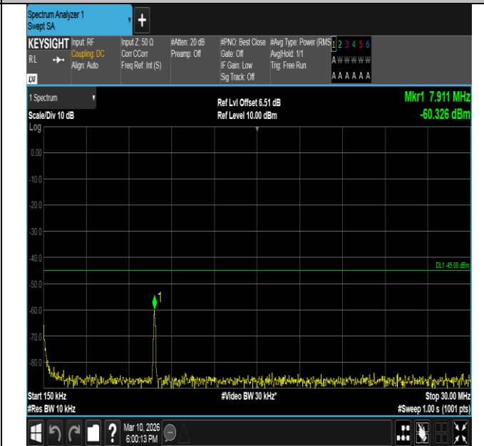
Band7-15MHz-16QAM-21375-1RB#74-0.15~30-PASS
