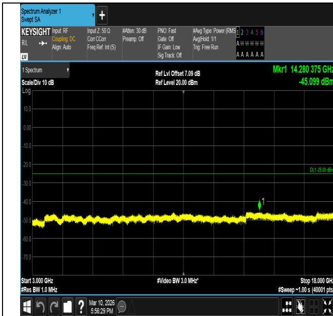
Band7-15MHz-16QAM-21100-75RB#0-3000~18000-PASS
