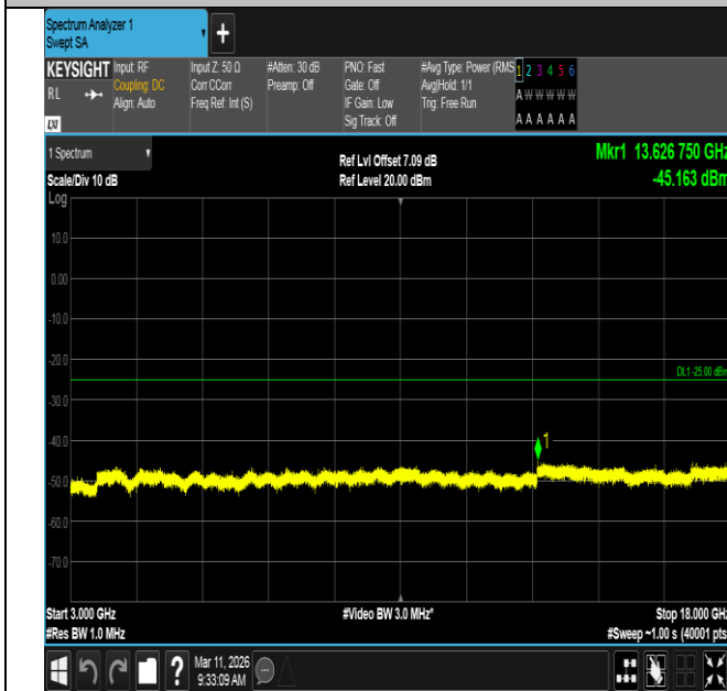
Band7-20MHz-QPSK-20850-100RB#0-3000~18000-PASS
