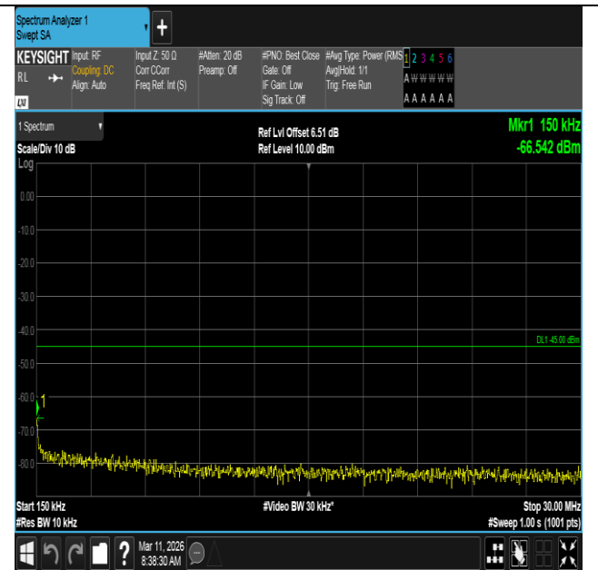
Band7-15MHz-16QAM-21375-75RB#0-0.15~30-PASS
