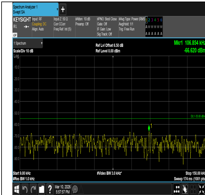
Band7-15MHz-16QAM-21375-1RB#0-0.009~0.15-PASS
