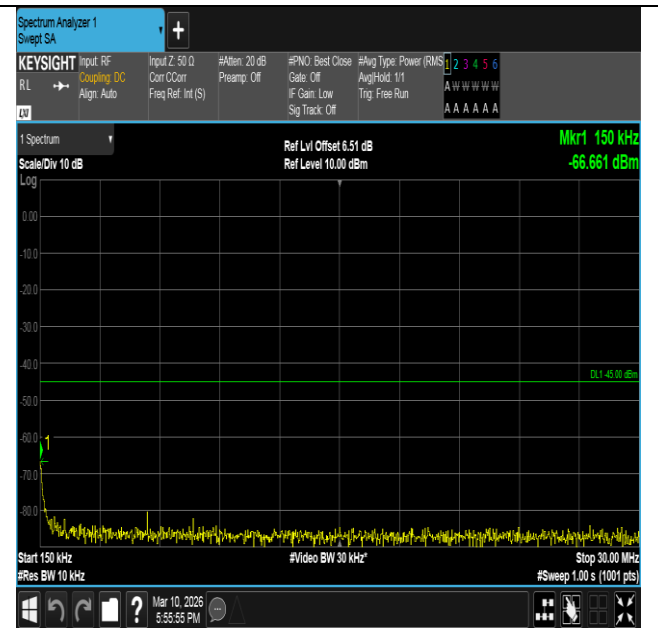
Band7-15MHz-16QAM-21100-75RB#0-0.15~30-PASS
