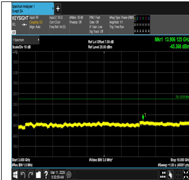
Band7-20MHz-QPSK-20850-1RB#99-3000~18000-PASS
