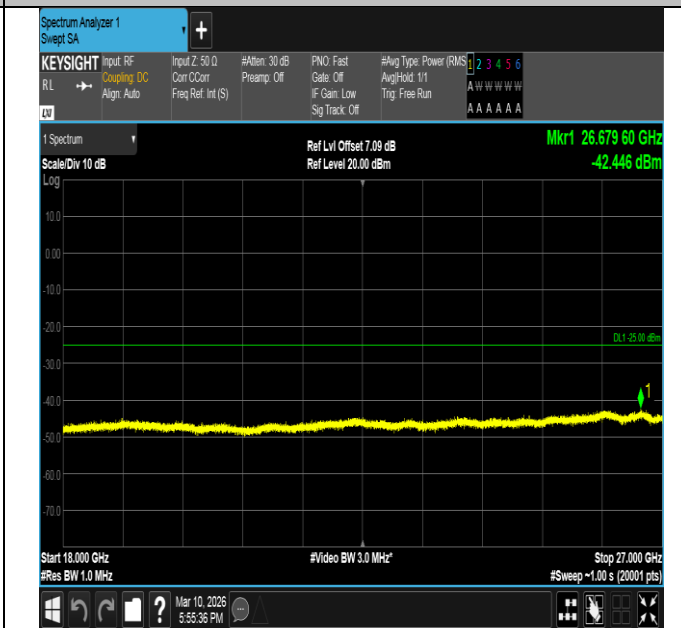
Band7-15MHz-QPSK-21100-75RB#0-18000~27000-PASS
