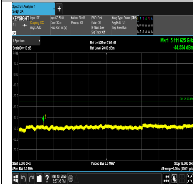
Band7-15MHz-QPSK-21375-1RB#0-3000~18000-PASS
