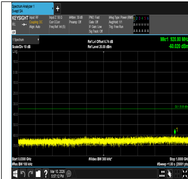
Band7-15MHz-QPSK-21375-1RB#0-30~1000-PASS
