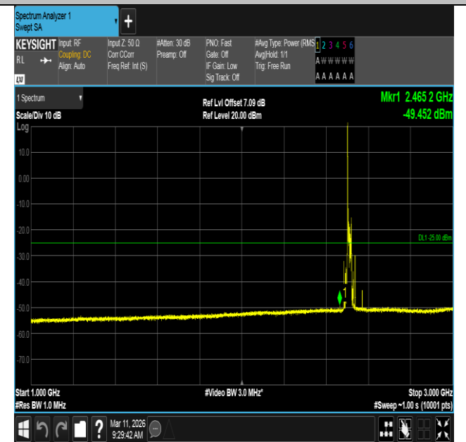
Band7-20MHz-16QAM-20850-1RB#0-1000~3000-PASS
