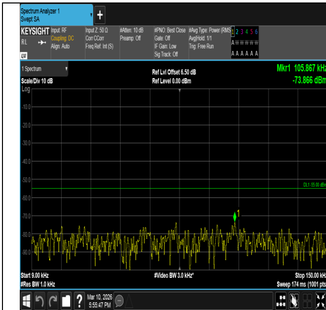
Band7-15MHz-16QAM-21100-75RB#0-0.009~0.15-PASS
