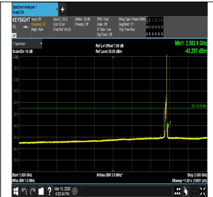
Band7-15MHz-16QAM-21375-1RB#74-1000~3000-PASS
