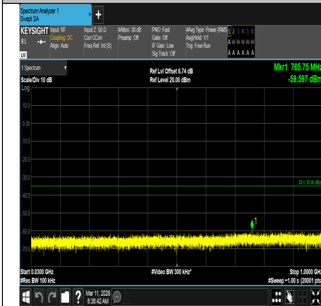
Band7-15MHz-16QAM-21375-75RB#0-30~1000-PASS
