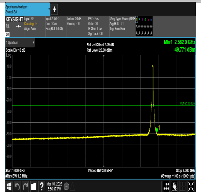
Band7-15MHz-16QAM-21100-75RB#0-1000~3000-PASS
