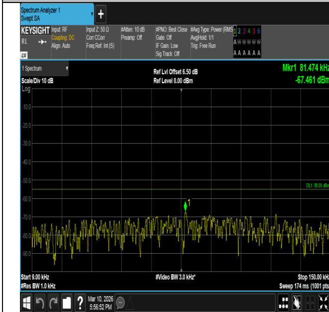
Band7-15MHz-QPSK-21375-1RB#0-0.009~0.15-PASS
