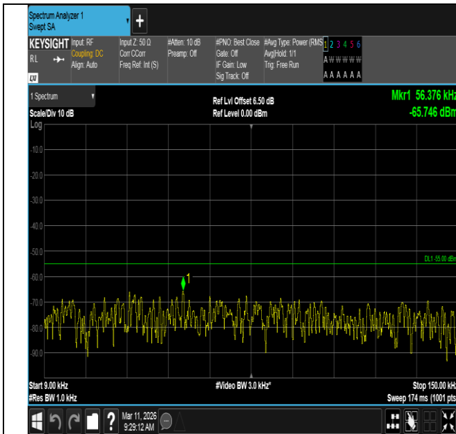
Band7-20MHz-16QAM-20850-1RB#0-0.009~0.15-PASS
