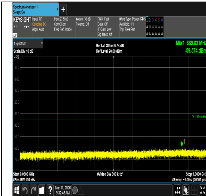
Band7-20MHz-QPSK-20850-100RB#0-30~1000-PASS
