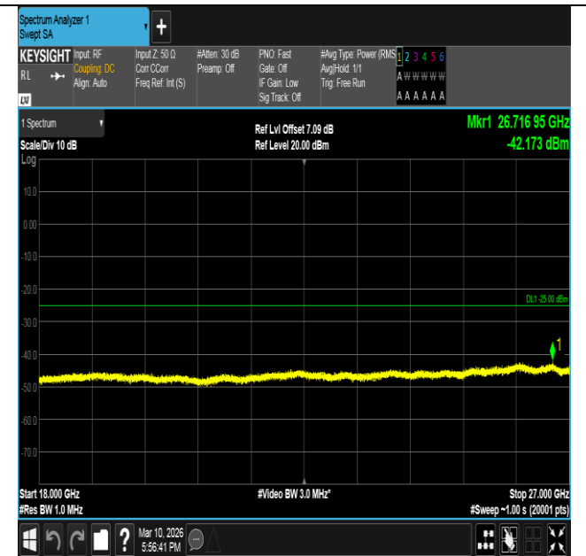
Band7-15MHz-16QAM-21100-75RB#0-18000~27000-PASS
