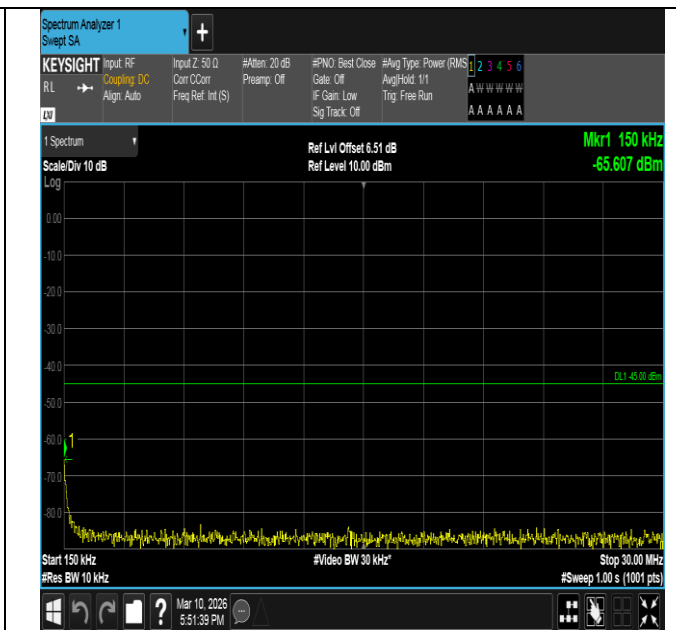
Band7-15MHz-16QAM-21100-1RB#0-0.15~30-PASS
