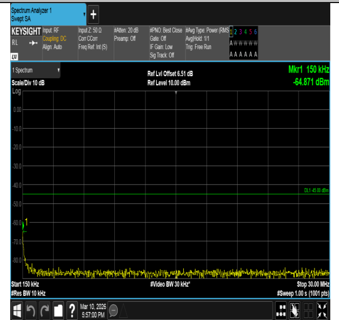
Band7-15MHz-QPSK-21375-1RB#0-0.15~30-PASS
