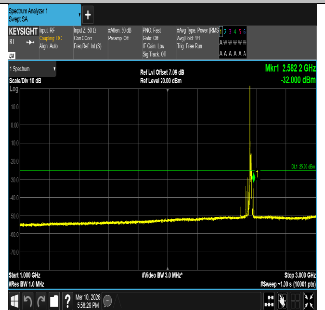
Band7-15MHz-16QAM-21375-1RB#0-1000~3000-PASS
