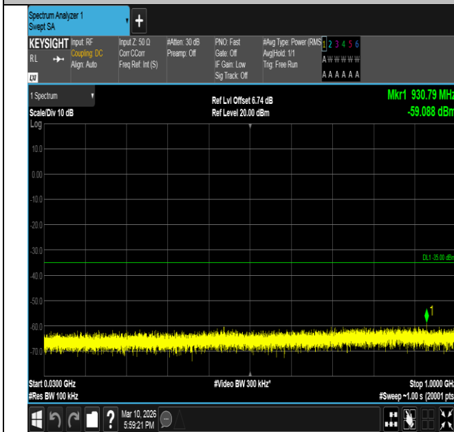
Band7-15MHz-QPSK-21375-1RB#74-30~1000-PASS
