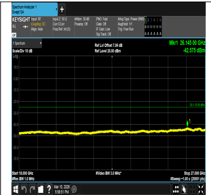
Band7-15MHz-16QAM-21375-1RB#0-18000~27000-PASS
