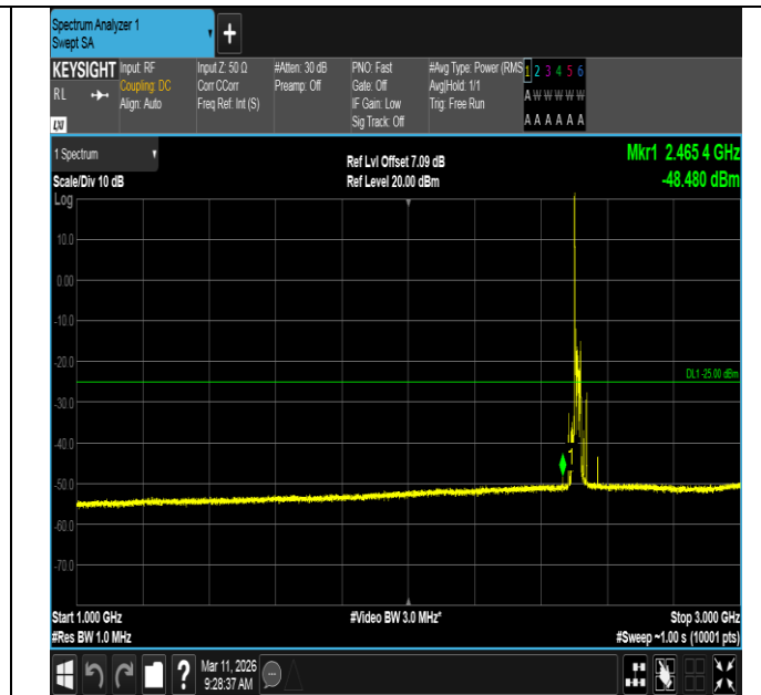
Band7-20MHz-QPSK-20850-1RB#0-1000~3000-PASS
