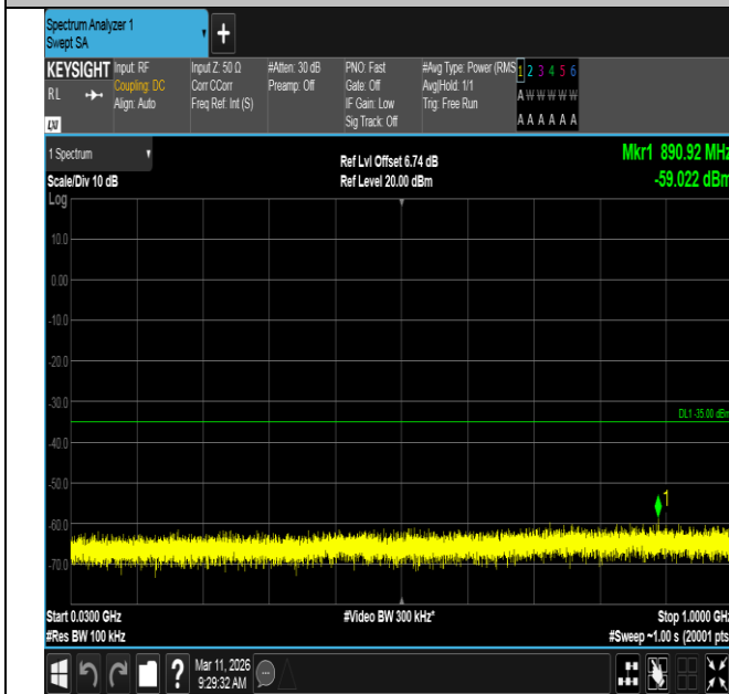
Band7-20MHz-16QAM-20850-1RB#0-30~1000-PASS
