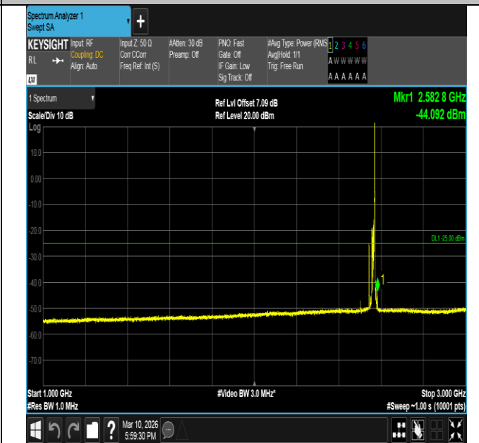
Band7-15MHz-QPSK-21375-1RB#74-1000~3000-PASS
