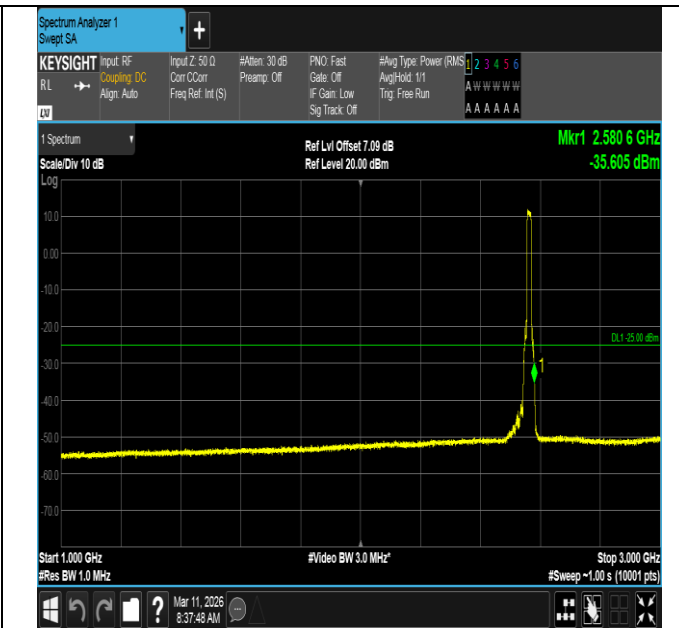
Band7-15MHz-QPSK-21375-75RB#0-1000~3000-PASS
