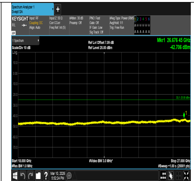
Band7-15MHz-16QAM-21100-1RB#0-18000~27000-PASS
