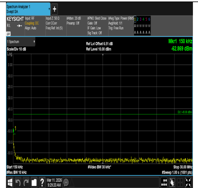
Band7-20MHz-16QAM-20850-1RB#0-0.15~30-PASS
