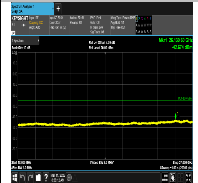
Band7-15MHz-QPSK-21375-75RB#0-18000~27000-PASS
