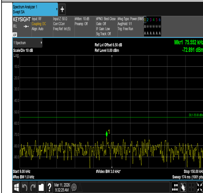
Band7-20MHz-QPSK-20850-100RB#0-0.009~0.15-PASS
