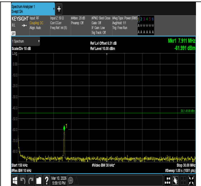
Band7-15MHz-QPSK-21375-1RB#74-0.15~30-PASS
