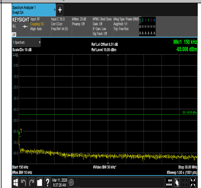
Band7-15MHz-QPSK-21375-75RB#0-0.15~30-PASS
