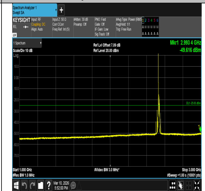
Band7-15MHz-16QAM-21100-1RB#0-1000~3000-PASS
