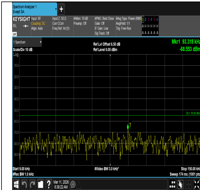
Band7-15MHz-16QAM-21375-75RB#0-0.009~0.15-PASS
