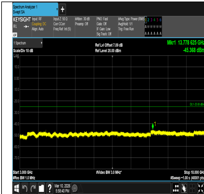
Band7-15MHz-16QAM-21375-1RB#0-3000~18000-PASS
