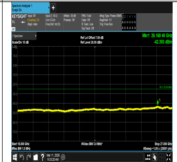
Band7-20MHz-QPSK-20850-100RB#0-18000~27000-PASS
