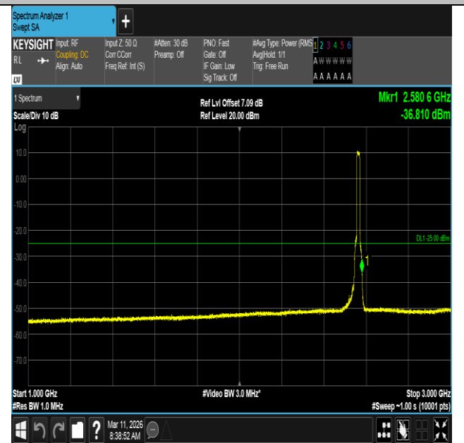
Band7-15MHz-16QAM-21375-75RB#0-1000~3000-PASS
