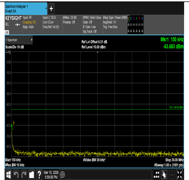
Band7-15MHz-16QAM-21375-1RB#0-0.15~30-PASS
