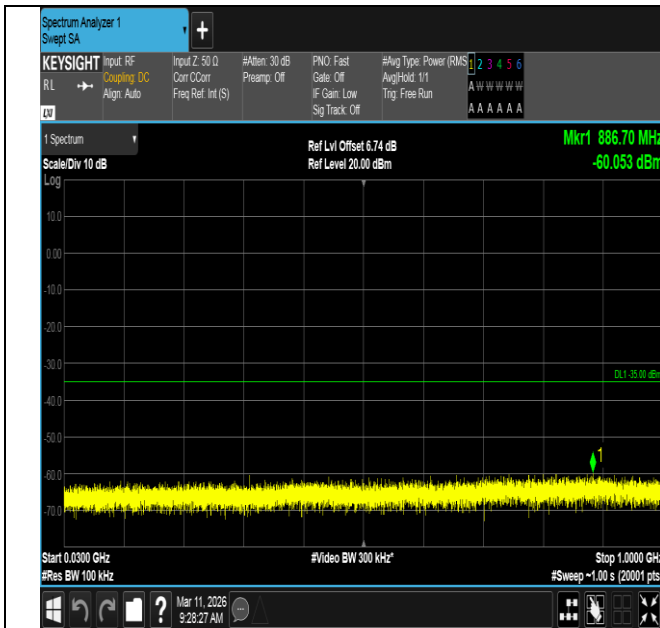
Band7-20MHz-QPSK-20850-1RB#0-30~1000-PASS
