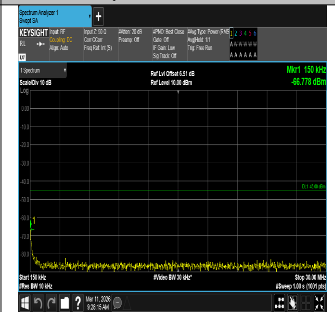
Band7-20MHz-QPSK-20850-1RB#0-0.15~30-PASS
