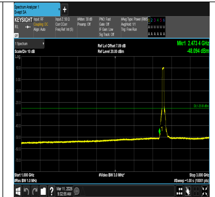
Band7-20MHz-QPSK-20850-100RB#0-1000~3000-PASS
