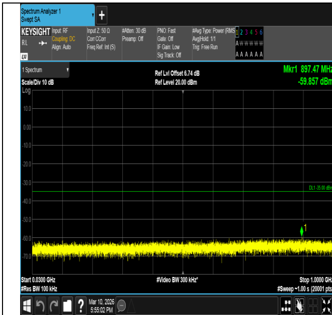
Band7-15MHz-QPSK-21100-75RB#0-30~1000-PASS
