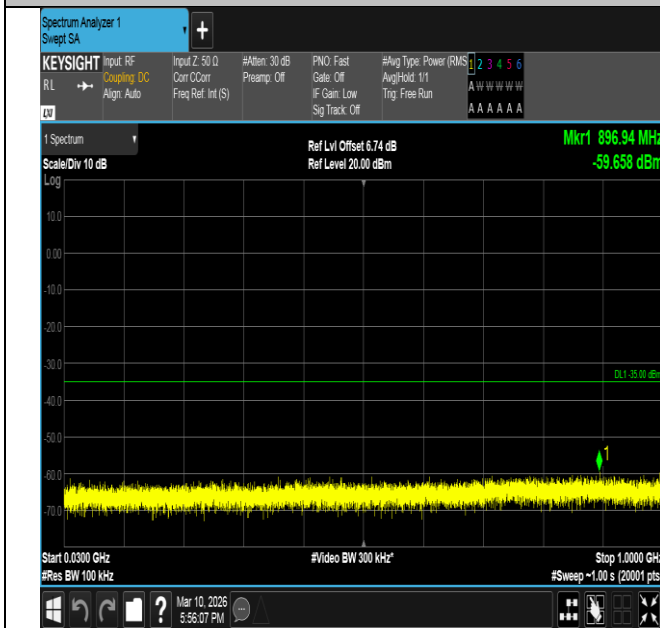
Band7-15MHz-16QAM-21100-75RB#0-30~1000-PASS
