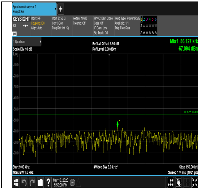
Band7-15MHz-QPSK-21375-1RB#74-0.009~0.15-PASS
