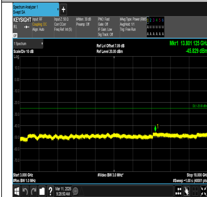
Band7-20MHz-QPSK-20850-1RB#0-3000~18000-PASS
