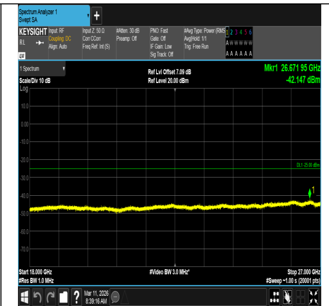
Band7-15MHz-16QAM-21375-75RB#0-18000~27000-PASS
