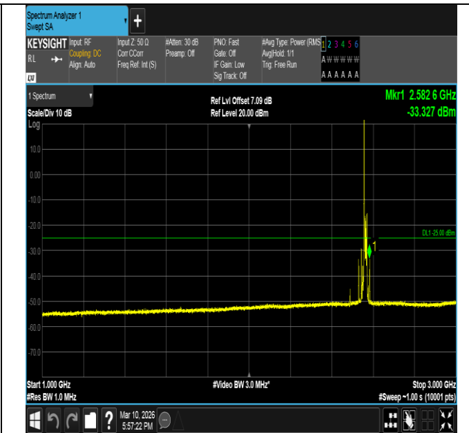
Band7-15MHz-QPSK-21375-1RB#0-1000~3000-PASS
