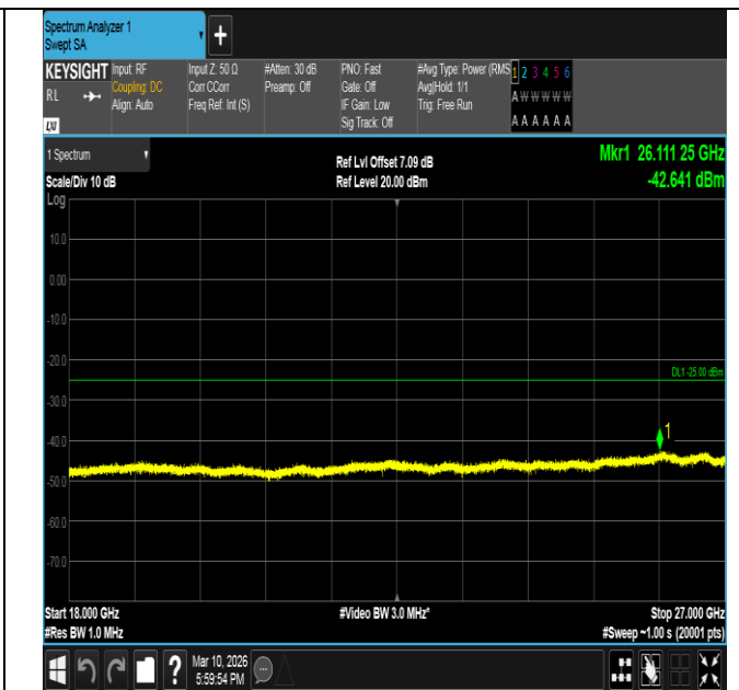
Band7-15MHz-QPSK-21375-1RB#74-18000~27000-PASS
