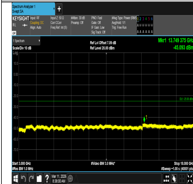
Band7-15MHz-QPSK-21375-75RB#0-3000~18000-PASS
