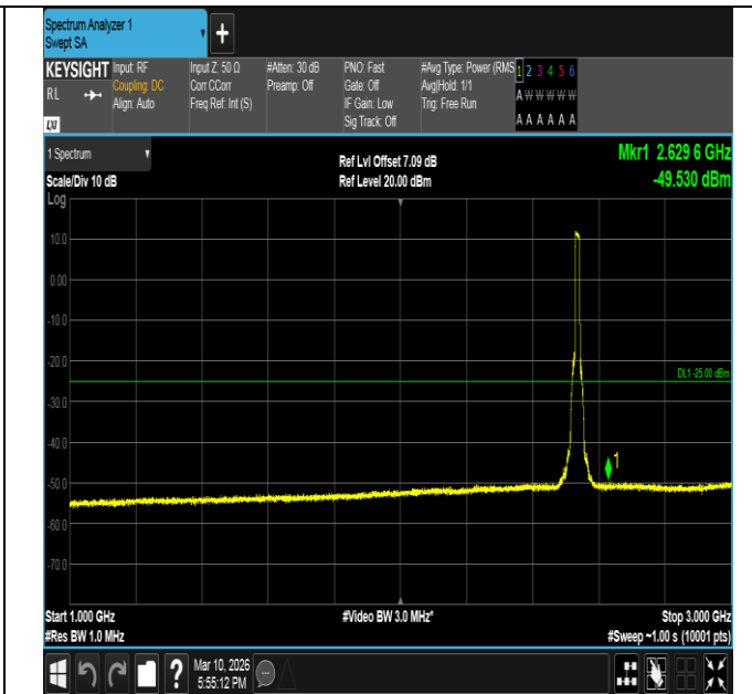
Band7-15MHz-QPSK-21100-75RB#0-1000~3000-PASS
