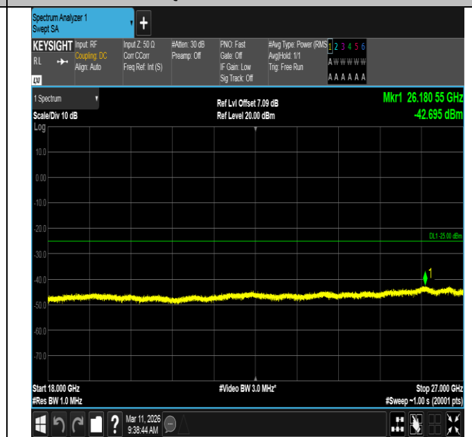
Band7-20MHz-16QAM-21100-1RB#99-18000~27000-PASS
