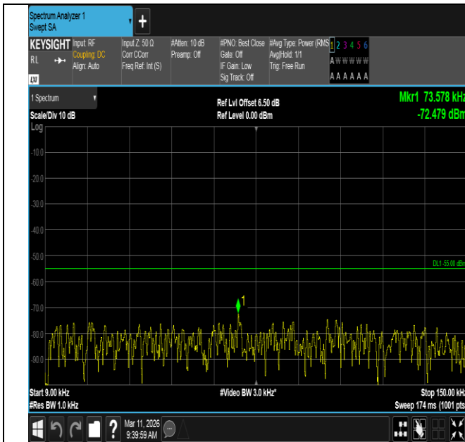
Band7-20MHz-16QAM-21100-100RB#0-0.009~0.15-PASS
