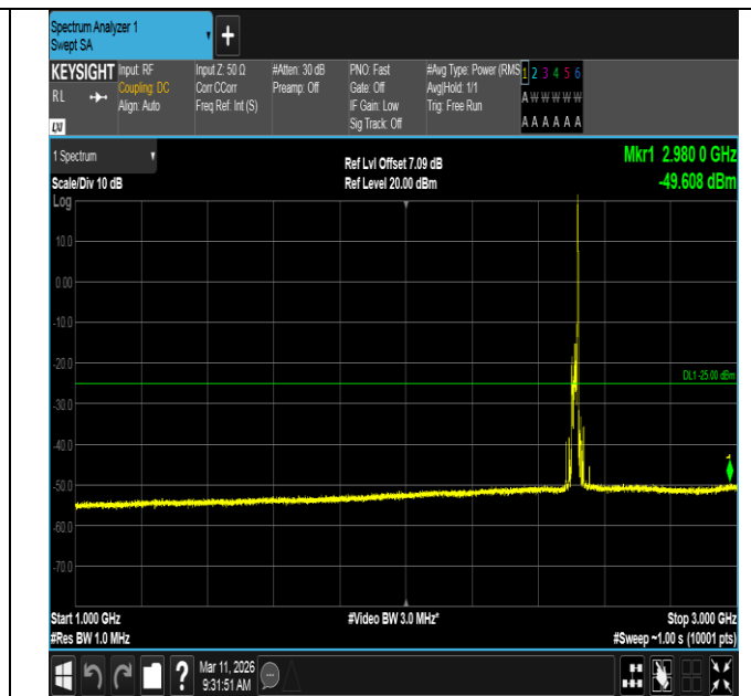
Band7-20MHz-16QAM-20850-1RB#99-1000~3000-PASS
