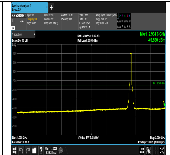
Band7-20MHz-QPSK-21100-100RB#0-1000~3000-PASS
