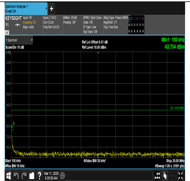
Band7-20MHz-16QAM-21100-1RB#0-0.15~30-PASS
