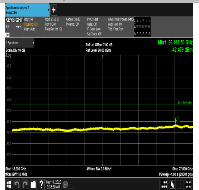
Band7-20MHz-QPSK-21100-1RB#0-18000~27000-PASS
