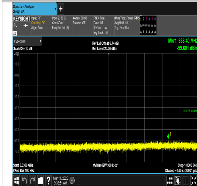
Band7-20MHz-16QAM-20850-100RB#0-30~1000-PASS
