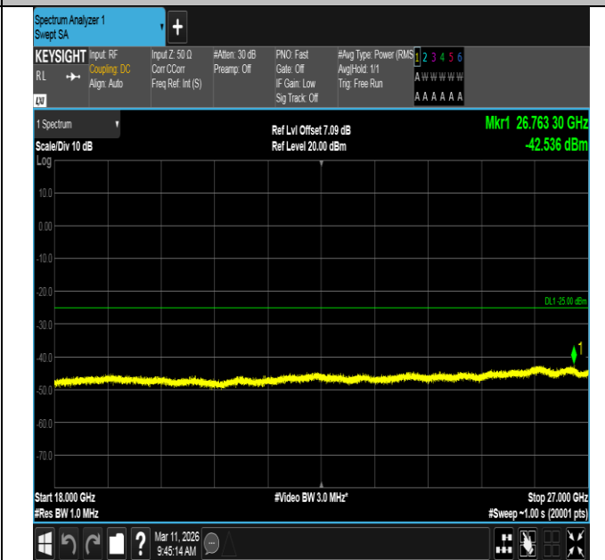
Band7-20MHz-16QAM-21350-1RB#99-18000~27000-PASS
