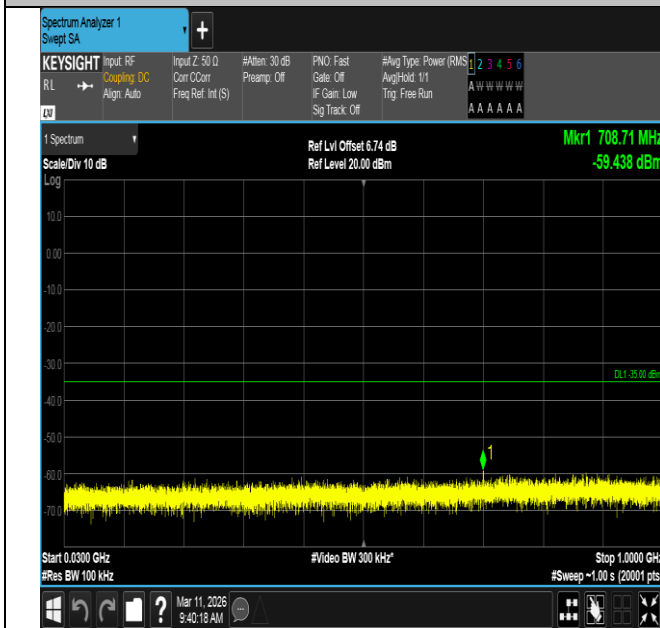
Band7-20MHz-16QAM-21100-100RB#0-30~1000-PASS
