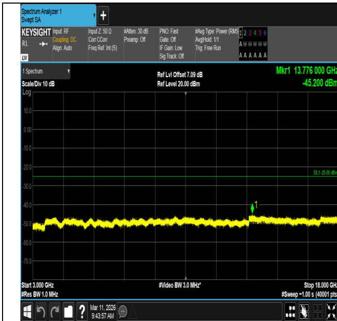
Band7-20MHz-QPSK-21350-1RB#99-3000~18000-PASS
