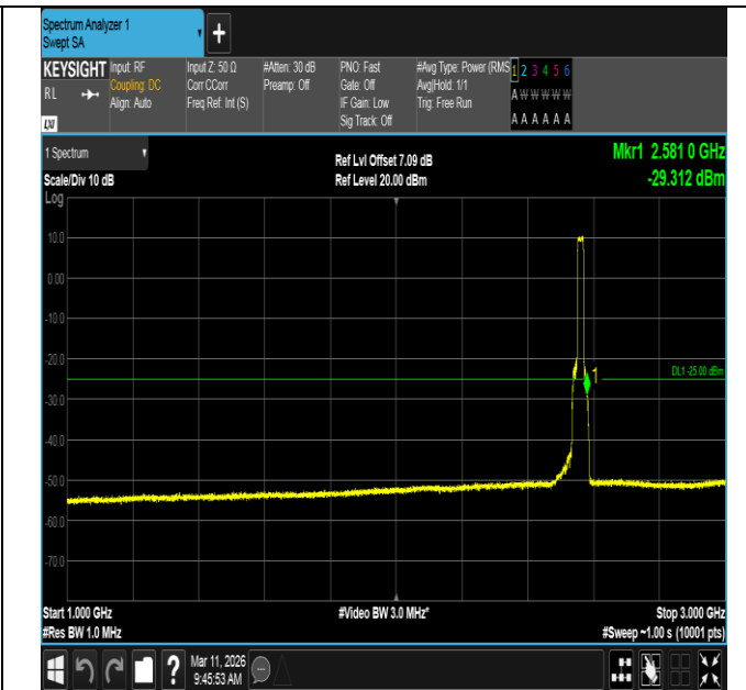
Band7-20MHz-QPSK-21350-100RB#0-1000~3000-PASS
