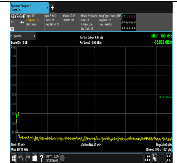
Band7-20MHz-16QAM-20850-100RB#0-0.15~30-PASS
