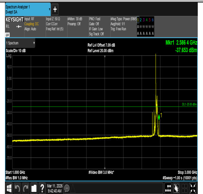
Band7-20MHz-16QAM-21350-1RB#0-1000~3000-PASS
