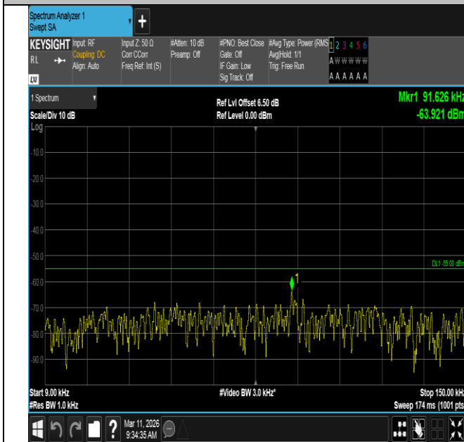
Band7-20MHz-QPSK-21100-1RB#0-0.009~0.15-PASS
