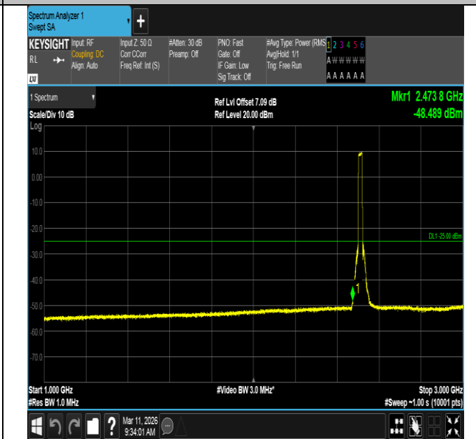
Band7-20MHz-16QAM-20850-100RB#0-1000~3000-PASS
