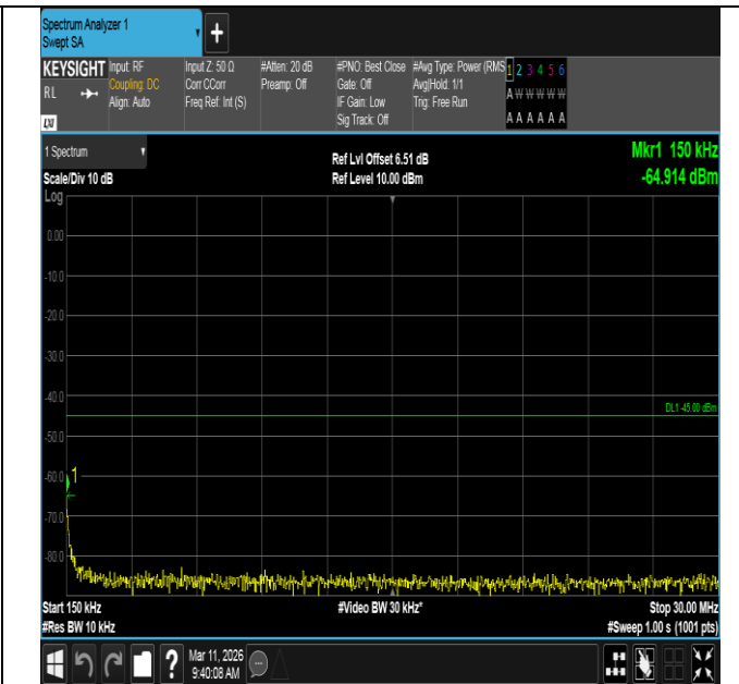
Band7-20MHz-16QAM-21100-100RB#0-0.15~30-PASS
