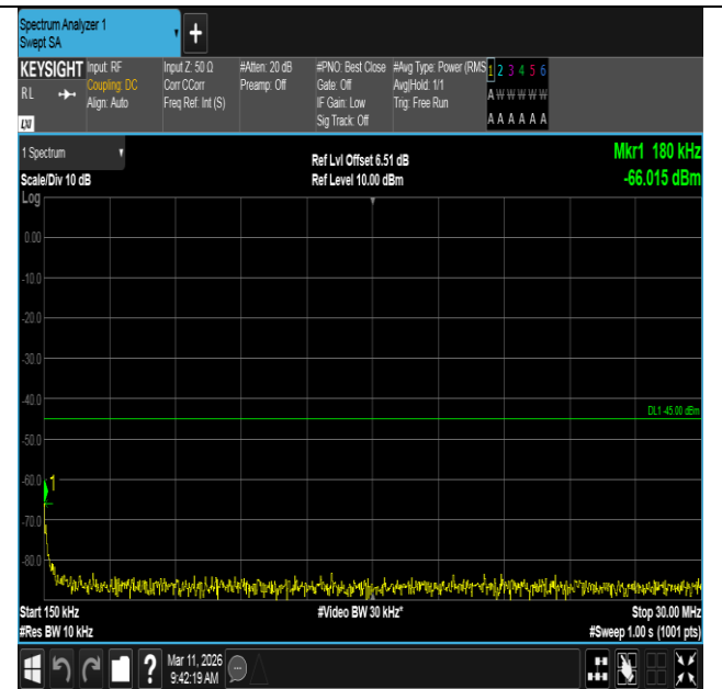
Band7-20MHz-16QAM-21350-1RB#0-0.15~30-PASS
