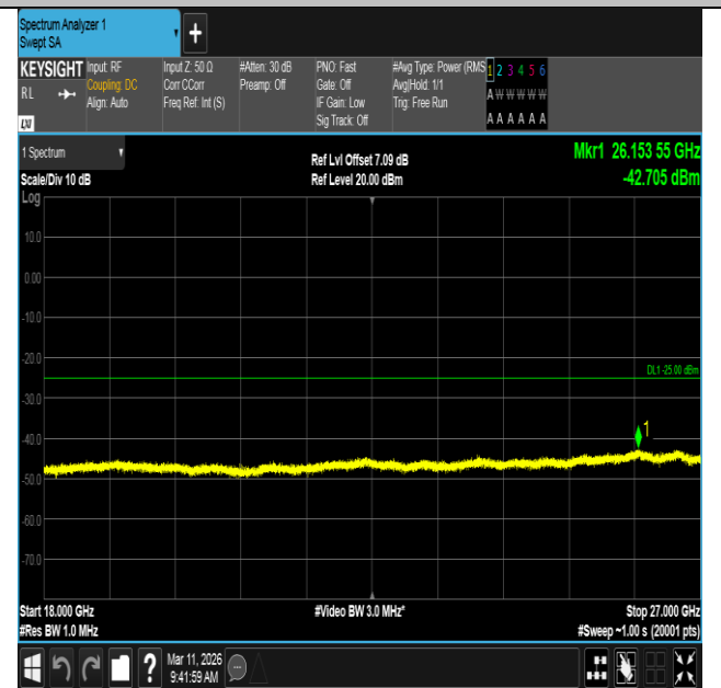
Band7-20MHz-QPSK-21350-1RB#0-18000~27000-PASS
