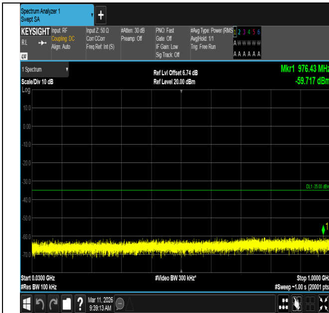
Band7-20MHz-QPSK-21100-100RB#0-30~1000-PASS
