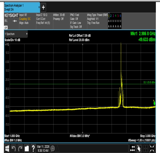
Band7-20MHz-16QAM-21100-1RB#0-1000~3000-PASS
