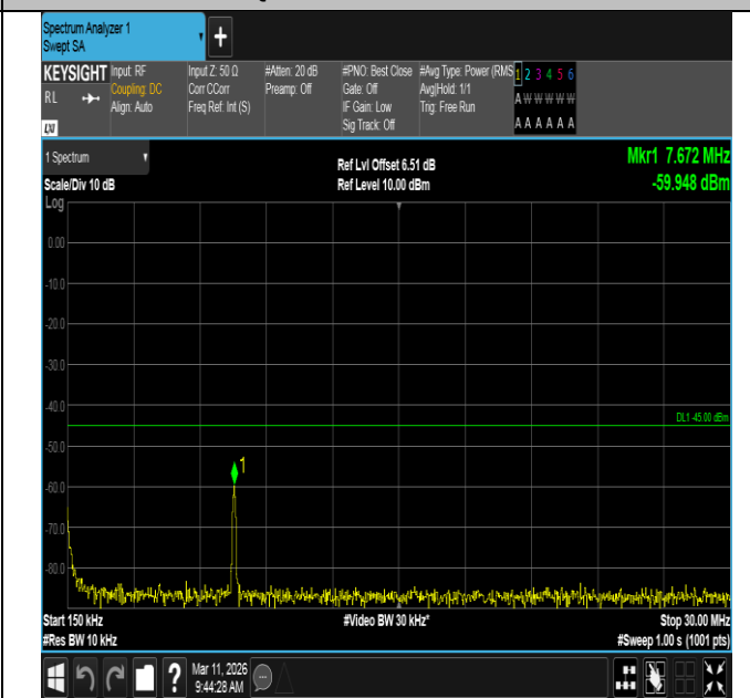
Band7-20MHz-16QAM-21350-1RB#99-0.15~30-PASS
