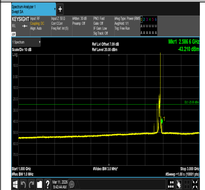
Band7-20MHz-QPSK-21350-1RB#99-1000~3000-PASS
