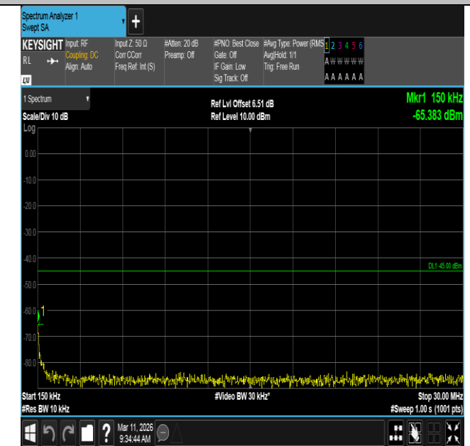
Band7-20MHz-QPSK-21100-1RB#0-0.15~30-PASS
