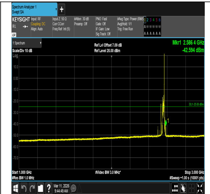
Band7-20MHz-16QAM-21350-1RB#99-1000~3000-PASS
