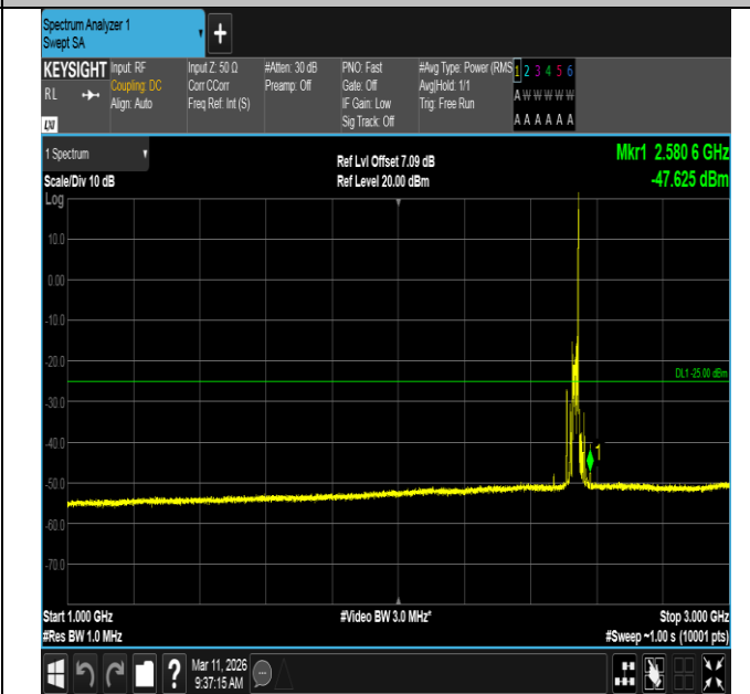
Band7-20MHz-QPSK-21100-1RB#99-1000~3000-PASS
