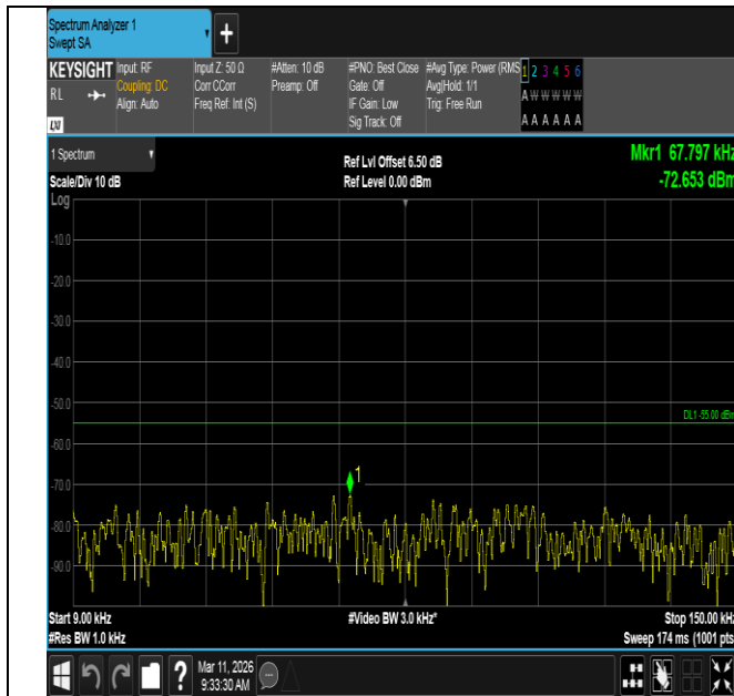
Band7-20MHz-16QAM-20850-100RB#0-0.009~0.15-PASS
