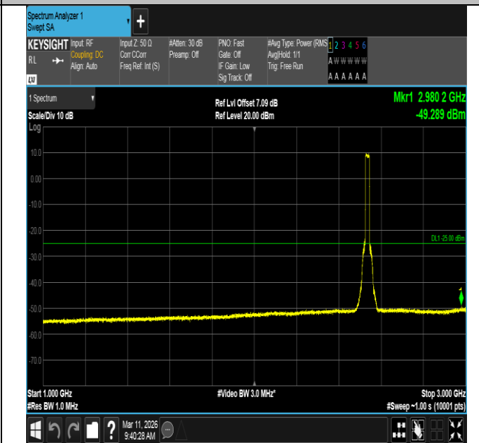
Band7-20MHz-16QAM-21100-100RB#0-1000~3000-PASS
