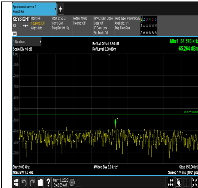
Band7-20MHz-16QAM-21350-1RB#0-0.009~0.15-PASS
