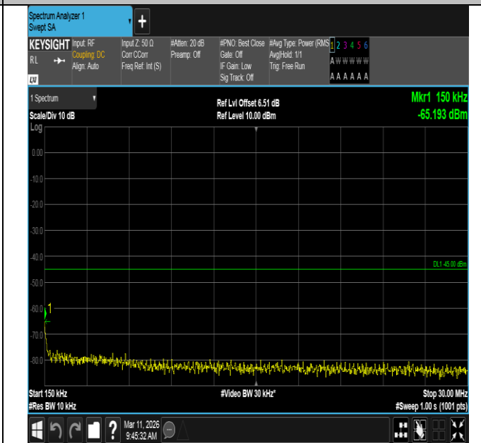
Band7-20MHz-QPSK-21350-100RB#0-0.15~30-PASS
