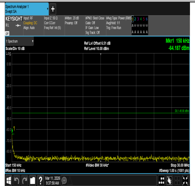
Band7-20MHz-16QAM-21100-1RB#99-0.15~30-PASS
