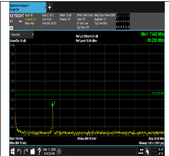
Band7-20MHz-QPSK-21350-1RB#99-0.15~30-PASS
