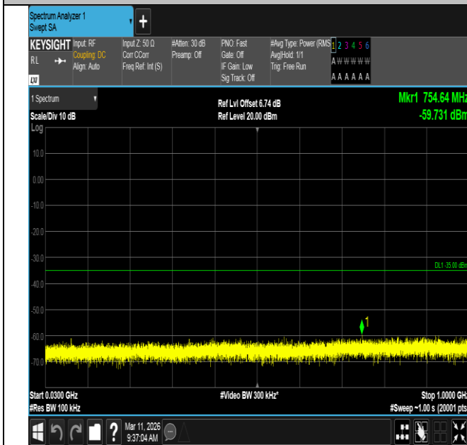
Band7-20MHz-QPSK-21100-1RB#99-30~1000-PASS
