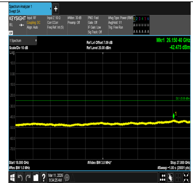
Band7-20MHz-16QAM-20850-100RB#0-18000~27000-PASS
