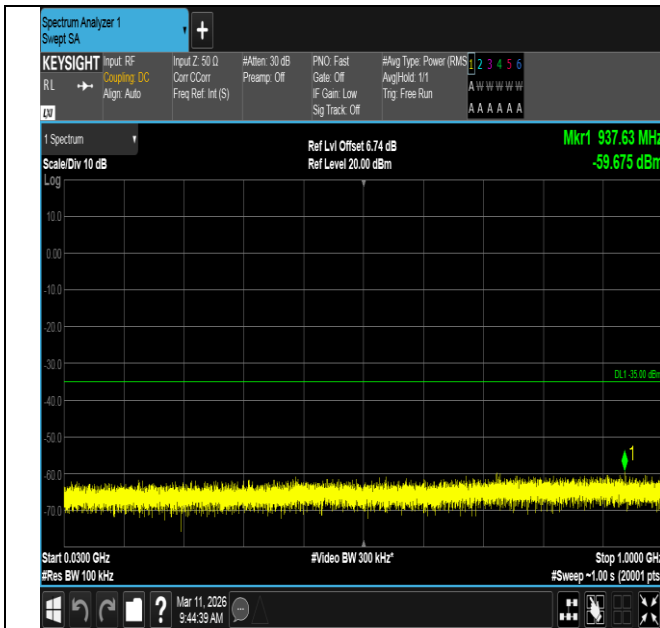
Band7-20MHz-16QAM-21350-1RB#99-30~1000-PASS
