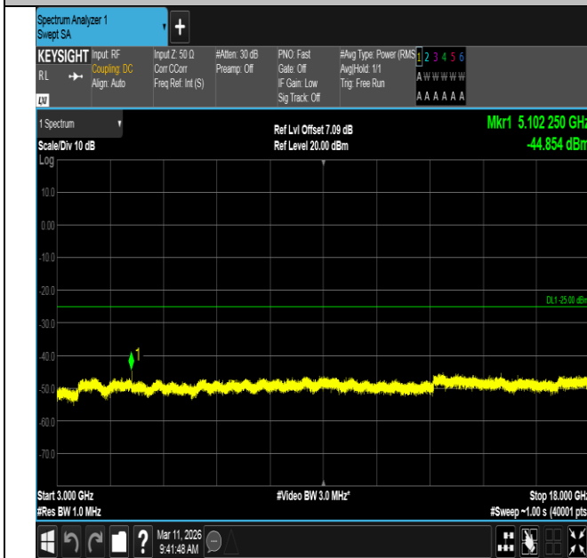
Band7-20MHz-QPSK-21350-1RB#0-3000~18000-PASS
