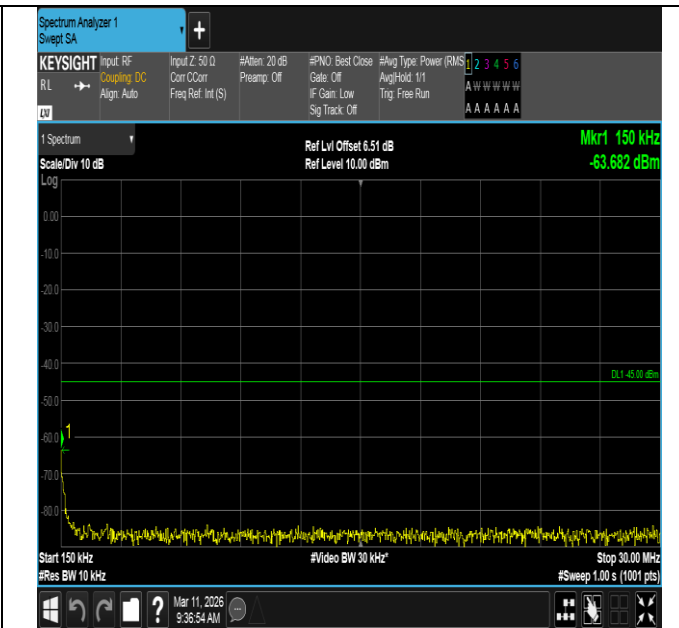
Band7-20MHz-QPSK-21100-1RB#99-0.15~30-PASS
