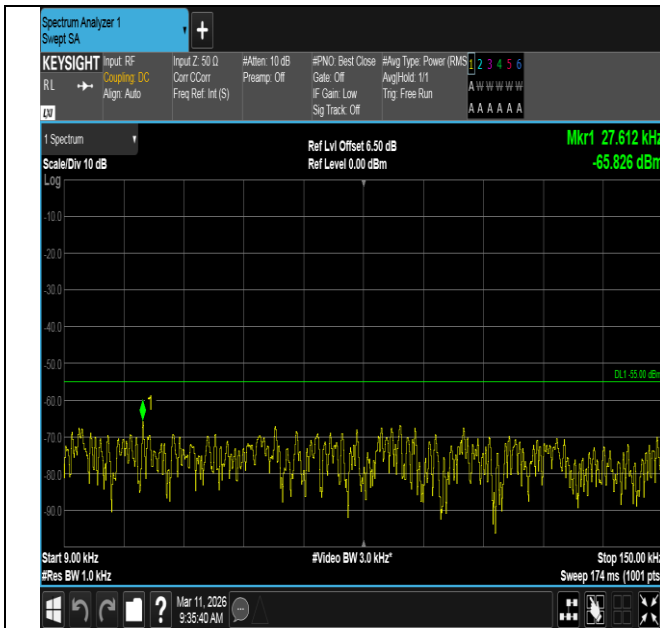
Band7-20MHz-16QAM-21100-1RB#0-0.009~0.15-PASS
