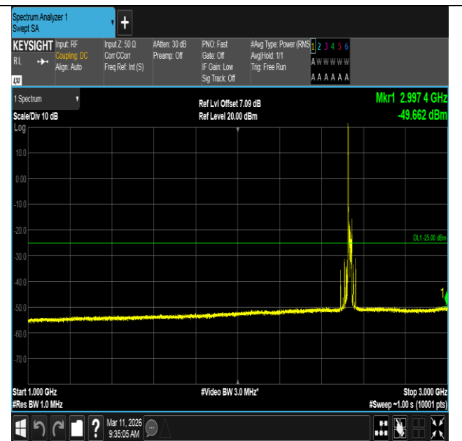
Band7-20MHz-QPSK-21100-1RB#0-1000~3000-PASS
