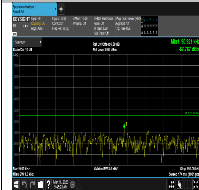
Band7-20MHz-QPSK-21350-100RB#0-0.009~0.15-PASS
