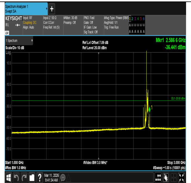
Band7-20MHz-QPSK-21350-1RB#0-1000~3000-PASS
