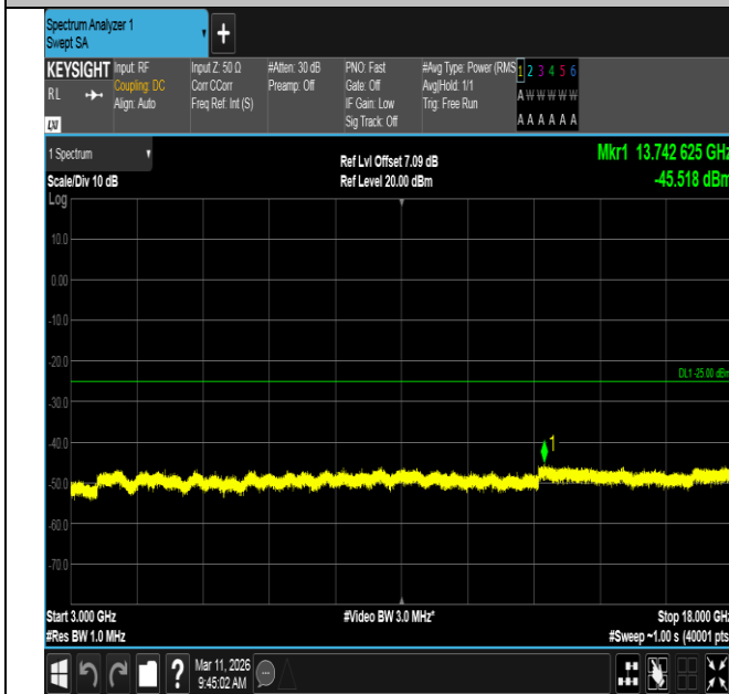
Band7-20MHz-16QAM-21350-1RB#99-3000~18000-PASS
