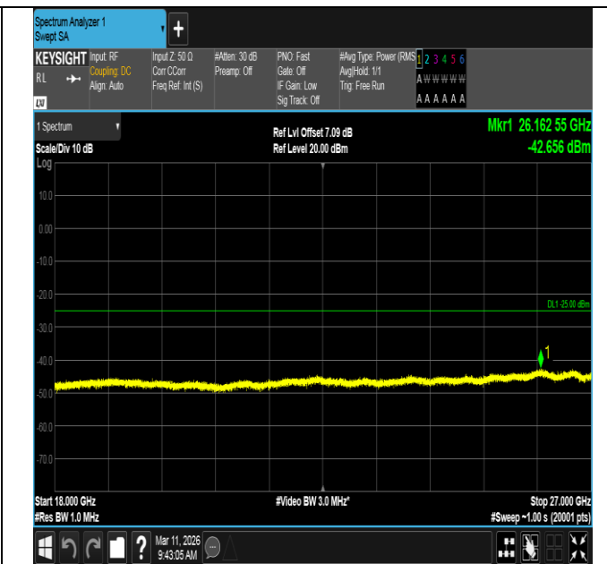
Band7-20MHz-16QAM-21350-1RB#0-18000~27000-PASS
