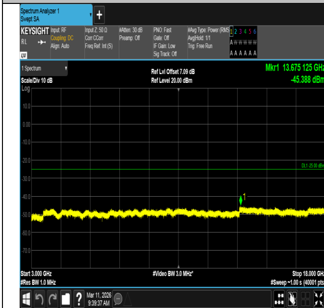
Band7-20MHz-QPSK-21100-100RB#0-3000~18000-PASS
