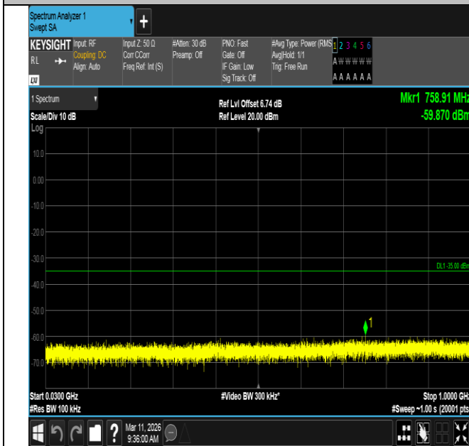
Band7-20MHz-16QAM-21100-1RB#0-30~1000-PASS
