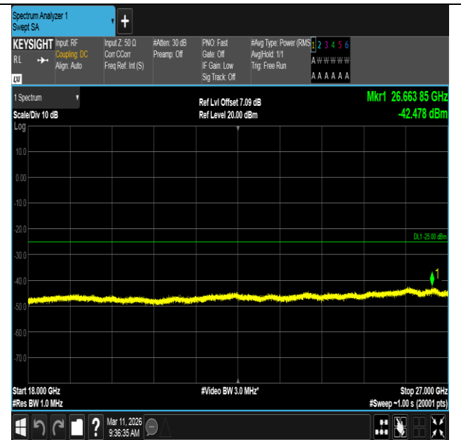
Band7-20MHz-16QAM-21100-1RB#0-18000~27000-PASS
