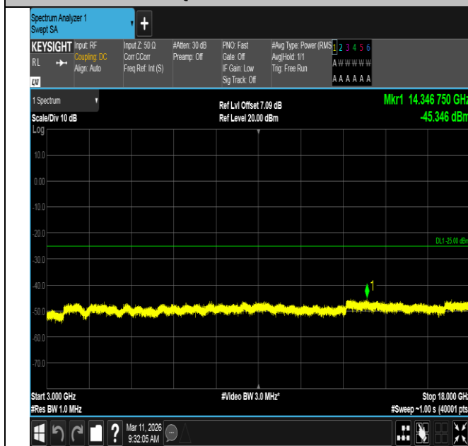
Band7-20MHz-16QAM-20850-1RB#99-3000~18000-PASS
