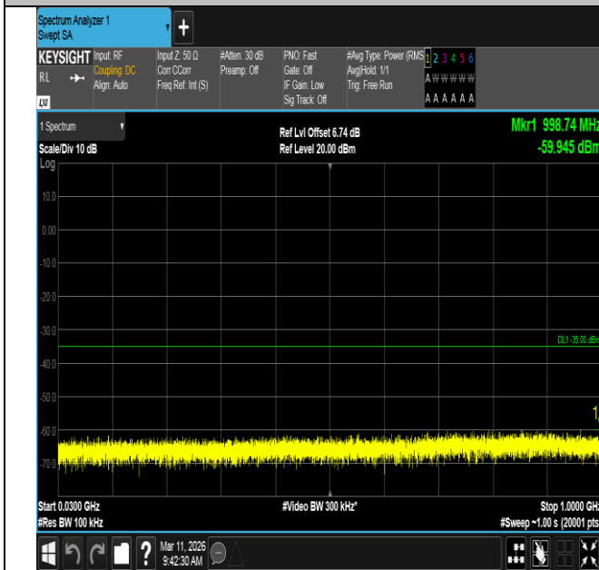
Band7-20MHz-16QAM-21350-1RB#0-30~1000-PASS
