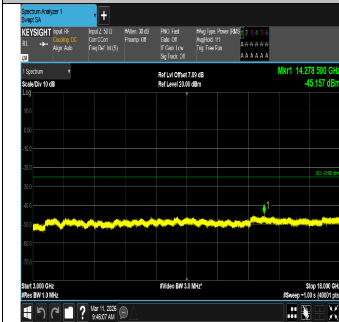
Band7-20MHz-QPSK-21350-100RB#0-3000~18000-PASS
