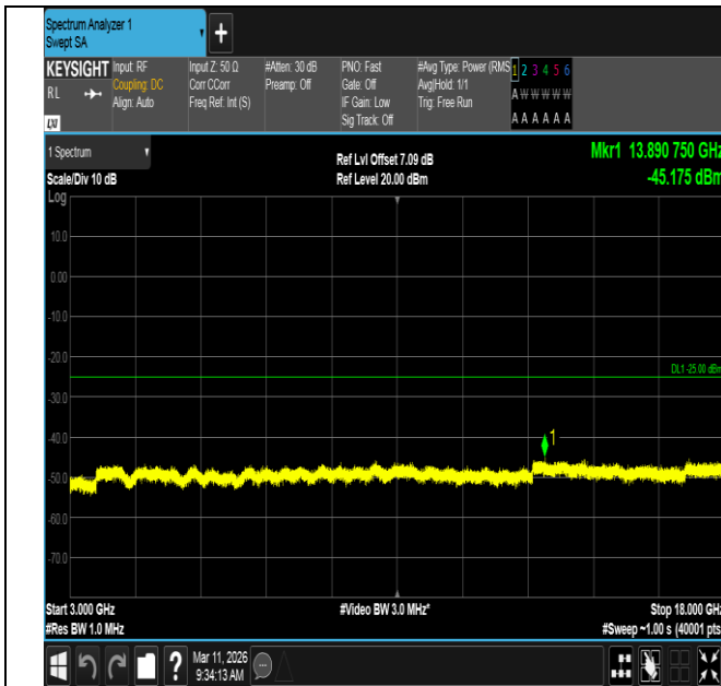
Band7-20MHz-16QAM-20850-100RB#0-3000~18000-PASS
