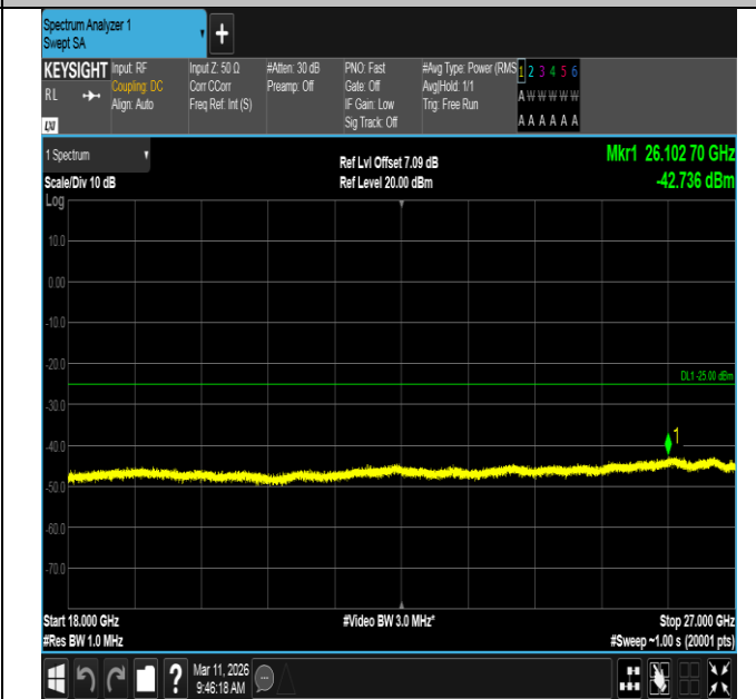
Band7-20MHz-QPSK-21350-100RB#0-18000~27000-PASS
