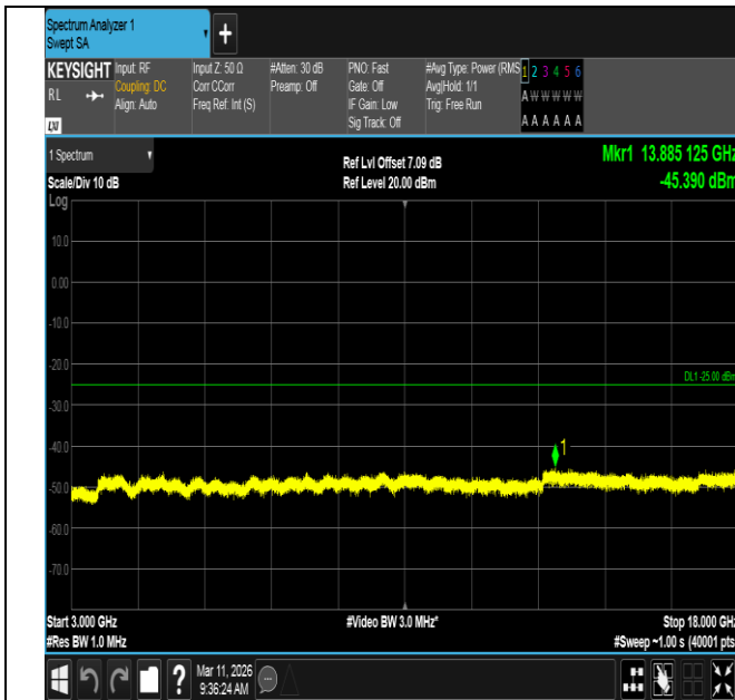
Band7-20MHz-16QAM-21100-1RB#0-3000~18000-PASS
