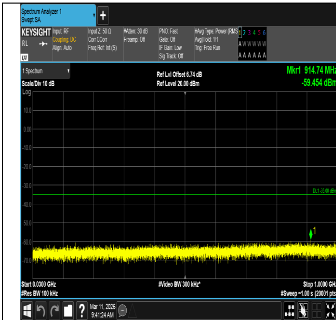
Band7-20MHz-QPSK-21350-1RB#0-30~1000-PASS
