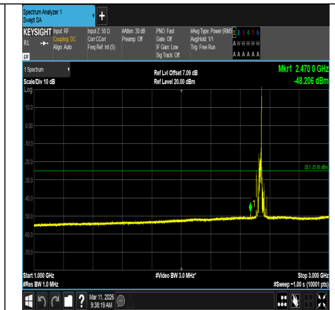
Band7-20MHz-16QAM-21100-1RB#99-1000~3000-PASS
