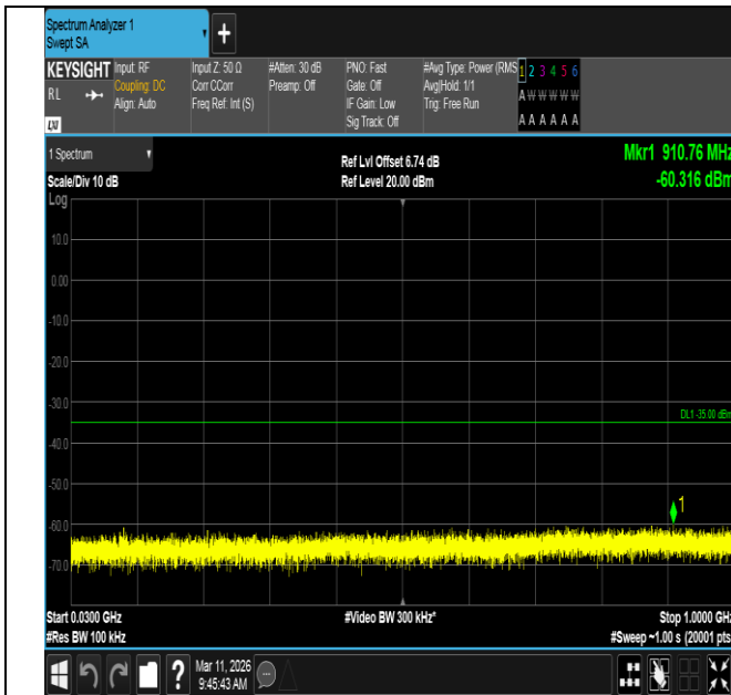
Band7-20MHz-QPSK-21350-100RB#0-30~1000-PASS
