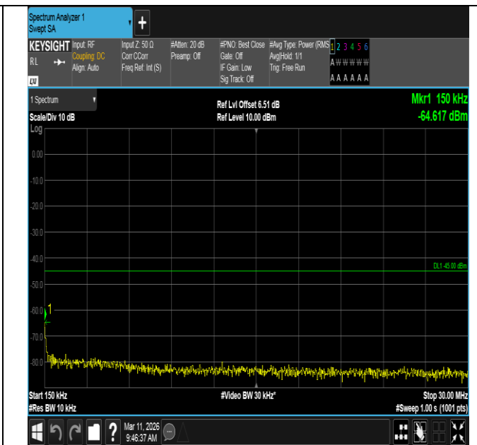
Band7-20MHz-16QAM-21350-100RB#0-0.15~30-PASS
