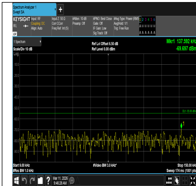
Band7-20MHz-16QAM-21350-100RB#0-0.009~0.15-PASS
