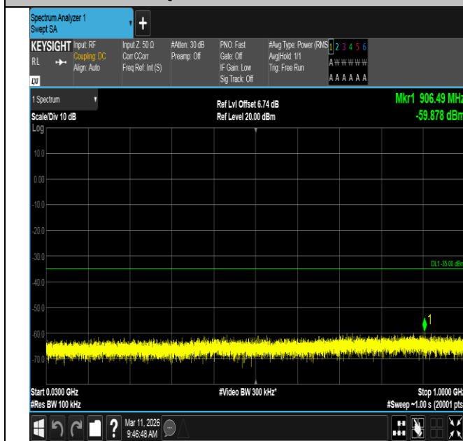
Band7-20MHz-16QAM-21350-100RB#0-30~1000-PASS
