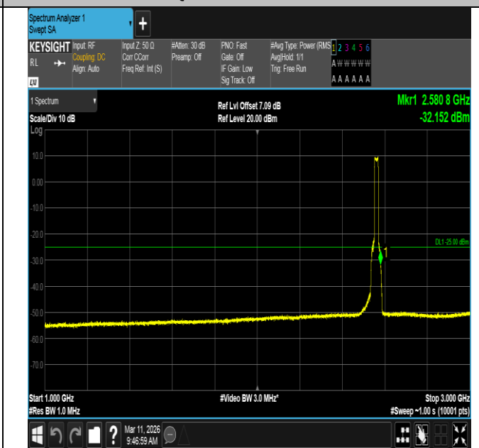
Band7-20MHz-16QAM-21350-100RB#0-1000~3000-PASS
