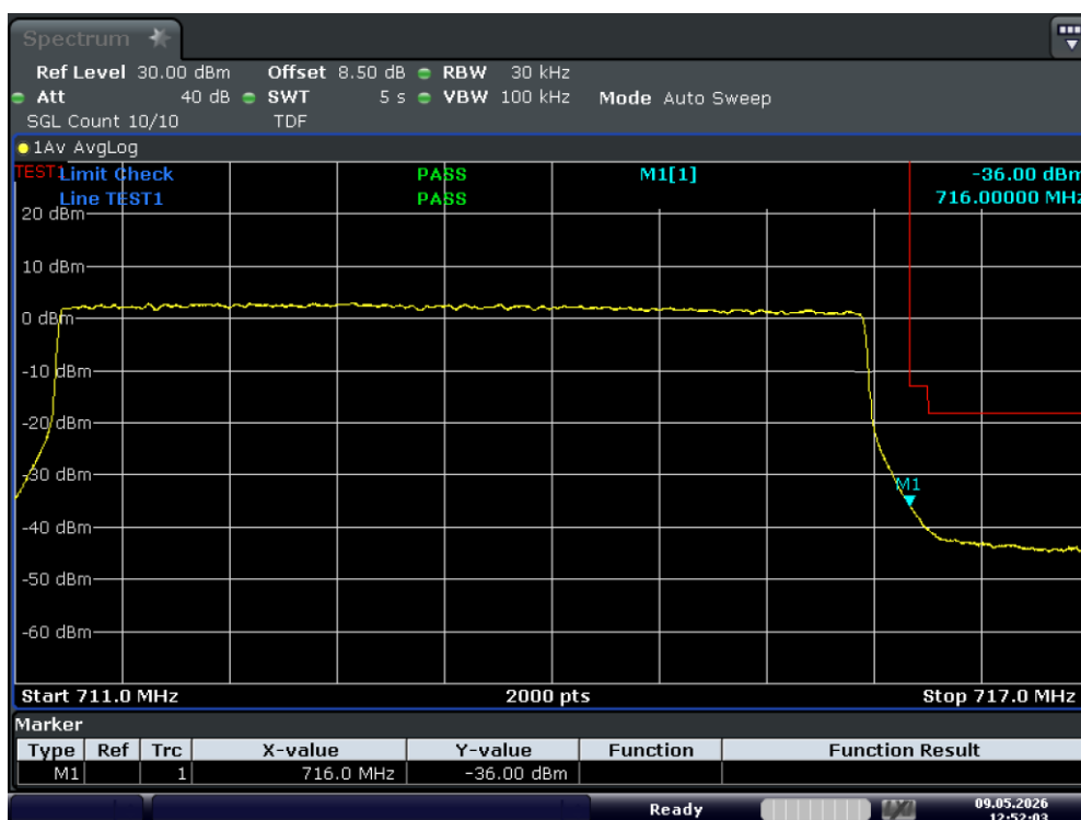
Test_Graph_band17_713.5MHz_5M_QPSK_1RB#HIGH_Band edge
