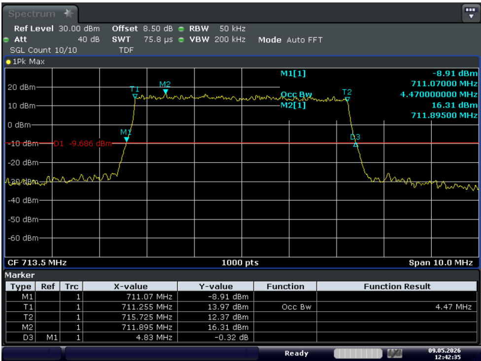
Test_Graph_band17_713.5MHz_5M_16QAM_25RB#LOW_OBW&EBW
