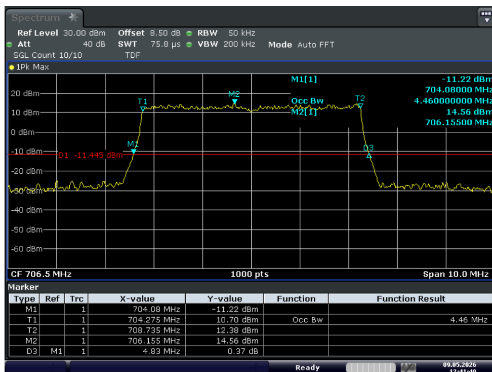
Test_Graph_band17_706.5MHz_5M_16QAM_25RB#LOW_OBW&EBW
