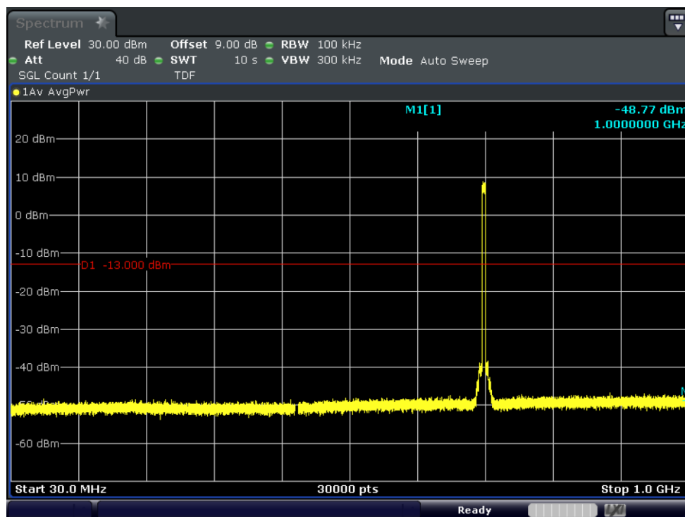
Test_Graph_band17_706.5MHz_5M_QPSK_25RB#LOW_30M_1G_TX
