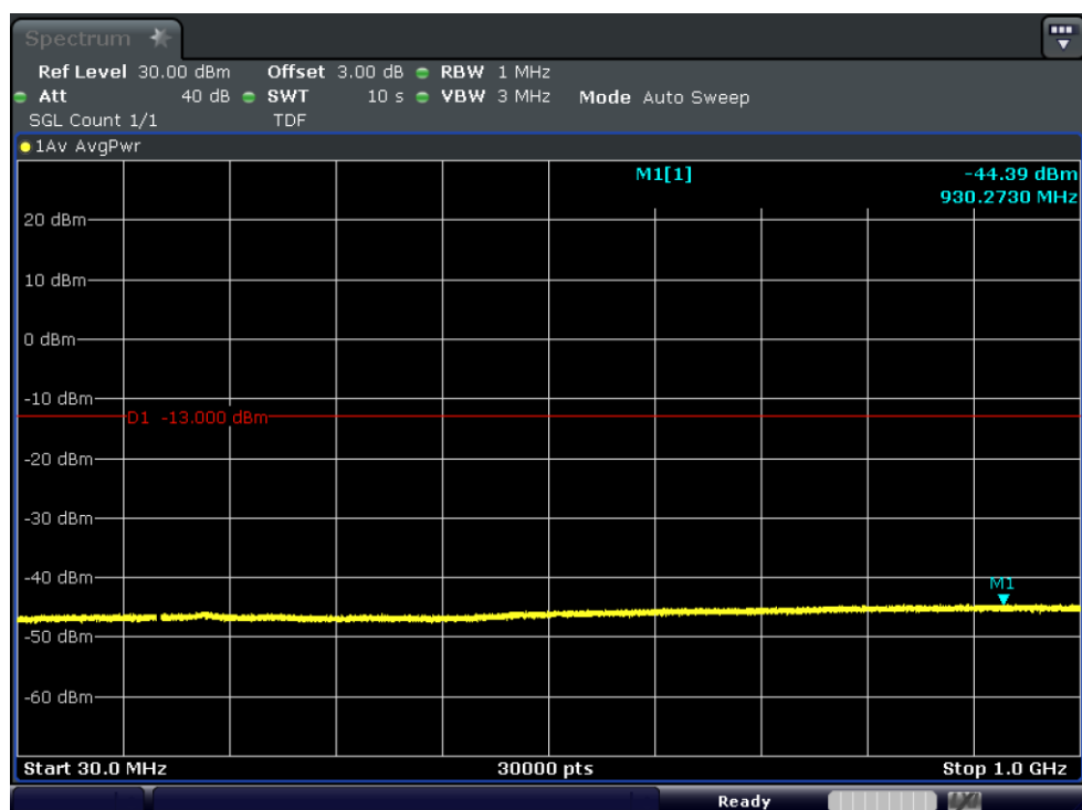
Test_Graph_band2_1857.5MHz_15M_QPSK_75RB#LOW_30M_1G_TX
