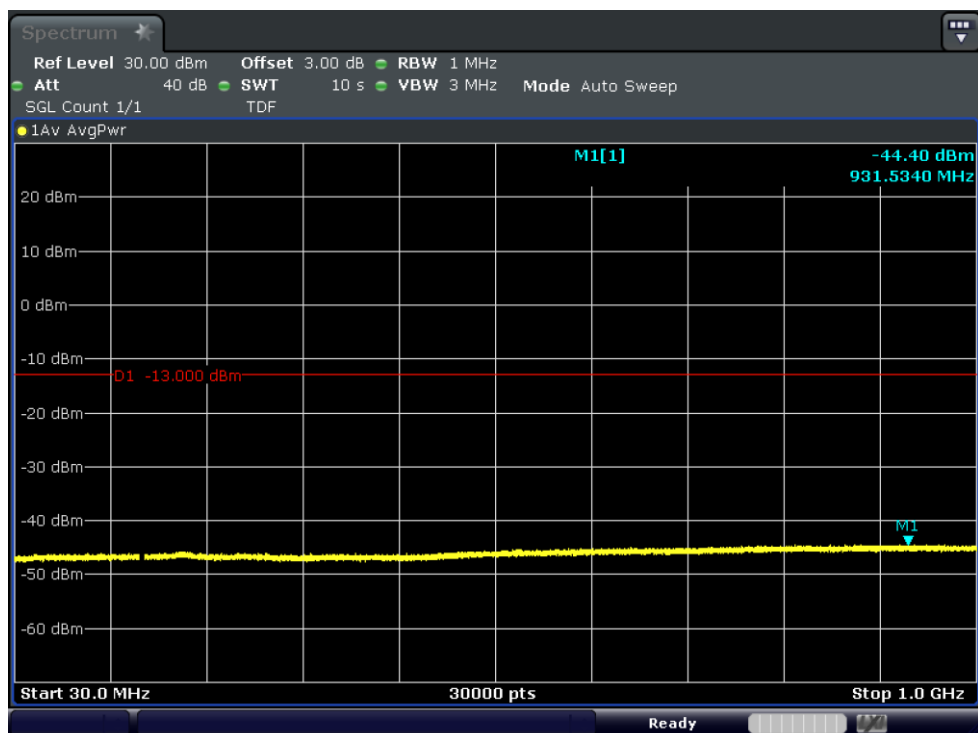
Test_Graph_band2_1907.5MHz_5M_QPSK_25RB#LOW_30M_1G_TX
