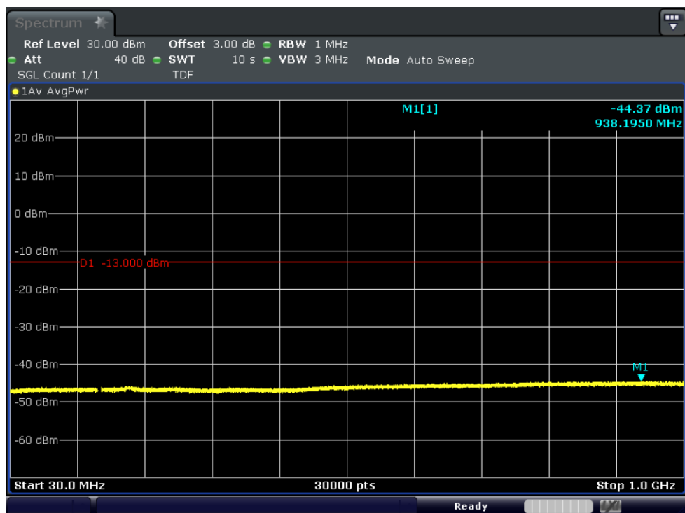
Test_Graph_band2_1902.5MHz_15M_QPSK_75RB#LOW_30M_1G_TX
