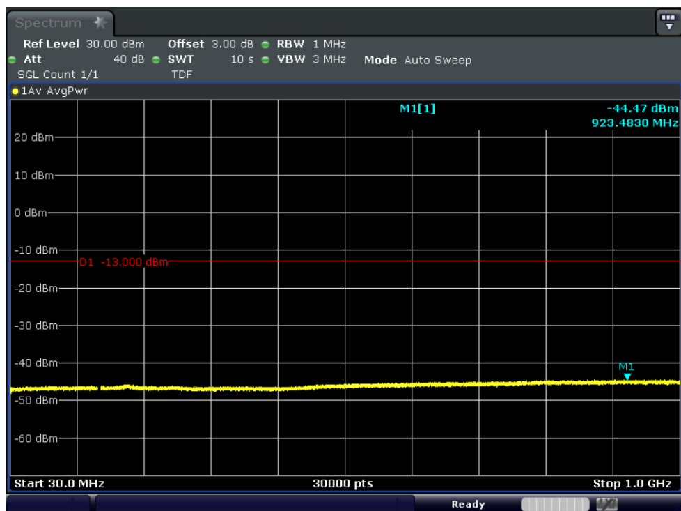
Test_Graph_band2_1909.3MHz_1.4M_QPSK_6RB#LOW_30M_1G_TX
