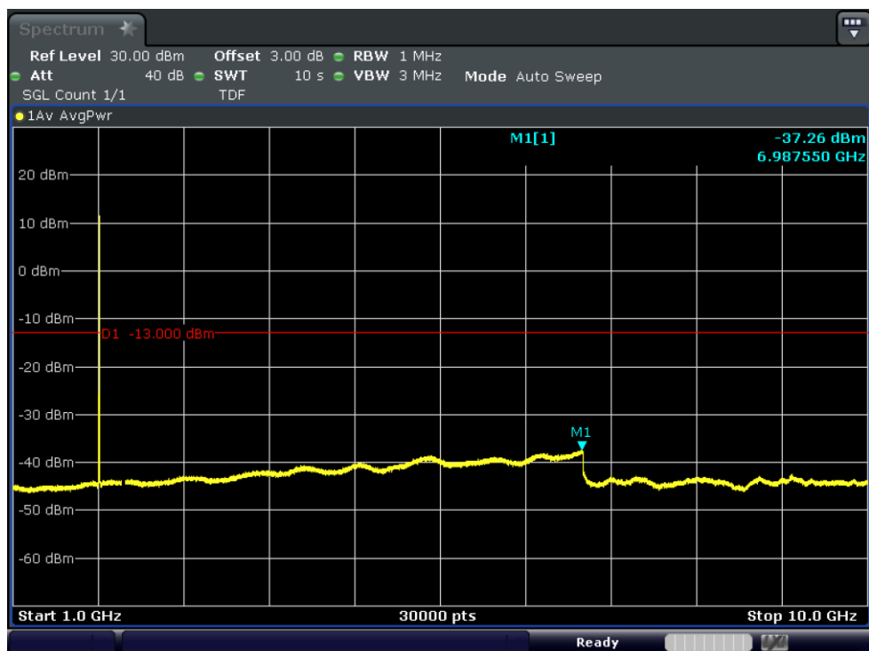
Test_Graph_band2_1908.5MHz_3M_QPSK_15RB#LOW_1G_10G_TX
