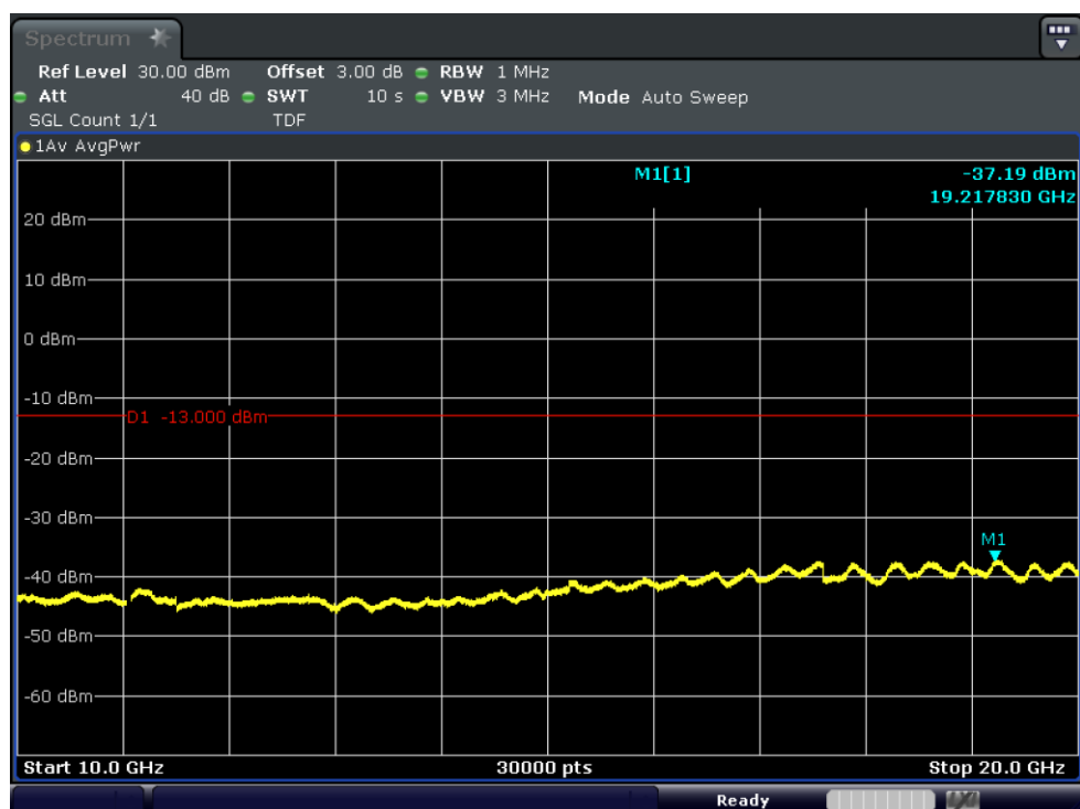
Test_Graph_band2_1902.5MHz_15M_QPSK_75RB#LOW_10G_20.0G_TX
