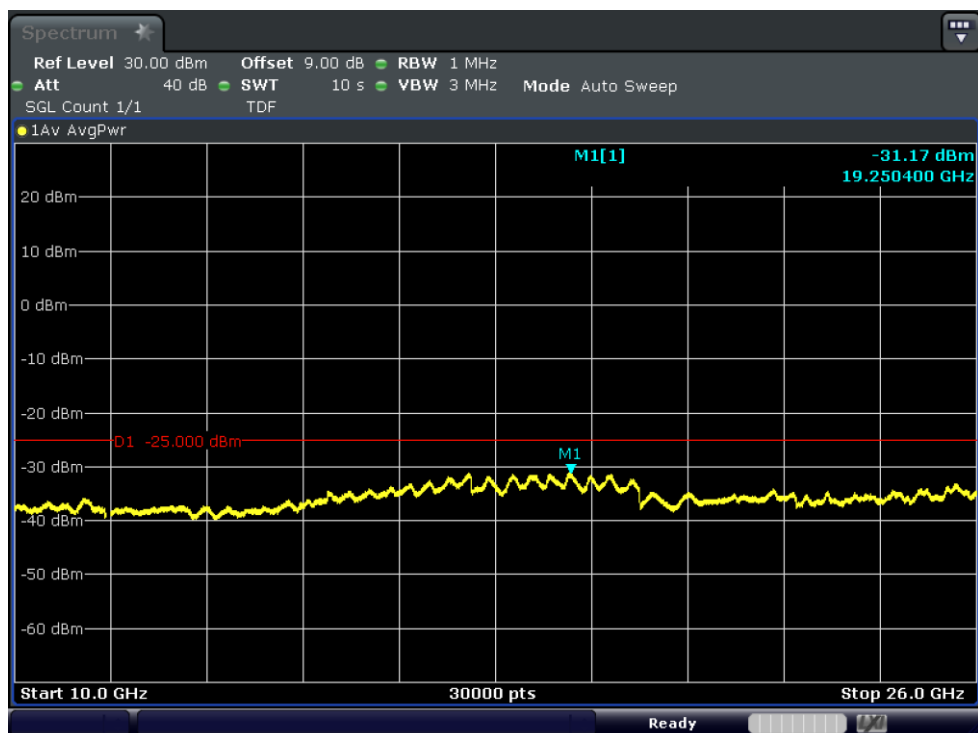
Test_Graph_band38_2595MHz_20M_QPSK_100RB#LOW_10G_26.0G_TX
