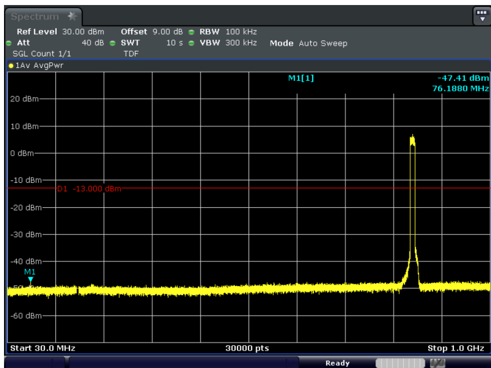
Test_Graph_band5_844MHz_10M_QPSK_50RB#LOW_30M_1G_TX
