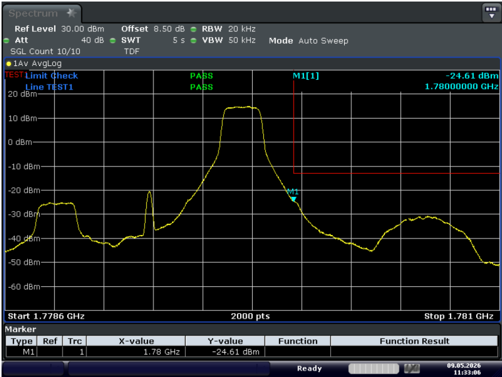
Test_Graph_band66_1779.3MHz_1.4M_QPSK_1RB#HIGH_Band edge
