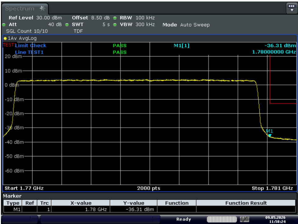
Test_Graph_band66_1775MHz_10M_QPSK_1RB#HIGH_Band edge
