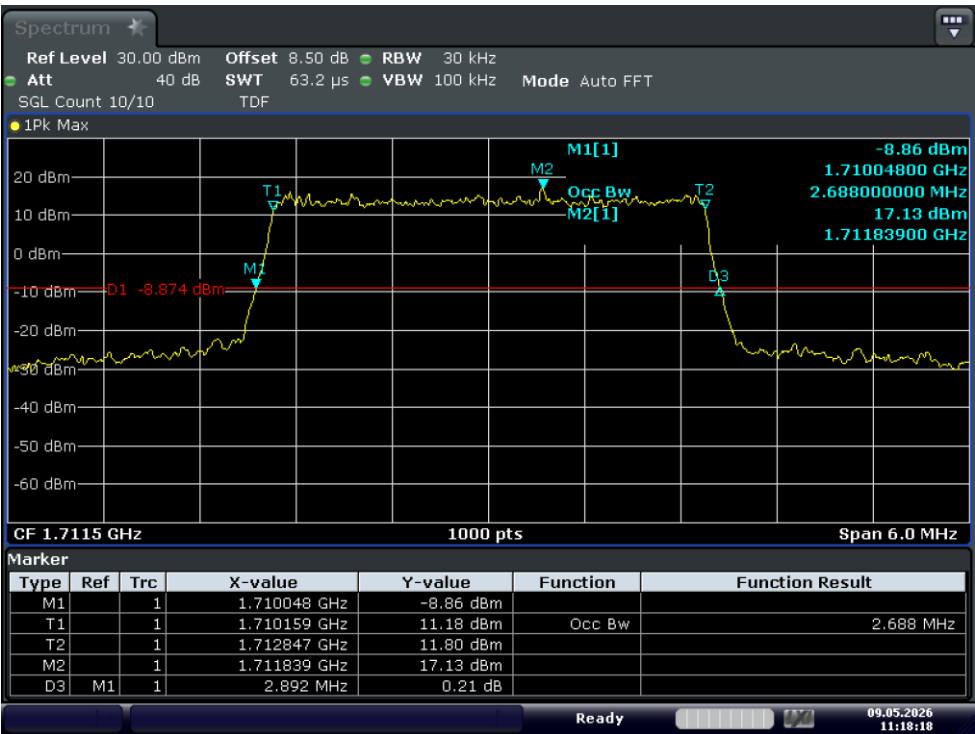
Test_Graph_band66_1711.5MHz_3M_16QAM_15RB#LOW_OBW&EBW
