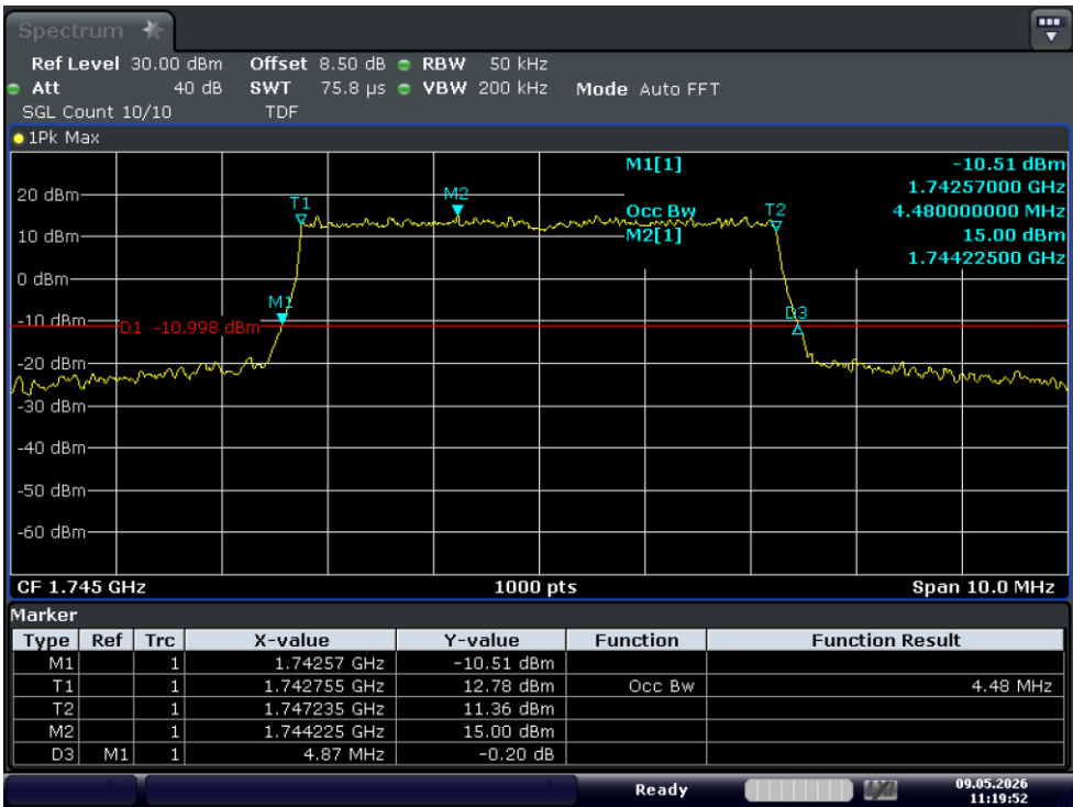
Test_Graph_band66_1745MHz_5M_16QAM_25RB#LOW_OBW&EBW
