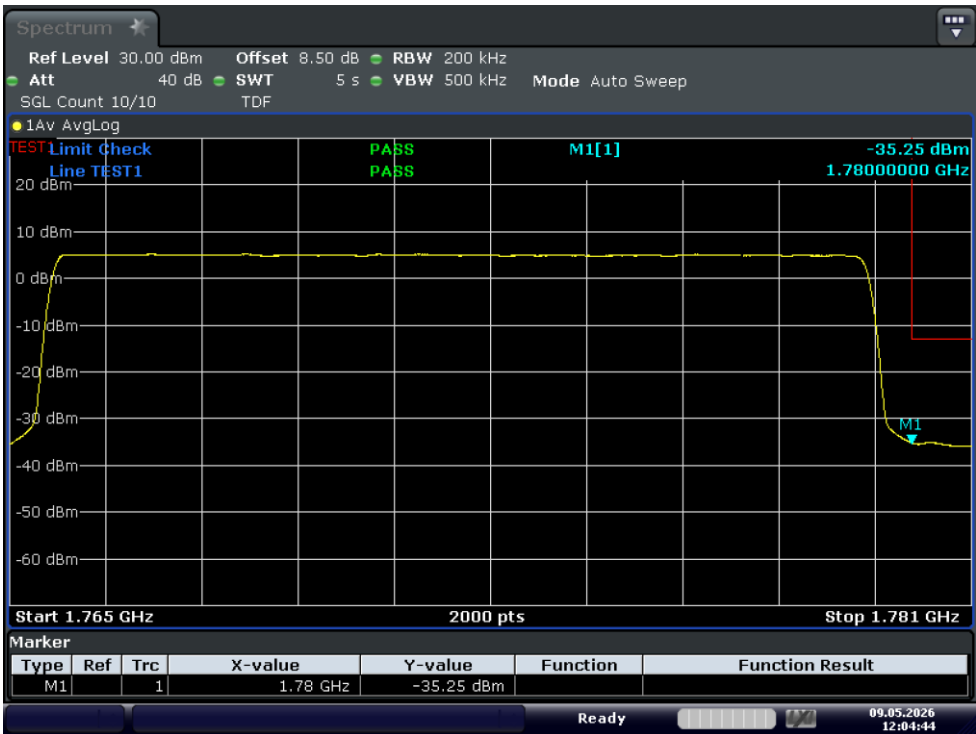
Test_Graph_band66_1772.5MHz_15M_QPSK_1RB#HIGH_Band edge
