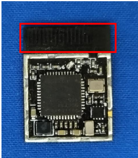
PCB Antenna
