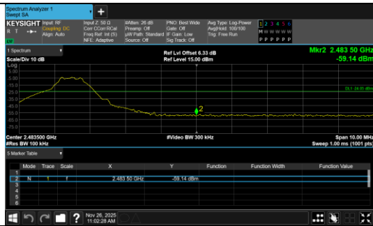
Out Of Band Emission BLE 1M_Channel 39
