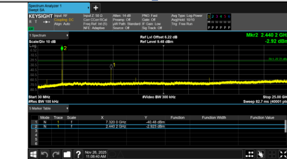
30.0 MHz - 25000.0 MHz BLE 2M_Channel 19
