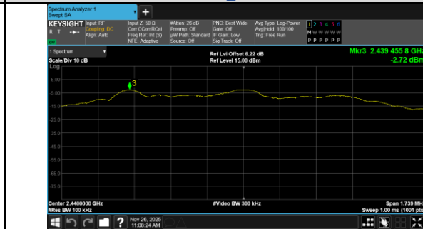
In-Band Reference Level BLE 2M_Channel 19
