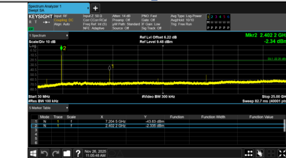
30.0 MHz - 25000.0 MHz BLE 2M_Channel 0
