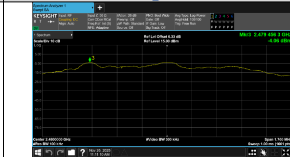
In-Band Reference Level BLE 2M_Channel 39
