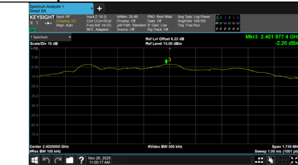
In-Band Reference Level BLE 2M_Channel 0
