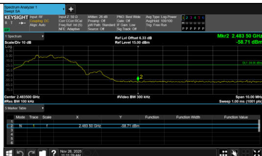
Out Of Band Emission BLE 2M_Channel 39
