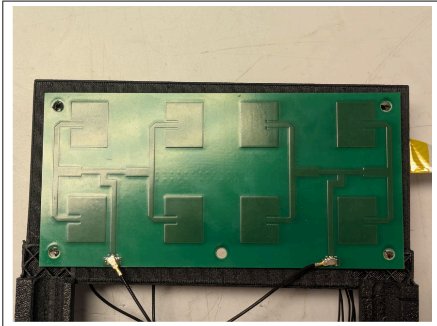
System Antenna - Rear
