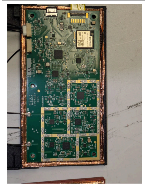
PCB Rear
