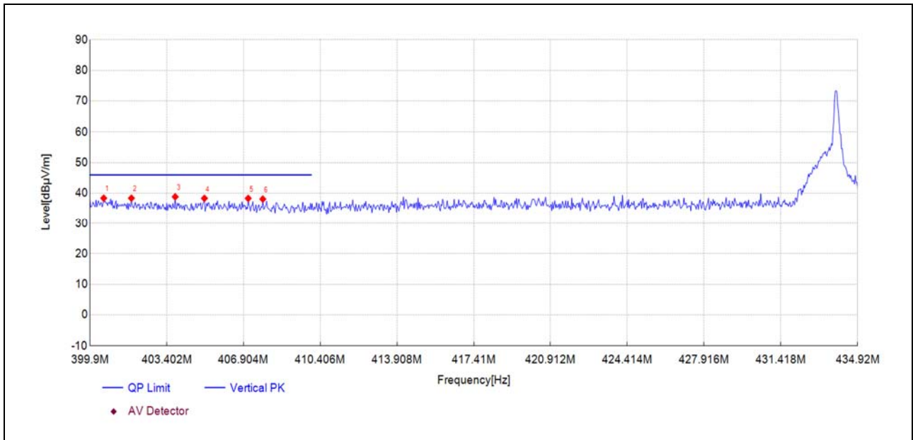
(Antenna Vertical)
