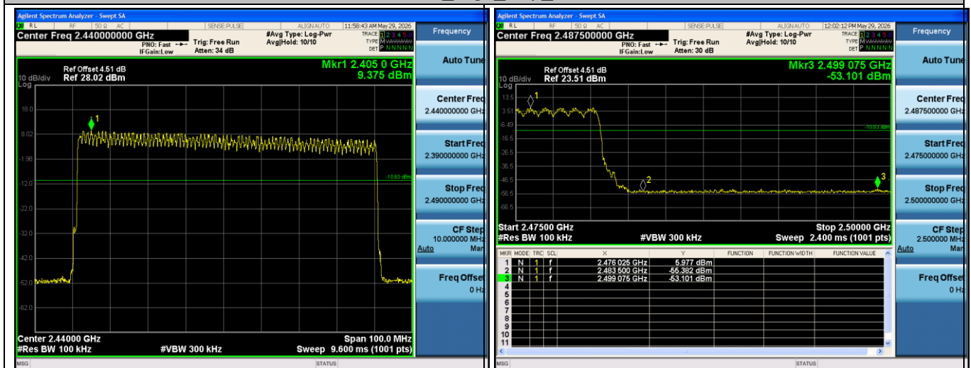
8-DPSK_High_Hop_2480
