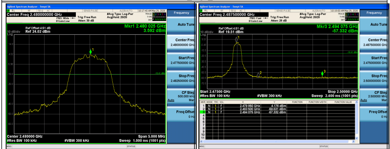
8-DPSK_High_Hop_2480
