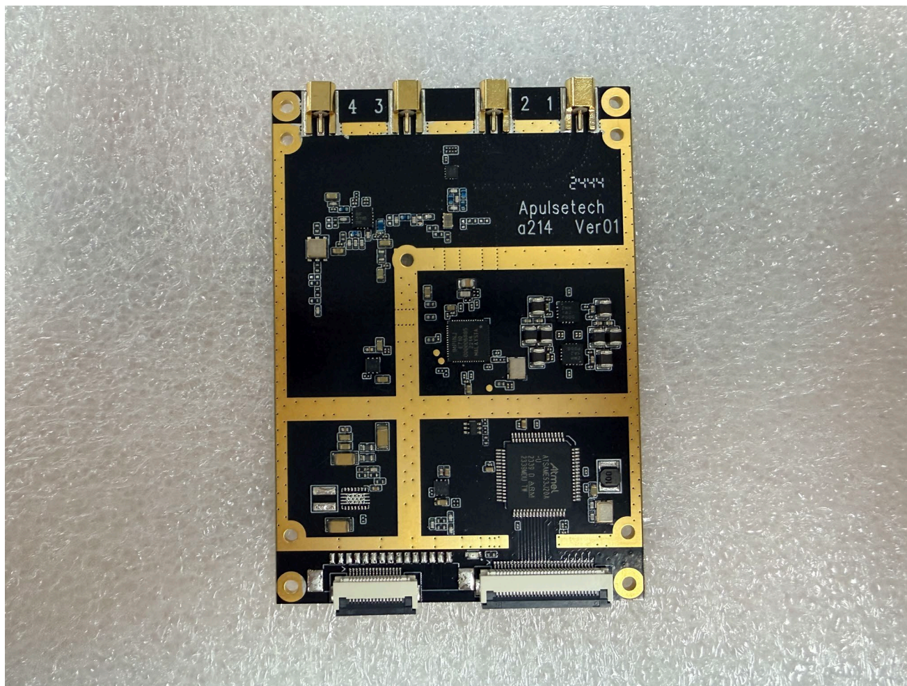
[Main board_Top]
