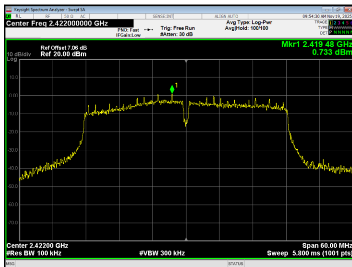
Tx. Spurious NVNT ax40 2422MHz Ant1 Emission
