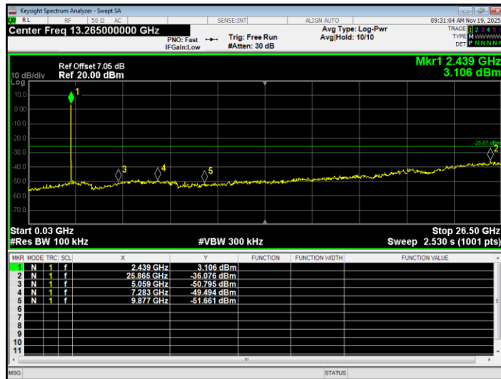
Tx. Spurious NVNT ax20 2462MHz Ant1 Ref
