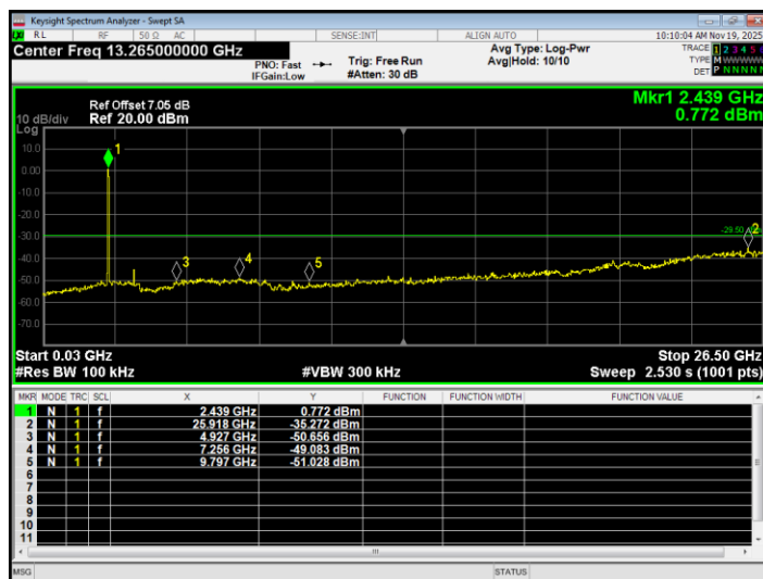
Tx. Spurious NVNT ax40 2452MHz Ant1 Ref
