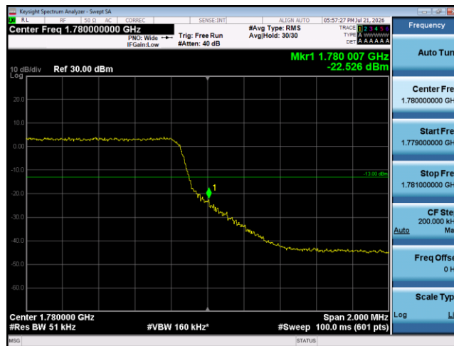
Band66-3MHz-16QAM-132657-15RB#0
