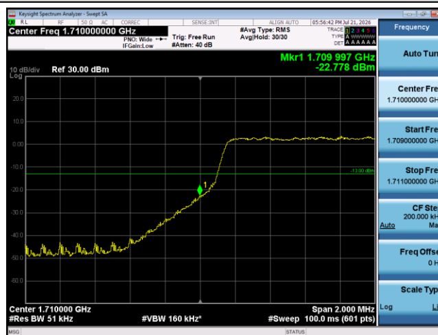
Band66-3MHz-16QAM-131987-15RB#0
