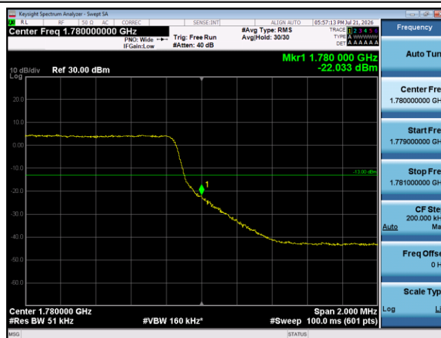
Band66-3MHz-QPSK-132657-15RB#0
