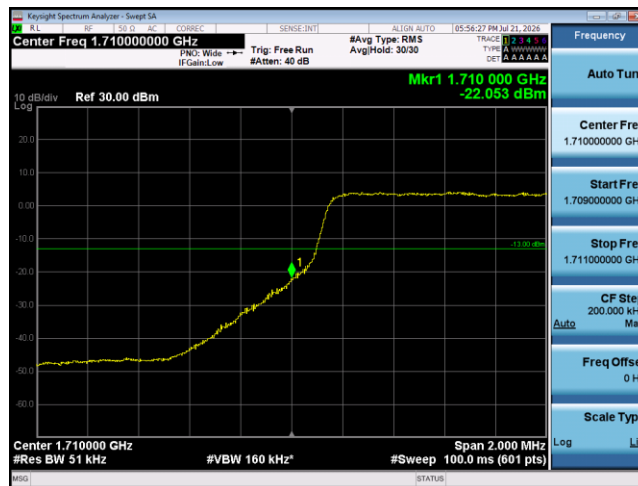
Band66-3MHz-QPSK-131987-15RB#0
