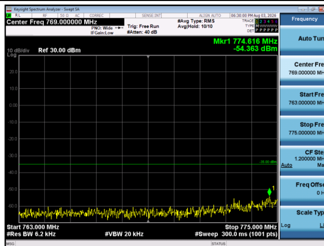
Band13-5MHz-16QAM-23205-1RB#0-Range3:763~775MHz
