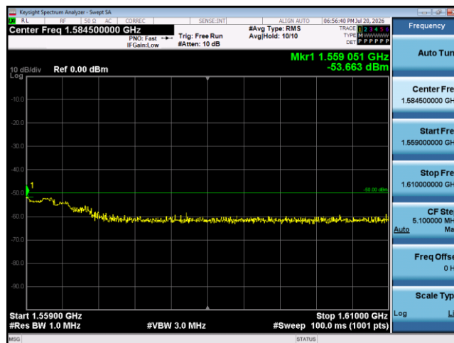
Band13-5MHz-QPSK-23205-1RB#0-Range5:1559~1610MHz
