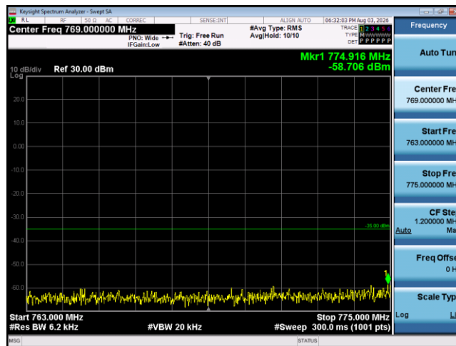
Band13-5MHz-16QAM-23230-1RB#0-Range3:763~775MHz
