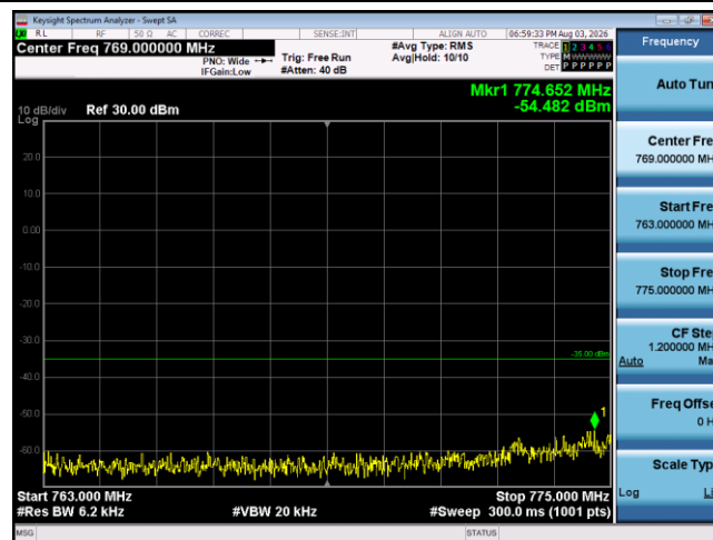
Band13-5MHz-QPSK-23205-1RB#0-Range3:763~775MHz
