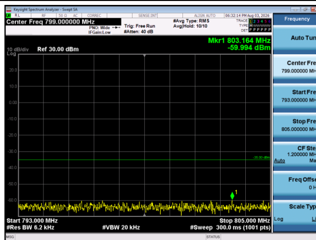
Band13-5MHz-16QAM-23230-1RB#0-Range4:793~805MHz
