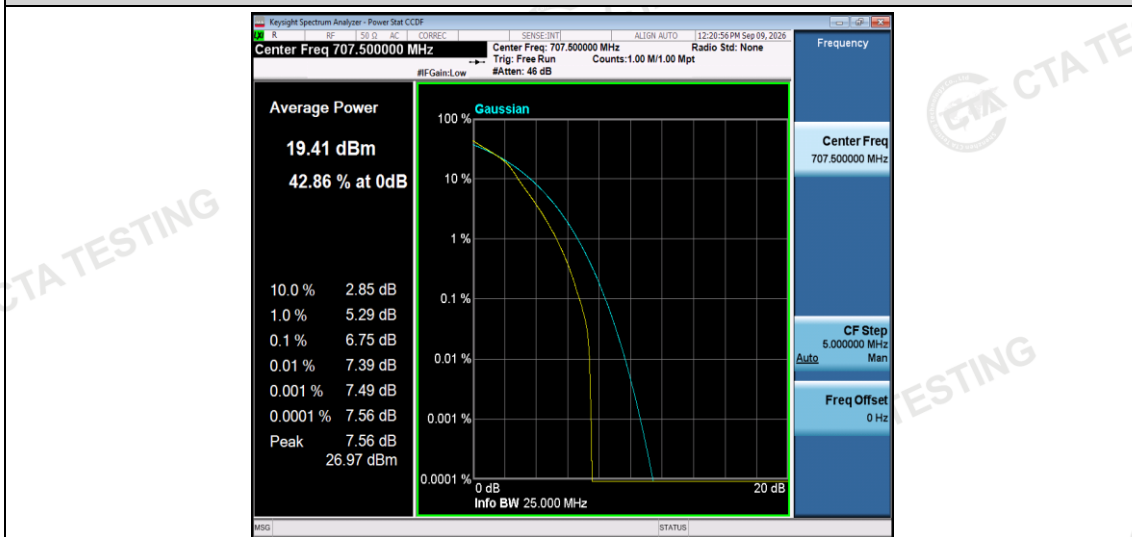
Band12-5MHz-16QAM-23095-25RB#0
