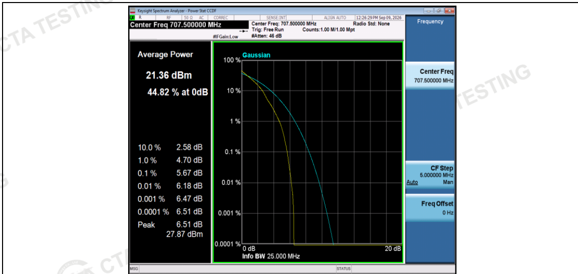
Band12-10MHz-QPSK-23095-1RB#0
