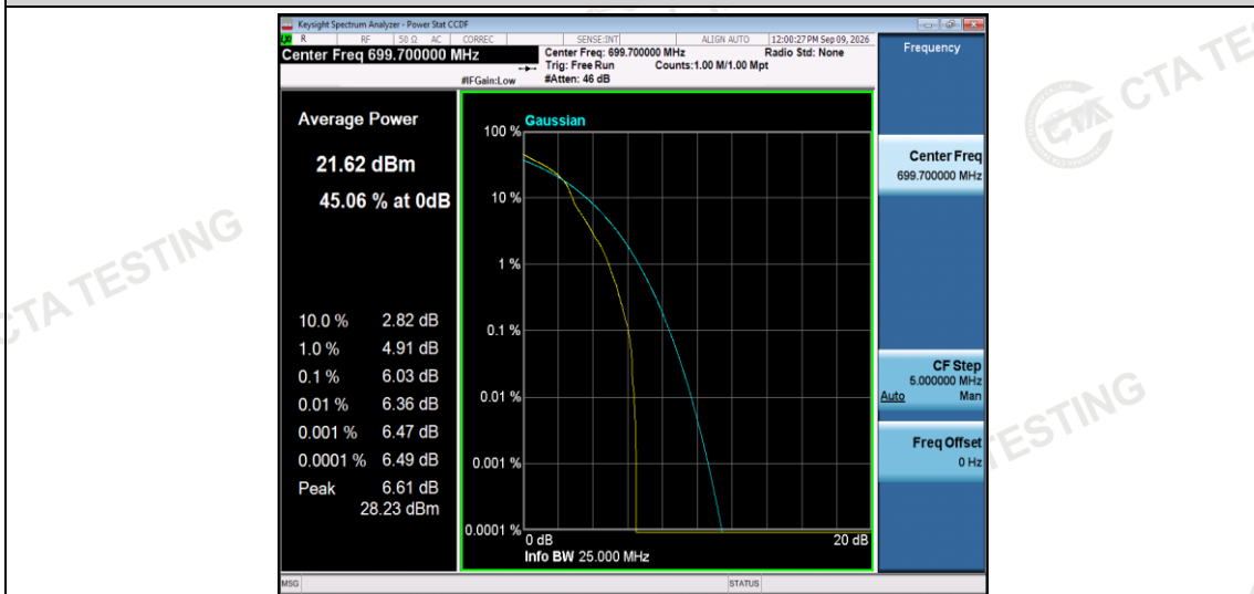
Band12-1.4MHz-16QAM-23017-1RB#0
