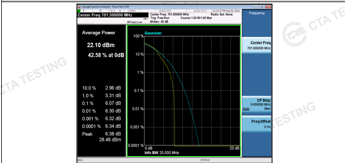
Band12-5MHz-16QAM-23035-1RB#0
