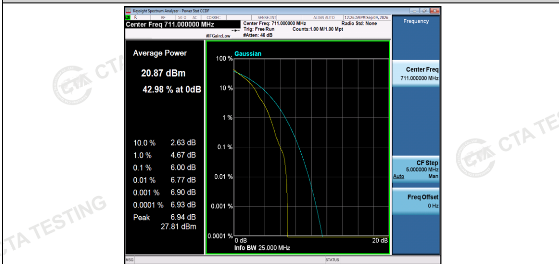
Band12-10MHz-QPSK-23130-1RB#0
