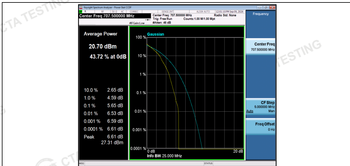
Band12-1.4MHz-QPSK-23095-1RB#0
