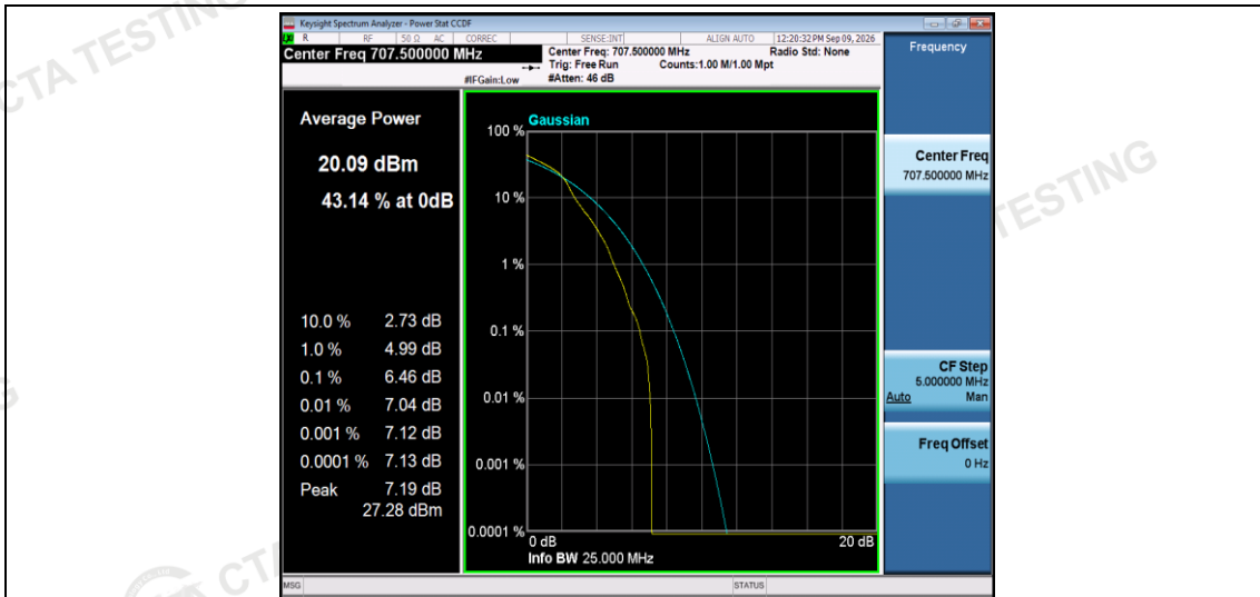
Band12-5MHz-16QAM-23095-1RB#0
