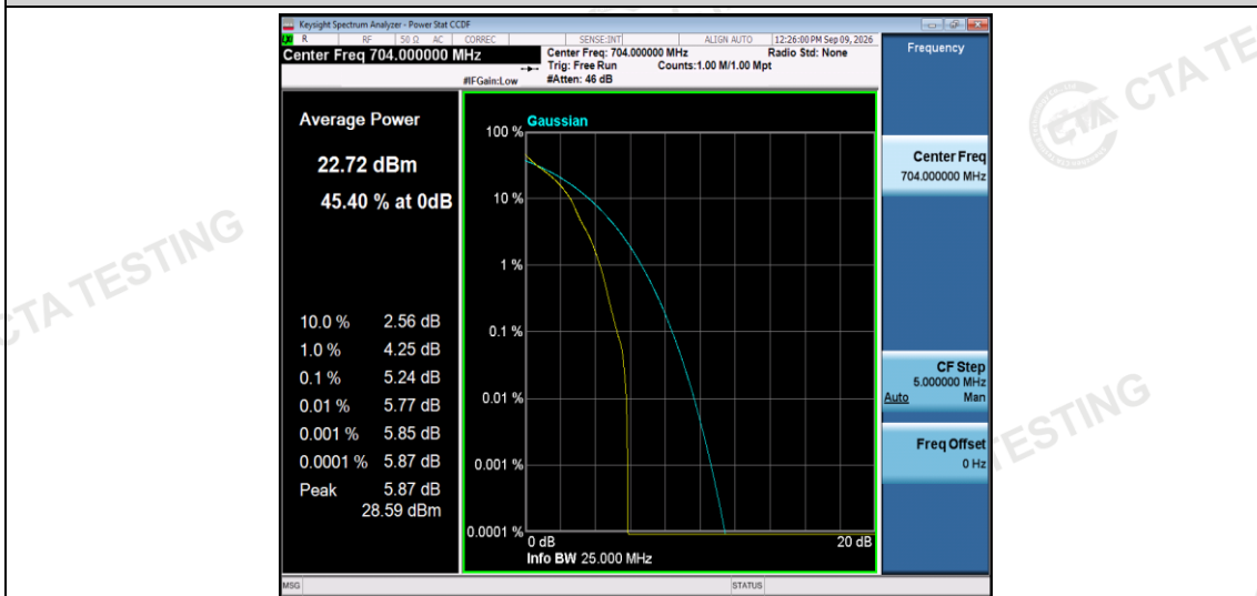
Band12-10MHz-QPSK-23060-1RB#0
