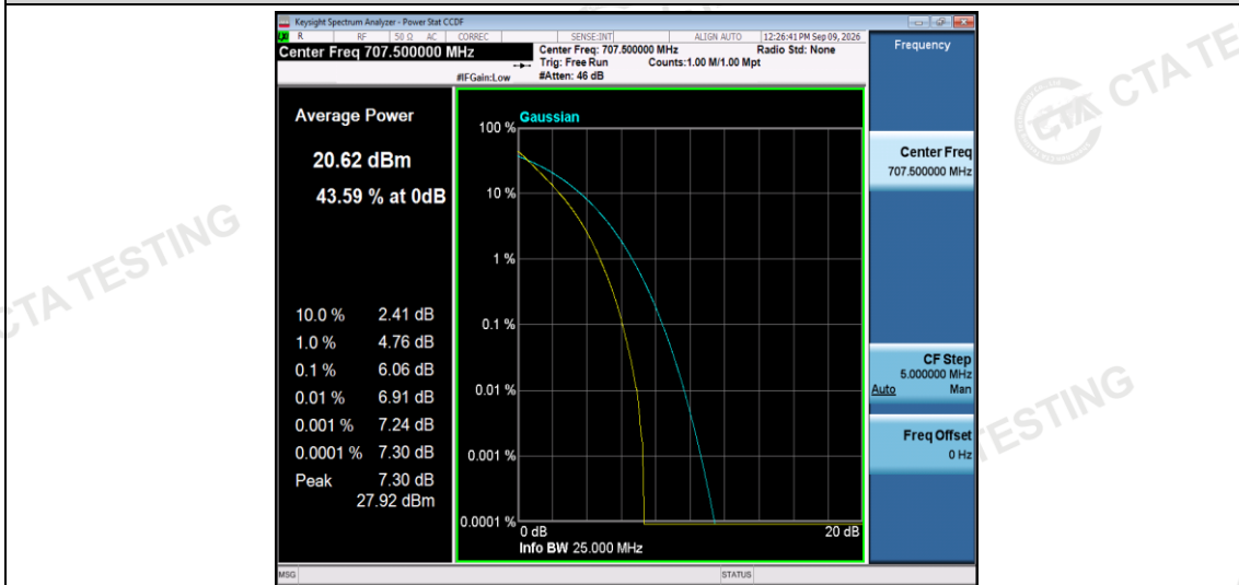
Band12-10MHz-QPSK-23095-50RB#0
