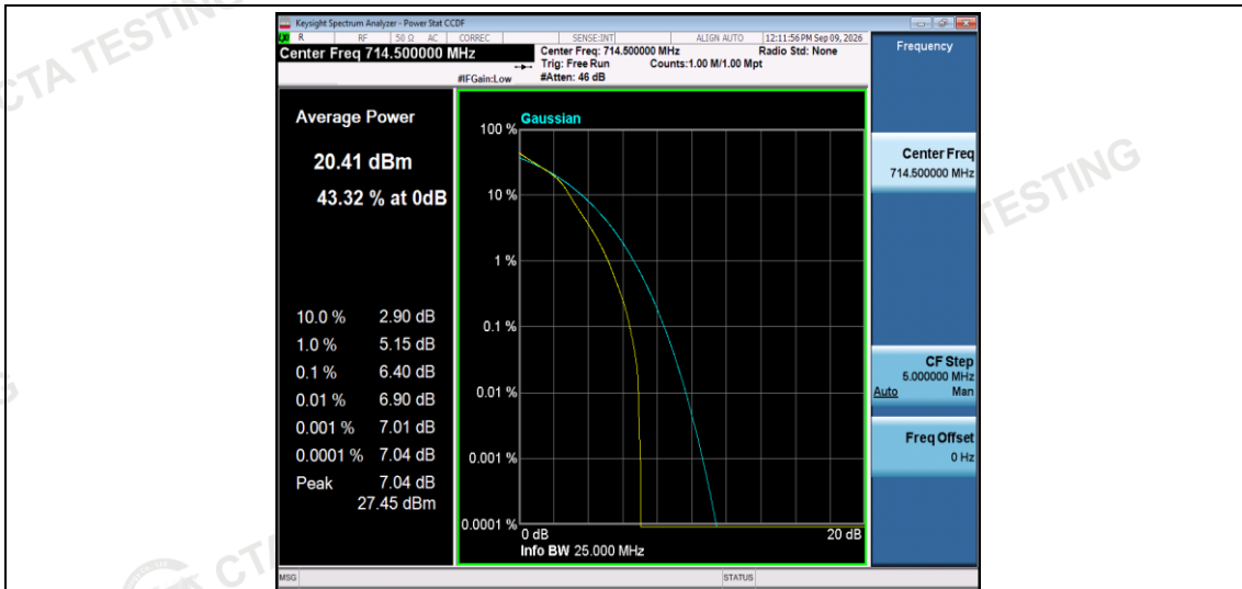
Band12-3MHz-16QAM-23165-15RB#0
