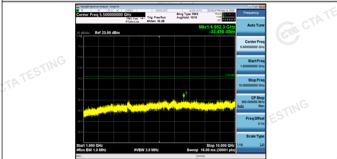
Band13-5MHz-16QAM-23255-1RB#0-Range2:1000~10000MHz
