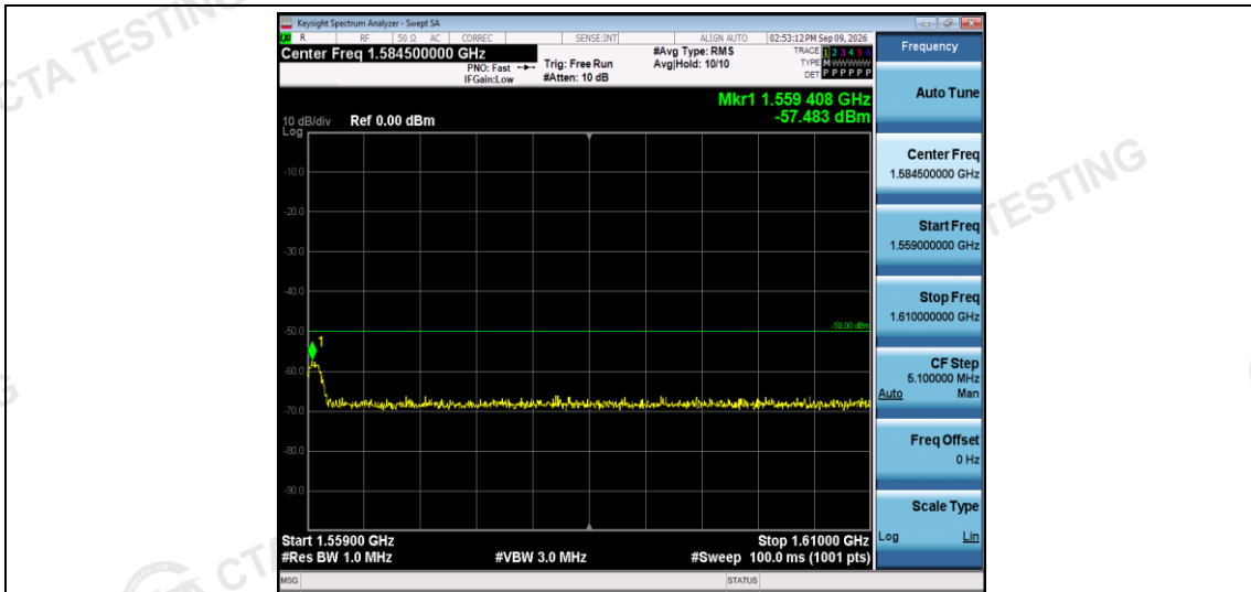
Band13-5MHz-16QAM-23230-1RB#0-Range5:1559~1610MHz
