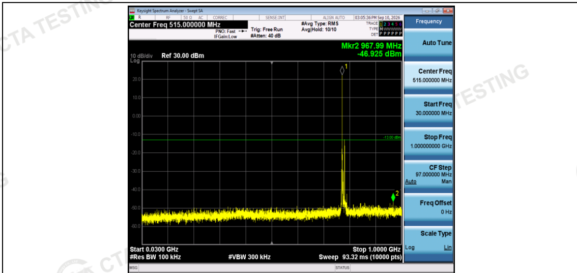
Band13-10MHz-QPSK-23230-1RB#0-Range1:30~1000MHz
