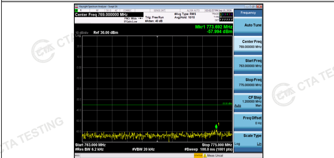
Band13-5MHz-16QAM-23255-1RB#0-Range3:763~775MHz
