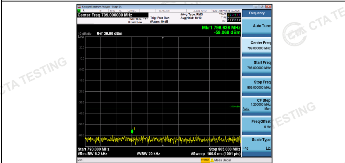
Band13-5MHz-16QAM-23230-1RB#0-Range4:793~805MHz
