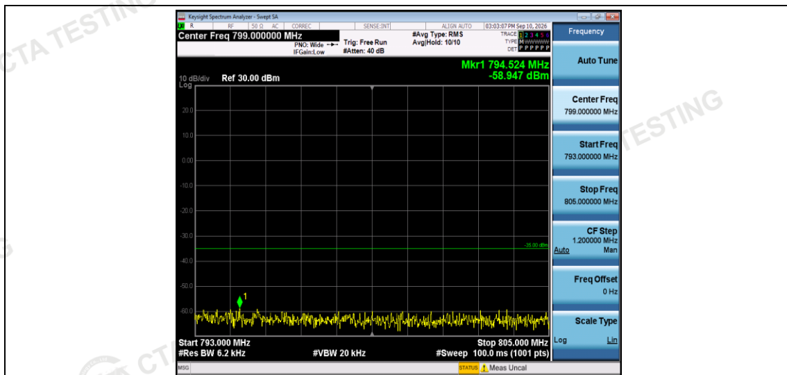
Band13-5MHz-16QAM-23255-1RB#0-Range4:793~805MHz
