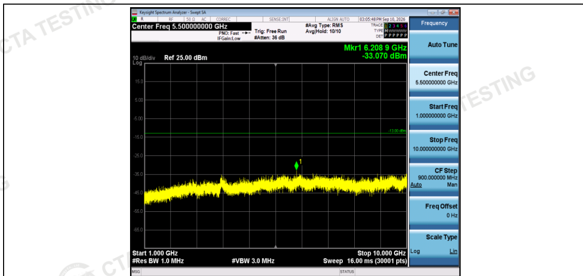
Band13-10MHz-QPSK-23230-1RB#0-Range2:1000~10000MHz
