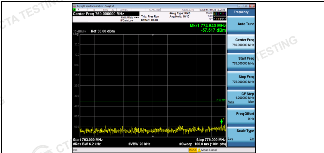
Band13-5MHz-16QAM-23230-1RB#0-Range3:763~775MHz
