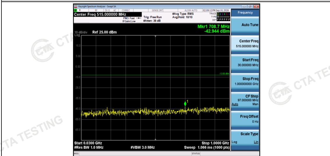
Band2-3MHz-16QAM-18615-1RB#0-Range1:30~1000MHz
