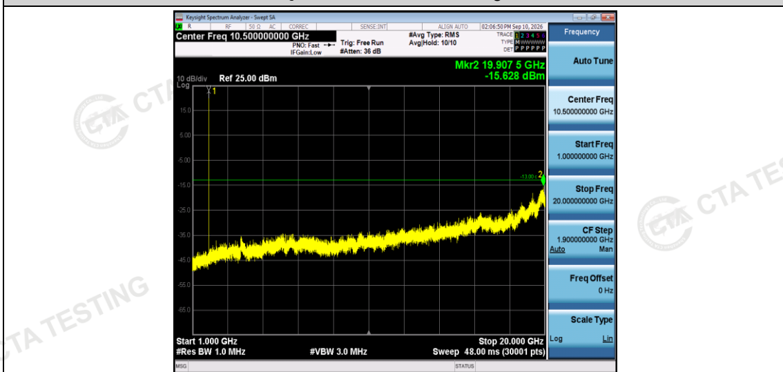
Band2-1.4MHz-QPSK-18900-1RB#0-Range2:1000~20000MHz
