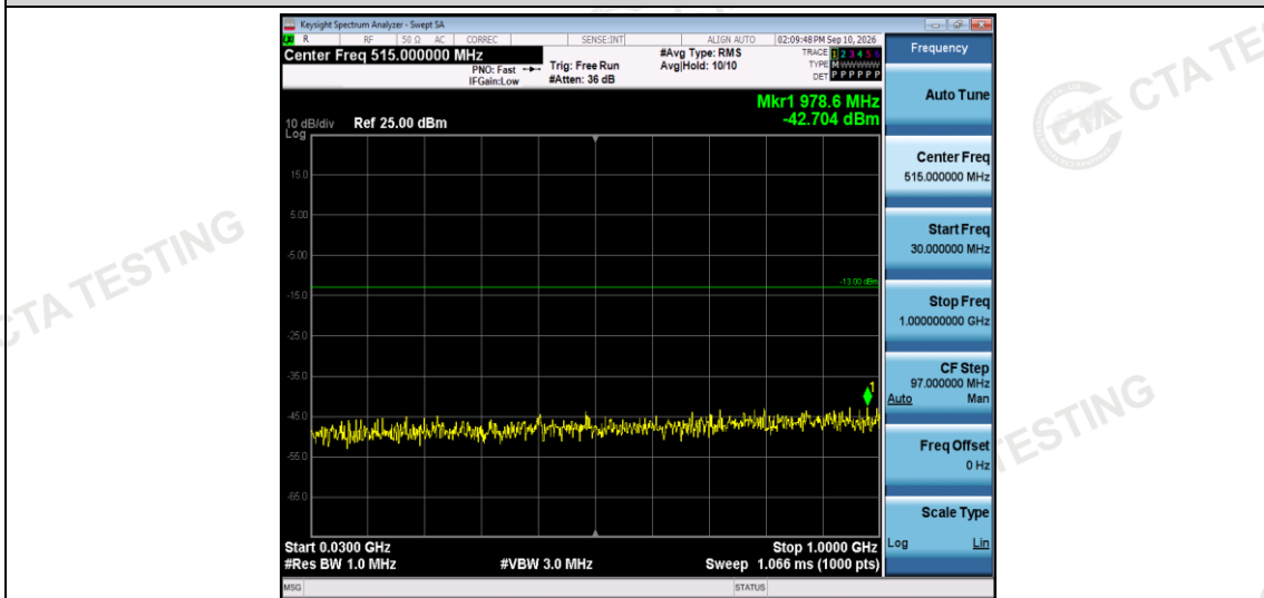
Band2-3MHz-QPSK-18900-1RB#0-Range1:30~1000MHz
