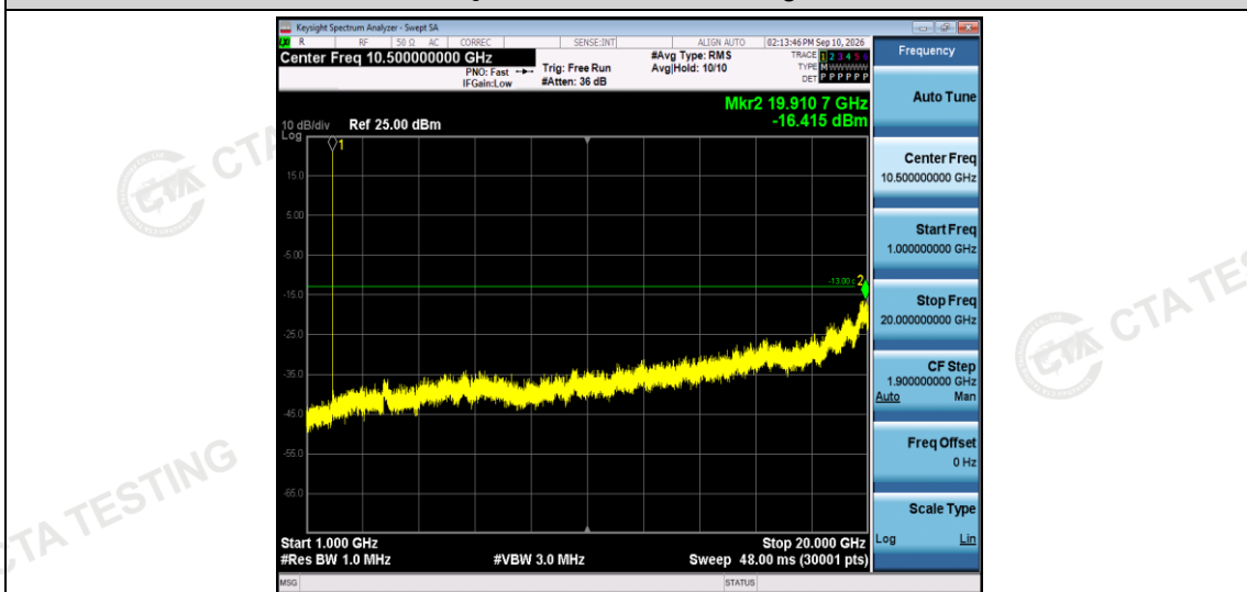
Band2-5MHz-16QAM-18900-1RB#0-Range2:1000~20000MHz
