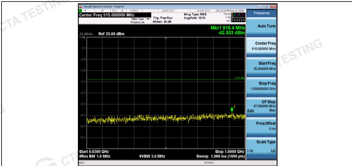
Band2-3MHz-QPSK-19185-1RB#0-Range1:30~1000MHz
