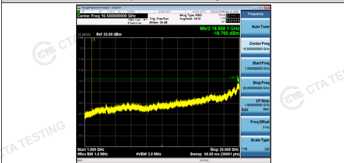
Band2-3MHz-16QAM-18900-1RB#0-Range2:1000~20000MHz
