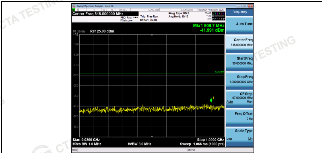
Band2-5MHz-QPSK-19175-1RB#0-Range1:30~1000MHz
