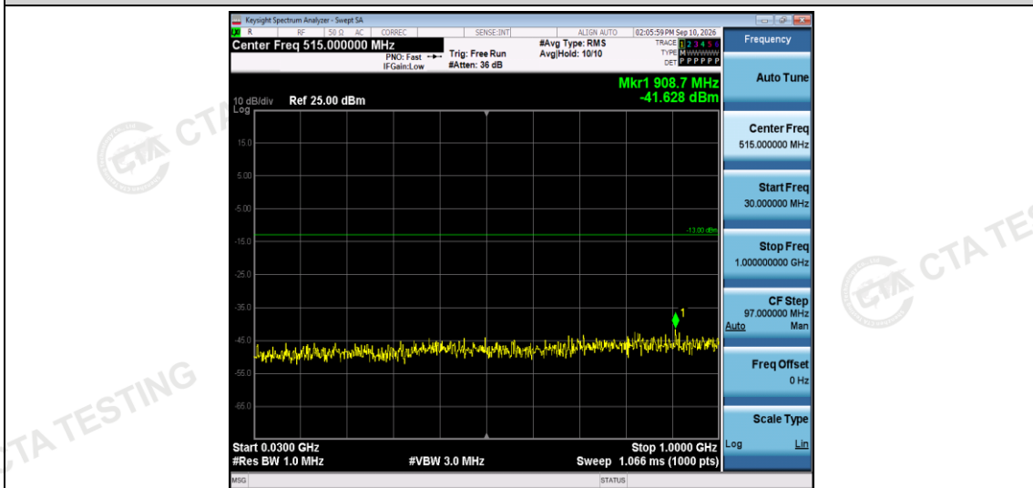
Band2-1.4MHz-16QAM-18607-1RB#0-Range1:30~1000MHz
