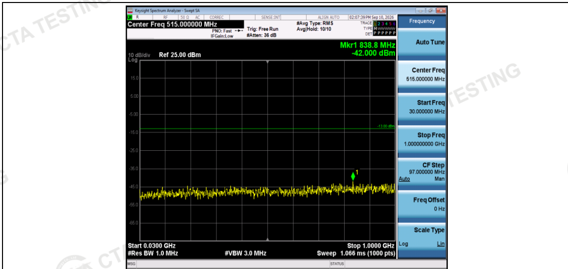
Band2-1.4MHz-QPSK-19193-1RB#0-Range1:30~1000MHz
