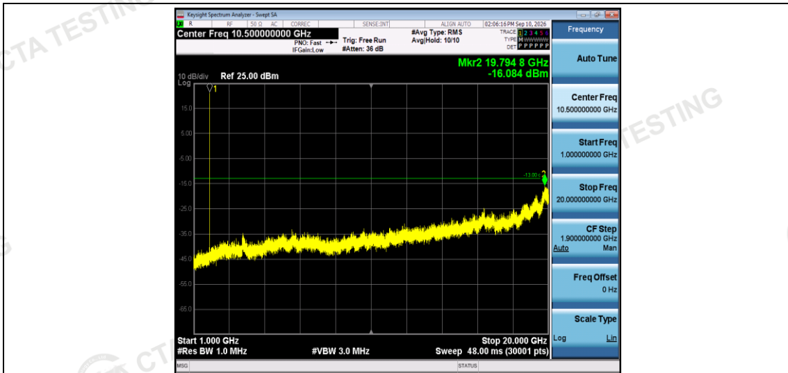
Band2-1.4MHz-16QAM-18607-1RB#0-Range2:1000~20000MHz
