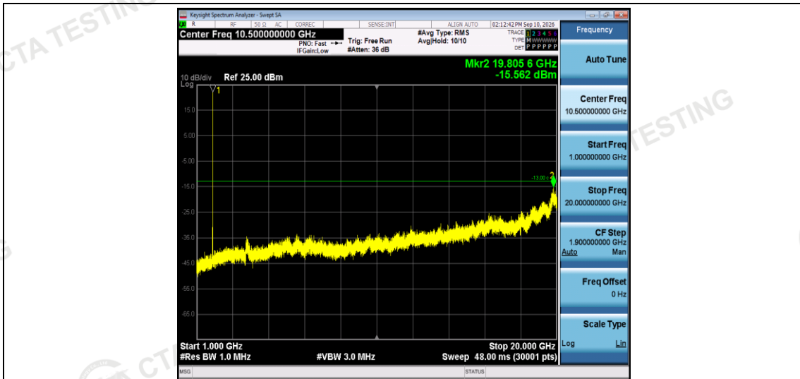
Band2-5MHz-16QAM-18625-1RB#0-Range2:1000~20000MHz
