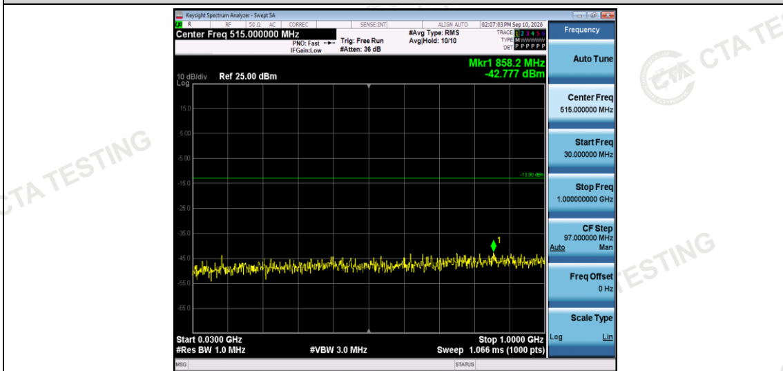
Band2-1.4MHz-16QAM-18900-1RB#0-Range1:30~1000MHz
