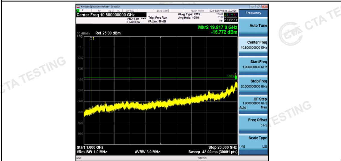
Band2-1.4MHz-16QAM-19193-1RB#0-Range2:1000~20000MHz
