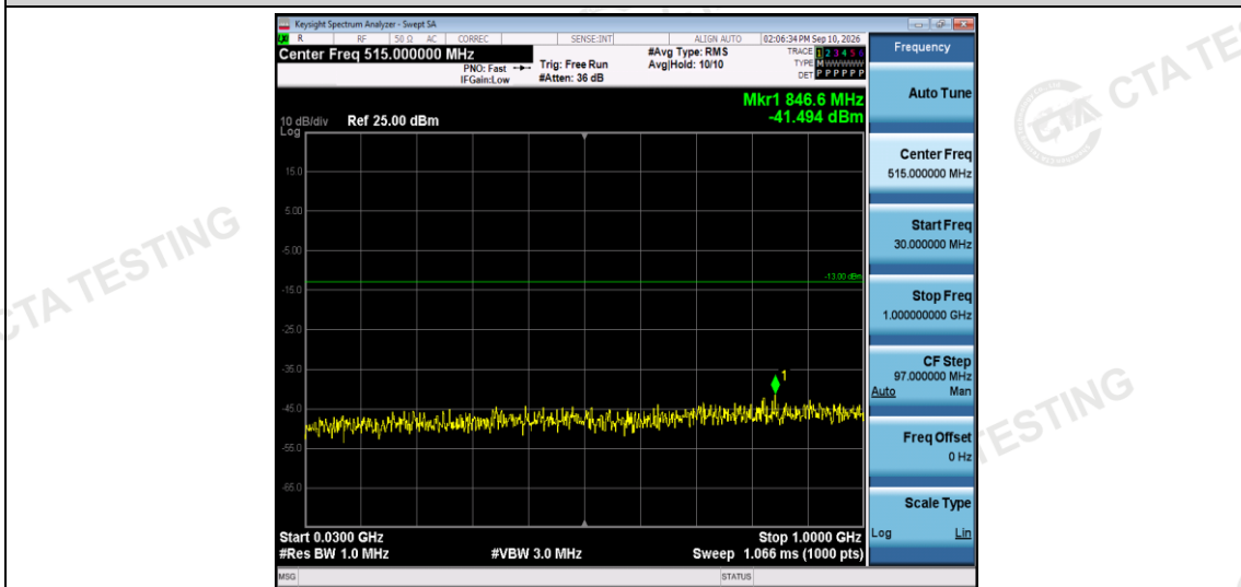
Band2-1.4MHz-QPSK-18900-1RB#0-Range1:30~1000MHz
