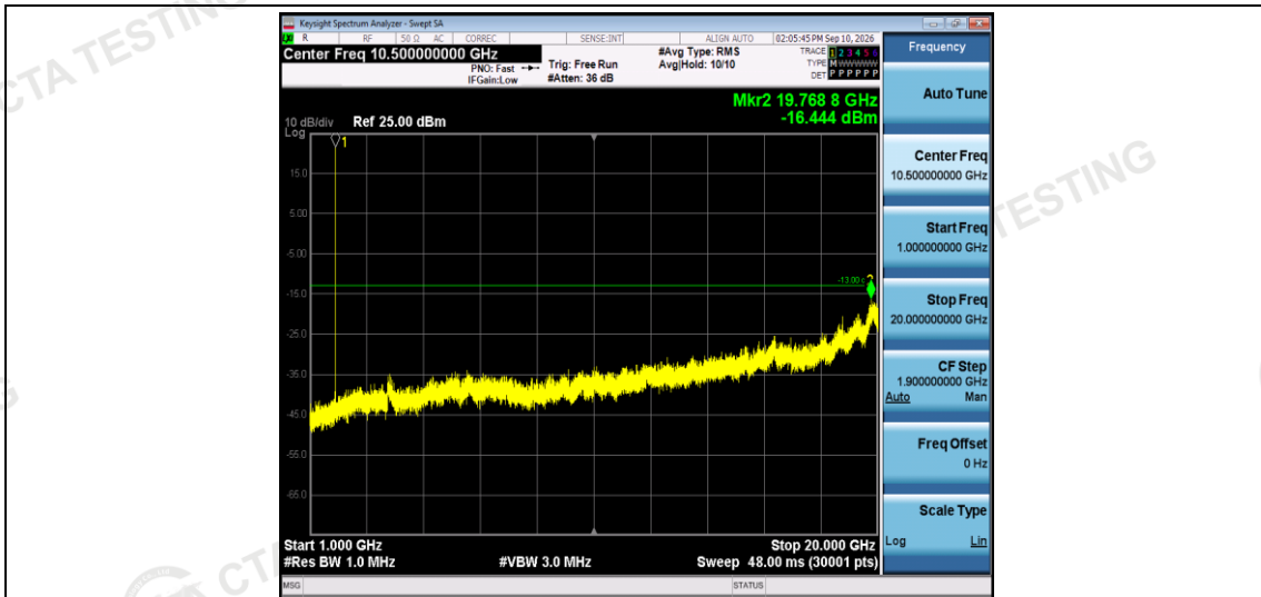
Band2-1.4MHz-QPSK-18607-1RB#0-Range2:1000~20000MHz
