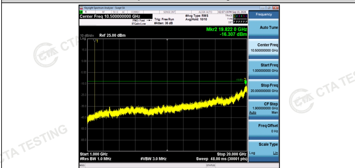
Band2-1.4MHz-16QAM-18900-1RB#0-Range2:1000~20000MHz
