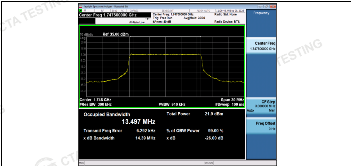
Band4-15MHz-QPSK-20325-75RB#0
