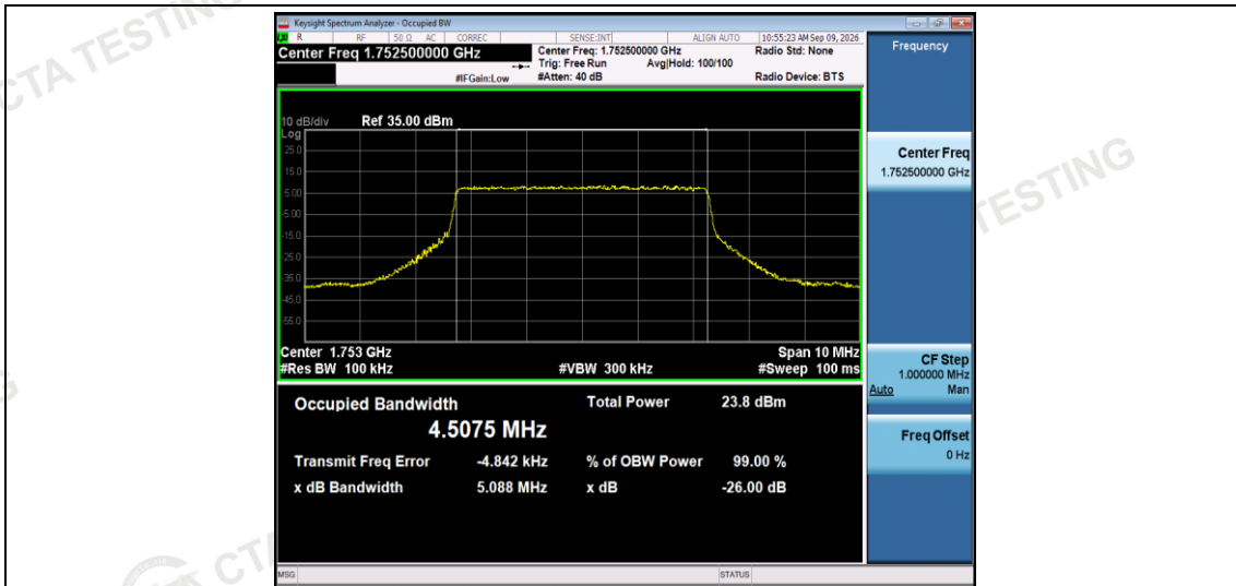
Band4-5MHz-QPSK-20375-25RB#0
