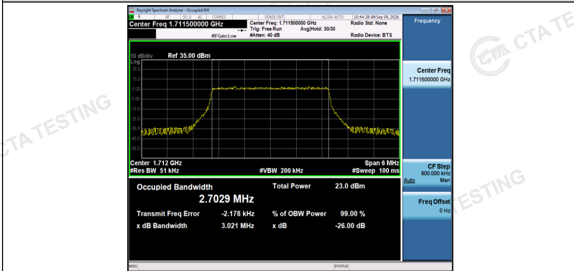
Band4-3MHz-16QAM-19965-15RB#0
