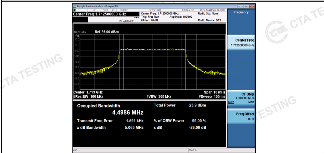
Band4-5MHz-16QAM-19975-25RB#0
