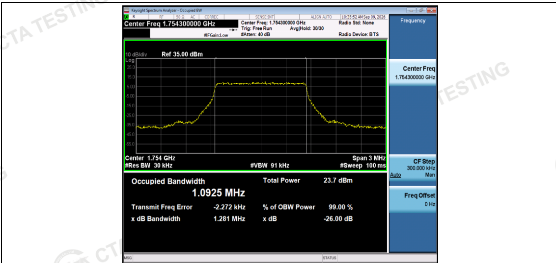
Band4-1.4MHz-QPSK-20393-6RB#0
