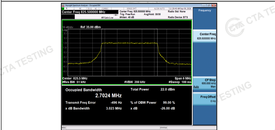
Band5-3MHz-QPSK-20415-15RB#0
