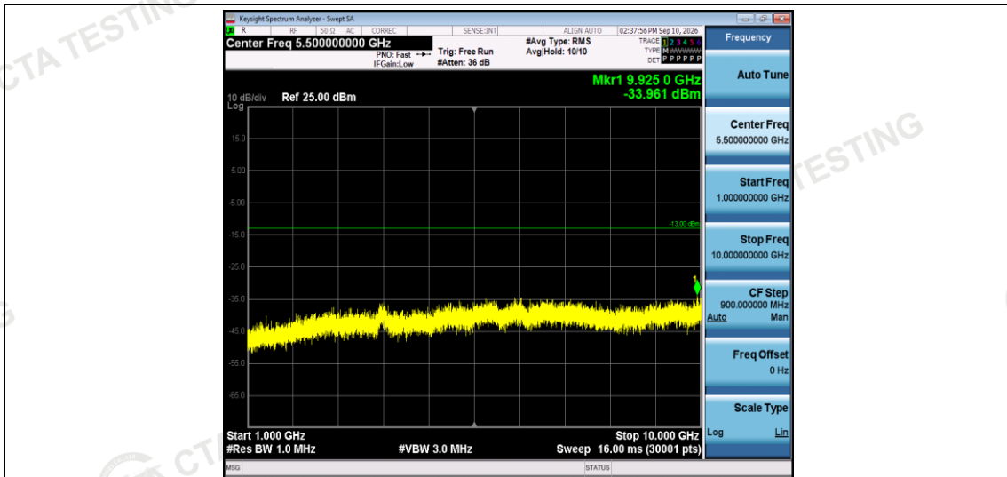
Band5-1.4MHz-QPSK-20643-1RB#0-Range2:1000~10000MHz
