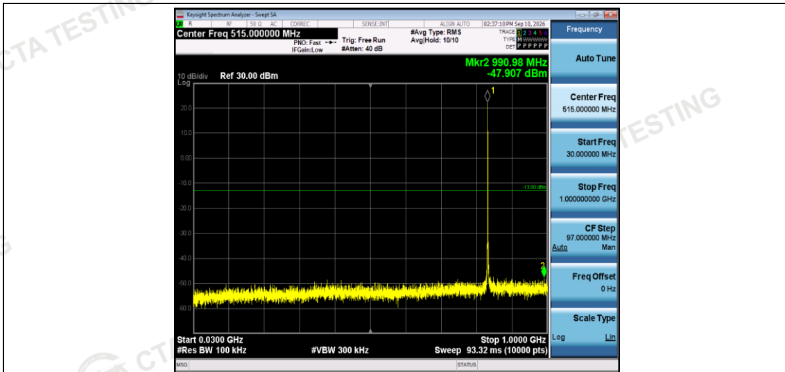
Band5-1.4MHz-16QAM-20525-1RB#0-Range1:30~1000MHz
