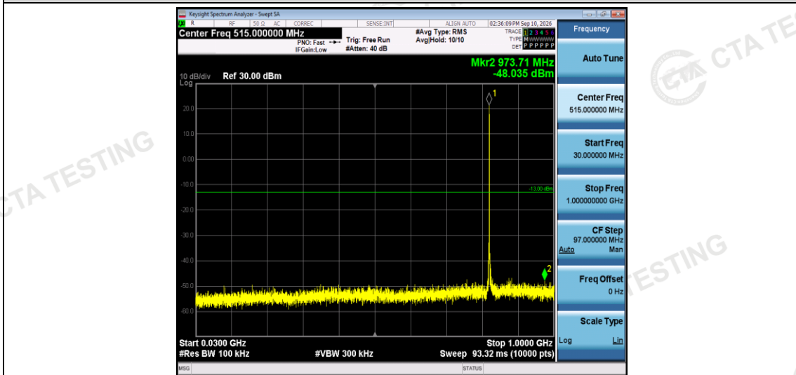
Band5-1.4MHz-16QAM-20407-1RB#0-Range1:30~1000MHz
