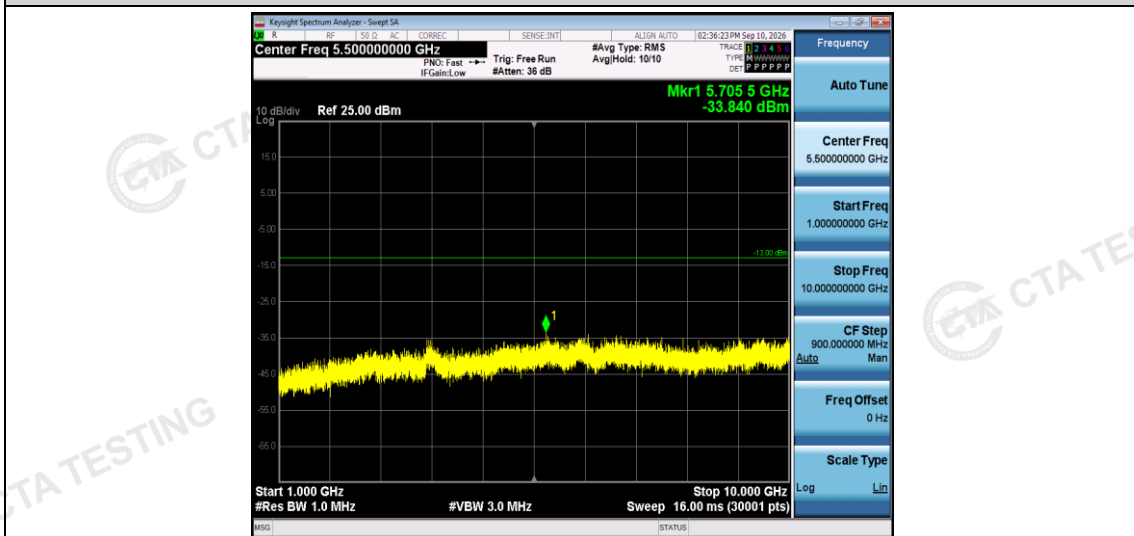
Band5-1.4MHz-16QAM-20407-1RB#0-Range2:1000~10000MHz
