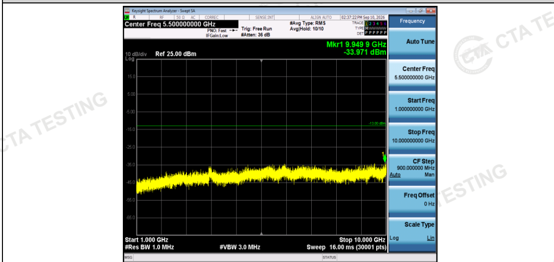
Band5-1.4MHz-16QAM-20525-1RB#0-Range2:1000~10000MHz
