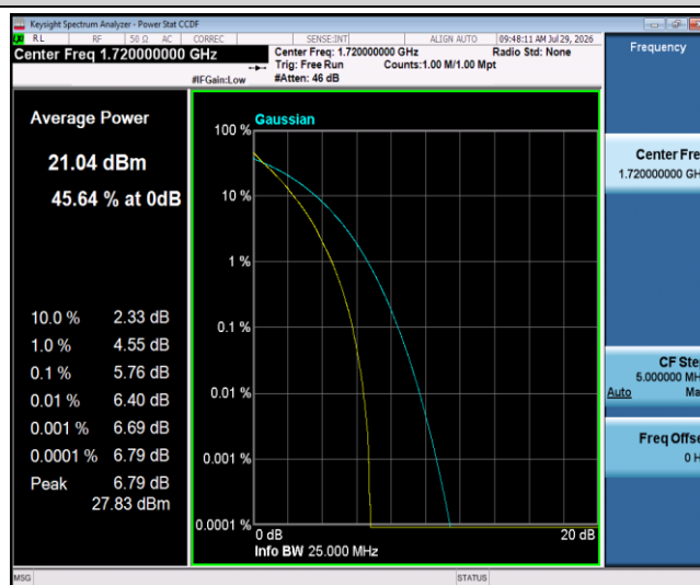
Band66-20MHz-QPSK-132072-100RB#0
