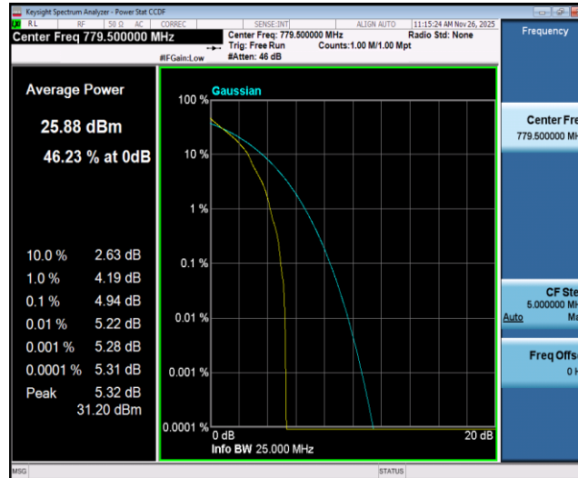
Band13-5MHz-QPSK-23205-1RB#0
