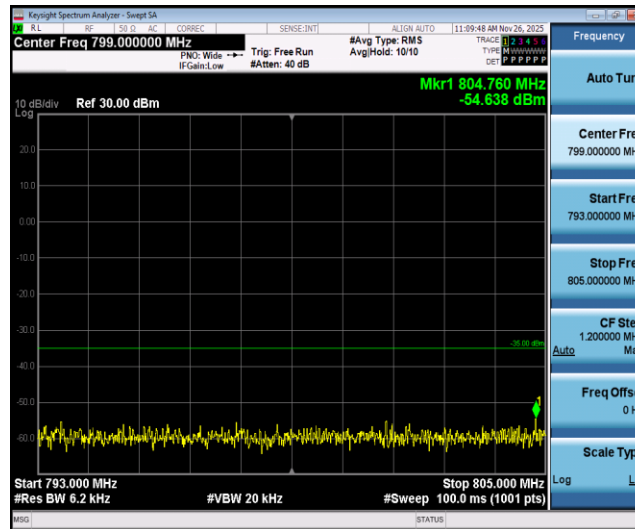
Band13-5MHz-QPSK-23205-1RB#0-Range4:793~805MHz
