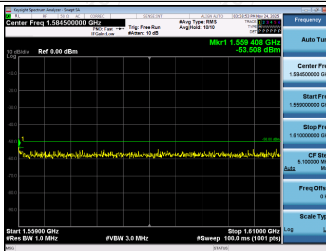
Band13-5MHz-QPSK-23205-1RB#0-Range5:1559~1610MHz
