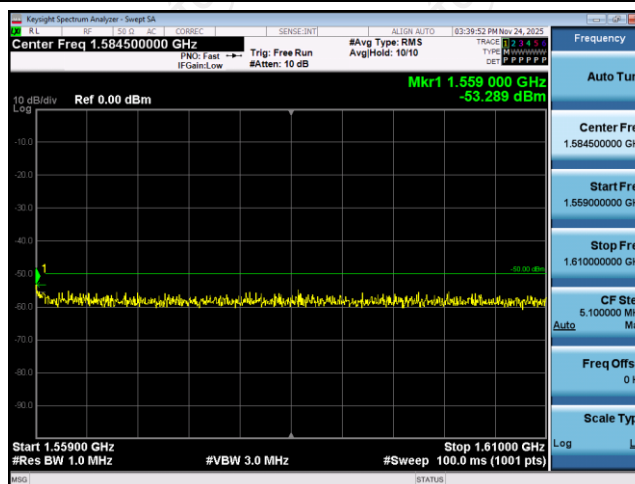
Band13-5MHz-16QAM-23205-1RB#0-Range5:1559~1610MHz
