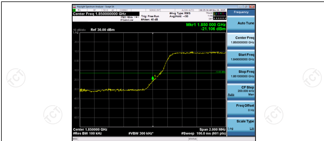
Band2-5MHz-16QAM-18625-25RB#0
