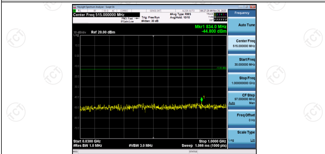
Band2-3MHz-QPSK-18615-1RB#0-Range1:30~1000MHz
