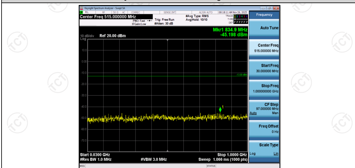
Band2-1.4MHz-16QAM-18607-1RB#0-Range1:30~1000MHz
