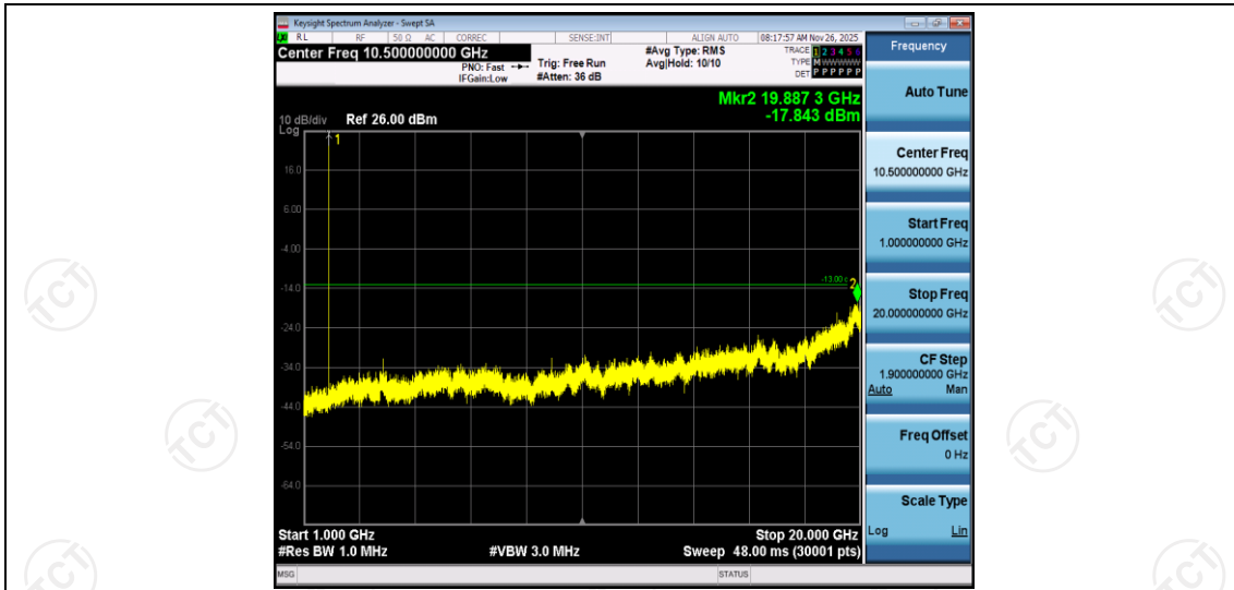
Band2-1.4MHz-QPSK-18607-1RB#0-Range2:1000~20000MHz
