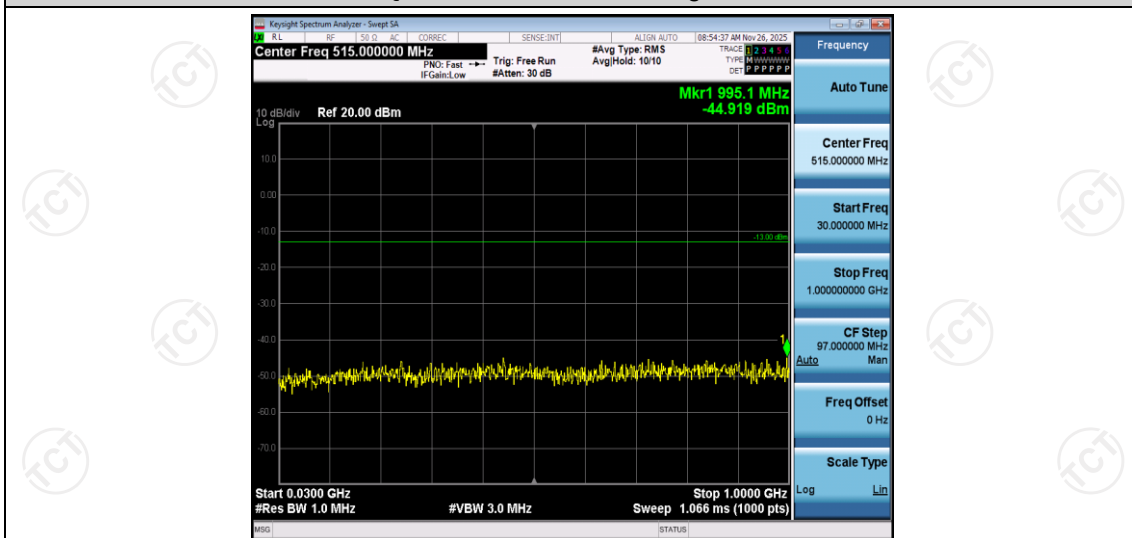
Band2-15MHz-QPSK-18900-1RB#0-Range1:30~1000MHz
