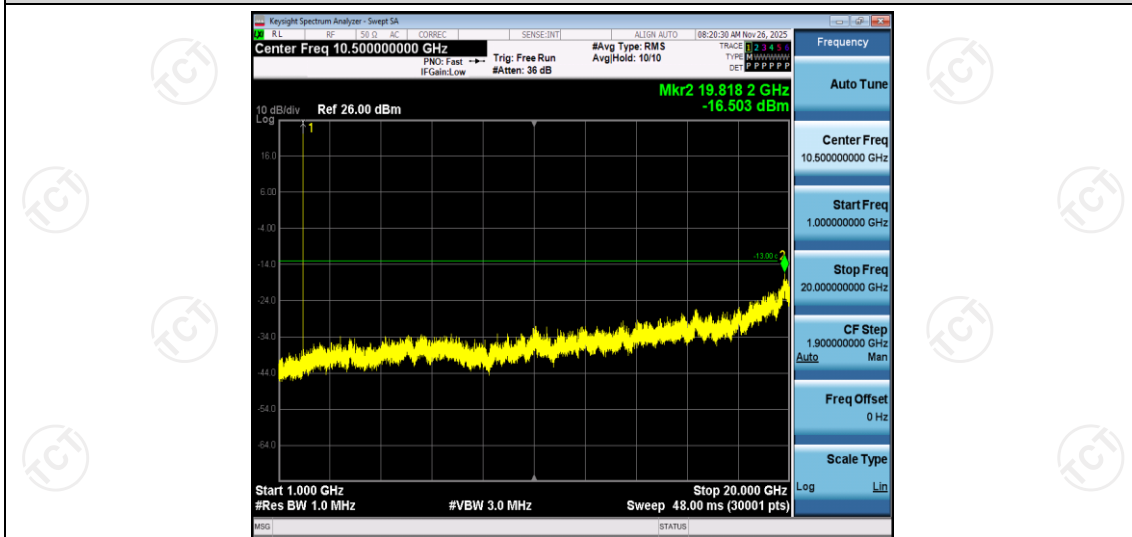
Band2-1.4MHz-16QAM-19193-1RB#0-Range2:1000~20000MHz
