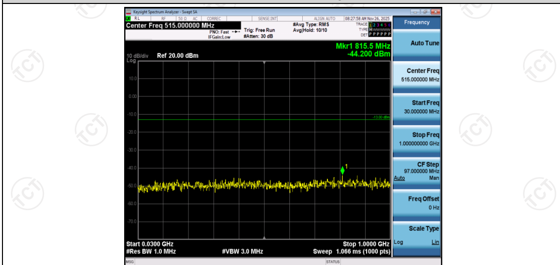
Band2-3MHz-16QAM-18615-1RB#0-Range1:30~1000MHz
