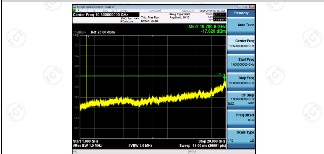
Band2-1.4MHz-16QAM-18900-1RB#0-Range2:1000~20000MHz
