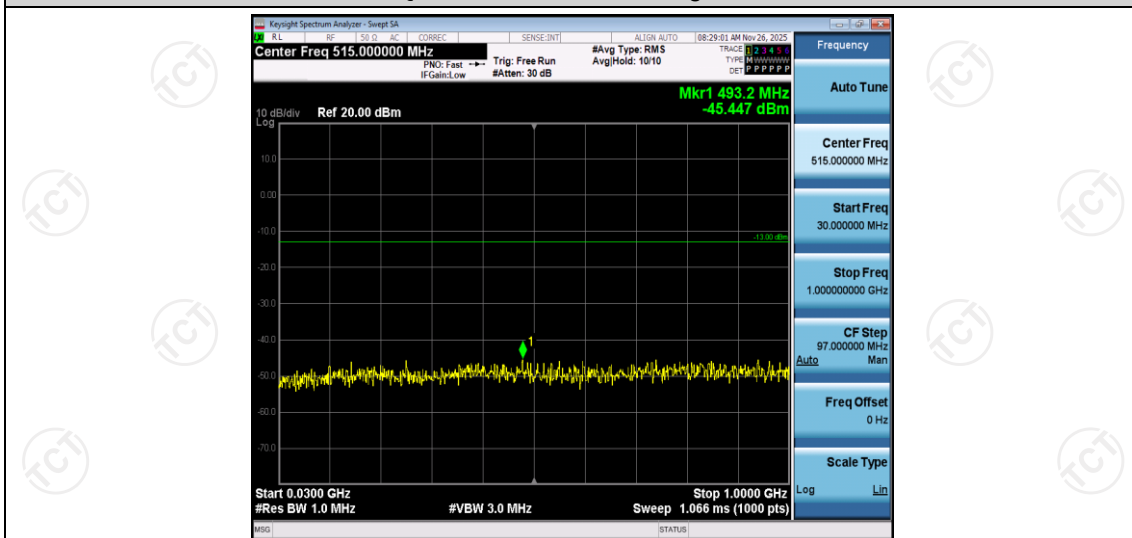
Band2-3MHz-16QAM-18900-1RB#0-Range1:30~1000MHz
