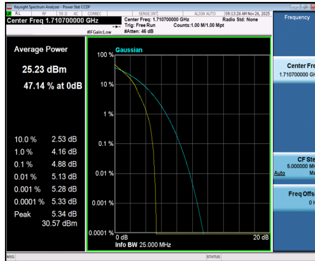
Band4-1.4MHz-QPSK-19957-1RB#0
