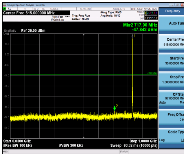
Band5-1.4MHz-QPSK-20525-1RB#0-Range1:30~1000MHz
