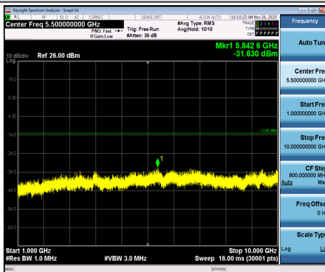
Band5-3MHz-QPSK-20525-1RB#0-Range2:1000~10000MHz
