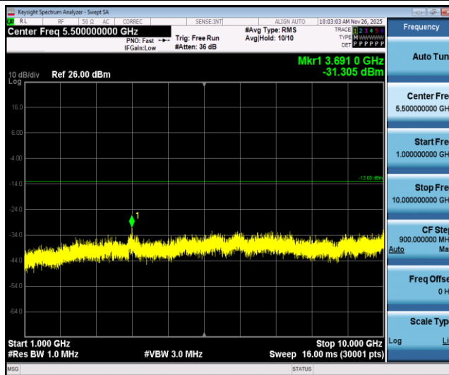
Band5-1.4MHz-QPSK-20643-1RB#0-Range2:1000~10000MHz
