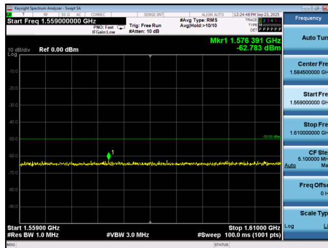
Band13-5MHz-16QAM-23205-1RB#0-Range5:1559~1610MHz
