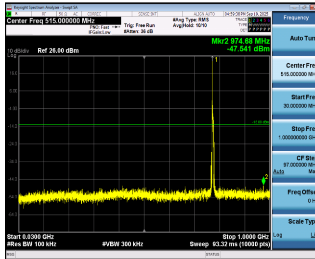
Band13-5MHz-16QAM-23205-1RB#0-Range1:30~1000MHz
