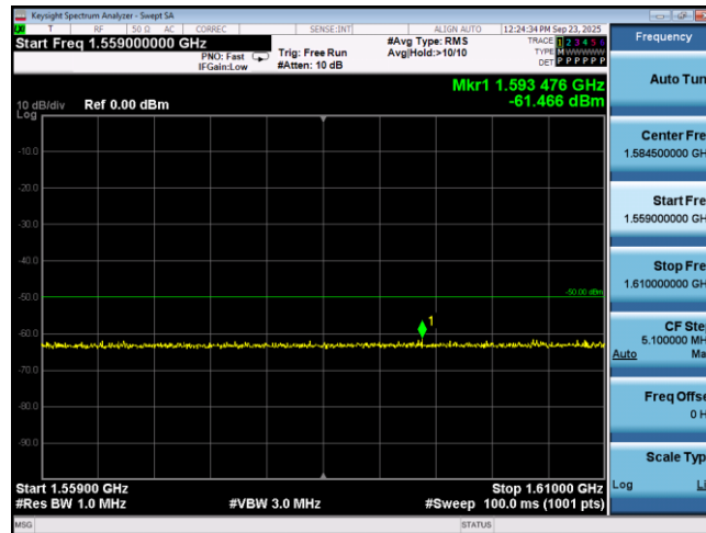
Band13-5MHz-QPSK-23230-1RB#0-Range5:1559~1610MHz
