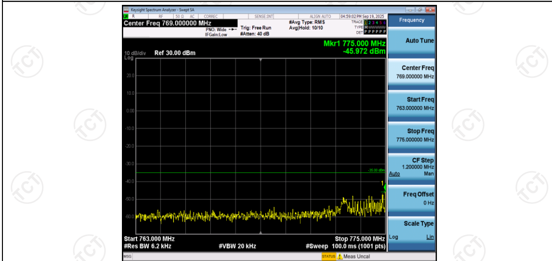
Band13-5MHz-QPSK-23205-1RB#0-Range3:763~775MHz
