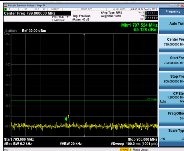
Band13-5MHz-16QAM-23205-1RB#0-Range4:793~805MHz
