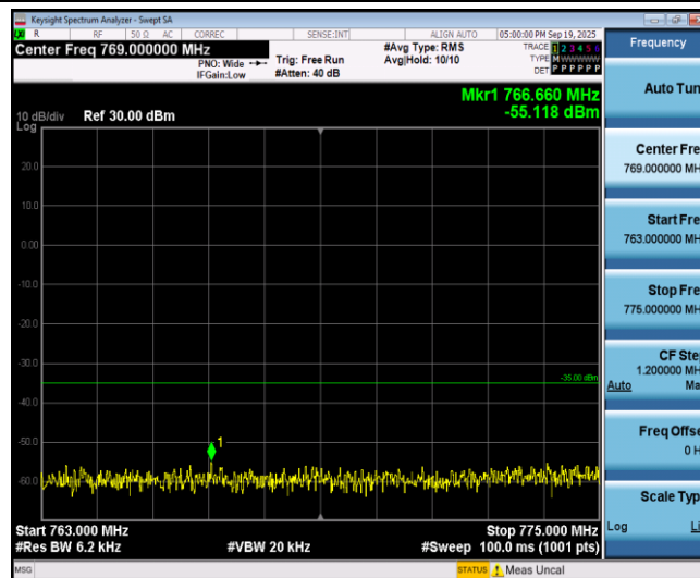
Band13-5MHz-16QAM-23205-1RB#0-Range3:763~775MHz
