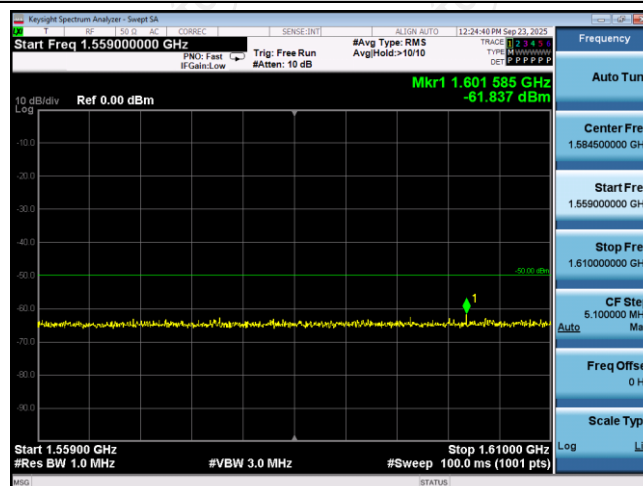
Band13-5MHz-QPSK-23255-1RB#0-Range5:1559~1610MHz
