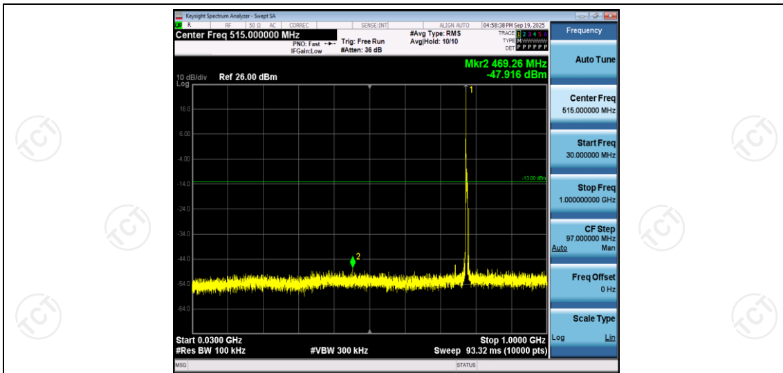
Band13-5MHz-QPSK-23205-1RB#0-Range1:30~1000MHz
