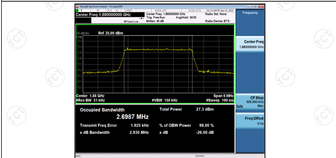
Band2-3MHz-QPSK-18900-15RB#0
