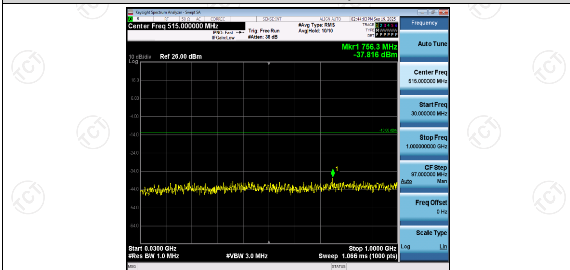
Band2-15MHz-QPSK-18900-1RB#0-Range1:30~1000MHz
