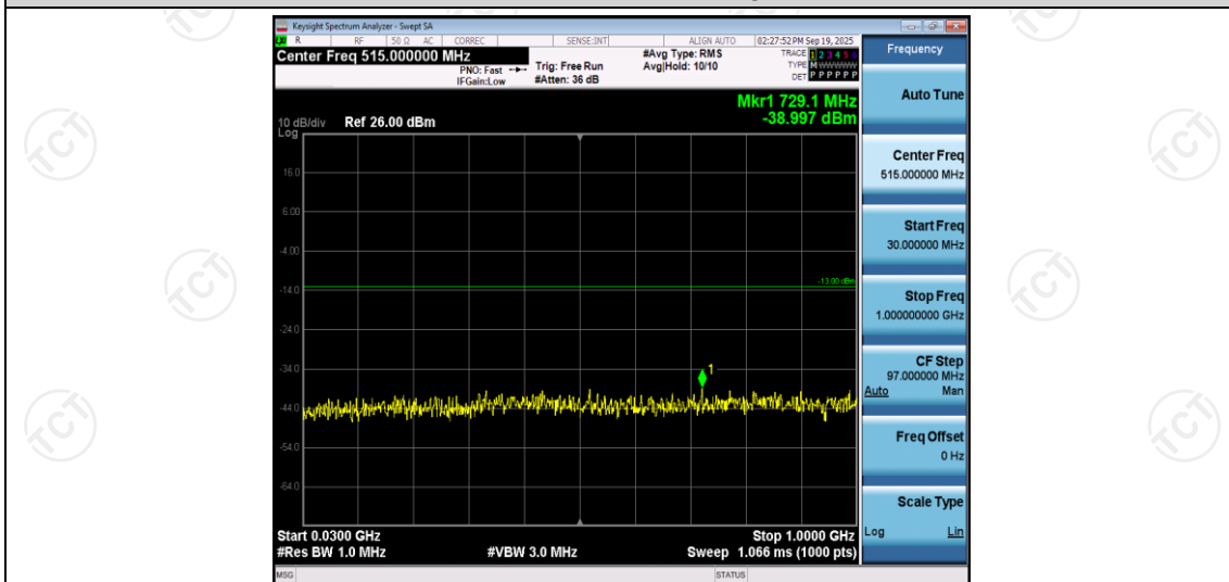
Band2-5MHz-16QAM-18900-1RB#0-Range1:30~1000MHz
