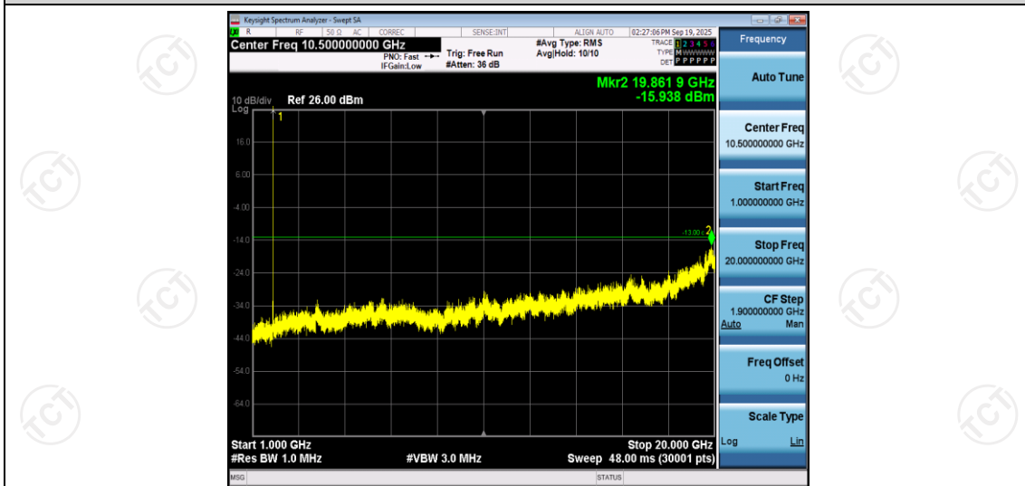
Band2-5MHz-16QAM-18625-1RB#0-Range2:1000~20000MHz
