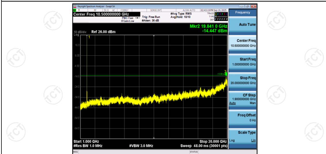
Band2-15MHz-QPSK-18675-1RB#0-Range2:1000~20000MHz
