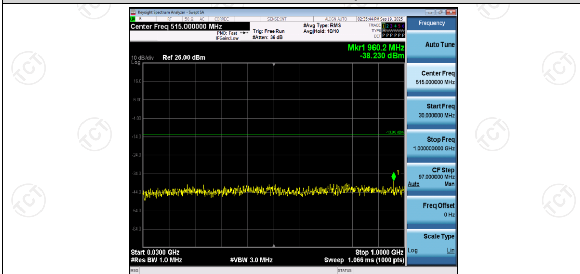
Band2-10MHz-QPSK-18900-1RB#0-Range1:30~1000MHz
