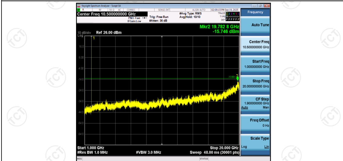
Band2-1.4MHz-QPSK-18607-1RB#0-Range2:1000~20000MHz
