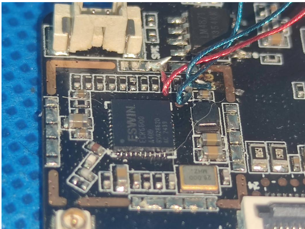
Photo 10 (sdio wifi and chip)
