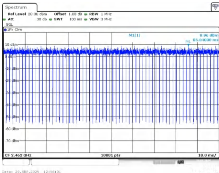
Duty Cycle NVNT ax20 2462MHz Ant1
