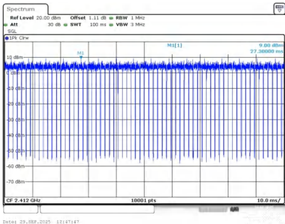
Duty Cycle NVNT ax20 2412MHz Ant1
