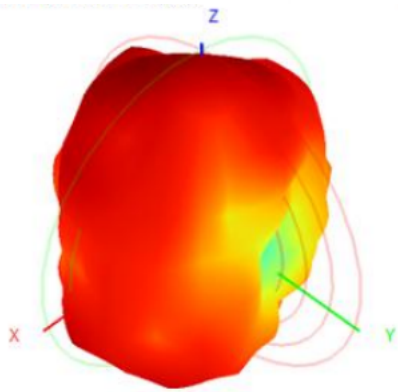
5800.0MHz Total, Eff: 68.7%
