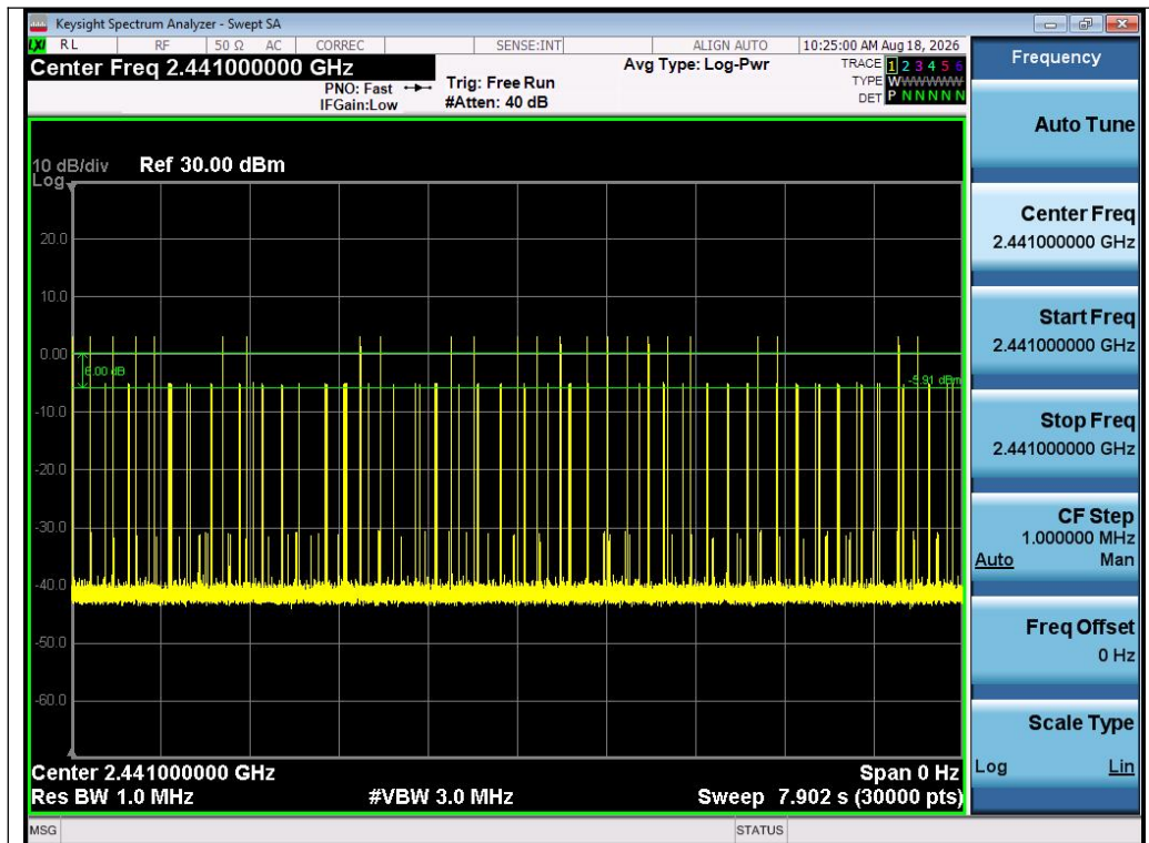
Test_Graph_EDR_HOP_ANT1_NA_2Mbps_2441_Number of Burstr
