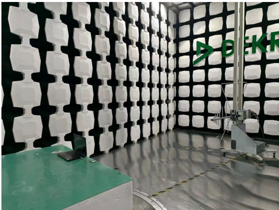
Radiated emissions
