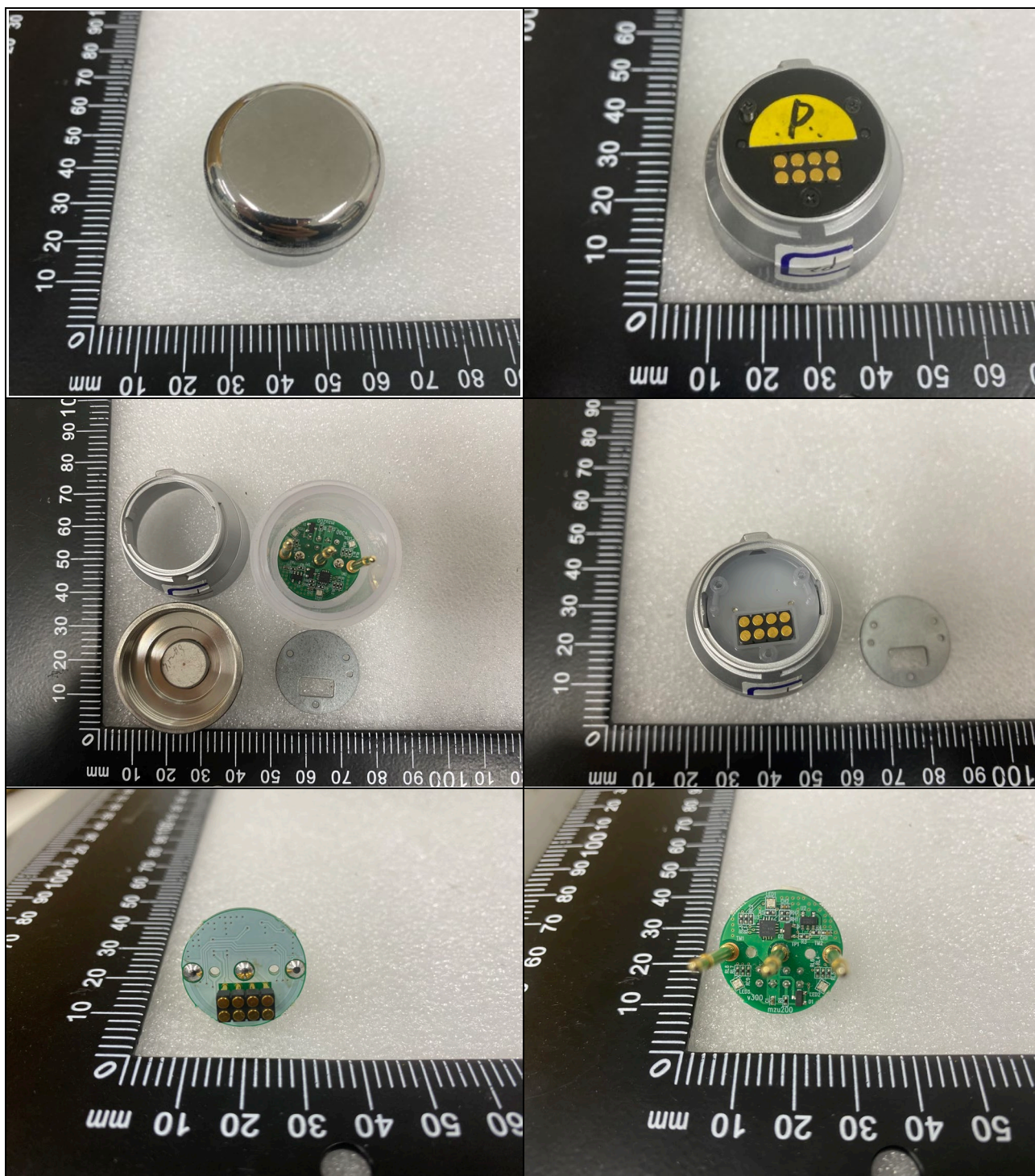
HEAD 3 (mzh-s201)
