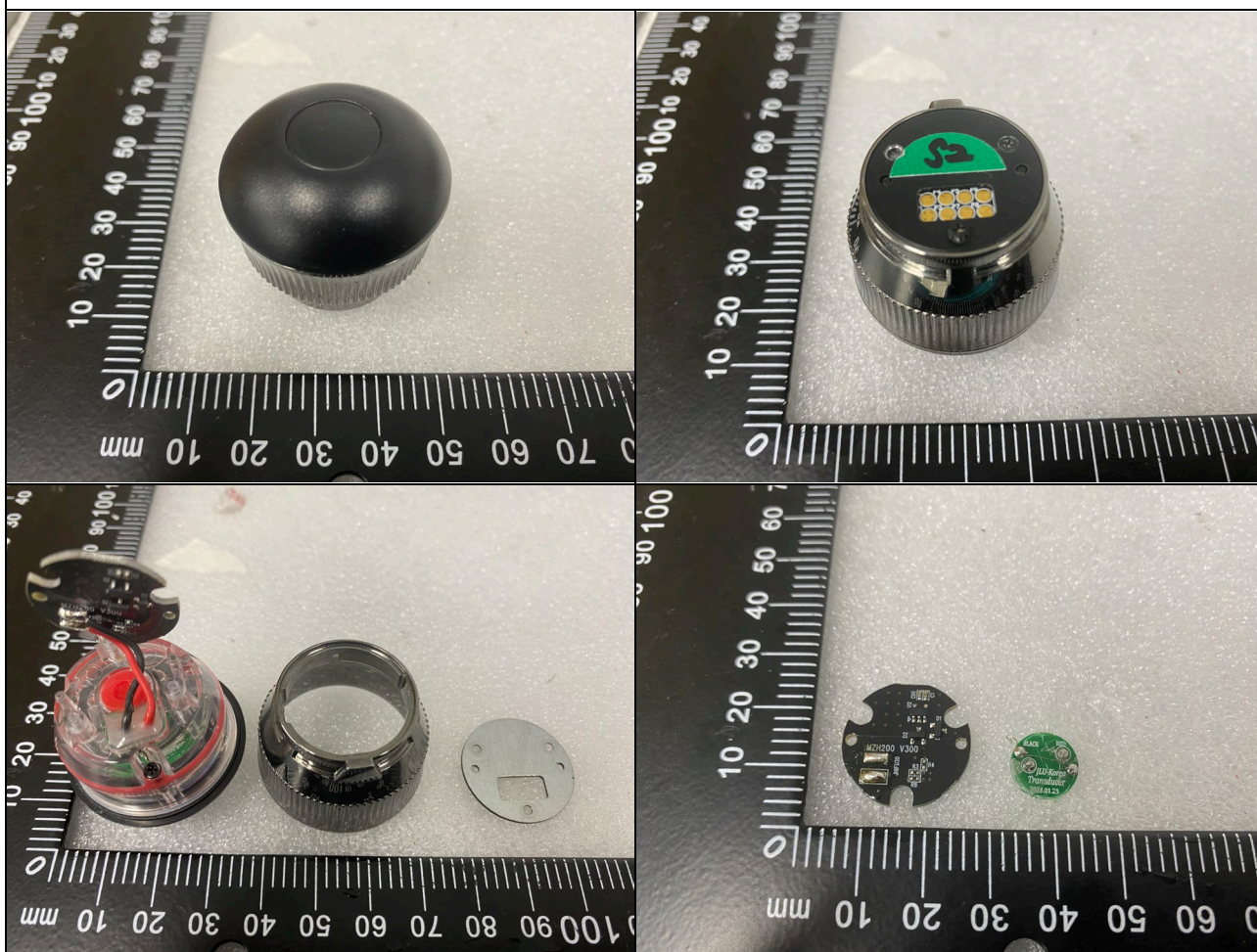
HEAD 4 (mzh-s204)
