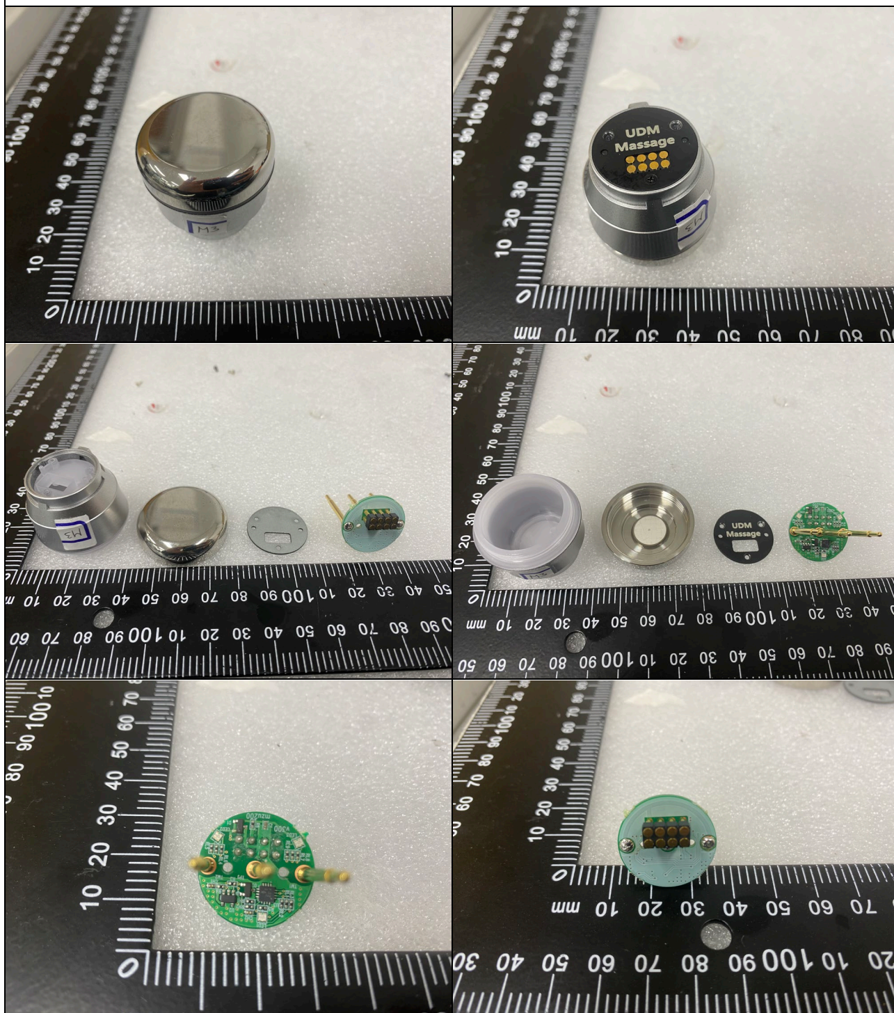
HEAD 2 (mzu-s205)
