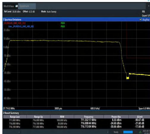
Band12-5MHz-QPSK-23155-25RB#0-PASS
