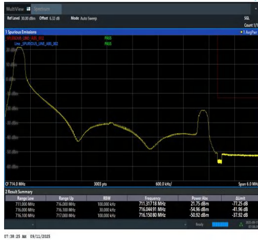
Band12-5MHz-QPSK-23155-1RB#0-PASS
