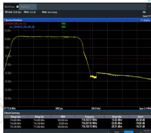
Band12-1.4MHz-16QAM-23173-6RB#0-PASS
