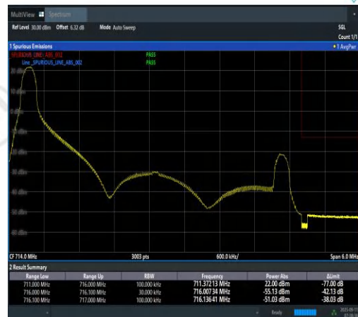
Band12-5MHz-16QAM-23155-1RB#0-PASS
