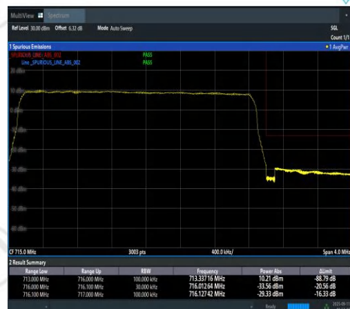
Band12-3MHz-16QAM-23165-15RB#0-PASS
