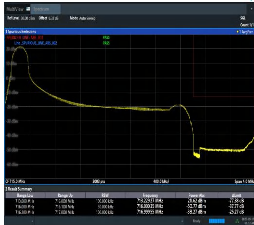
Band12-3MHz-QPSK-23165-1RB#0-PASS
