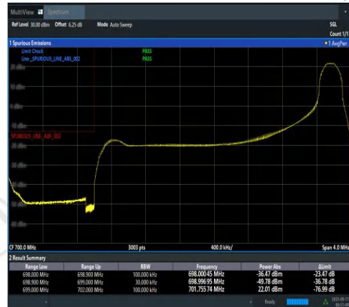
Band12-3MHz-QPSK-23025-1RB#14-PASS
