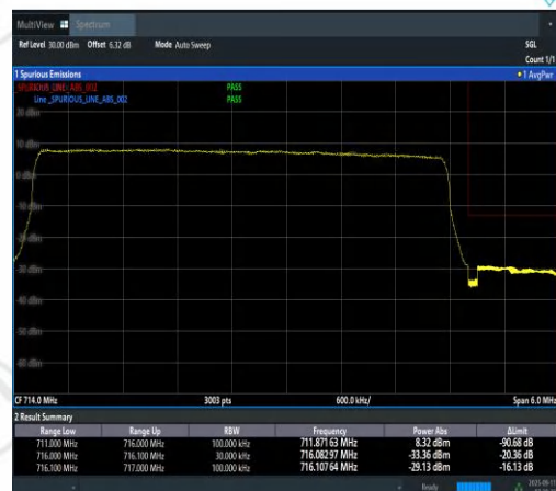
Band12-5MHz-16QAM-23155-25RB#0-PASS
