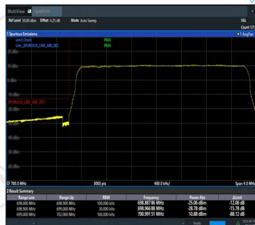
Band12-3MHz-16QAM-23025-15RB#0-PASS
