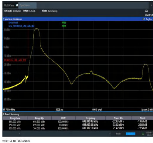
Band12-5MHz-QPSK-23035-1RB#0-PASS
