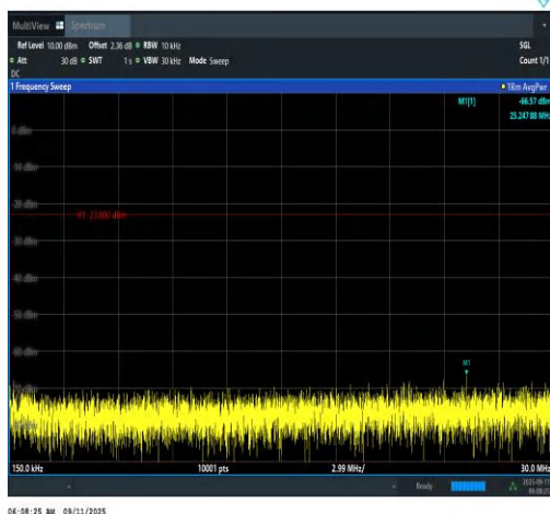
Band12-1.4MHz-16QAM-23017-1RB#0-0.15~30-PASS
