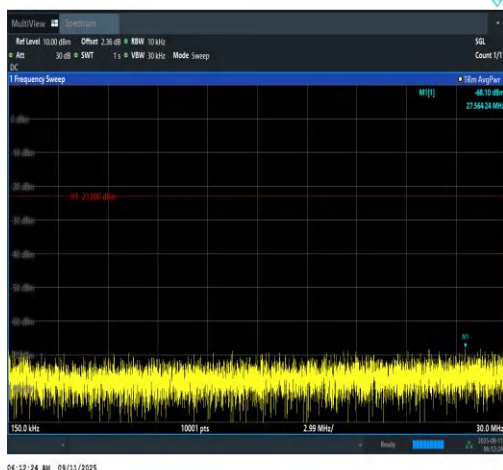
Band12-1.4MHz-16QAM-23095-1RB#0-0.15~30-PASS
