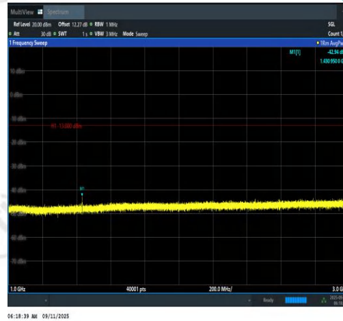
Band12-1.4MHz-QPSK-23173-6RB#0-1000~3000-PASS
