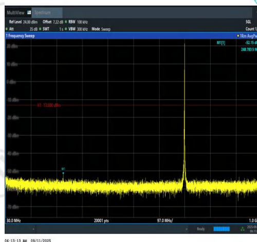
Band12-1.4MHz-QPSK-23095-1RB#5-30~1000- PASS
