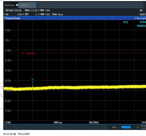
Band12-1.4MHz-QPSK-23017-6RB#0-1000~3000-PASS
