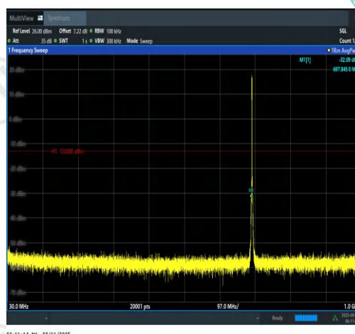
Band12-1.4MHz-16QAM-23017-6RB#0-30~1000-PASS
