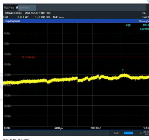
Band12-1.4MHz-16QAM-23017-6RB#0-3000~10000-PASS
