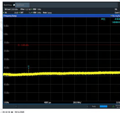
Band12-1.4MHz-QPSK-23173-1RB#0-1000~3000 0-PASS
