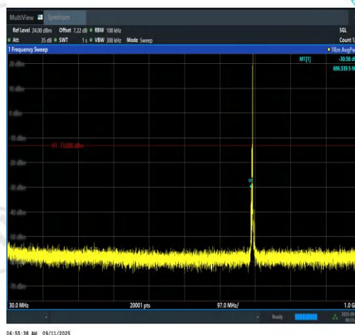
Band12-3MHz-QPSK-23025-1RB#14-30~1000-P ASS
