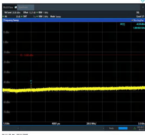
Band12-1.4MHz-16QAM-23017-6RB#0-1000~3000-PASS
