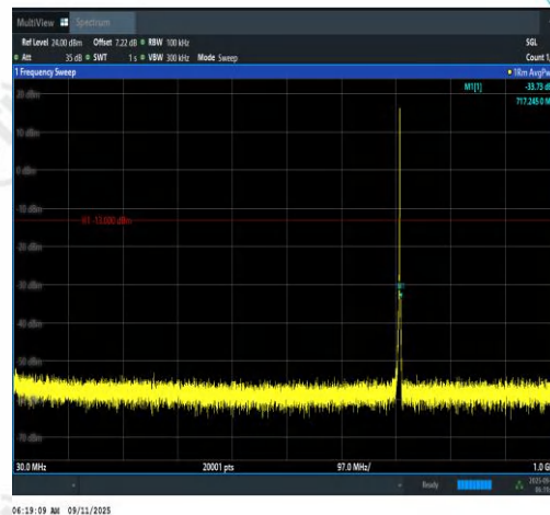
Band12-1.4MHz-16QAM-23173-6RB#0-30~1000-PASS
