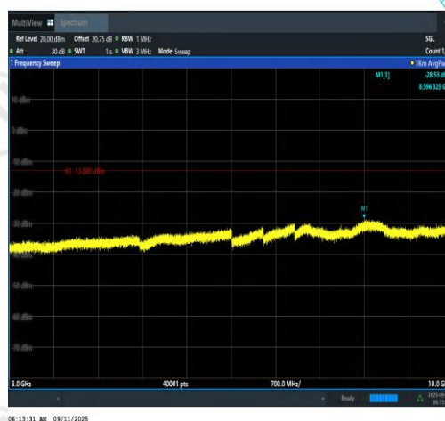
Band12-1.4MHz-QPSK-23095-1RB#5-3000~100 00-PASS
