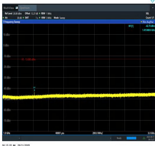
Band12-1.4MHz-QPSK-23095-1RB#5-1000~3000 0-PASS
