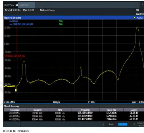
Band12-10MHz-QPSK-23060-1RB#49-PASS
