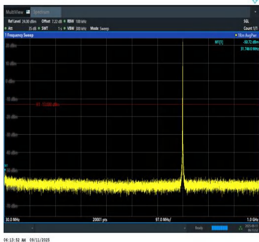
Band12-1.4MHz-16QAM-23095-1RB#5-30~1000 -PASS
