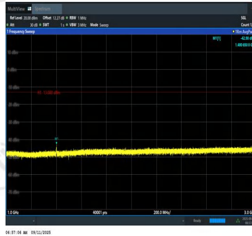
Band12-3MHz-QPSK-23025-15RB#0-1000~300 0-PASS
