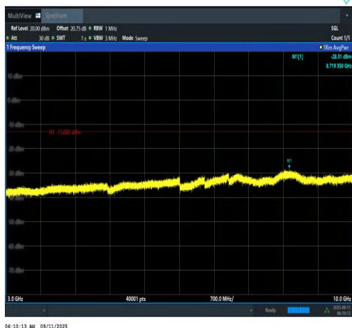
Band12-1.4MHz-16QAM-23017-1RB#5-3000~10000-PASS
