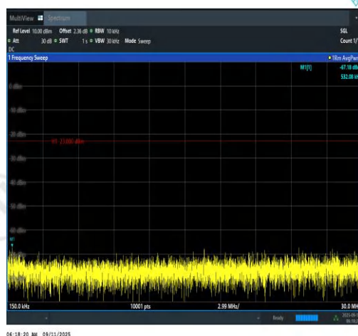
Band12-1.4MHz-QPSK-23173-6RB#0-0.15~30-P ASS
