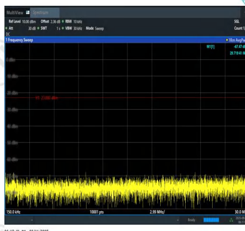
Band12-1.4MHz-16QAM-23173-1RB#5-0.15~30- PASS
