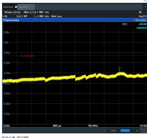
Band12-1.4MHz-QPSK-23173-1RB#0-3000~10000 00-PASS
