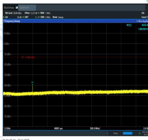
Band12-3MHz-QPSK-23025-1RB#0-1000~3000- PASS
