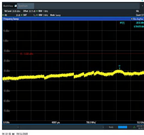
Band12-1.4MHz-QPSK-23017-6RB#0-3000~10000-PASS
