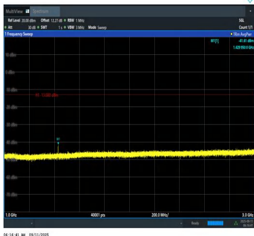
Band12-1.4MHz-16QAM-23173-1RB#0-1000~30 00-PASS
