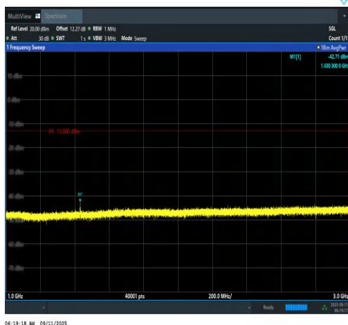
Band12-1.4MHz-16QAM-23173-6RB#0-1000~3000-PASS
