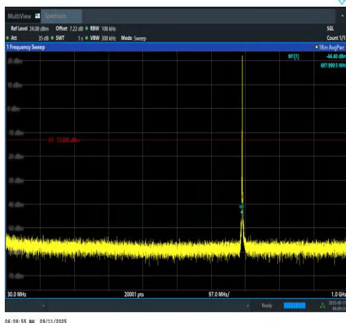
Band12-1.4MHz-16QAM-23017-1RB#5-30~1000 -PASS
