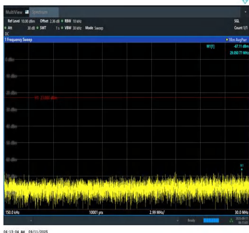
Band12-1.4MHz-QPSK-23095-1RB#5-0.15~30-P ASS
