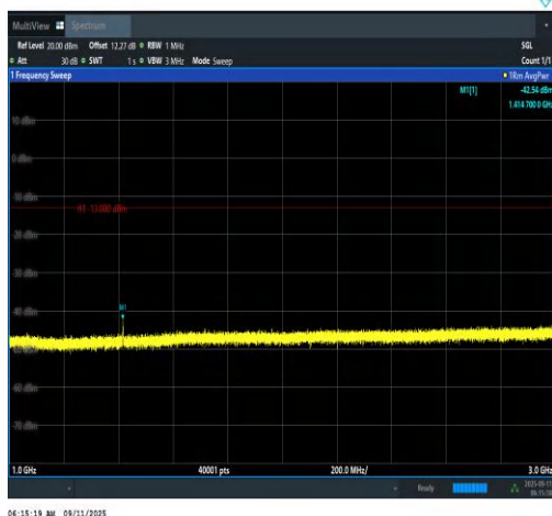
Band12-1.4MHz-16QAM-23095-6RB#0-1000~3000-PASS
