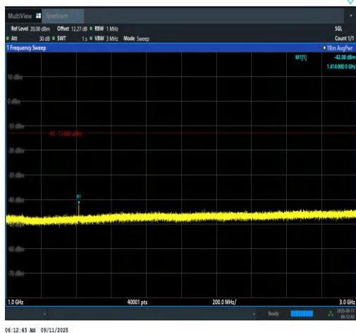
Band12-1.4MHz-16QAM-23095-1RB#0-1000~30 00-PASS
