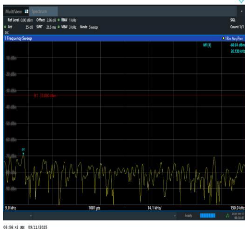
Band12-3MHz-QPSK-23025-15RB#0-0.009~0.1 5-PASS
