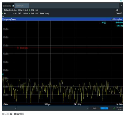
Band12-1.4MHz-QPSK-23095-6RB#0-0.009~0.1 5-PASS
