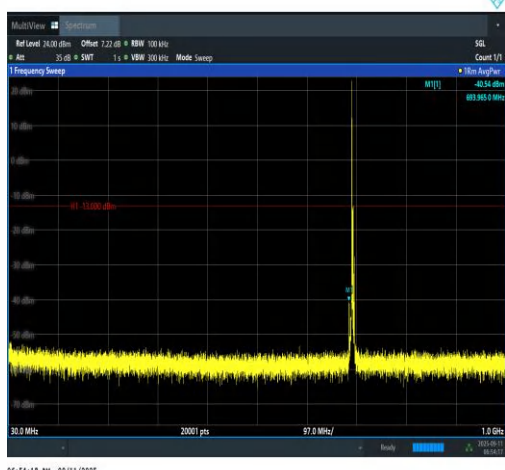
Band12-3MHz-QPSK-23025-1RB#0-30~1000-P ASS
