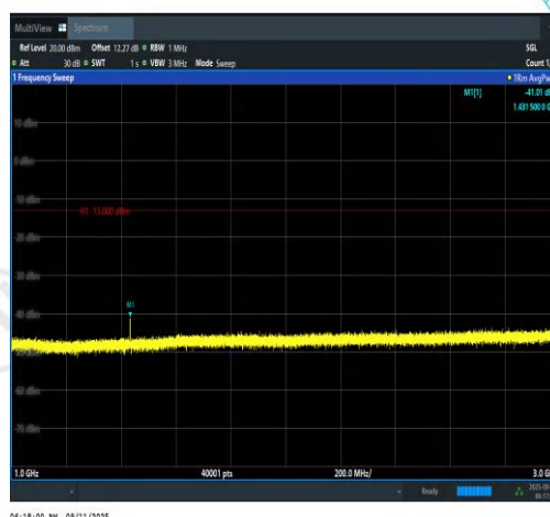
Band12-1.4MHz-16QAM-23173-1RB#5-1000~30 00-PASS
