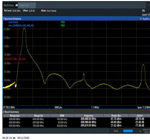
Band12-10MHz-QPSK-23060-1RB#0-PASS
