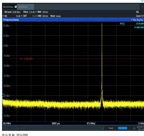
Band12-1.4MHz-QPSK-23095-1RB#0-30~1000- PASS
