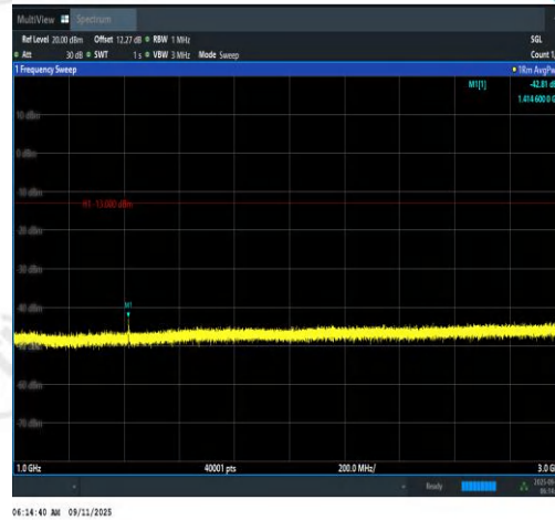
Band12-1.4MHz-QPSK-23095-6RB#0-1000~3000-PASS
