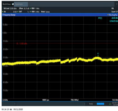
Band12-1.4MHz-16QAM-23095-1RB#5-3000~10000-PASS
