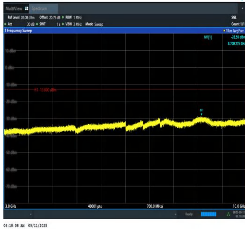
Band12-1.4MHz-16QAM-23173-1RB#5-3000~10000-PASS
