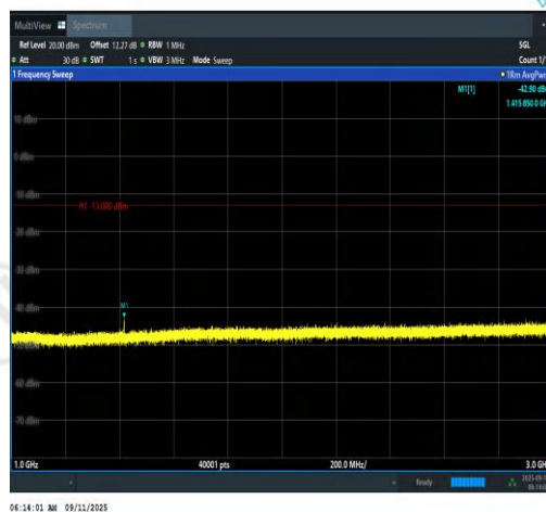
Band12-1.4MHz-16QAM-23095-1RB#5-1000~30 00-PASS
