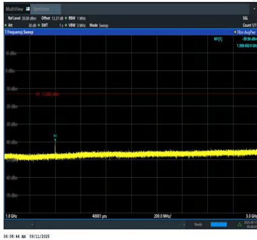
Band12-1.4MHz-16QAM-23017-1RB#0-1000~30 00-PASS
