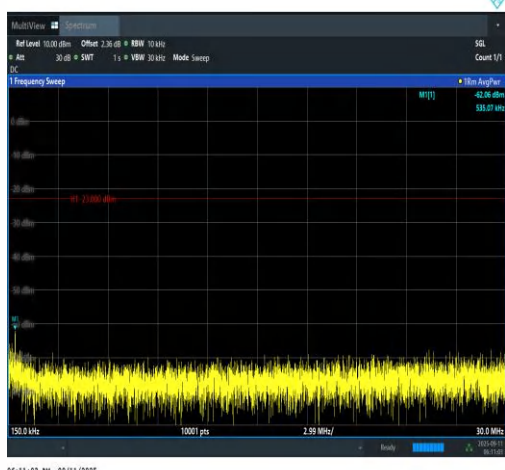
Band12-1.4MHz-16QAM-23017-6RB#0-0.15~30-PASS
