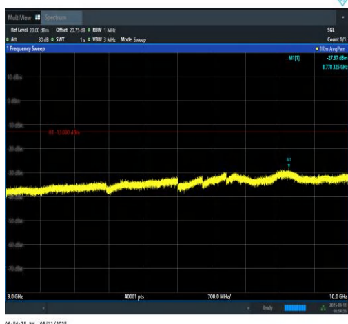
Band12-3MHz-QPSK-23025-1RB#0-3000~1000 0-PASS
