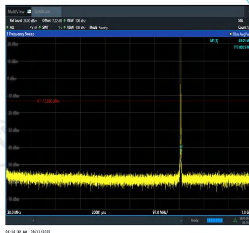
Band12-1.4MHz-16QAM-23173-1RB#0-30~1000-PASS
