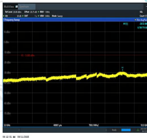
Band12-1.4MHz-16QAM-23095-1RB#0-3000~10 000-PASS
