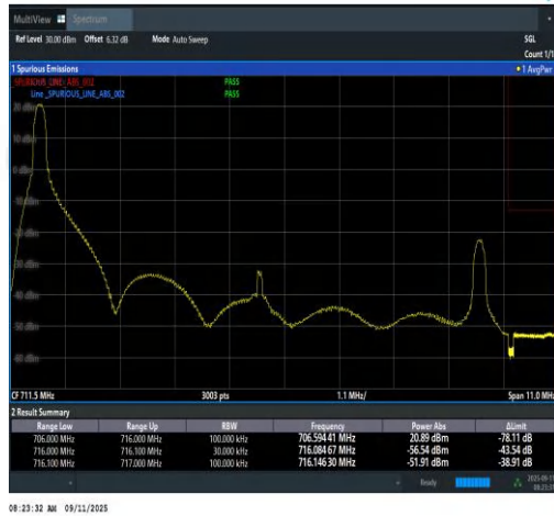
Band12-10MHz-QPSK-23130-1RB#0-PASS
