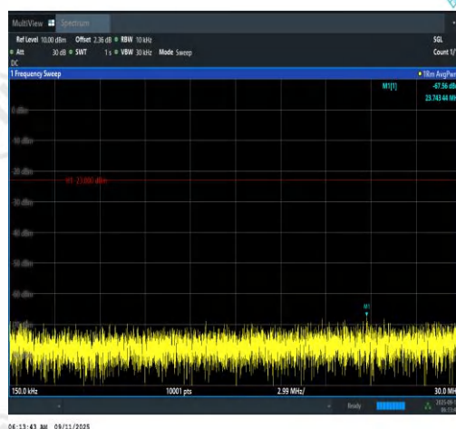
Band12-1.4MHz-16QAM-23095-1RB#5-0.15~30- PASS
