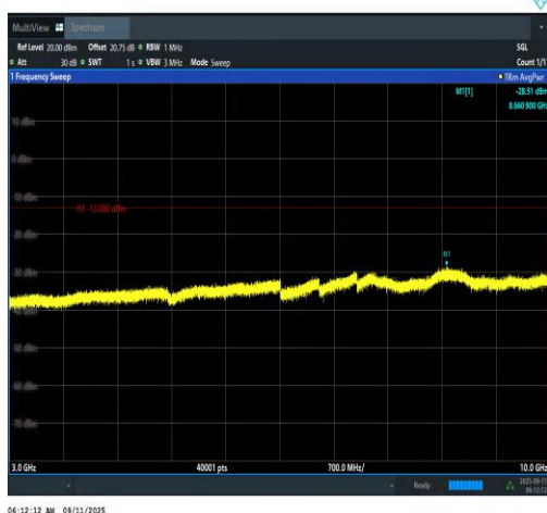
Band12-1.4MHz-QPSK-23095-1RB#0-3000~100 00-PASS
