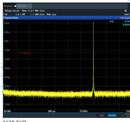
Band12-1.4MHz-16QAM-23095-1RB#0-30~1000-PASS
