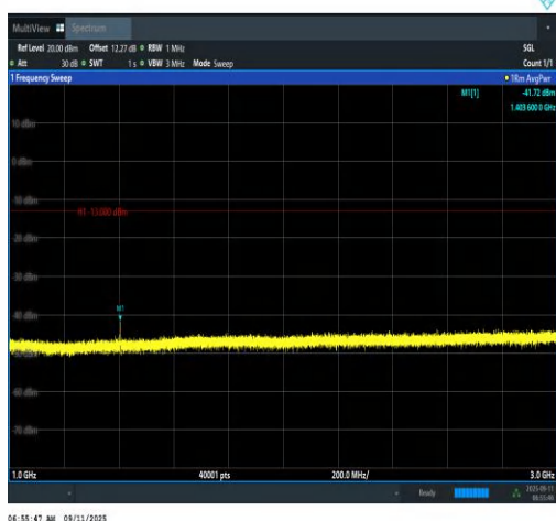
Band12-3MHz-QPSK-23025-1RB#14-1000~300 0-PASS
