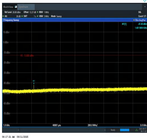
Band12-1.4MHz-QPSK-23173-1RB#5-1000~3000-P 0-PASS
