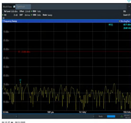
Band12-1.4MHz-16QAM-23095-1RB#5-0.009~0. 15-PASS
