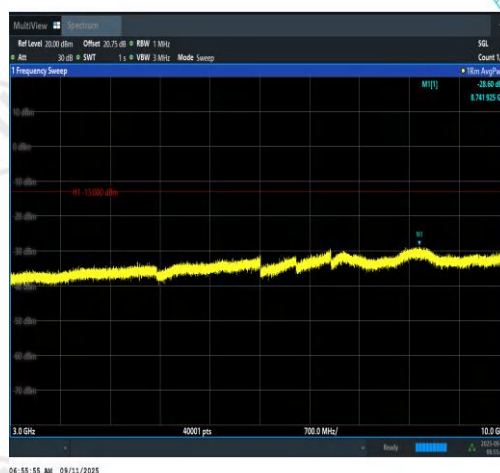
Band12-3MHz-QPSK-23025-1RB#14-3000~100 00-PASS
