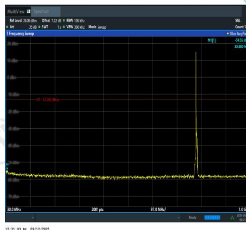
Band13-5MHz-16QAM-23255-1RB#0-30~1000-P ASS
