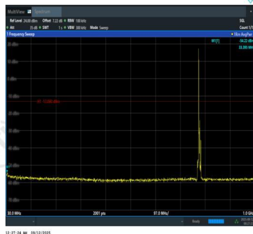
Band13-5MHz-16QAM-23230-1RB#0-30~1000-P ASS
