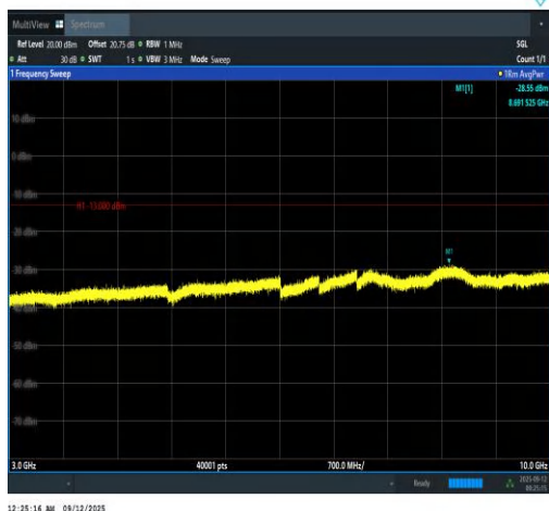
Band13-5MHz-16QAM-23205-1RB#24-3000~10000-PASS
