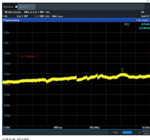
Band13-5MHz-16QAM-23230-1RB#24-3000~10000-PASS
