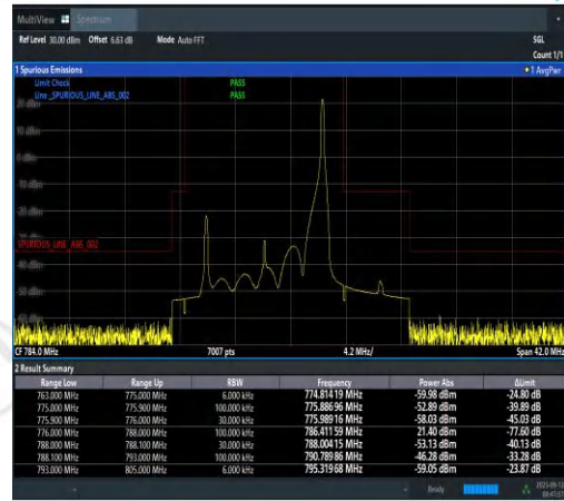
Band13-10MHz-QPSK-23230-1RB#49-PASS
