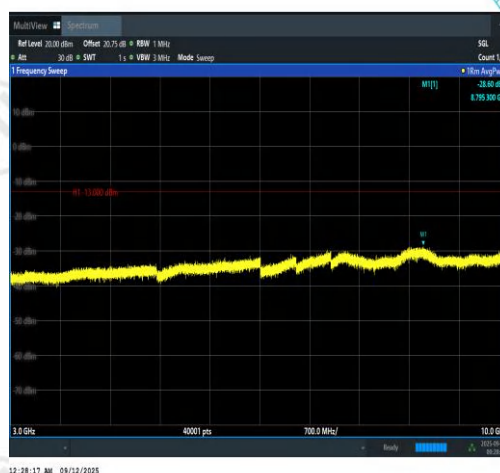
Band13-5MHz-QPSK-23230-1RB#24-3000~100 00-PASS
