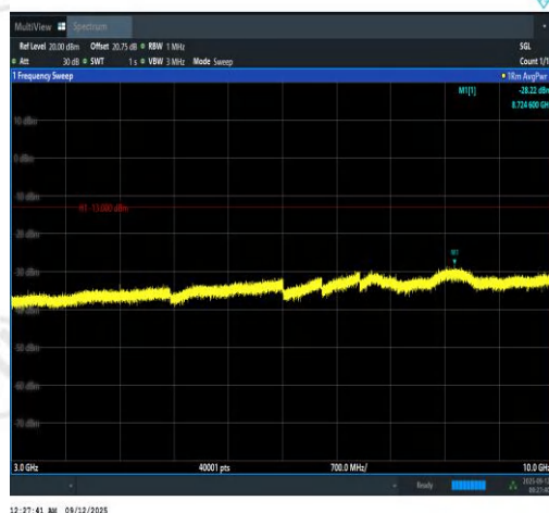
Band13-5MHz-16QAM-23230-1RB#0-3000~100 00-PASS
