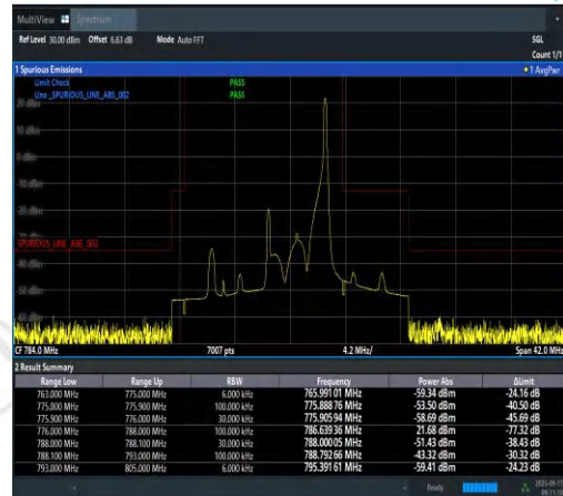
Band13-5MHz-QPSK-23255-1RB#24-PASS
