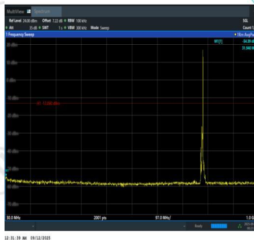
Band13-5MHz-QPSK-23255-1RB#24-30~1000-P ASS
