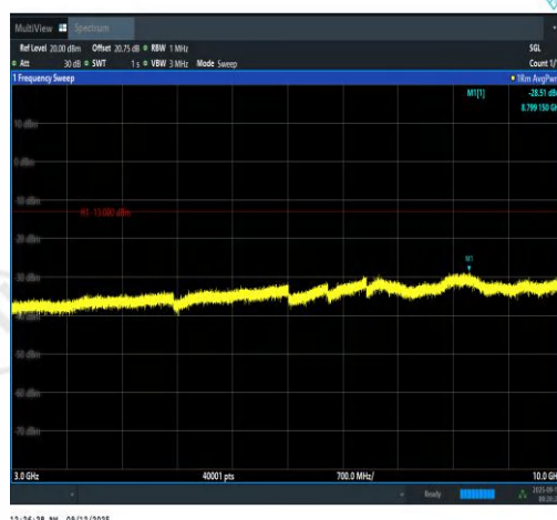
Band13-5MHz-16QAM-23205-25RB#0-3000~10000-PASS
