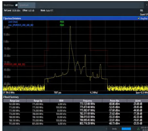
Band13-5MHz-QPSK-23255-1RB#0-PASS
