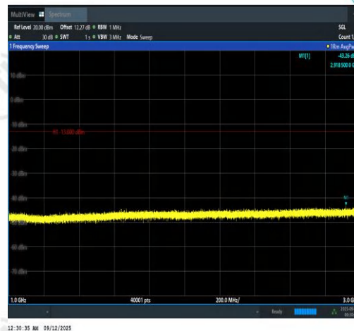
Band13-5MHz-QPSK-23255-1RB#0-1000~3000- PASS
