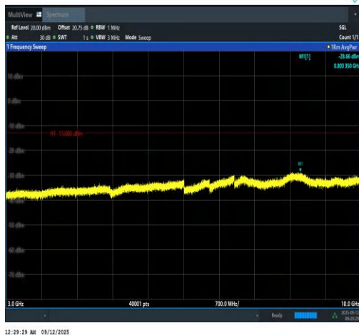
Band13-5MHz-QPSK-23230-25RB#0-3000~100 00-PASS
