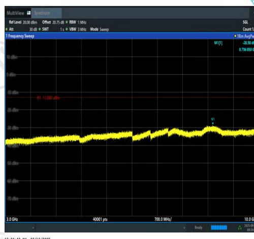
Band13-5MHz-QPSK-23205-1RB#24-3000~100 00-PASS
