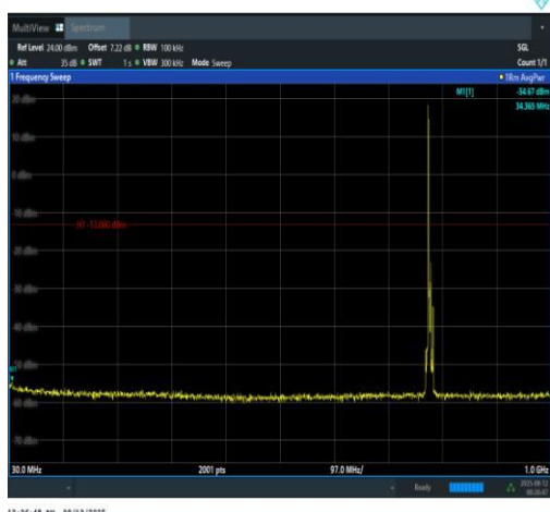
Band13-5MHz-QPSK-23230-1RB#0-30~1000-P ASS
