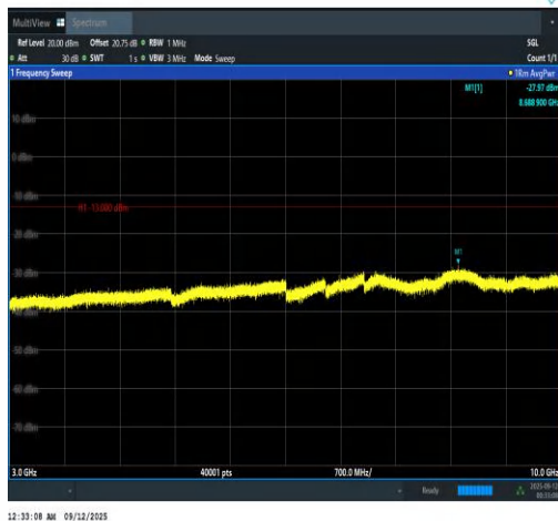
Band13-5MHz-QPSK-23255-25RB#0-3000~100 00-PASS
