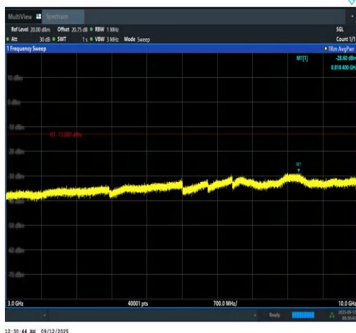
Band13-5MHz-QPSK-23255-1RB#0-3000~1000 0-PASS
