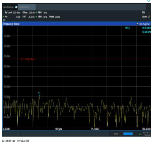
Band13-5MHz-QPSK-23230-25RB#0-0.009~0.1 5-PASS
