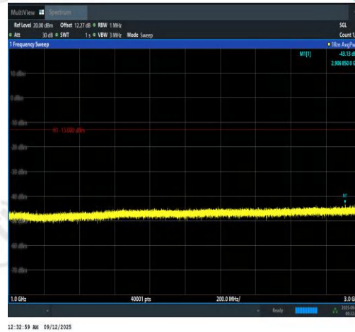
Band13-5MHz-QPSK-23255-25RB#0-1000~300 0-PASS
