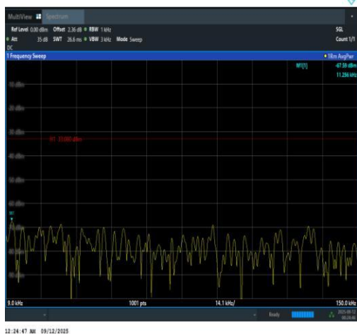
Band13-5MHz-16QAM-23205-1RB#24-0.009~0. 15-PASS
