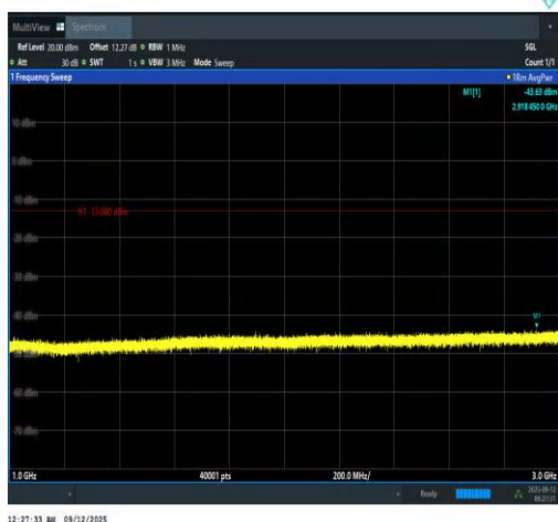
Band13-5MHz-16QAM-23230-1RB#0-1000~300 0-PASS
