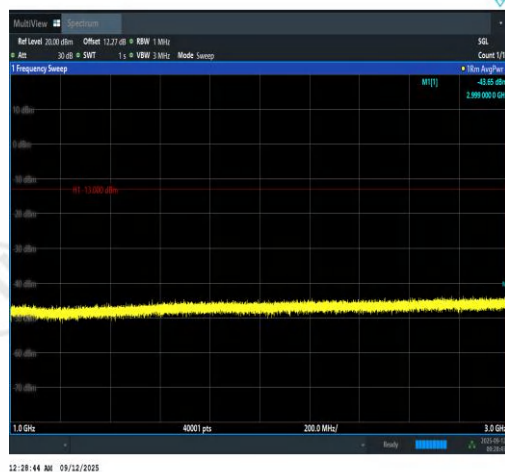
Band13-5MHz-16QAM-23230-1RB#24-1000~30 00-PASS
