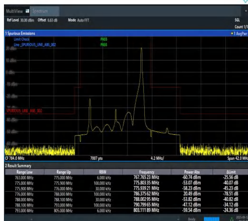
Band13-10MHz-16QAM-23230-1RB#49-PASS
