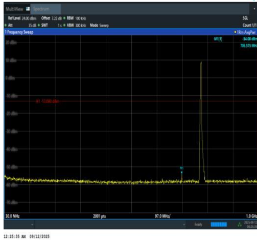
Band13-5MHz-QPSK-23205-25RB#0-30~1000-P ASS
