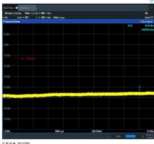
Band13-5MHz-QPSK-23230-1RB#24-1000~300 0-PASS
