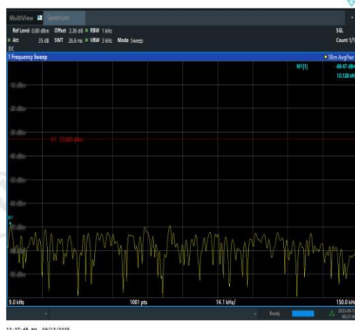
Band13-5MHz-QPSK-23230-1RB#24-0.009~0.1 5-PASS
