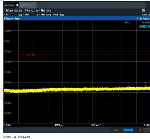
Band13-5MHz-QPSK-23205-25RB#0-1000~300 0-PASS
