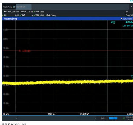
Band13-5MHz-QPSK-23255-1RB#24-1000~300 0-PASS
