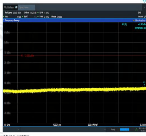
Band13-5MHz-QPSK-23230-1RB#0-1000~3000- PASS
