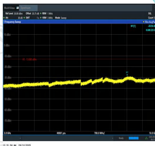
Band13-5MHz-QPSK-23255-1RB#24-3000~100 00-PASS
