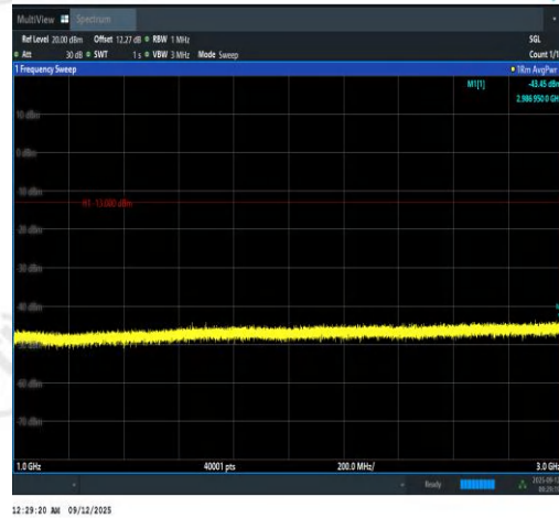
Band13-5MHz-QPSK-23230-25RB#0-1000~300 0-PASS
