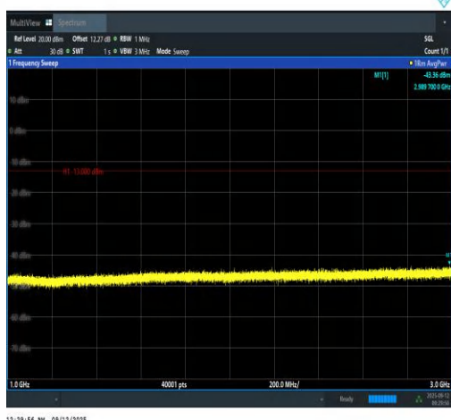
Band13-5MHz-16QAM-23230-25RB#0-1000~3000-PASS
