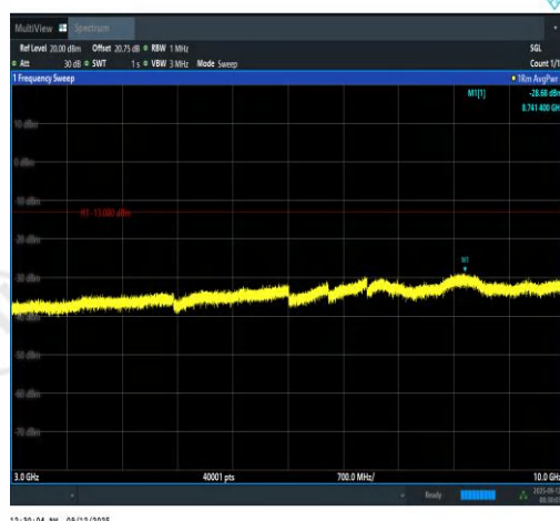
Band13-5MHz-16QAM-23230-25RB#0-3000~10000-PASS
