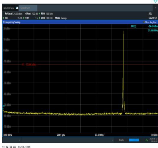
Band13-5MHz-16QAM-23205-1RB#24-30~1000- PASS
