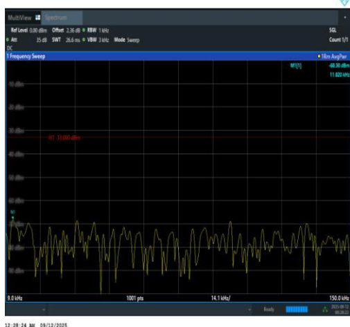
Band13-5MHz-16QAM-23230-1RB#24-0.009~0. 15-PASS
