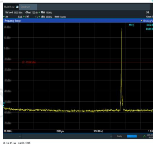
Band13-5MHz-QPSK-23205-1RB#24-30~1000-P ASS
