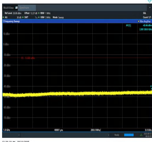
Band13-5MHz-16QAM-23205-25RB#0-1000~3000-PASS
