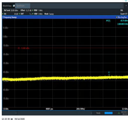
Band13-5MHz-16QAM-23205-1RB#0-1000~300 0-PASS
