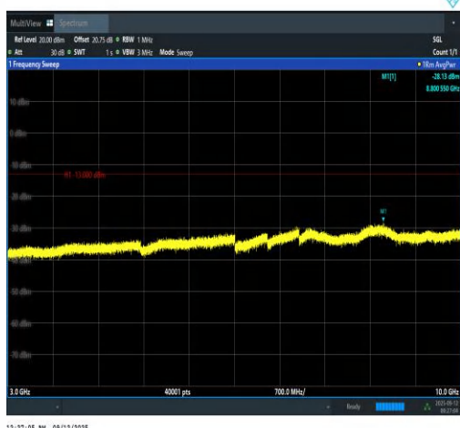
Band13-5MHz-QPSK-23230-1RB#0-3000~1000 0-PASS
